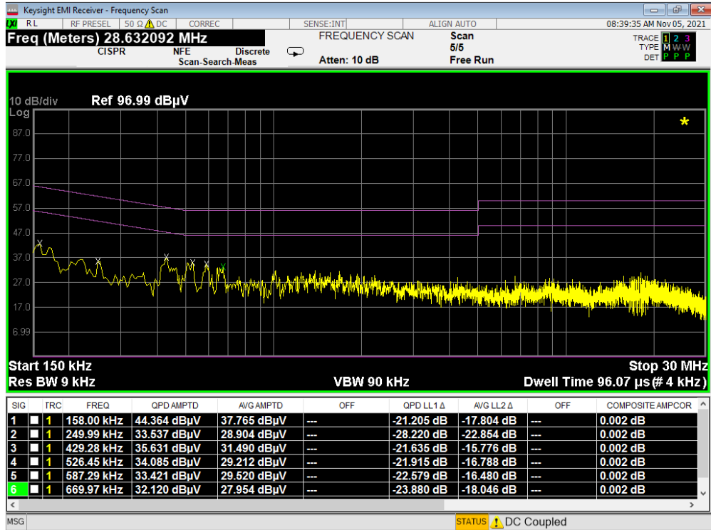
Plot 7-6. Line-Conducted Test Plot (L1) w/Antenna Terminated
