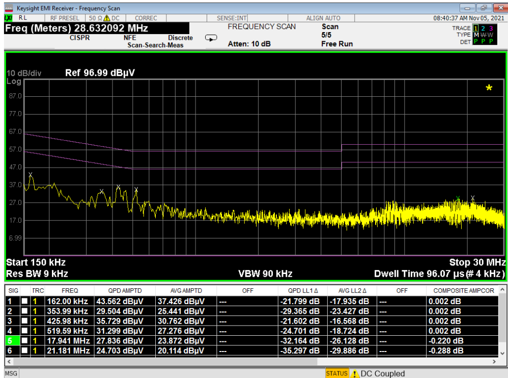
Plot 7-7. Line-Conducted Test Plot (N) w/Antenna Terminated
