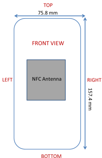
Figure E-2 NFC Antenna Locations
