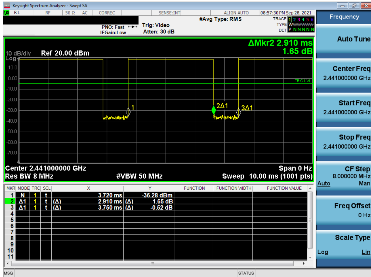
Bluetooth Antenna 1 Transmission Plot
