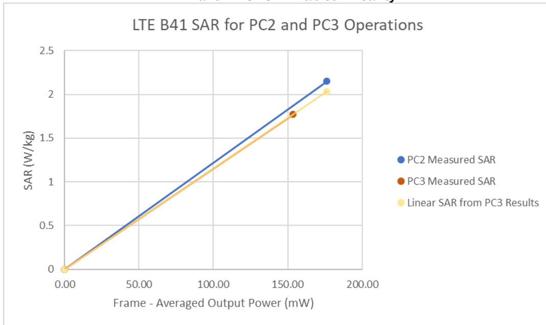
Figure 13-8 LTE Band 41 ULCA Phablet Linearity
