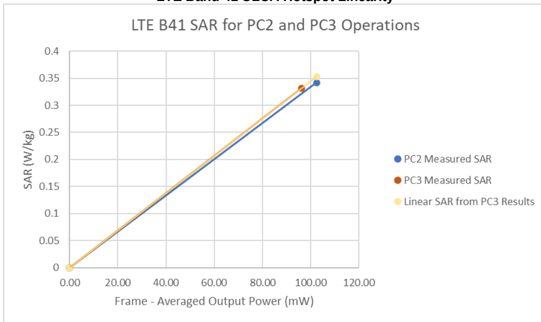
Figure 13-6 LTE Band 41 ULCA Hotspot Linearity
