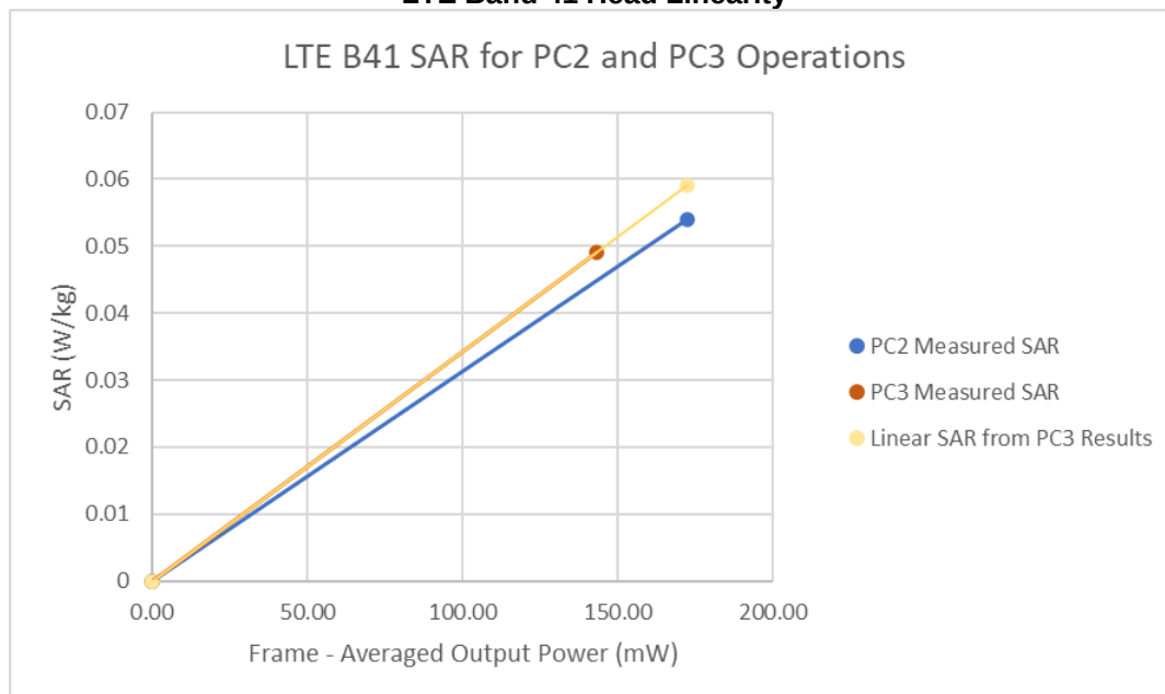
Figure 13-1 LTE Band 41 Head Linearity
