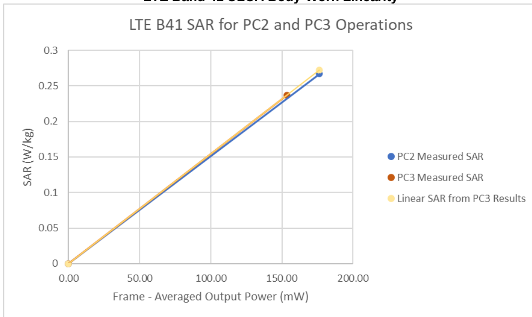
Figure 13-4 LTE Band 41 ULCA Body-Worn Linearity
