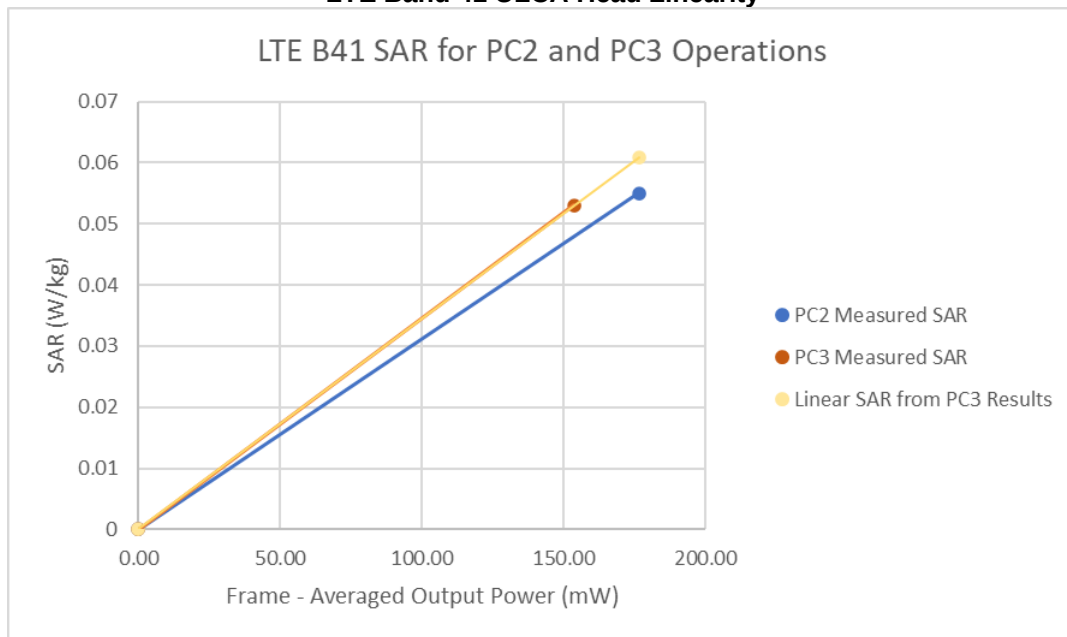
Figure 13-2 LTE Band 41 ULCA Head Linearity
