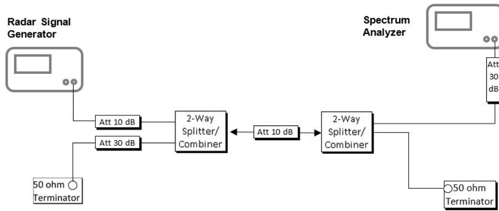
Figure 7-2. Radar Waveform Calibration
