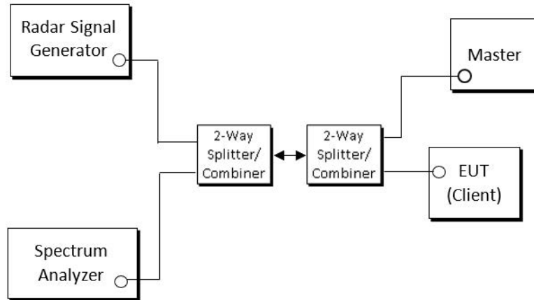
Figure 8-1. Test Setup
