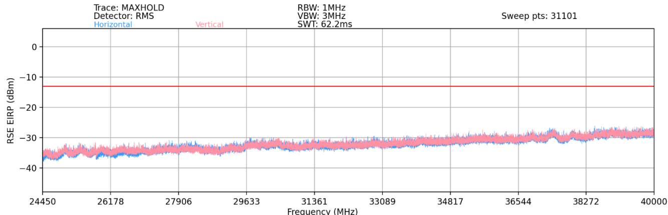
Plot 7-92. Ant 1 - n258-R1 Radiated Spurious Plot (1CC QPSK Mid Channel 2Tx – EN-DC Anchor Band 2)
