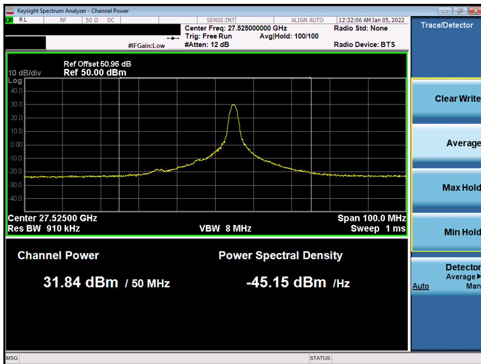
Plot 7-77. Ant 1 EIRP Plot (Band n261 – 50MHz-1CC – QPSK – Low Channel)
