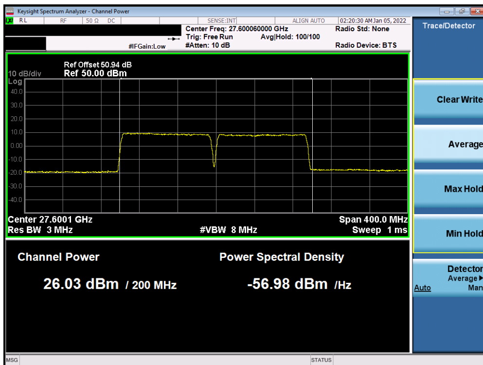
Plot 7-82. Ant 2 EIRP Plot (Band n261 – 100MHz-2CC – pi/2-BPSK – Low Channel)
