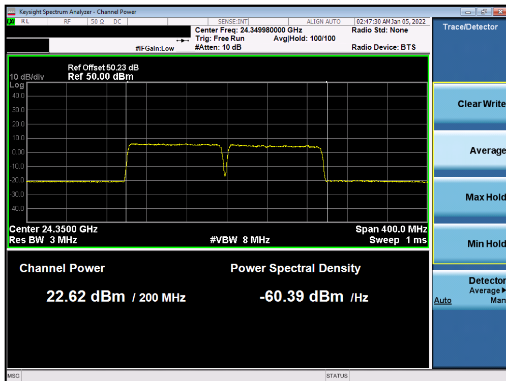
Plot 7-70. Ant 2 EIRP Plot (Band n258-R1 - 100MHz-2CC - QPSK - Mid Channel)
