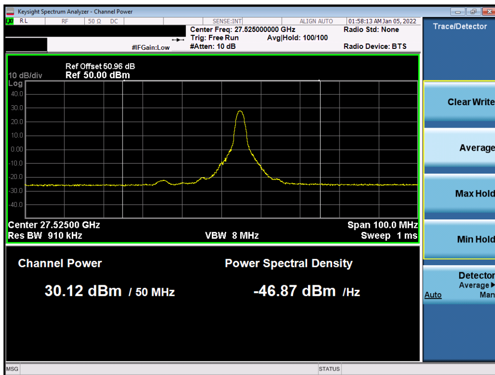
Plot 7-80. Ant 2 EIRP Plot (Band n261 – 50MHz-1CC – QPSK – Low Channel)
