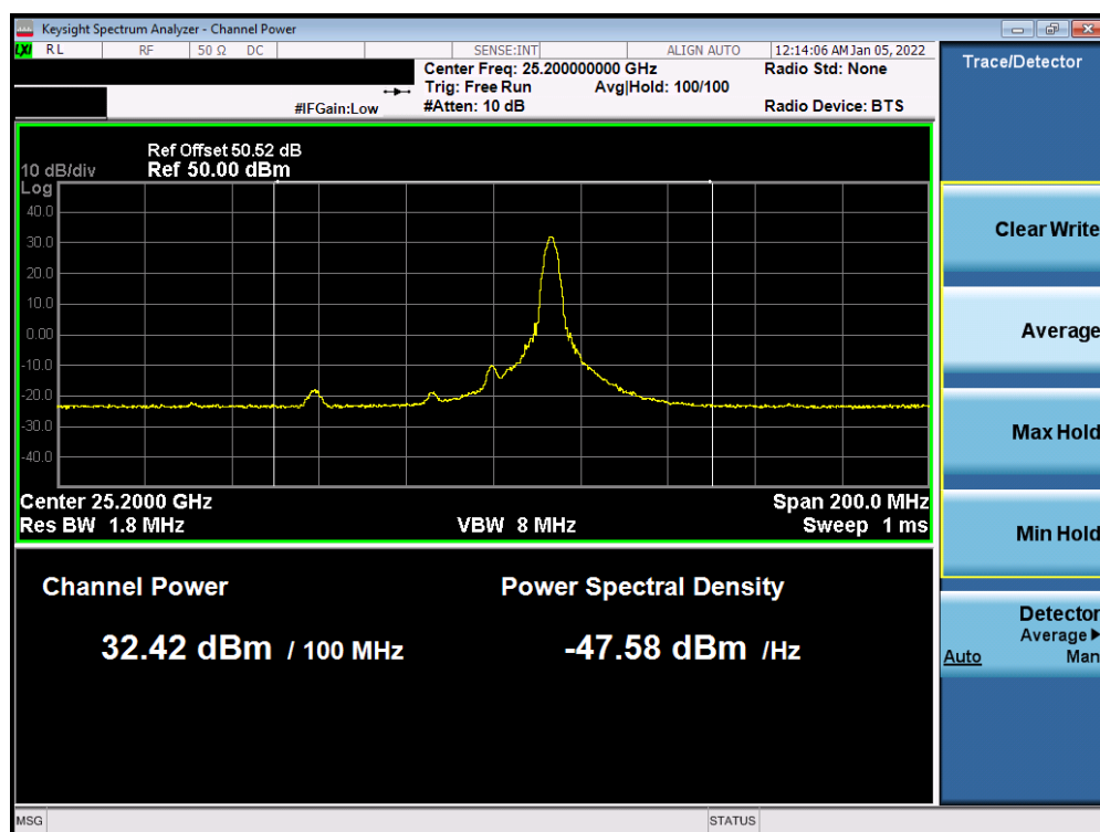
Plot 7-72. Ant 1 EIRP Plot (Band n258-R2 – 100MHz-1CC – QPSK – High Channel)
