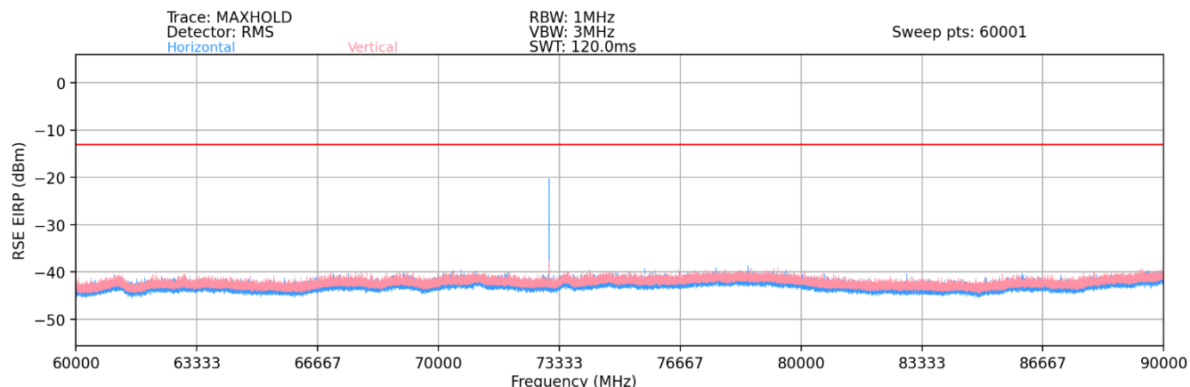
Plot 7-94. Ant 1 - n258-R1 Radiated Spurious Plot (1CC QPSK Mid Channel 2Tx – EN-DC Anchor Band 2)
