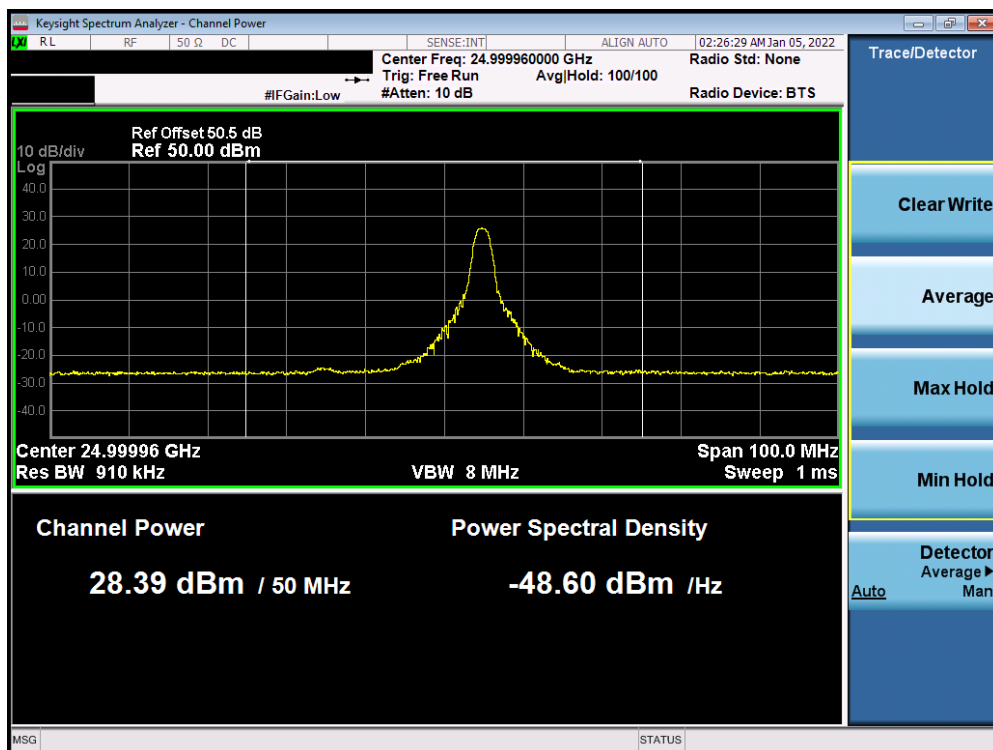
Plot 7-74. Ant 2 EIRP Plot (Band n258-R2 – 50MHz-1CC – QPSK – Mid Channel)
