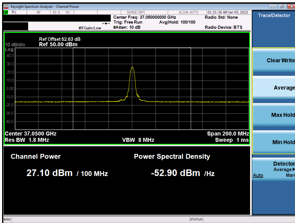
Plot 7-87. Ant 2 EIRP Plot (Band n260 – 100MHz-1CC – QPSK – Low Channel)
