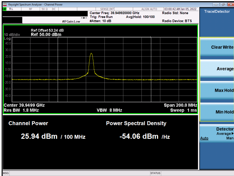
Plot 7-84. Ant 1 EIRP Plot (Band n260 – 100MHz-1CC – QPSK – High Channel)
