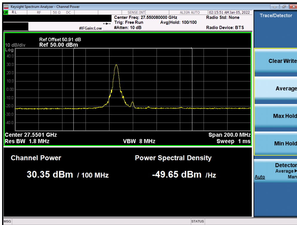
Plot 7-81. Ant 2 EIRP Plot (Band n261 – 100MHz-1CC – QPSK – Low Channel)
