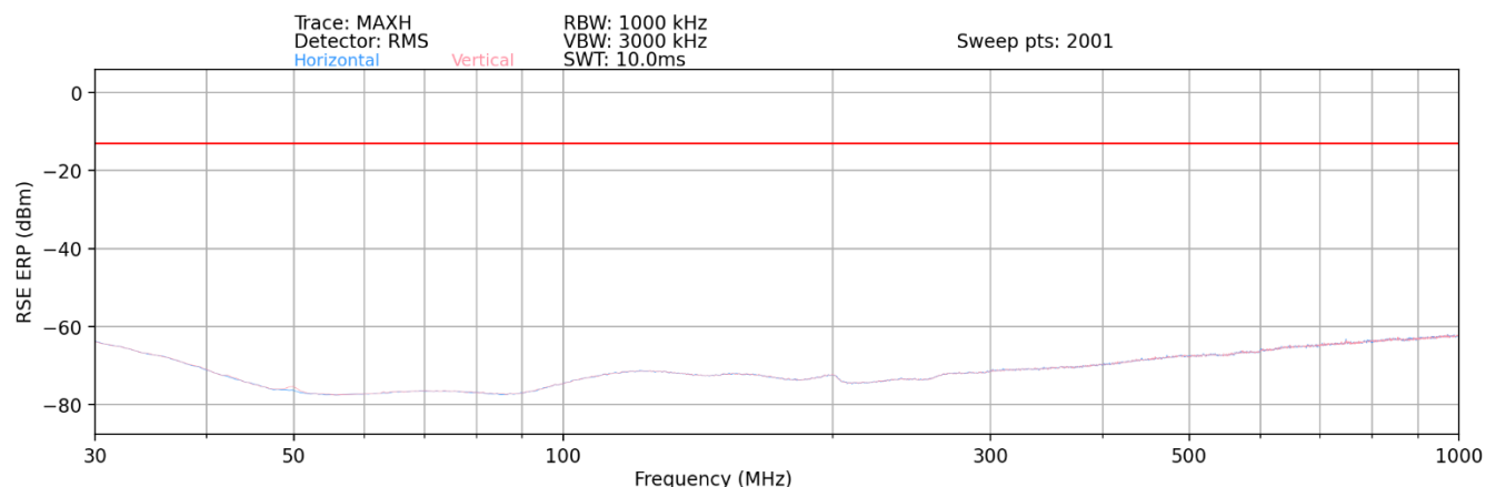
Plot 7-89. Ant 1 - n258-R1 Radiated Spurious Plot (1CC QPSK Mid Channel 2Tx – EN-DC Anchor Band 2)
