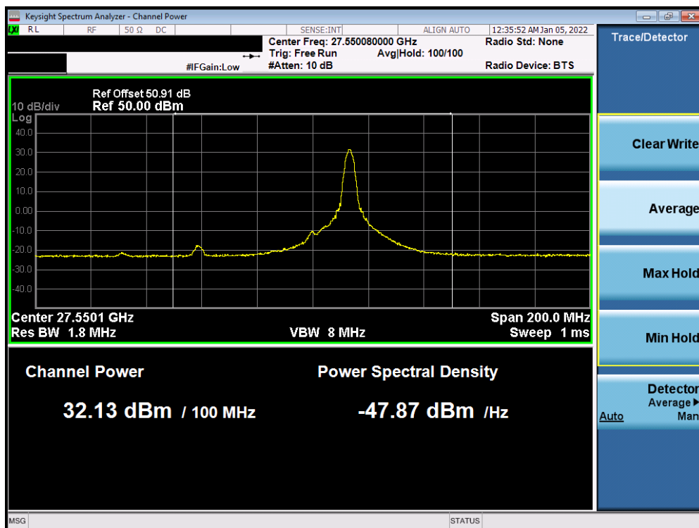
Plot 7-78. Ant 1 EIRP Plot (Band n261 – 100MHz-1CC – QPSK – Low Channel)
