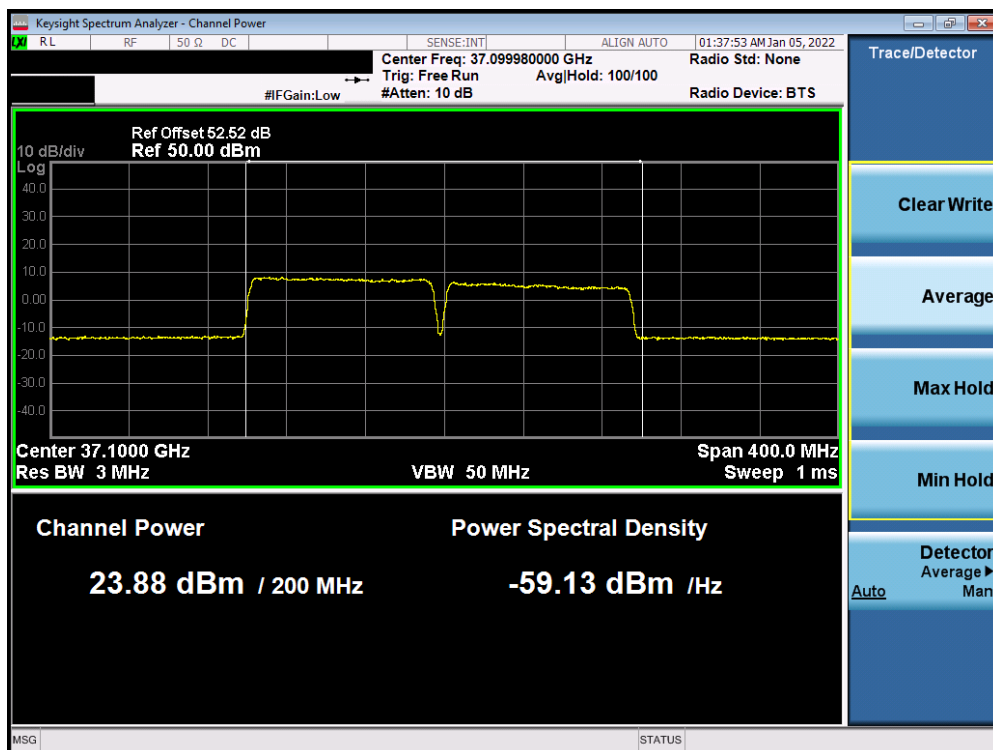
Plot 7-88. Ant 2 EIRP Plot (Band n260 – 100MHz-2CC – pi/2-BPSK – Low Channel)
