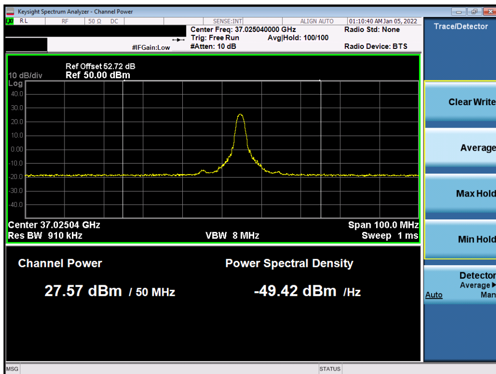
Plot 7-86. Ant 2 EIRP Plot (Band n260 – 50MHz-1CC – pi/2-BPSK – Low Channel)
