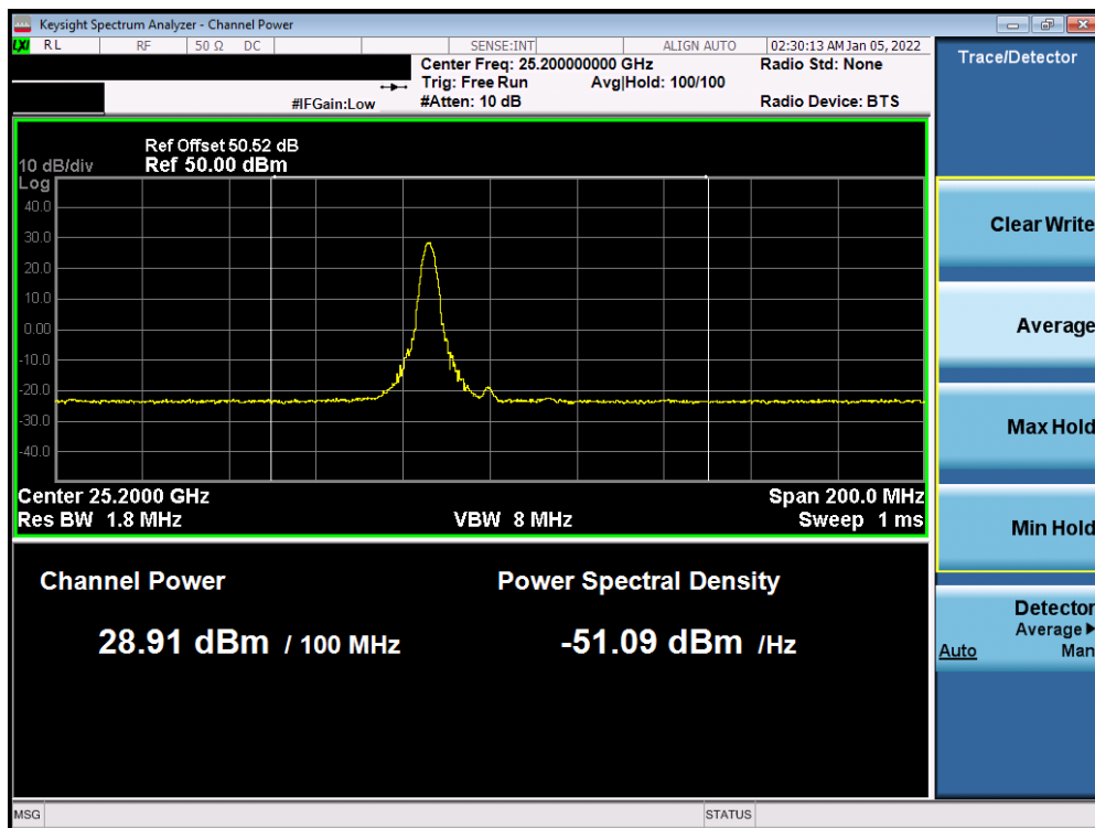
Plot 7-75. Ant 2 EIRP Plot (Band n258-R2 – 100MHz-1CC – QPSK – High Channel)
