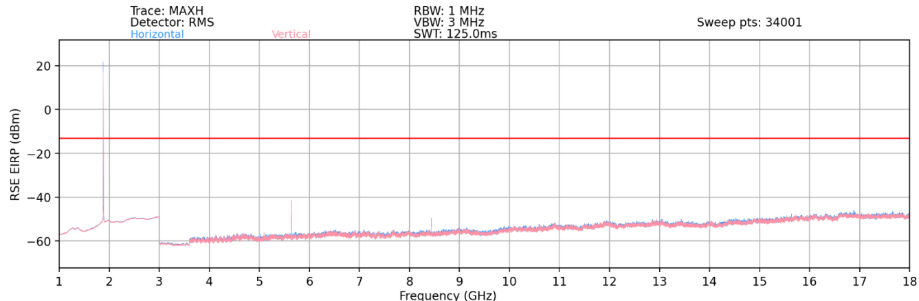
Plot 7-90. Ant 1 - n258-R1 Radiated Spurious Plot (1CC QPSK Mid Channel 2Tx – EN-DC Anchor Band 2)
