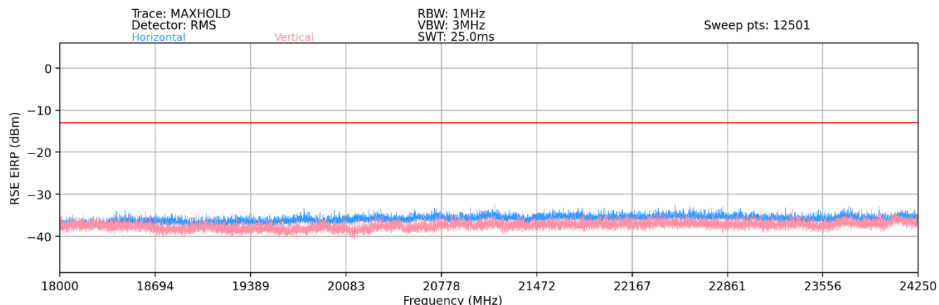
Plot 7-91. Ant 1 - n258-R1 Radiated Spurious Plot (1CC QPSK Mid Channel 2Tx – EN-DC Anchor Band 2)
