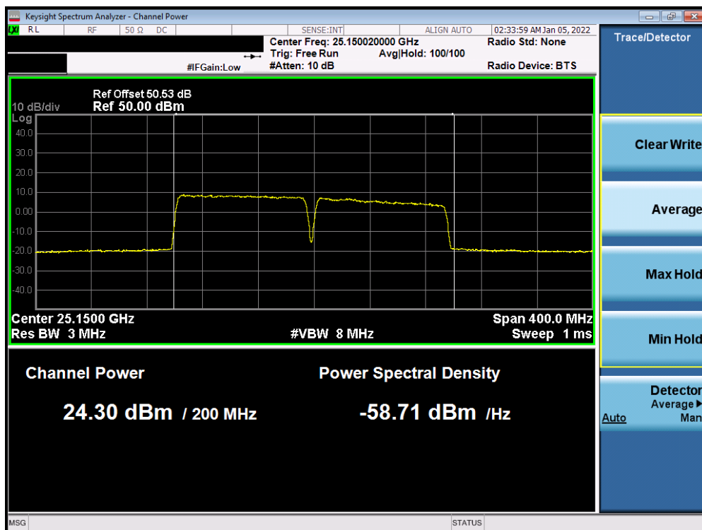
Plot 7-76. Ant 2 EIRP Plot (Band n258-R2 – 100MHz-2CC – pi/2-BPSK – High Channel)
