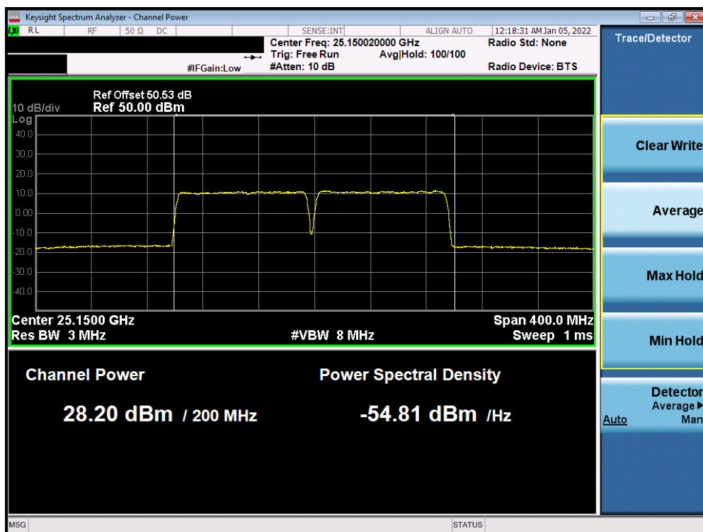
Plot 7-73. Ant 1 EIRP Plot (Band n258-R2 – 100MHz-2CC – QPSK – High Channel)
