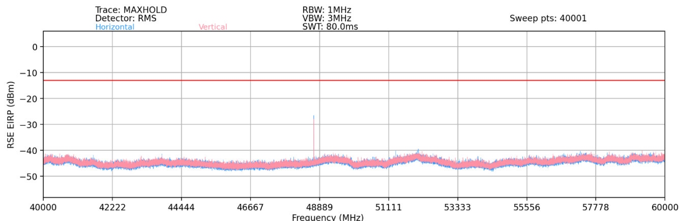
Plot 7-93. Ant 1 - n258-R1 Radiated Spurious Plot (1CC QPSK Mid Channel 2Tx – EN-DC Anchor Band 2)
