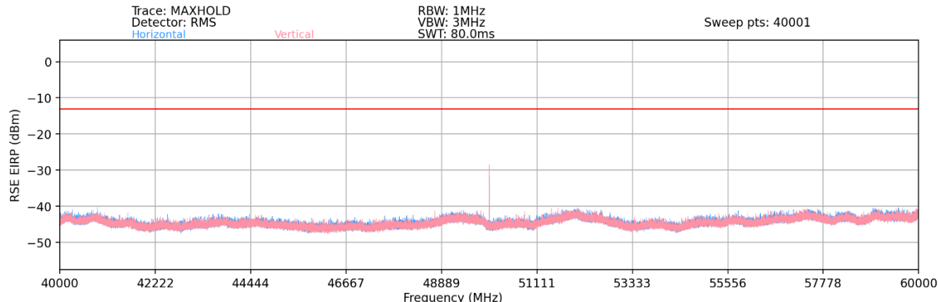
Plot 7-114. Ant 2 - n258-R2 Radiated Spurious Plot (1CC QPSK Mid Channel 2Tx – EN-DC Anchor Band 2)
