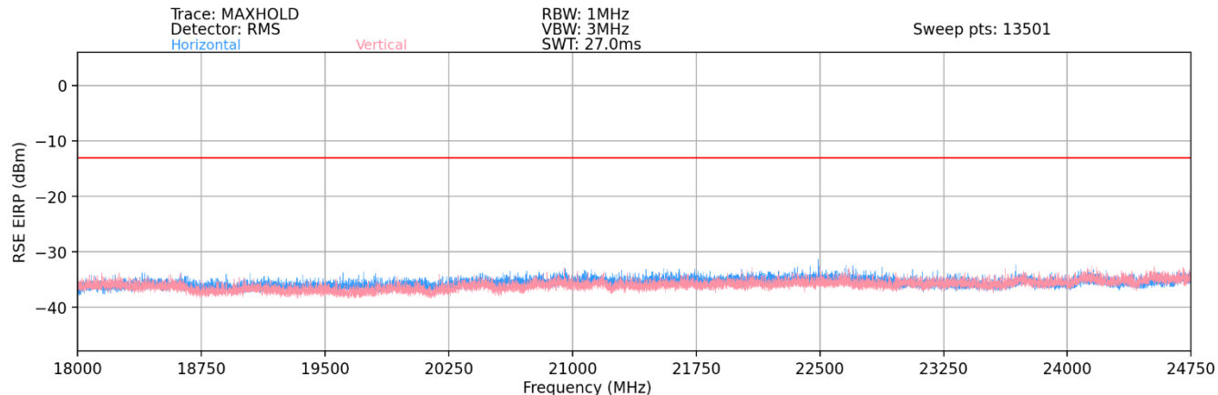
Plot 7-105. Ant 1 - n258-R2 Radiated Spurious Plot (1CC QPSK Mid Channel 2Tx – EN-DC Anchor Band 2)
