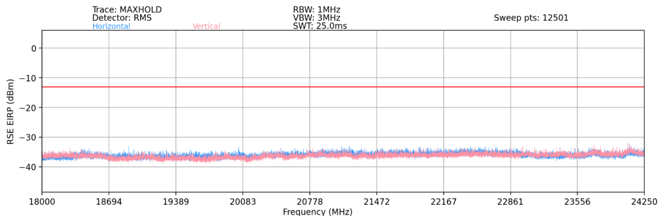
Plot 7-98. Ant 2 - n258-R1 Radiated Spurious Plot (1CC QPSK Mid Channel 2Tx – EN-DC Anchor Band 2)
