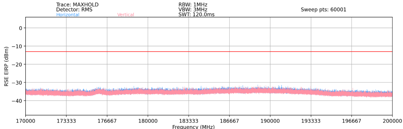
Plot 7-138. Ant 1 - n260 Radiated Spurious Plot (1CC QPSK Mid Channel 2Tx – EN-DC Anchor Band 2)
