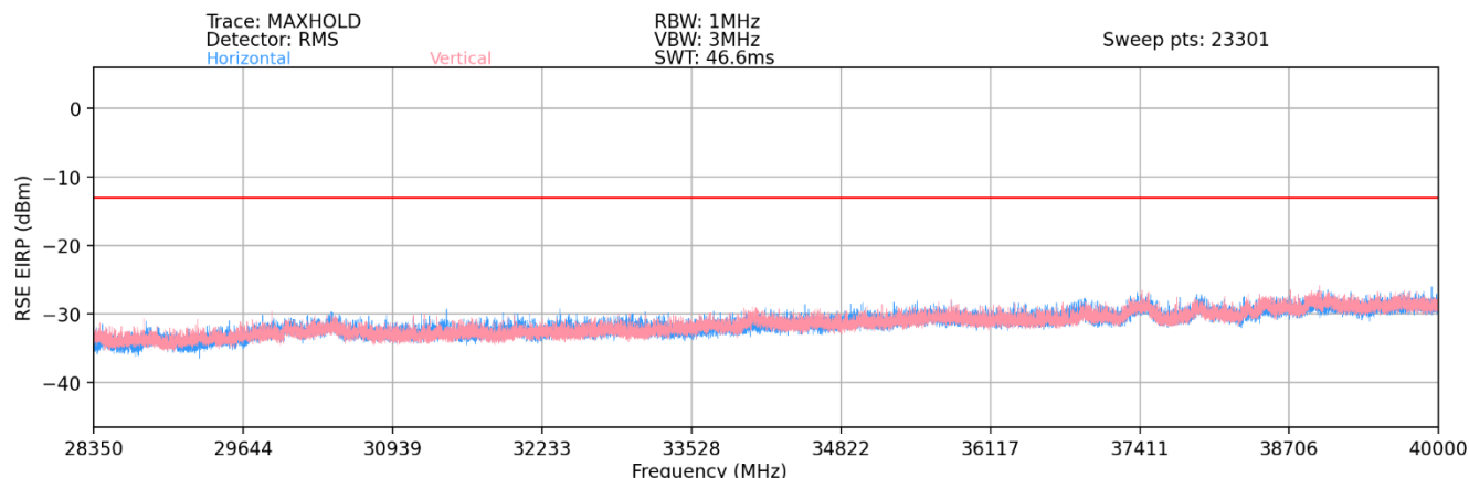
Plot 7-120. Ant 1 - n261 Radiated Spurious Plot (1CC QPSK Mid Channel 2Tx – EN-DC Anchor Band 2)
