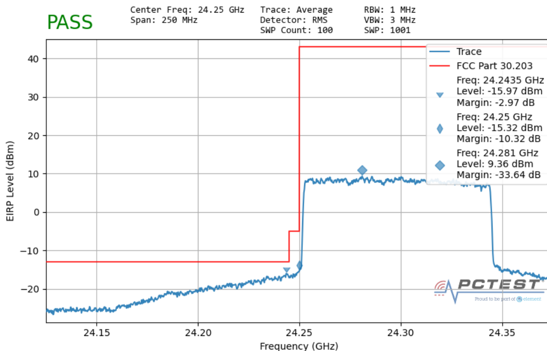
Plot 7-151. Ant 1 Lower Band Edge (100MHz-1CC – QPSK Full RB)
