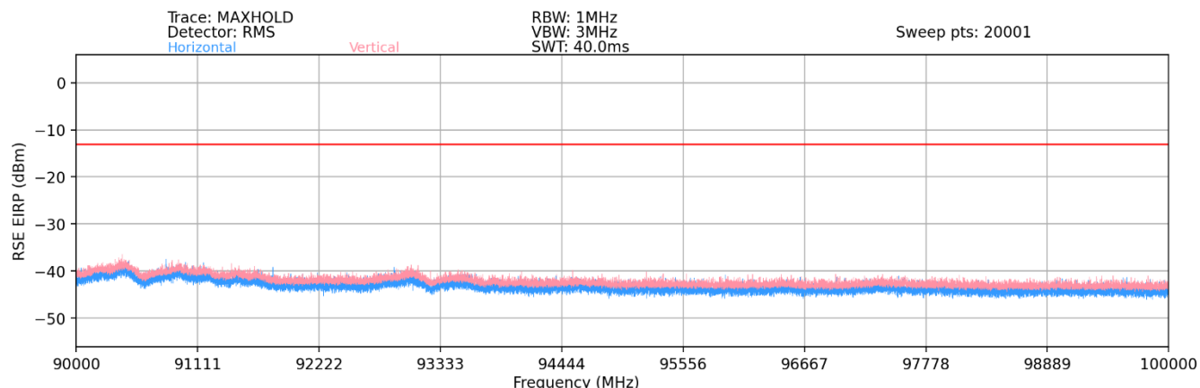
Plot 7-116. Ant 2 - n258-R2 Radiated Spurious Plot (1CC QPSK Mid Channel 2Tx – EN-DC Anchor Band 2)
