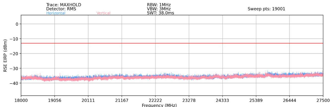
Plot 7-119. Ant 1 - n261 Radiated Spurious Plot (1CC QPSK Mid Channel 2Tx – EN-DC Anchor Band 2)
