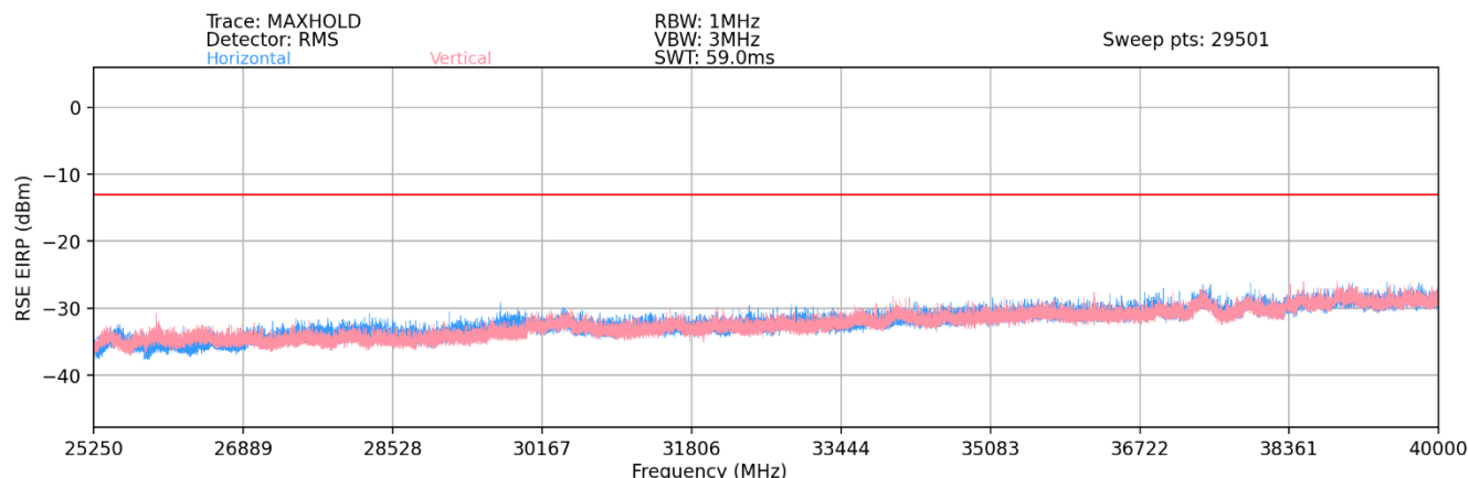
Plot 7-113. Ant 2 - n258-R2 Radiated Spurious Plot (1CC QPSK Mid Channel 2Tx – EN-DC Anchor Band 2)
