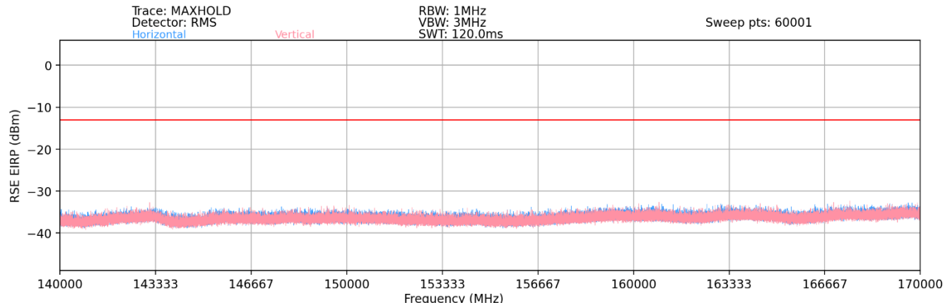
Plot 7-145. Ant 2 - n260 Radiated Spurious Plot (1CC QPSK Mid Channel 2Tx – EN-DC Anchor Band 2)
