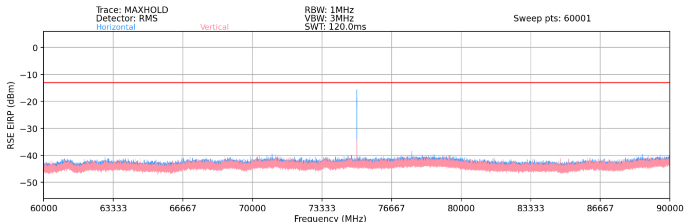
Plot 7-108. Ant 1 - n258-R2 Radiated Spurious Plot (1CC QPSK Mid Channel 2Tx – EN-DC Anchor Band 2)
