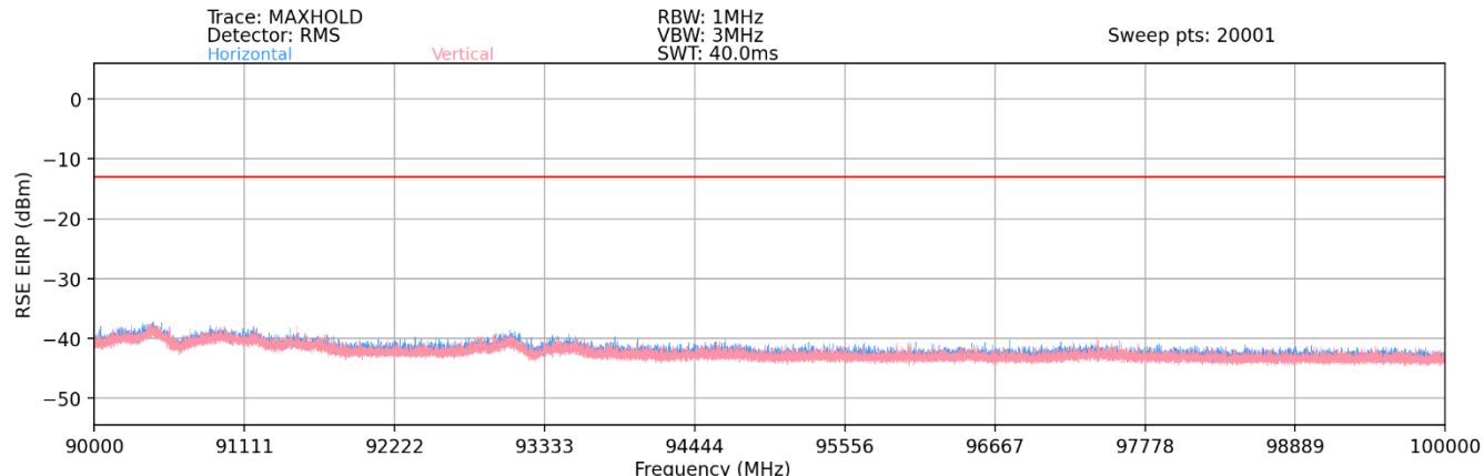
Plot 7-123. Ant 1 - n261 Radiated Spurious Plot (1CC QPSK Mid Channel 2Tx – EN-DC Anchor Band 2)
