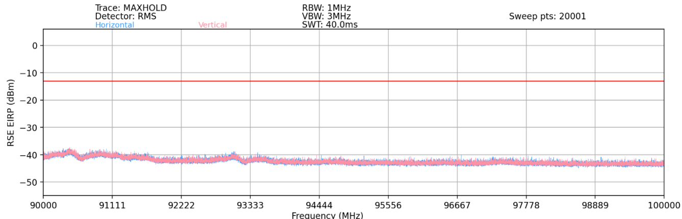
Plot 7-95. Ant 1 - n258-R1 Radiated Spurious Plot (1CC QPSK Mid Channel 2Tx – EN-DC Anchor Band 2)
