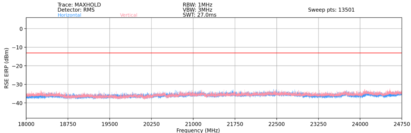
Plot 7-112. Ant 2 - n258-R2 Radiated Spurious Plot (1CC QPSK Mid Channel 2Tx – EN-DC Anchor Band 2)
