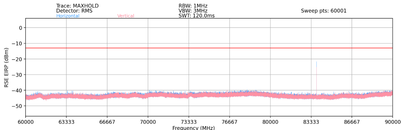
Plot 7-129. Ant 2 - n261 Radiated Spurious Plot (1CC QPSK Mid Channel 2Tx – EN-DC Anchor Band 2)
