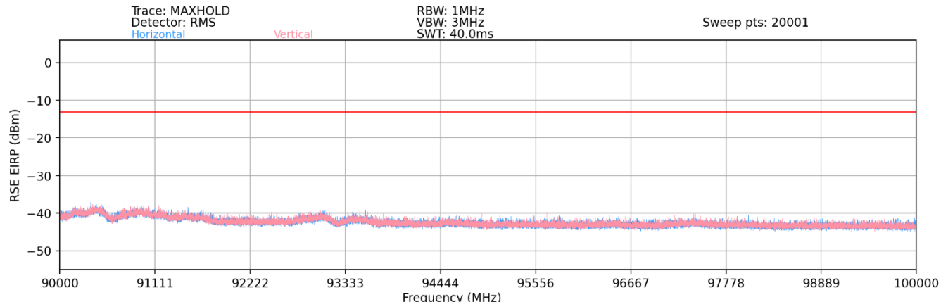
Plot 7-102. Ant 2 - n258-R1 Radiated Spurious Plot (1CC QPSK Mid Channel 2Tx – EN-DC Anchor Band 2)
