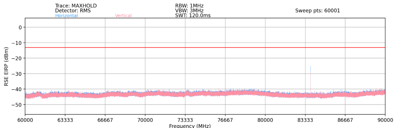
Plot 7-122. Ant 1 - n261 Radiated Spurious Plot (1CC QPSK Mid Channel 2Tx – EN-DC Anchor Band 2)
