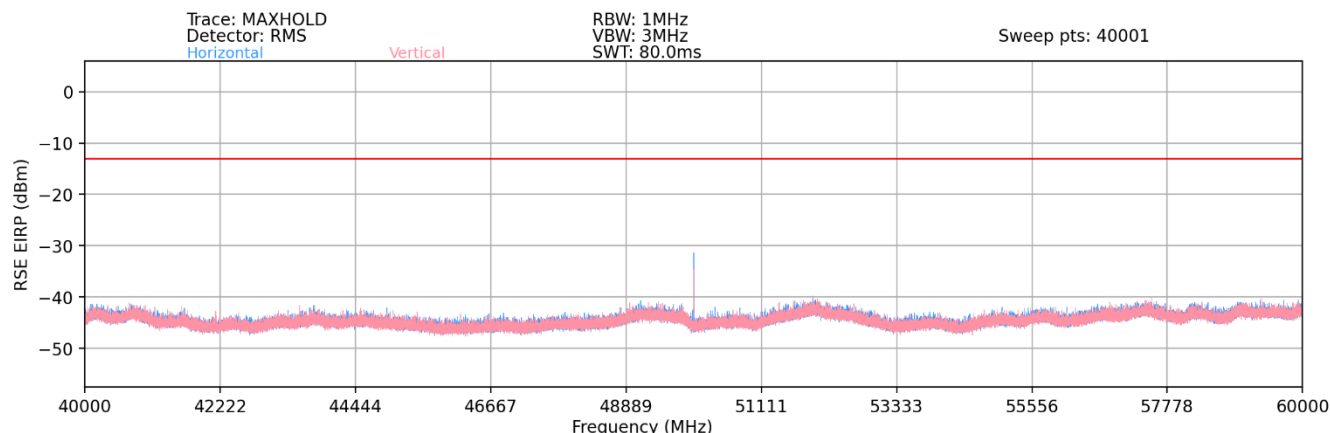
Plot 7-107. Ant 1 - n258-R2 Radiated Spurious Plot (1CC QPSK Mid Channel 2Tx – EN-DC Anchor Band 2)
