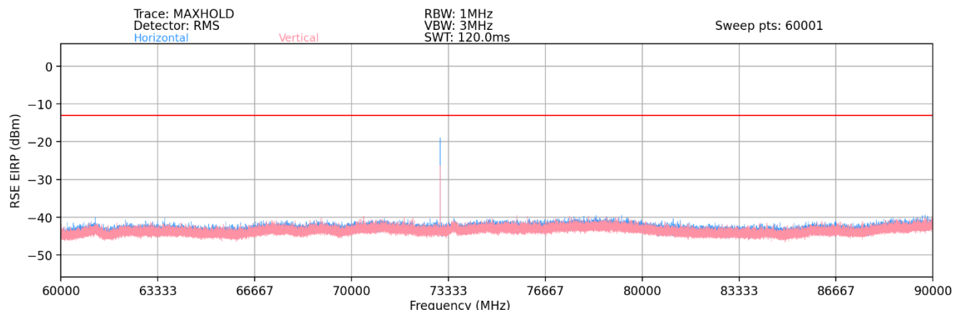
Plot 7-101. Ant 2 - n258-R1 Radiated Spurious Plot (1CC QPSK Mid Channel 2Tx – EN-DC Anchor Band 2)
