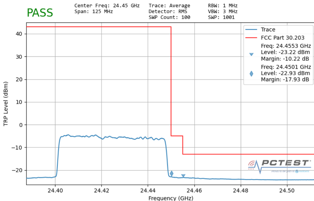
Plot 7-149. Ant 1 Upper Band Edge – TRP (50MHz-1CC – QPSK Full RB)
