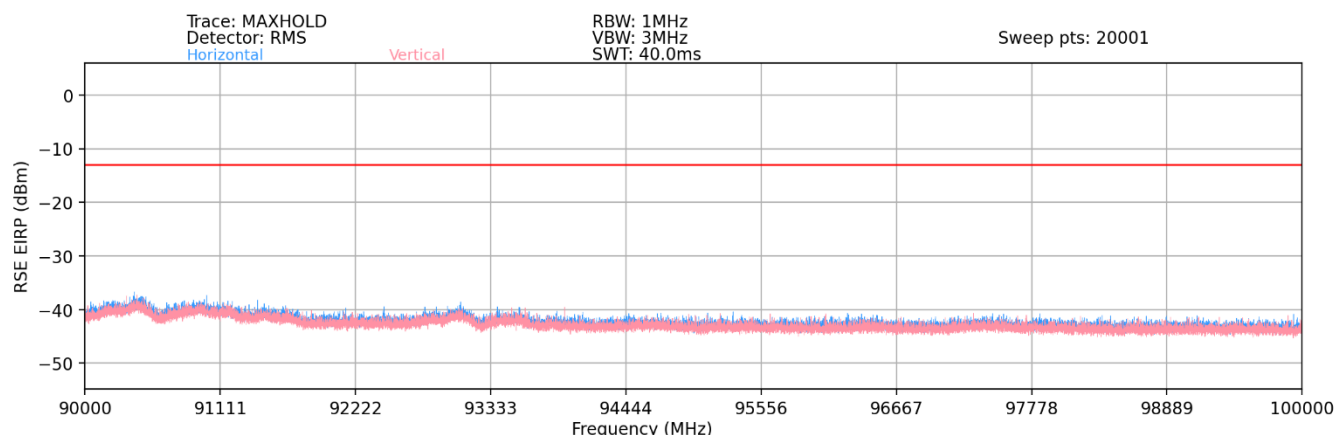
Plot 7-130. Ant 2 - n261 Radiated Spurious Plot (1CC QPSK Mid Channel 2Tx – EN-DC Anchor Band 2)
