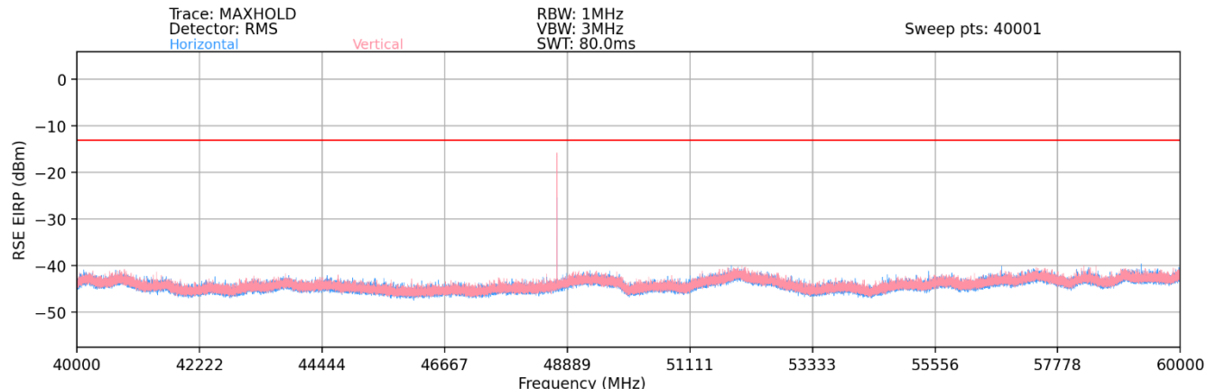
Plot 7-100. Ant 2 - n258-R1 Radiated Spurious Plot (1CC QPSK Mid Channel 2Tx – EN-DC Anchor Band 2)
