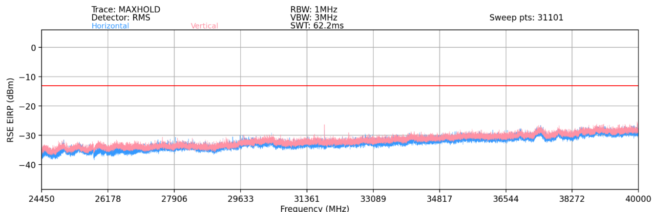
Plot 7-99. Ant 2 - n258-R1 Radiated Spurious Plot (1CC QPSK Mid Channel 2Tx – EN-DC Anchor Band 2)
