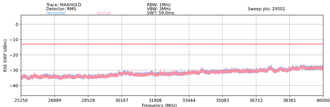
Plot 7-106. Ant 1 - n258-R2 Radiated Spurious Plot (1CC QPSK Mid Channel 2Tx – EN-DC Anchor Band 2)
