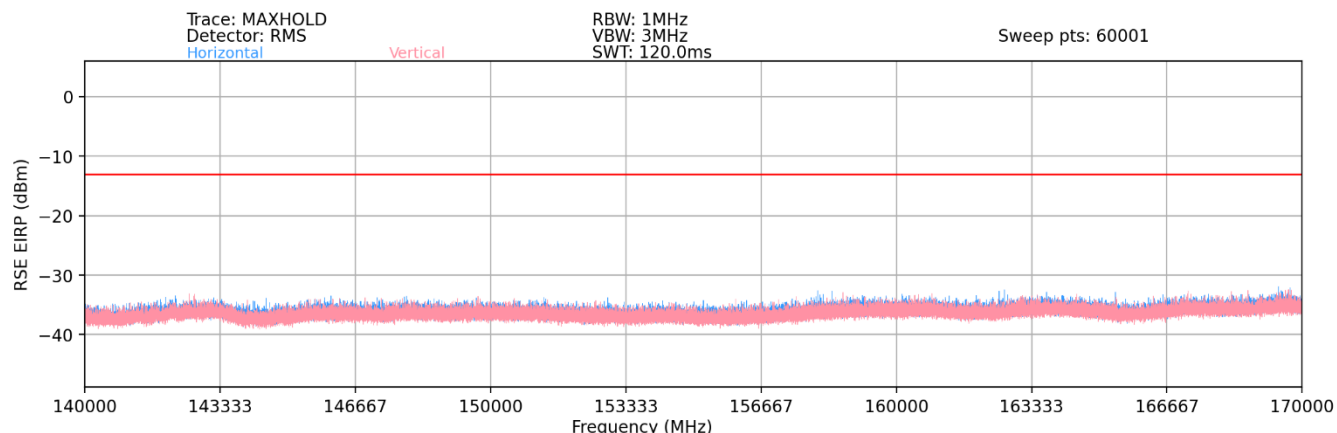
Plot 7-137. Ant 1 - n260 Radiated Spurious Plot (1CC QPSK Mid Channel 2Tx – EN-DC Anchor Band 2)
