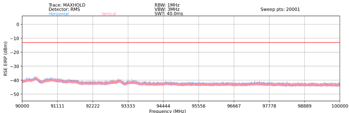
Plot 7-109. Ant 1 - n258-R2 Radiated Spurious Plot (1CC QPSK Mid Channel 2Tx – EN-DC Anchor Band 2)
