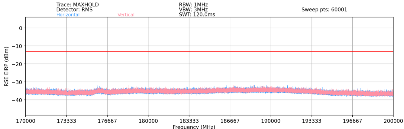
Plot 7-146. Ant 2 - n260 Radiated Spurious Plot (1CC QPSK Mid Channel 2Tx – EN-DC Anchor Band 2)
