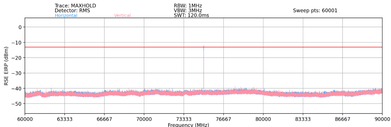
Plot 7-115. Ant 2 - n258-R2 Radiated Spurious Plot (1CC QPSK Mid Channel 2Tx – EN-DC Anchor Band 2)
