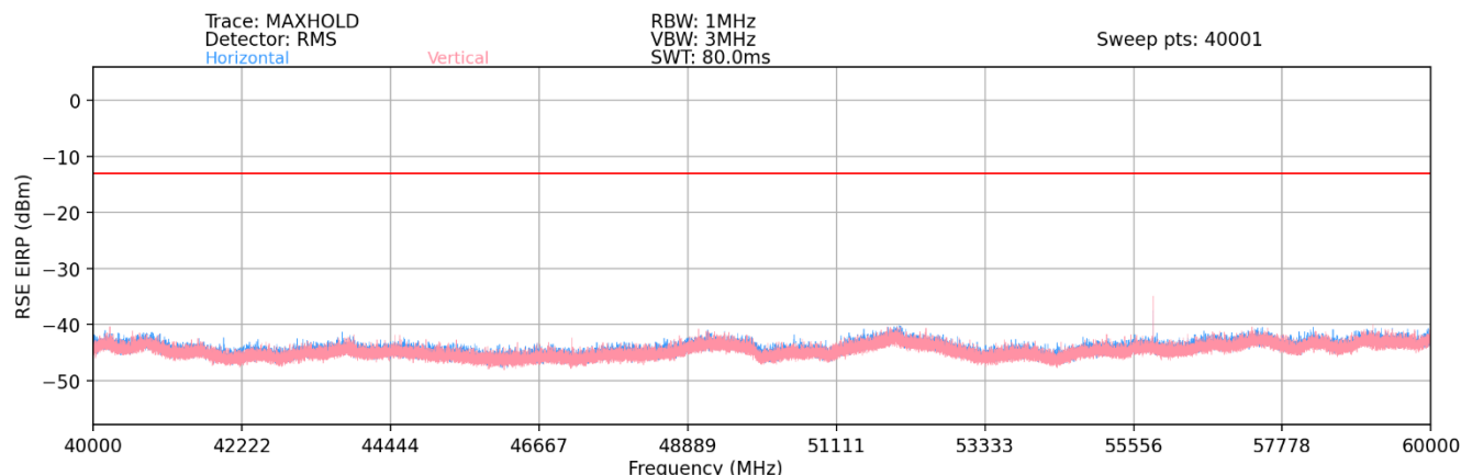
Plot 7-128. Ant 2 - n261 Radiated Spurious Plot (1CC QPSK Mid Channel 2Tx – EN-DC Anchor Band 2)
