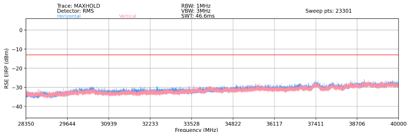
Plot 7-127. Ant 2 - n261 Radiated Spurious Plot (1CC QPSK Mid Channel 2Tx – EN-DC Anchor Band 2)
