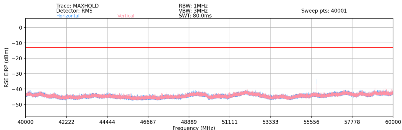
Plot 7-121. Ant 1 - n261 Radiated Spurious Plot (1CC QPSK Mid Channel 2Tx – EN-DC Anchor Band 2)
