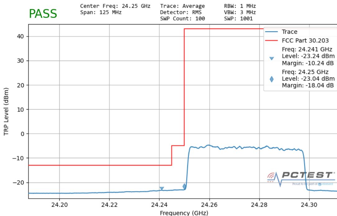
Plot 7-147. Ant 1 Lower Band Edge – TRP (50MHz-1CC – QPSK Full RB)
