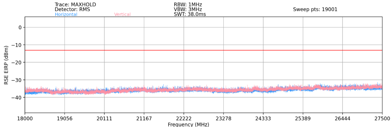
Plot 7-126. Ant 2 - n261 Radiated Spurious Plot (1CC QPSK Mid Channel 2Tx – EN-DC Anchor Band 2)
