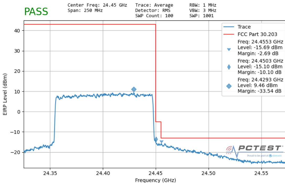
Plot 7-153. Ant 1 Upper Band Edge (100MHz-1CC – QPSK Full RB)
