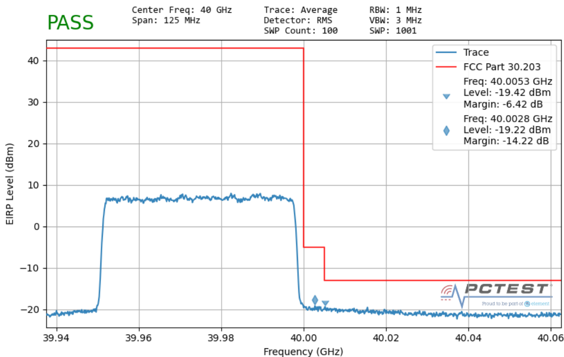
Plot 7-181. Ant 2 Upper Band Edge (50MHz-1CC – QPSK Full RB)
