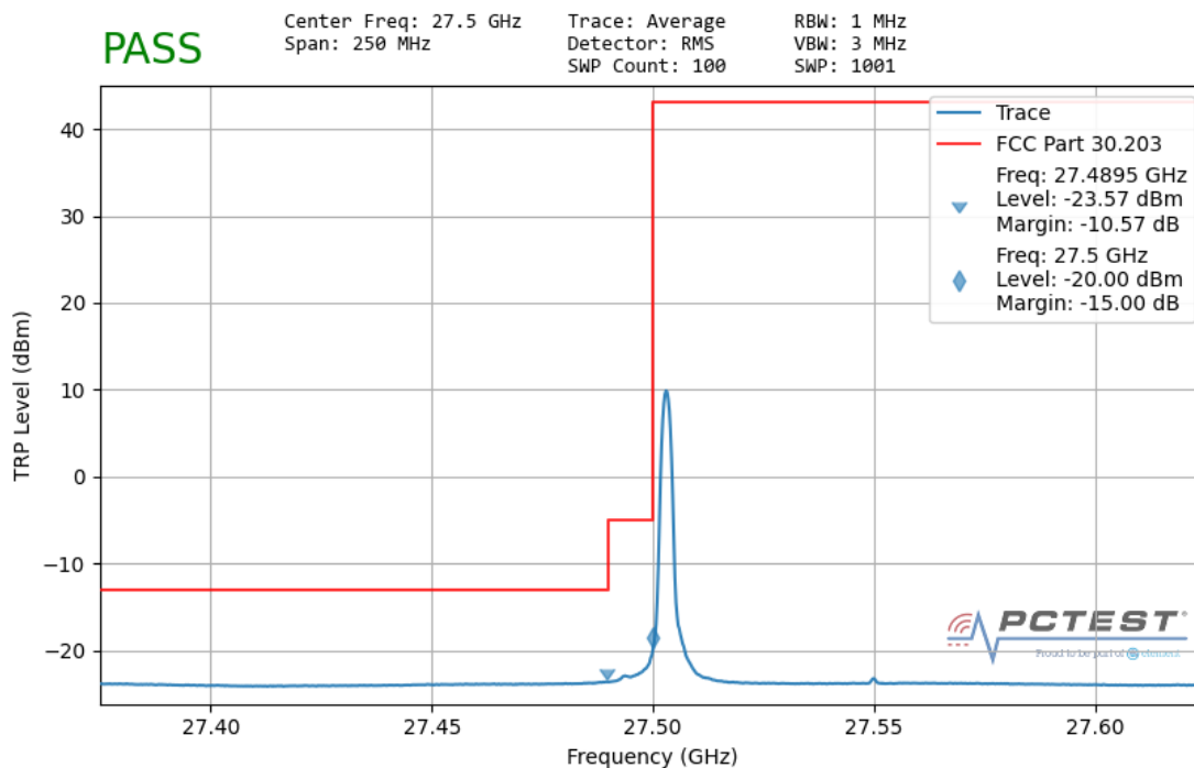
Plot 7-159. Ant 1 Lower Band Edge – TRP (100MHz-1CC – QPSK 1 RB)
