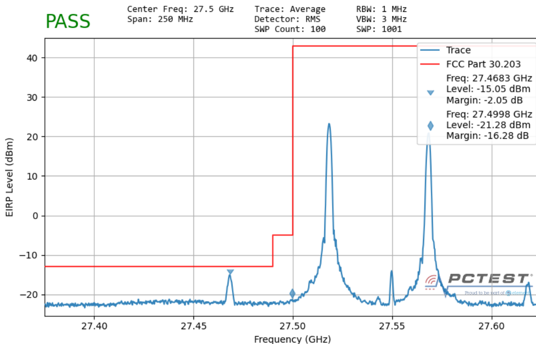
Plot 7-156. Ant 1 Lower Band Edge (50MHz-2CC – QPSK 1 RB)
