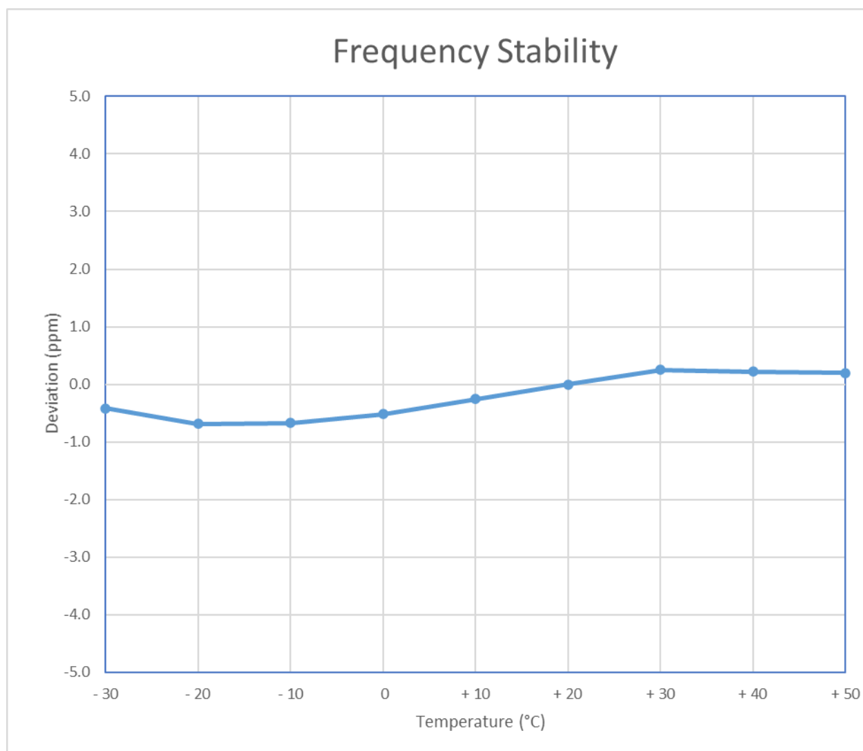
Figure 7-3. Frequency Stability Graph (n261)
