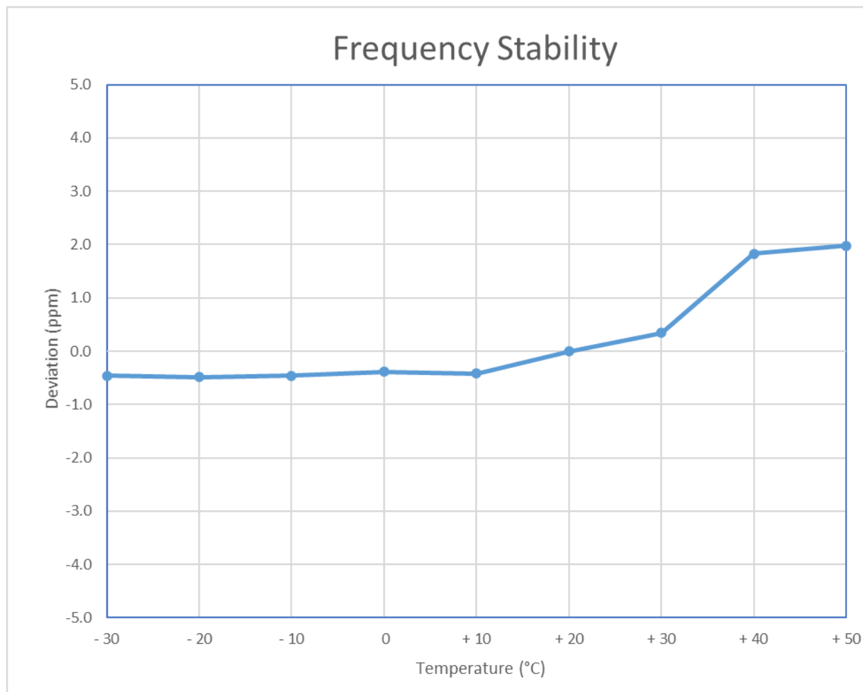
Figure 7-4. Frequency Stability Graph (n260)
