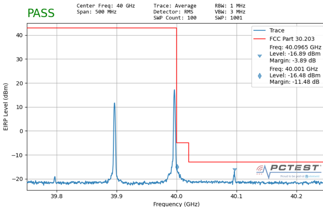
Plot 7-178. Ant 1 Upper Band Edge (100MHz-2CC – QPSK 1 RB)
