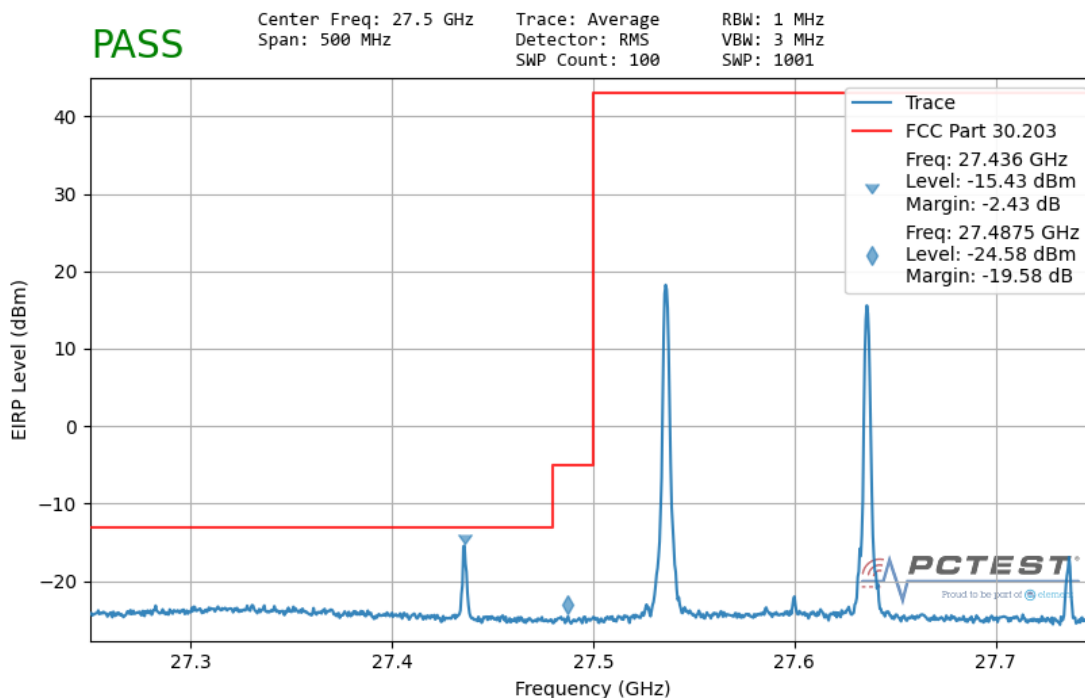
Plot 7-168. Ant 2 Lower Band Edge (100MHz-2CC – QPSK 1 RB)
