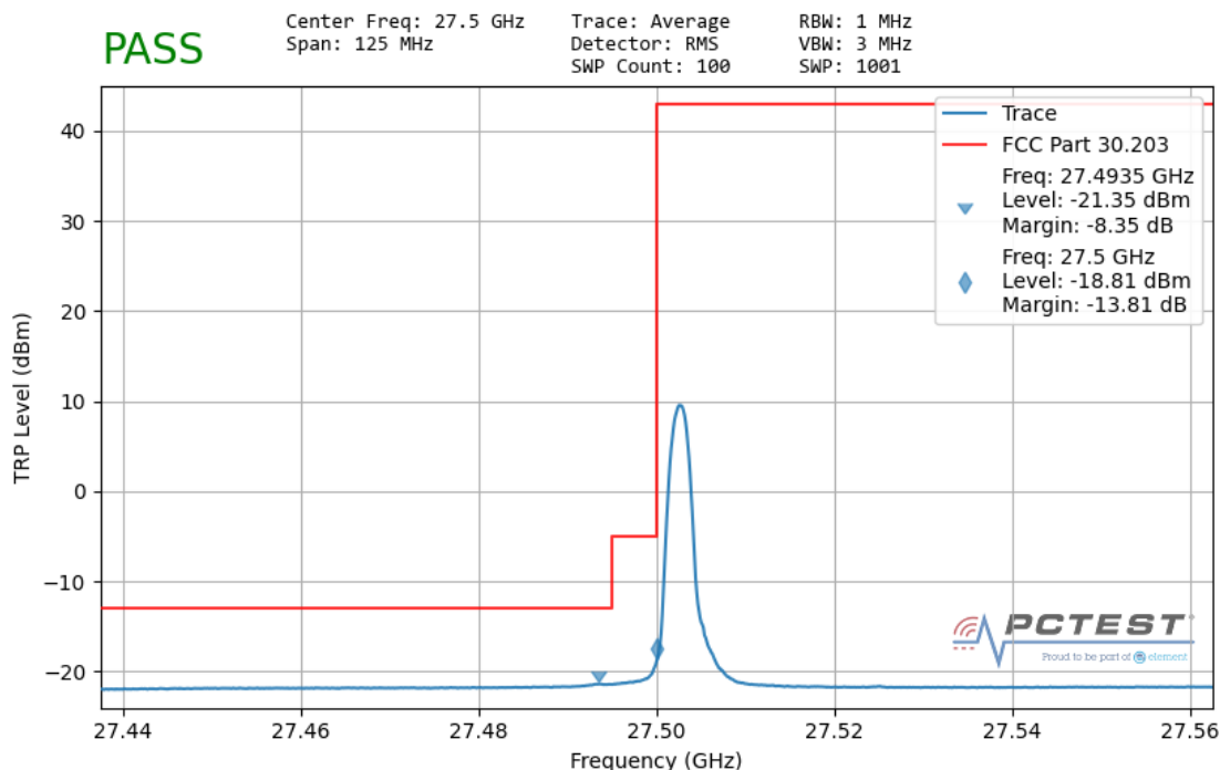
Plot 7-155. Ant 1 Lower Band Edge – TRP (50MHz-1CC – QPSK 1 RB)
