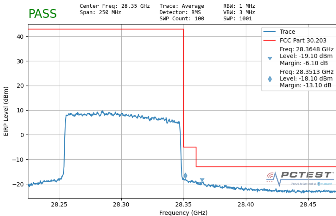
Plot 7-169. Ant 2 Upper Band Edge (100MHz-1CC – QPSK Full RB)
