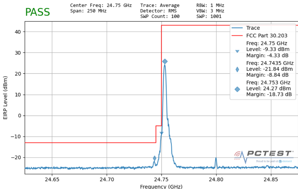
Plot 7-151. Ant 2 Lower Band Edge (100MHz-1CC – QPSK 1 RB)
