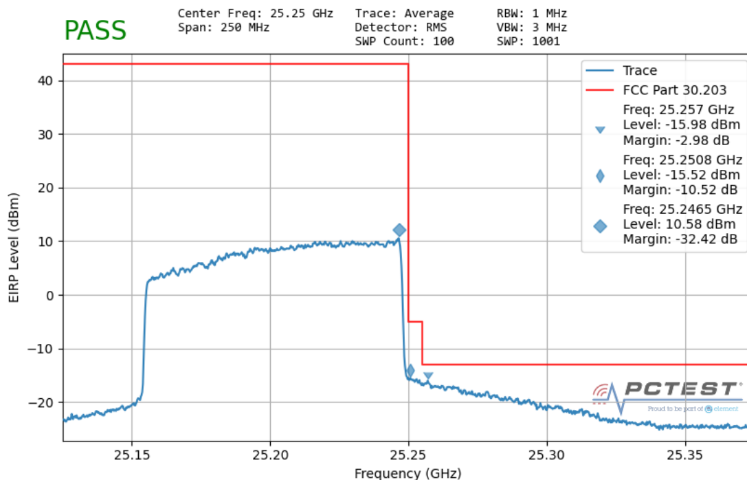
Plot 7-153. Ant 2 Upper Band Edge (100MHz-1CC – QPSK Full RB)
