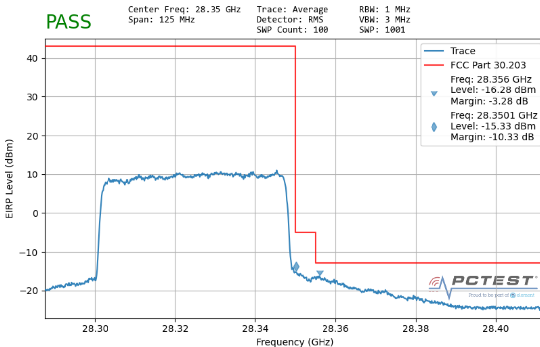
Plot 7-165. Ant 2 Upper Band Edge (50MHz-1CC – QPSK Full RB)
