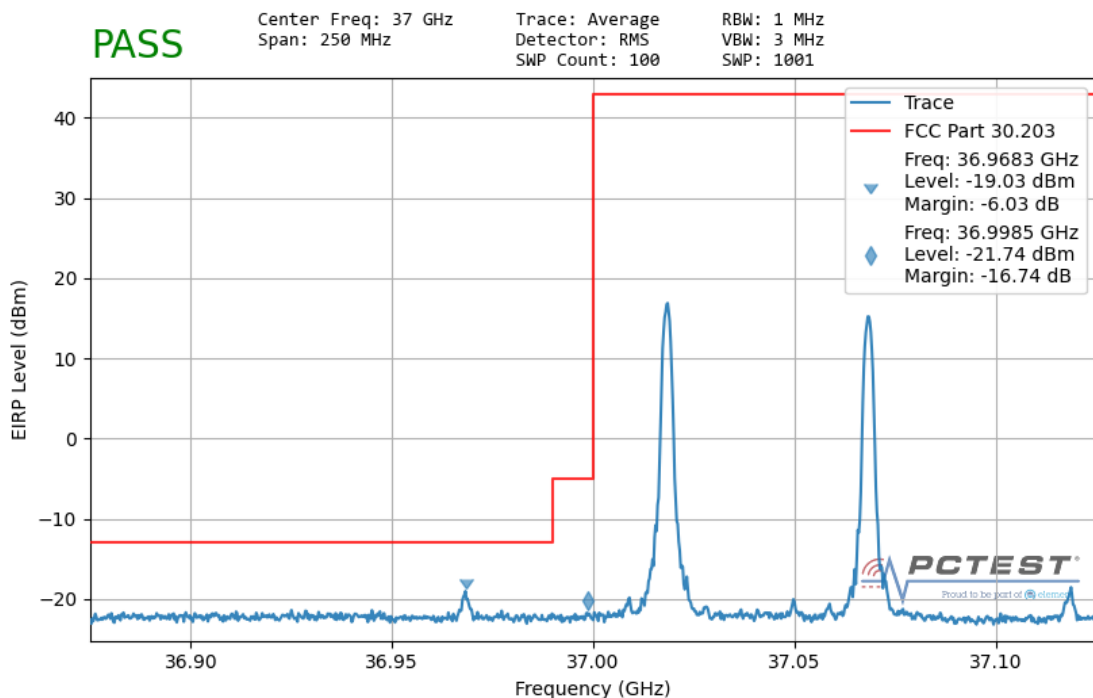
Plot 7-180. Ant 2 Lower Band Edge (50MHz-2CC – QPSK 1 RB)
