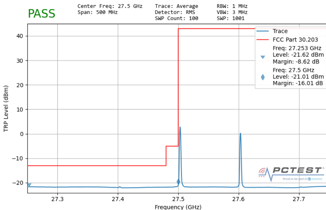
Plot 7-160. Ant 1 Lower Band Edge – TRP (100MHz-2CC – QPSK 1 RB)
