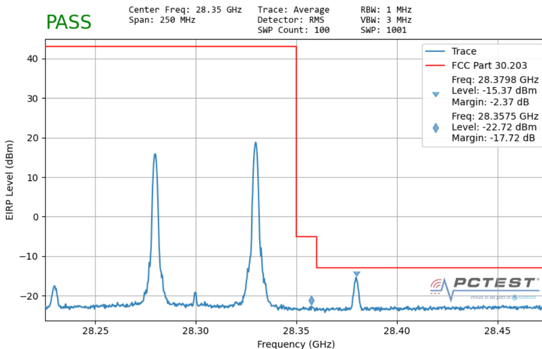
Plot 7-166. Ant 2 Upper Band Edge (50MHz-2CC – QPSK 1 RB)
