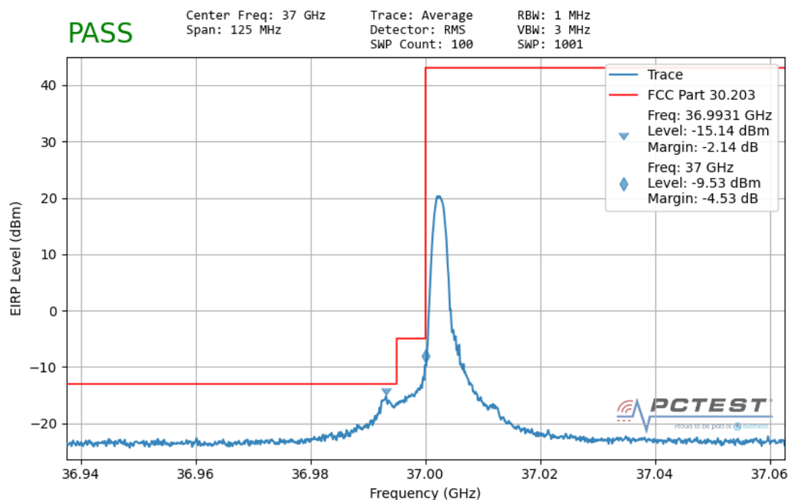
Plot 7-171. Ant 1 Lower Band Edge (50MHz-1CC QPSK 1 RB)
