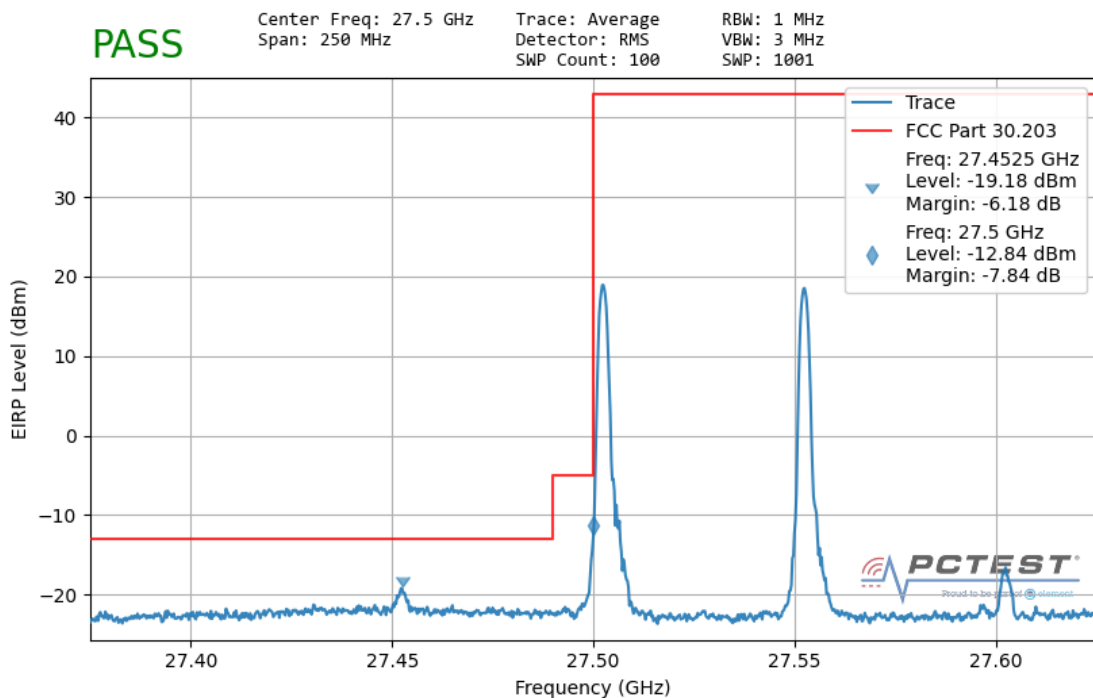
Plot 7-164. Ant 2 Lower Band Edge (50MHz-2CC – QPSK 1 RB)
