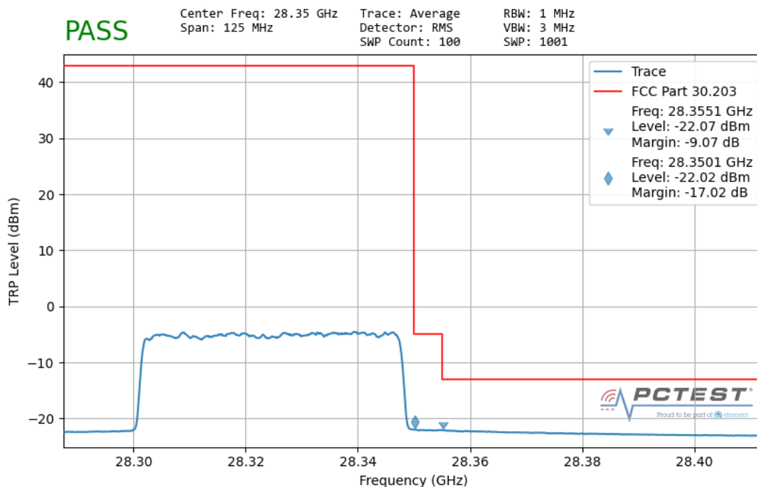
Plot 7-157. Ant 1 Upper Band Edge – TRP (50MHz-1CC – QPSK Full RB)
