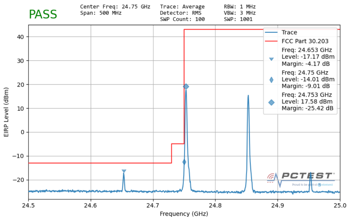
Plot 7-152. Ant 2 Lower Band Edge (100MHz-2CC – QPSK 1 RB)
