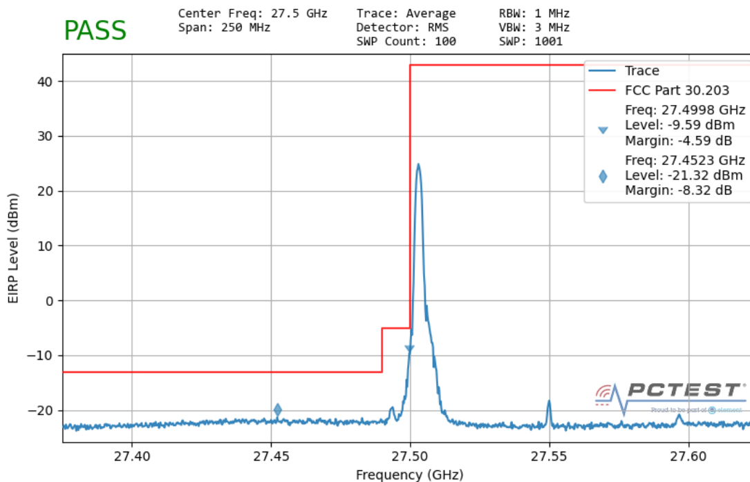
Plot 7-167. Ant 2 Lower Band Edge (100MHz-1CC – QPSK 1 RB)
