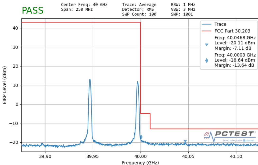
Plot 7-174. Ant 1 Upper Band Edge (50MHz-2CC – QPSK 1 RB)
