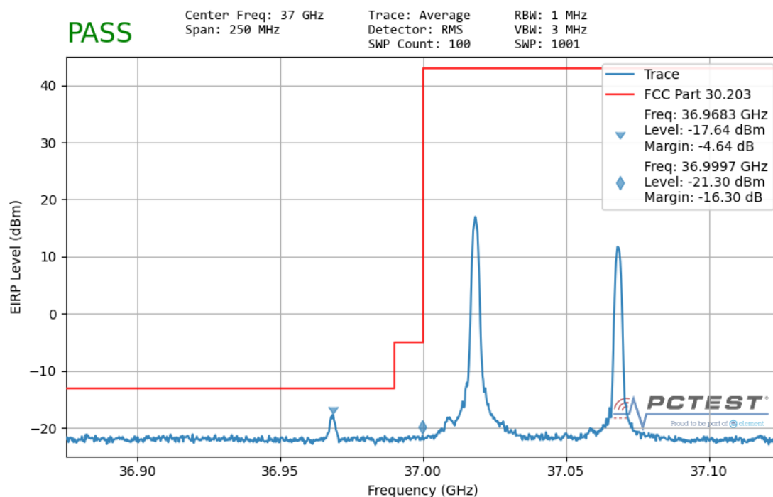
Plot 7-172. Ant 1 Lower Band Edge (50MHz-2CC – QPSK 1 RB)
