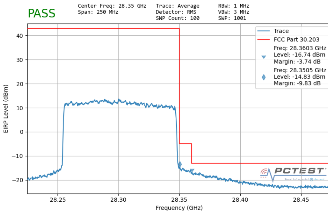
Plot 7-161. Ant 1 Upper Band Edge (100MHz-1CC – QPSK Full RB)
