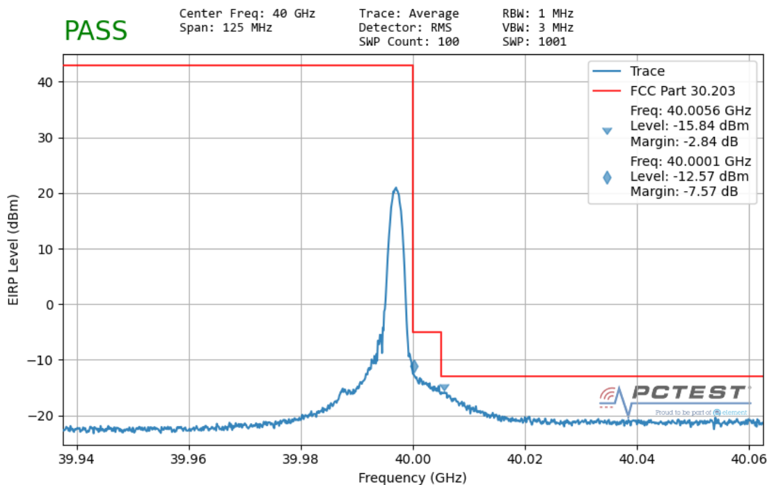
Plot 7-173. Ant 1 Upper Band Edge (50MHz-1CC – QPSK 1 RB)
