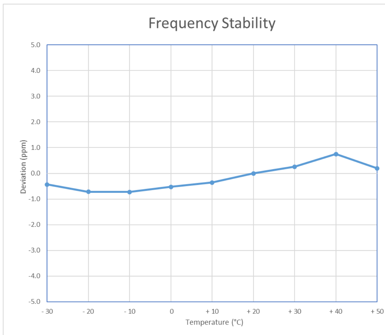
Figure 7-2. Frequency Stability Graph (n258-R2)
