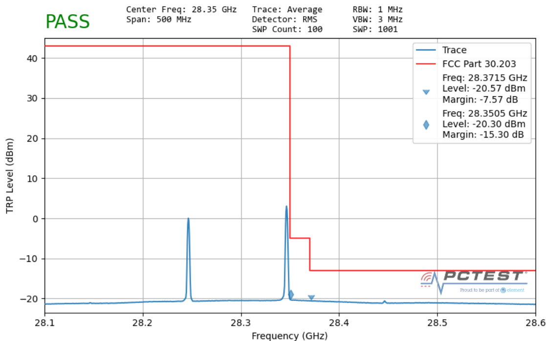
Plot 7-162. Ant 1 Upper Band Edge – TRP (100MHz-2CC – QPSK 1 RB)
