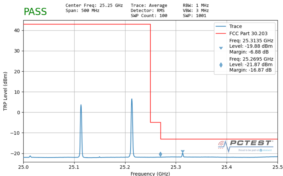
Plot 7-154. Ant 2 Upper Band Edge – TRP (100MHz-2CC – QPSK 1 RB)
