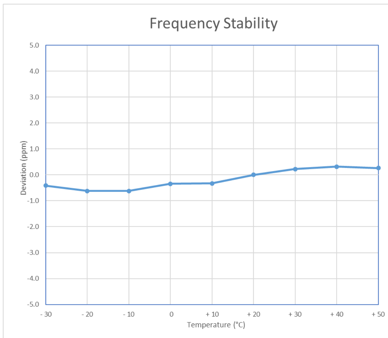
Figure 7-1. Frequency Stability Graph (n258-R1)
