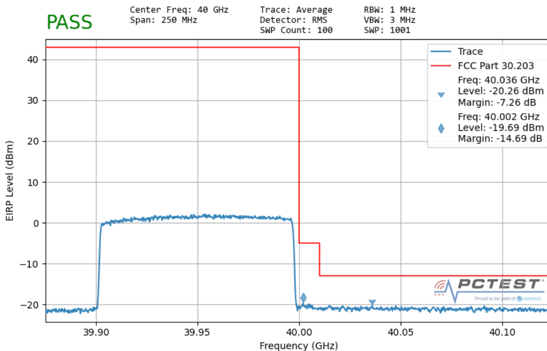
Plot 7-185. Ant 2 Upper Band Edge (100MHz-1CC – QPSK Full RB)
