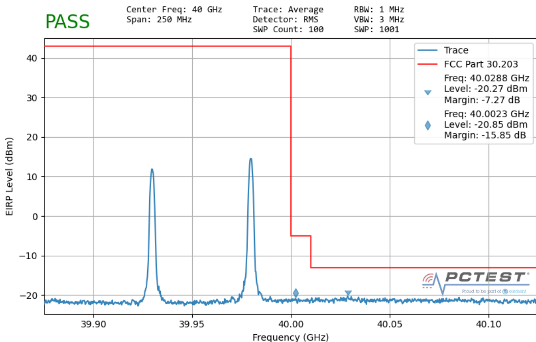
Plot 7-182. Ant 2 Upper Band Edge (50MHz-2CC – QPSK 1 RB)
