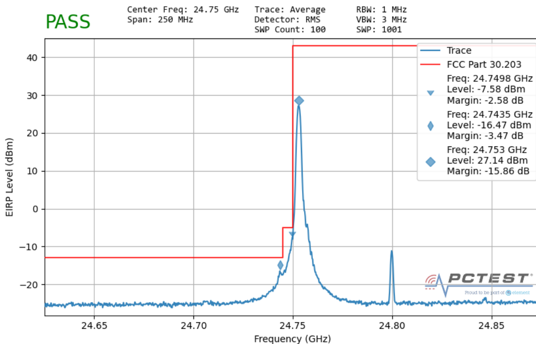
Plot 7-167. Ant 1 Lower Band Edge (100MHz-1CC – QPSK 1 RB)
