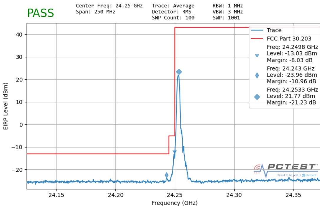
Plot 7-159. Ant 2 Lower Band Edge (100MHz-1CC – QPSK 1 RB)
