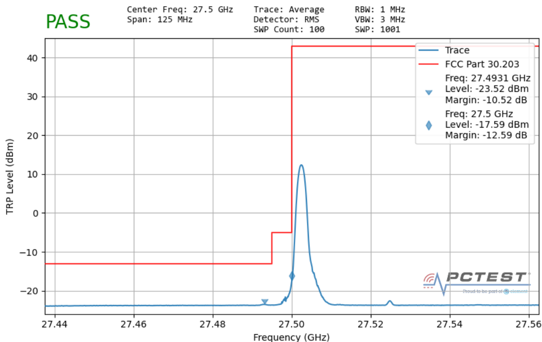
Plot 7-187. Ant 2 Lower Band Edge – TRP (50MHz-1CC – QPSK 1 RB)
