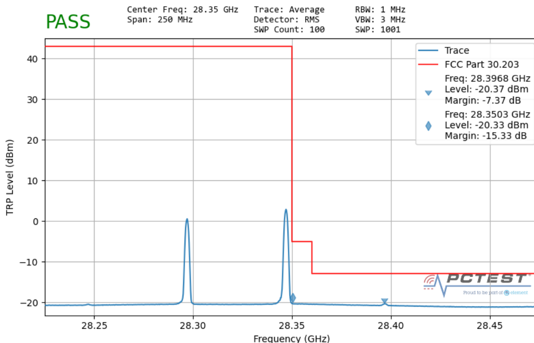
Plot 7-182. Ant 1 Upper Band Edge – TRP (50MHz-2CC – QPSK 1 RB)
