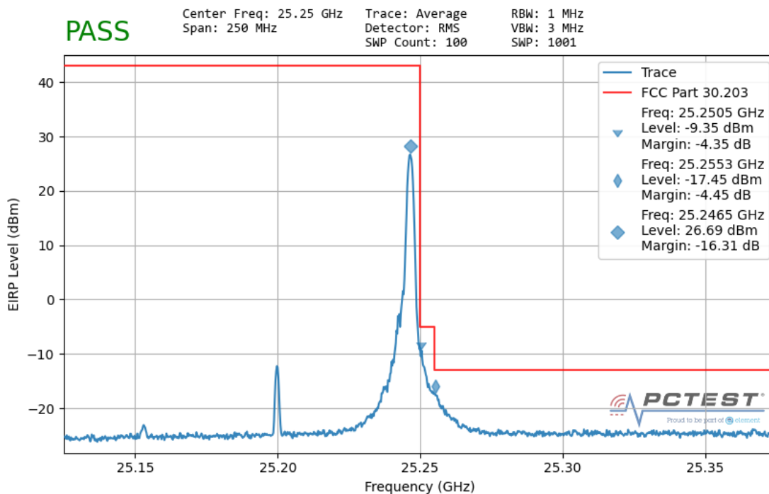
Plot 7-169. Ant 1 Upper Band Edge (100MHz-1CC – QPSK 1 RB)
