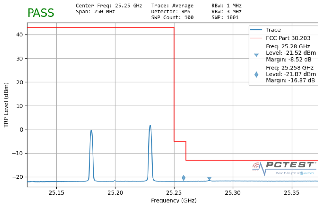
Plot 7-166. Ant 1 Upper Band Edge – TRP (50MHz-2CC – QPSK 1 RB)
