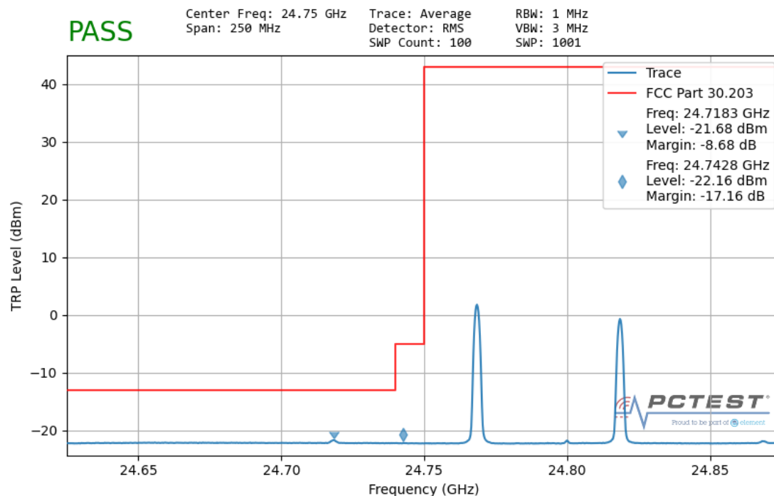
Plot 7-164. Ant 1 Lower Band Edge – TRP (50MHz-2CC – QPSK 1 RB)
