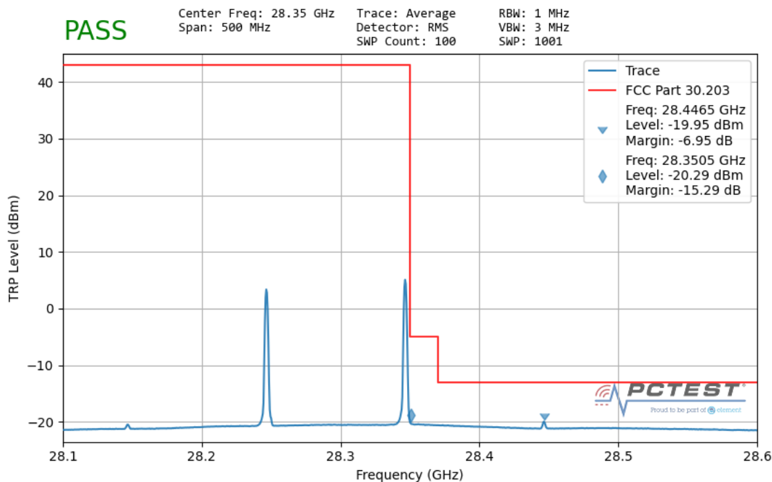
Plot 7-194. Ant 2 Upper Band Edge – TRP (100MHz-2CC – QPSK 1 RB)
