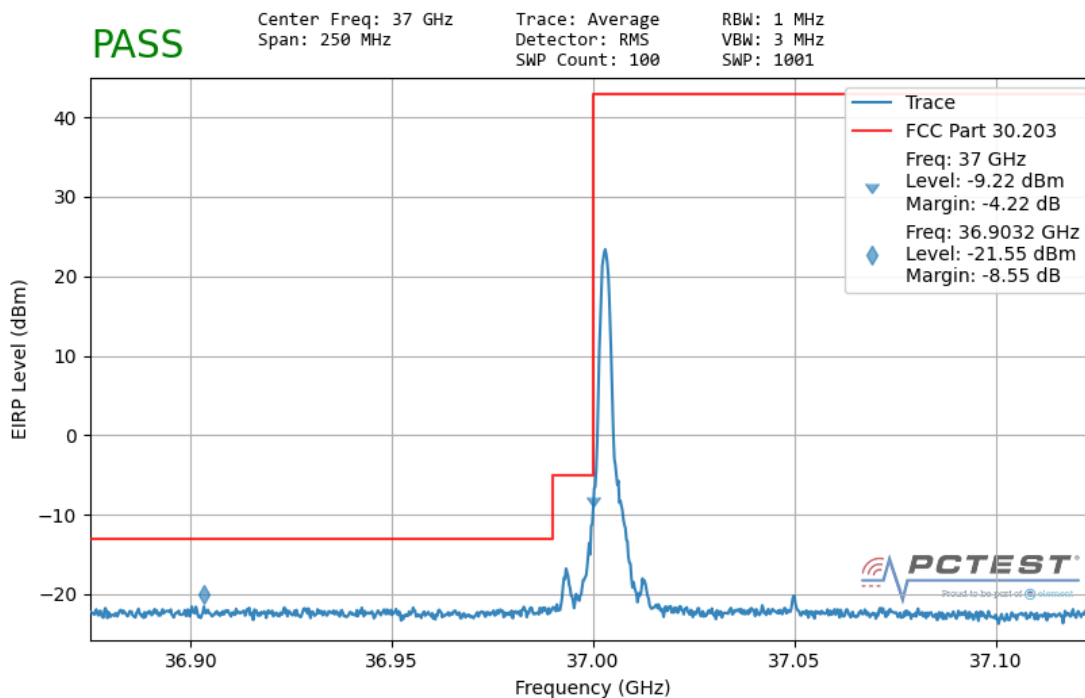
Plot 7-207. Ant 2 Lower Band Edge (100MHz-1CC – QPSK 1 RB)
