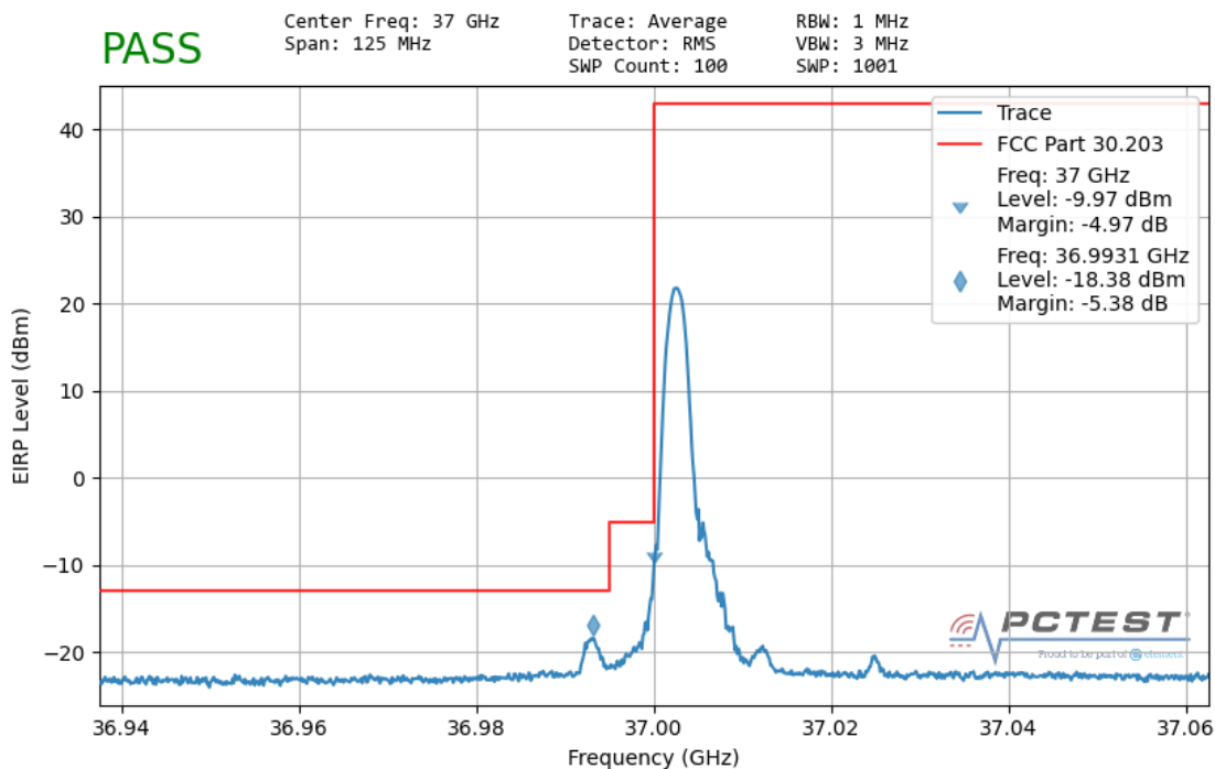
Plot 7-203. Ant 2 Lower Band Edge (50MHz-1CC – QPSK 1 RB)
