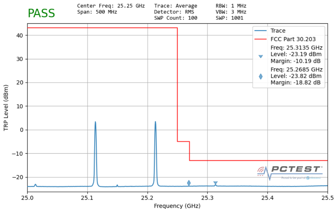
Plot 7-170. Ant 1 Upper Band Edge – TRP (100MHz-2CC – QPSK 1 RB)
