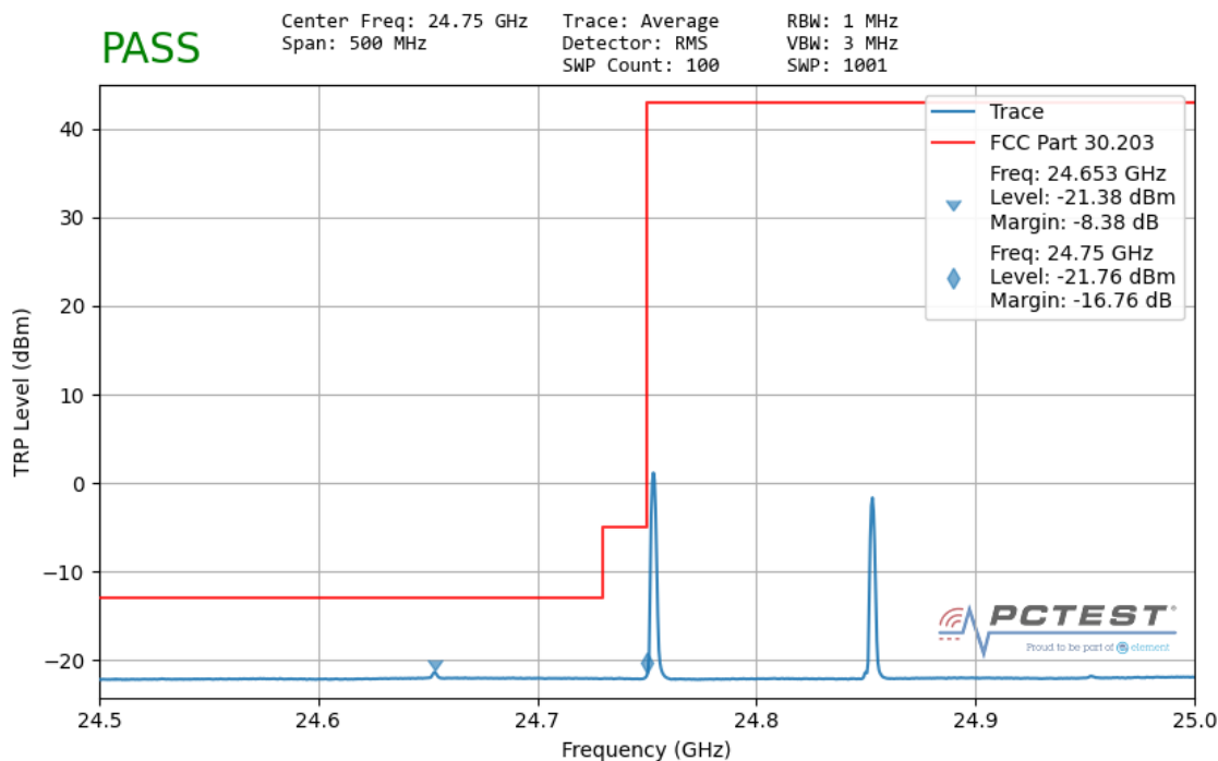
Plot 7-168. Ant 1 Lower Band Edge – TRP (100MHz-2CC – QPSK 1 RB)
