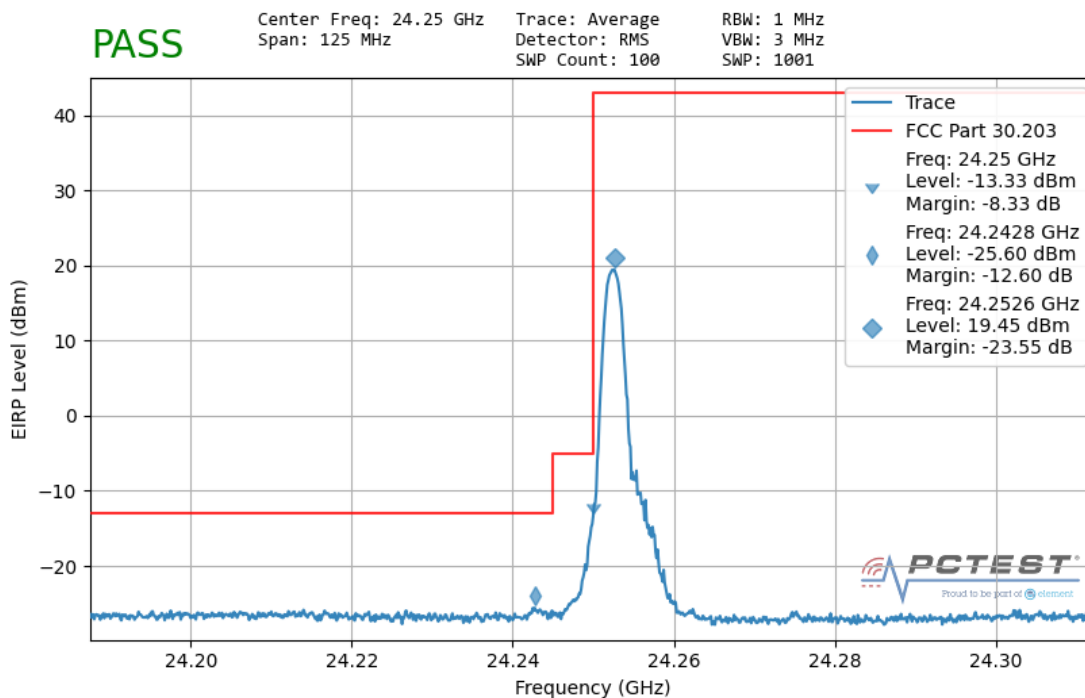
Plot 7-155. Ant 2 Lower Band Edge (50MHz-1CC – QPSK 1 RB)
