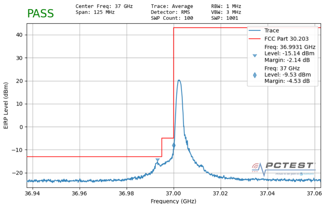
Plot 7-195. Ant 1 Lower Band Edge (50MHz-1CC QPSK 1 RB)
