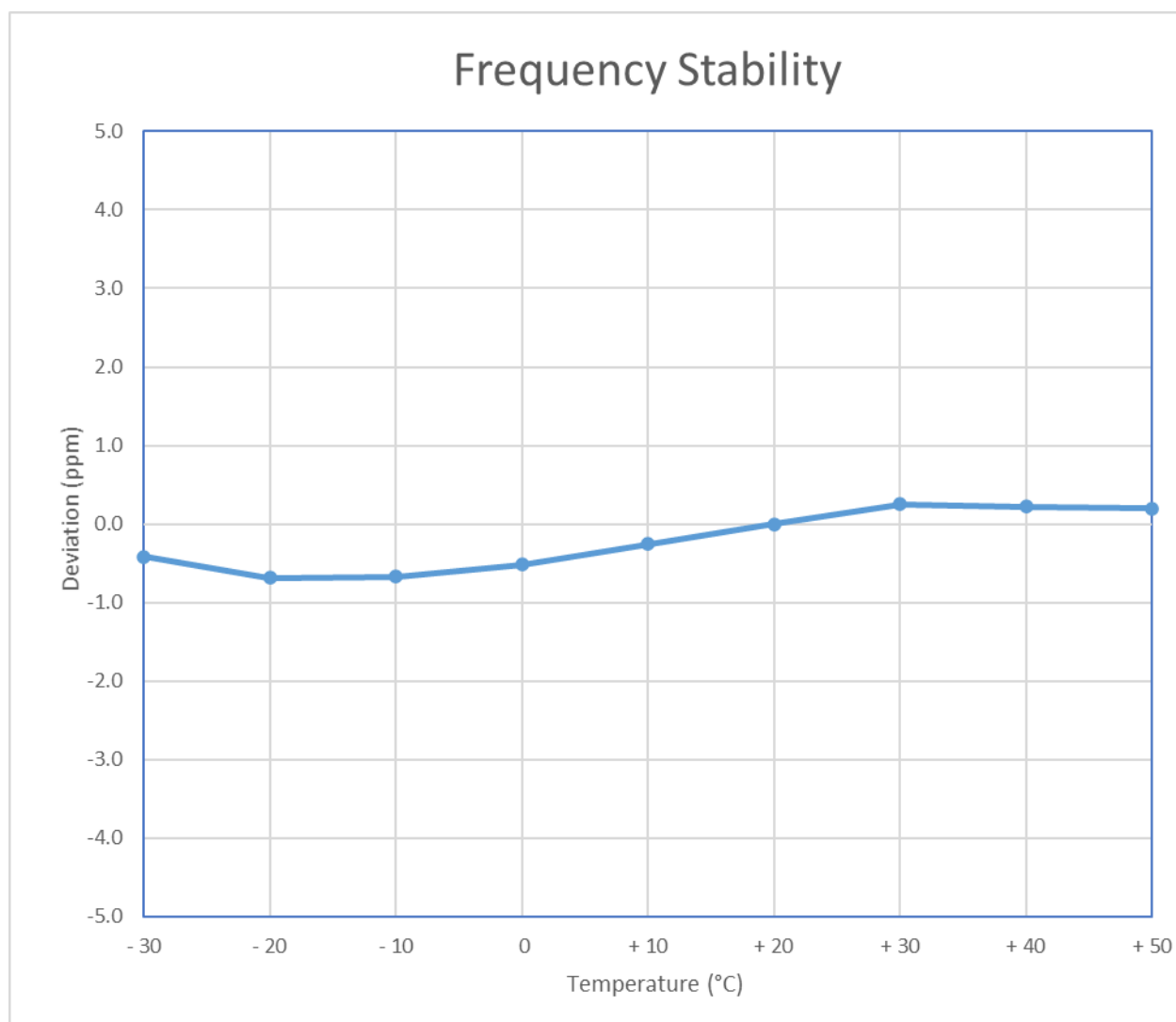
Figure 7-3. Frequency Stability Graph (n261)
