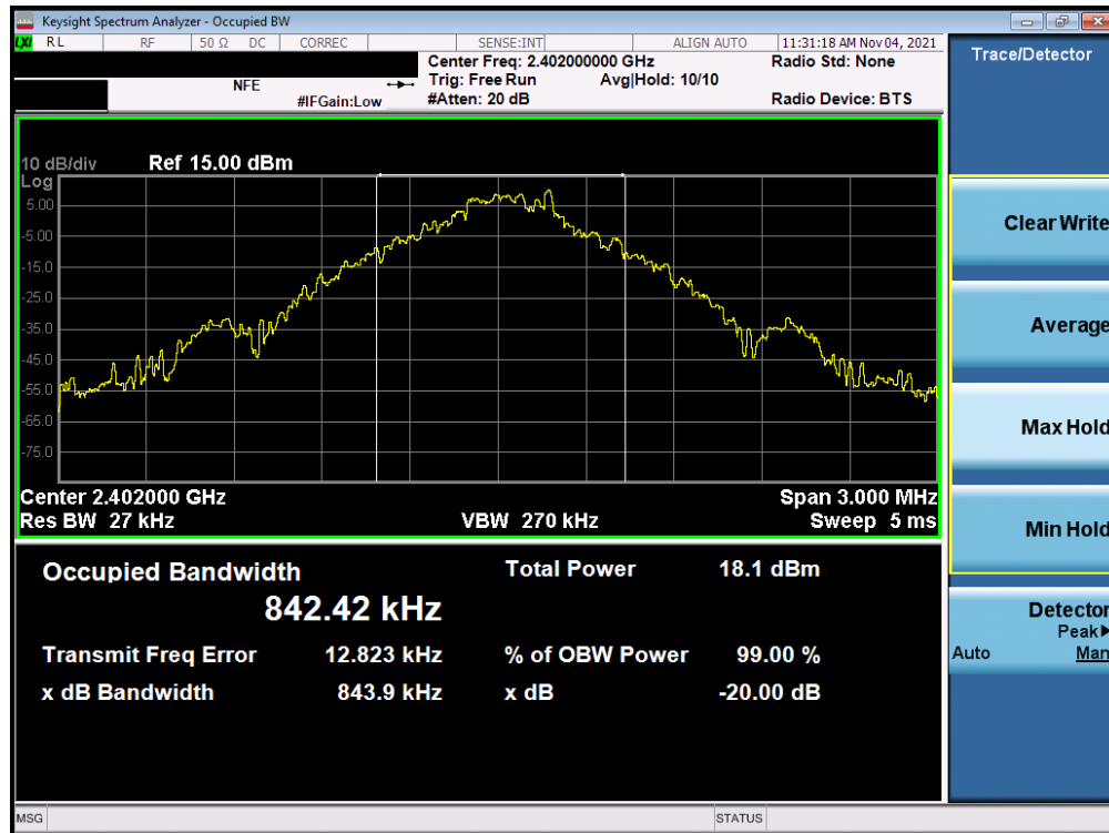
Plot 7-1. 20dB Bandwidth Plot (Bluetooth, 1Mbps – Ch. 0) Antenna 1
