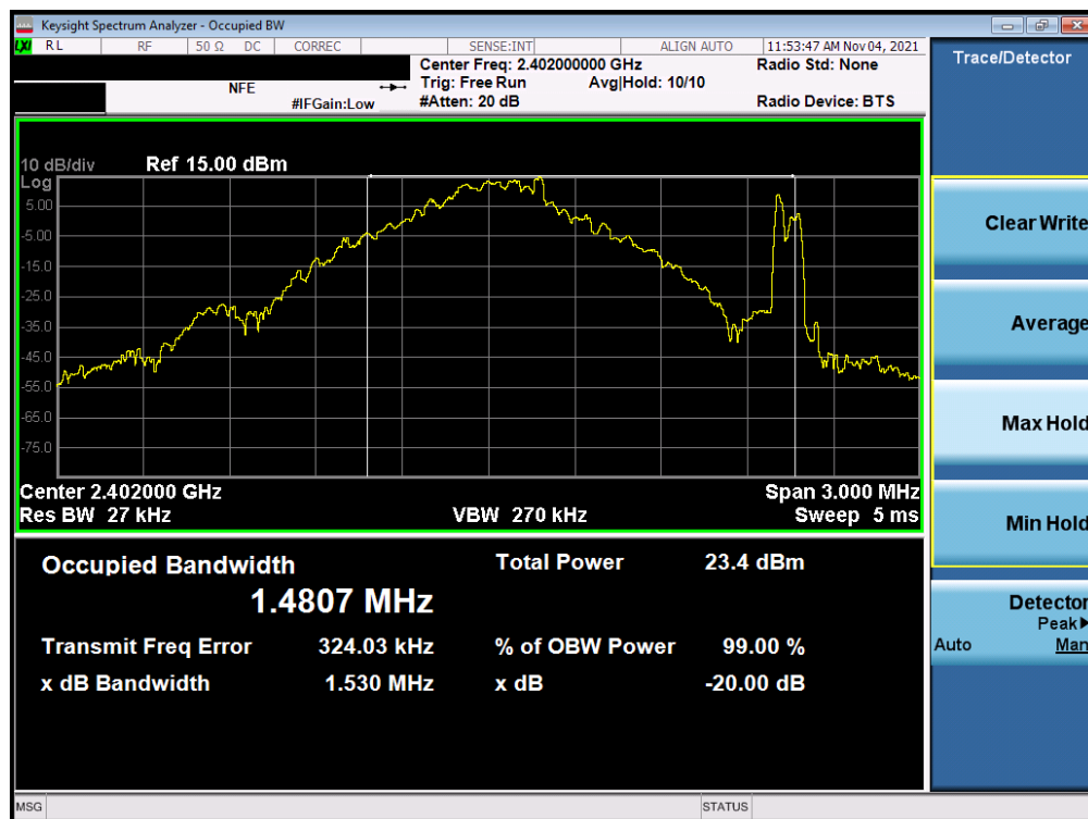
Plot 7-10. 20dB Bandwidth Plot (Bluetooth, 1Mbps – Ch. 0) Antenna 2
