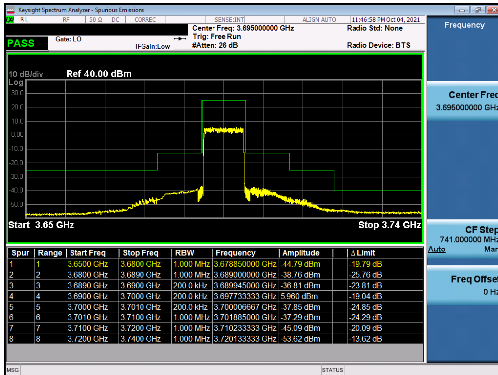
Plot 7-46. Channel Edge Plot (LTE Band 48 - 10MHz QPSK - High Channel)
