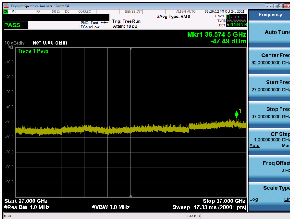
Plot 7-40. Conducted Spurious Plot (ULCA LB48 - 20+20MHz QPSK - High Channel)
