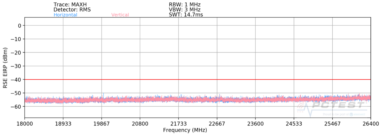
Plot 7-71. Radiated Spurious Plot (LTE Band 48)
