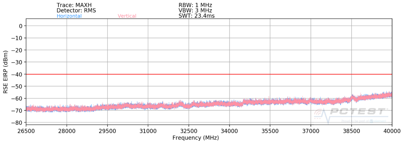
Plot 7-72. Radiated Spurious Plot (LTE Band 48)
