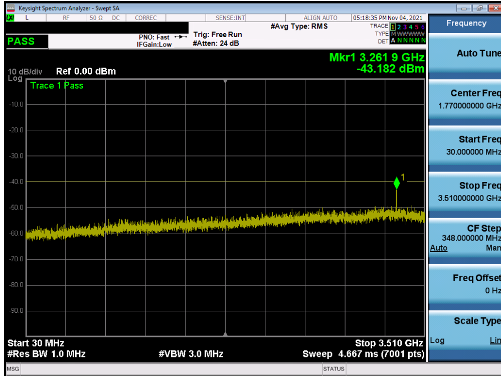
Plot 7-52. Conducted Spurious Plot (ULCA LB48 - 20+20MHz QPSK - Low Channel)
