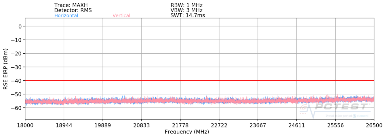
Plot 7-76. Radiated Spurious Plot (ULCA LB48)
