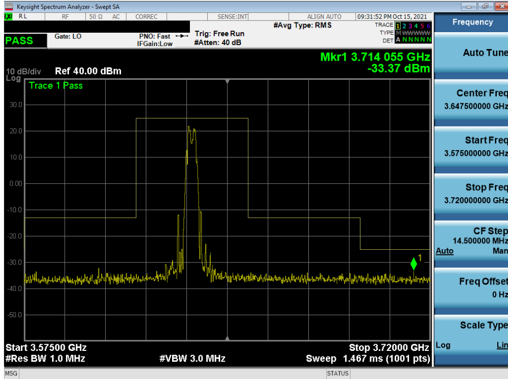
Plot 7-58. Conducted Spurious Plot (ULCA LB48 - 20+20MHz QPSK - Mid Channel)
