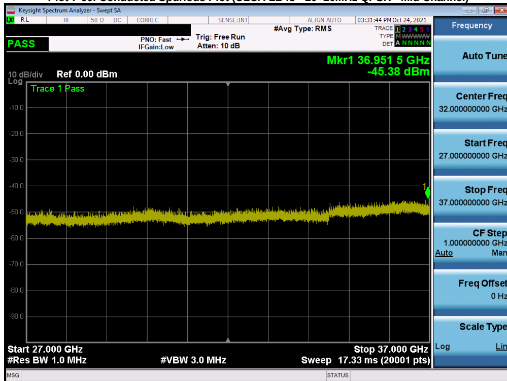
Plot 7-61. Conducted Spurious Plot (ULCA LB48 - 20+20MHz QPSK - Mid Channel)
