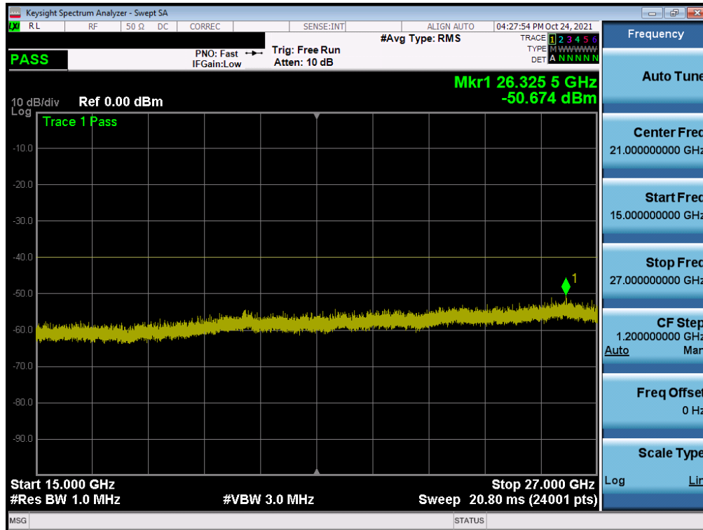
Plot 7-39. Conducted Spurious Plot (ULCA LB48 - 20+20MHz QPSK - High Channel)
