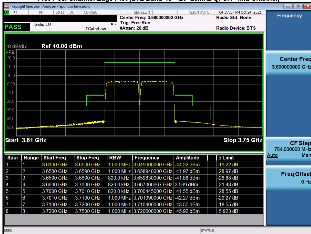
Plot 7-69. Channel Edge Plot (LTE Band 48 – 20+20MHz QPSK - High Channel)
