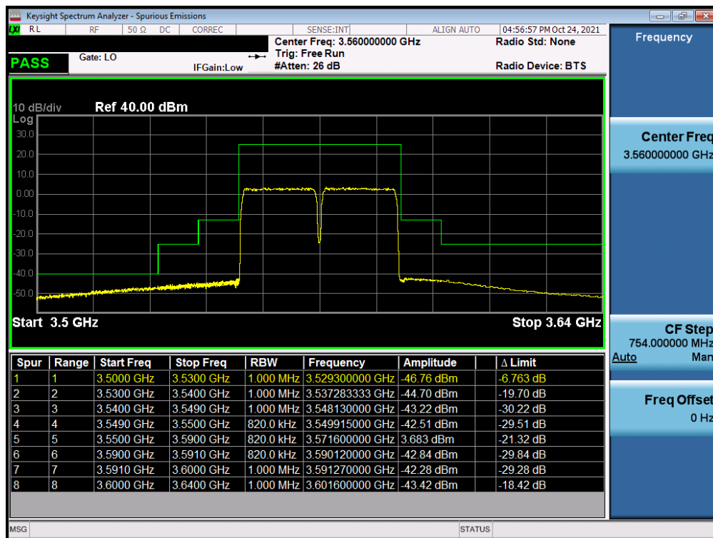
Plot 7-67. Channel Edge Plot (LTE Band 48 – 20+20MHz QPSK - Low Channel)
