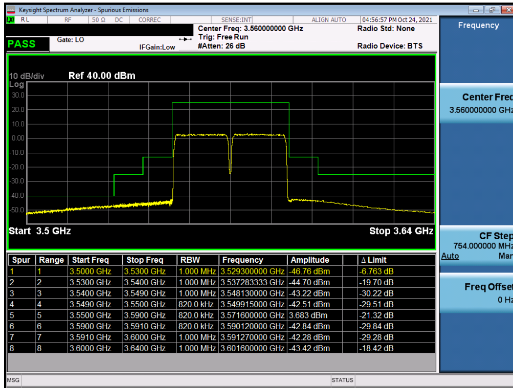
Plot 7-49. Channel Edge Plot (LTE Band 48 – 20+20MHz QPSK - Low Channel)
