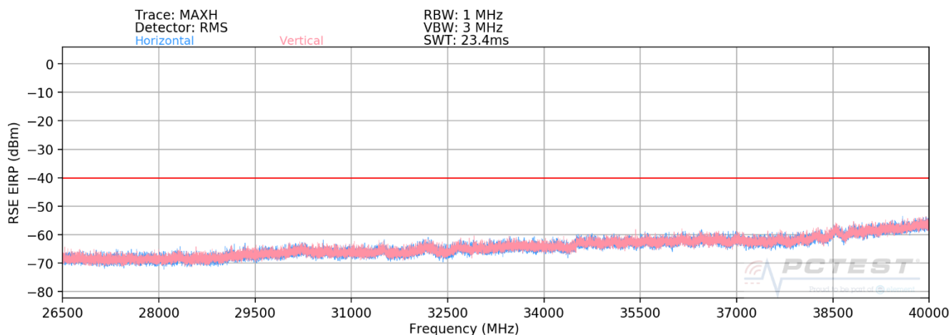
Plot 7-77. Radiated Spurious Plot (ULCA LB48)
