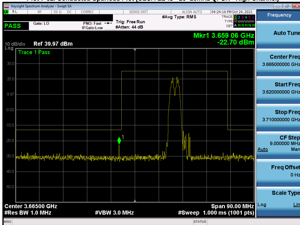
Plot 7-63. Conducted Spurious Plot (ULCA LB48 - 20+20MHz QPSK - High Channel)
