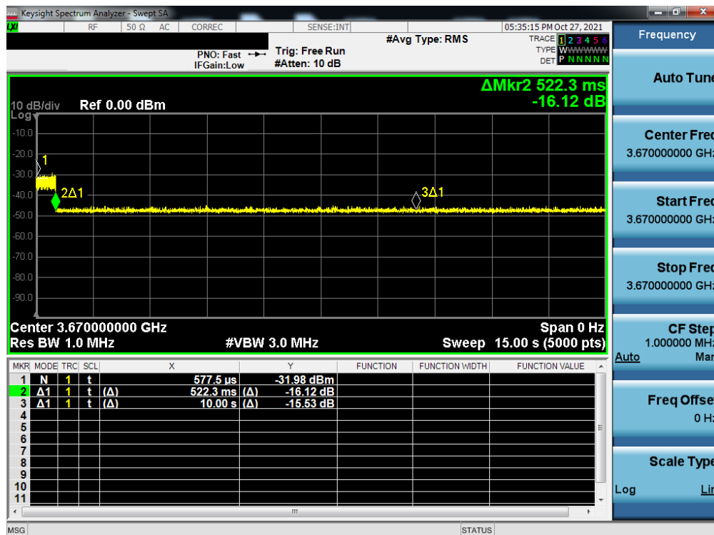
Plot 7-82. Run#2 End User Device Discontinues Operations within 10s
