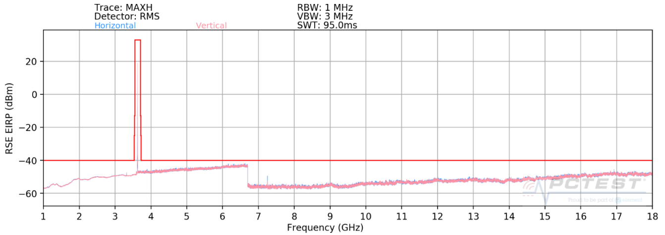
Plot 7-70. Radiated Spurious Plot (LTE Band 48)
