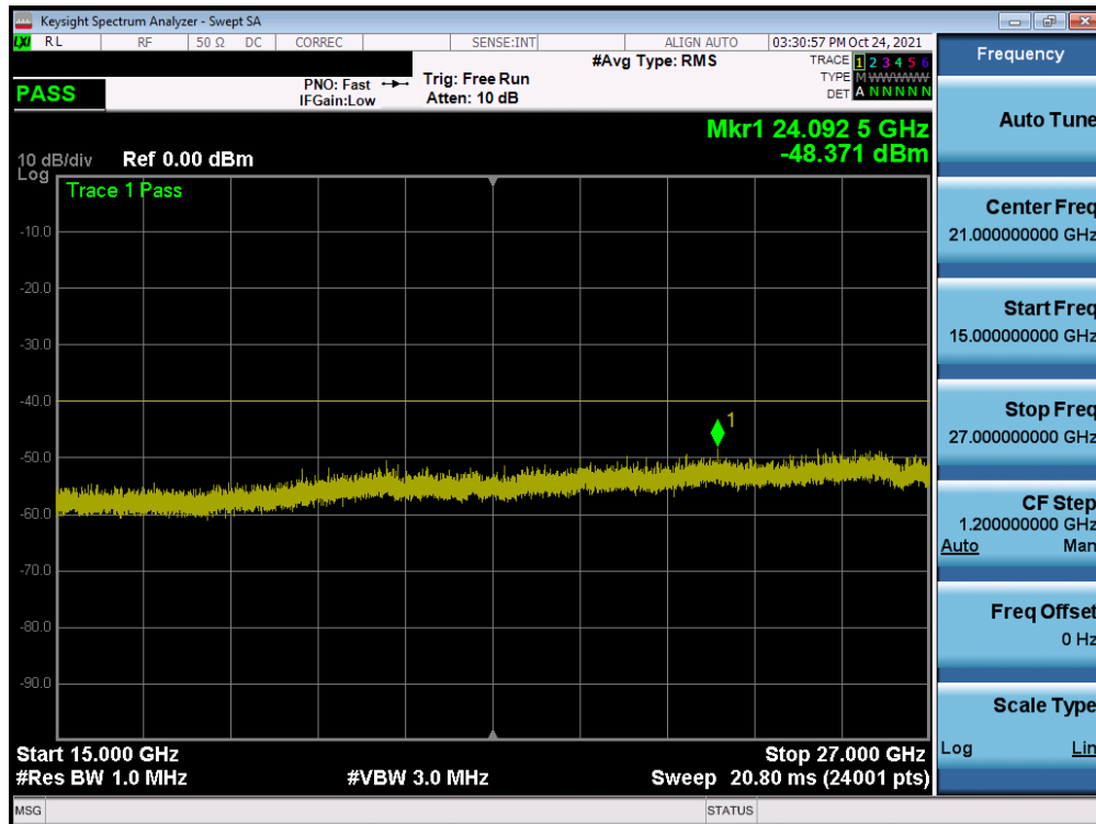
Plot 7-60. Conducted Spurious Plot (ULCA LB48 - 20+20MHz QPSK - Mid Channel)
