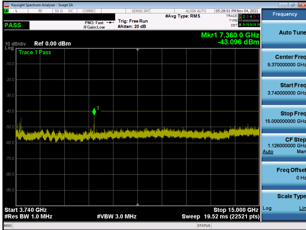
Plot 7-64. Conducted Spurious Plot (ULCA LB48 - 20+20MHz QPSK - High Channel)
