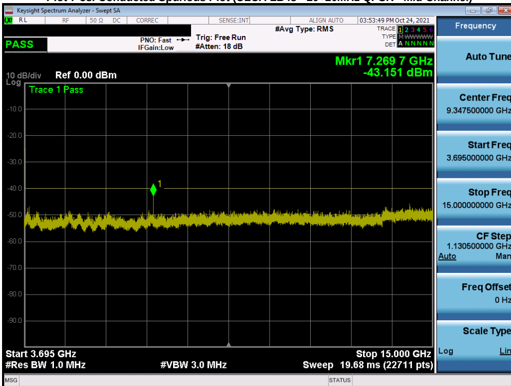
Plot 7-59. Conducted Spurious Plot (ULCA LB48 - 20+20MHz QPSK - Mid Channel)
