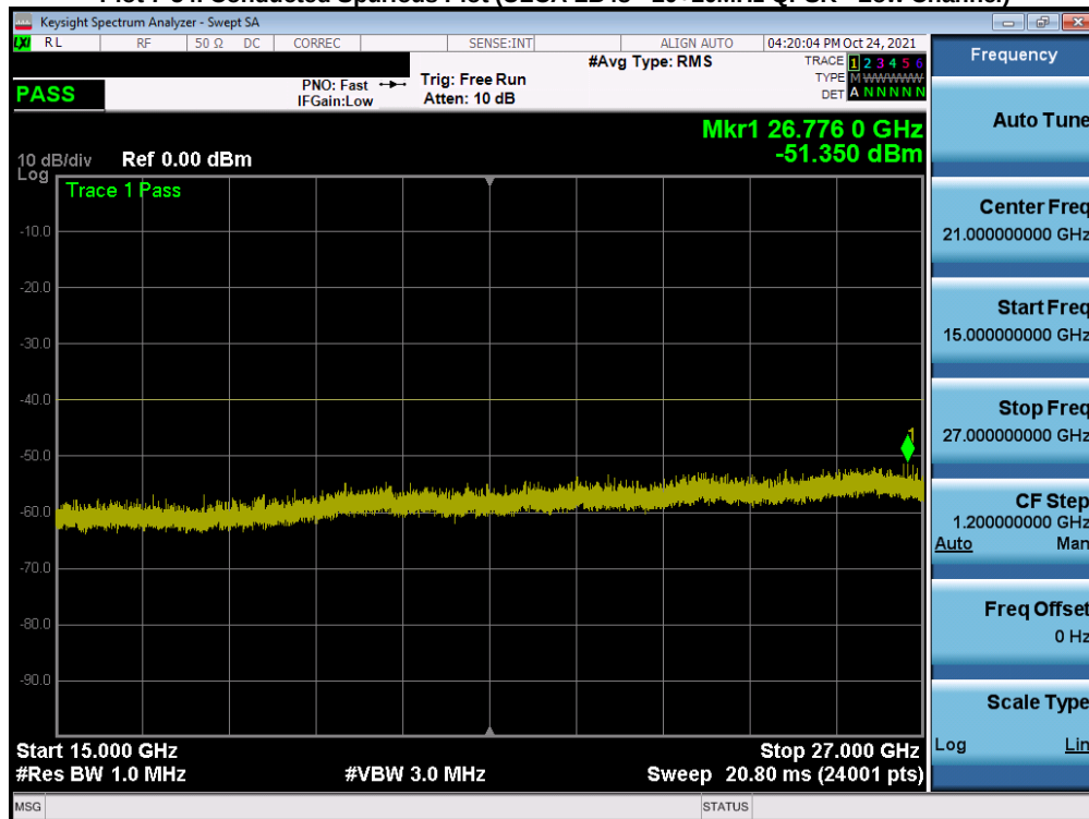
Plot 7-55. Conducted Spurious Plot (ULCA LB48 - 20+20MHz QPSK - Low Channel)
