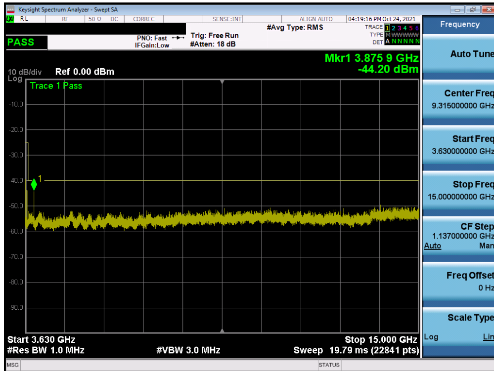
Plot 7-54. Conducted Spurious Plot (ULCA LB48 - 20+20MHz QPSK - Low Channel)
