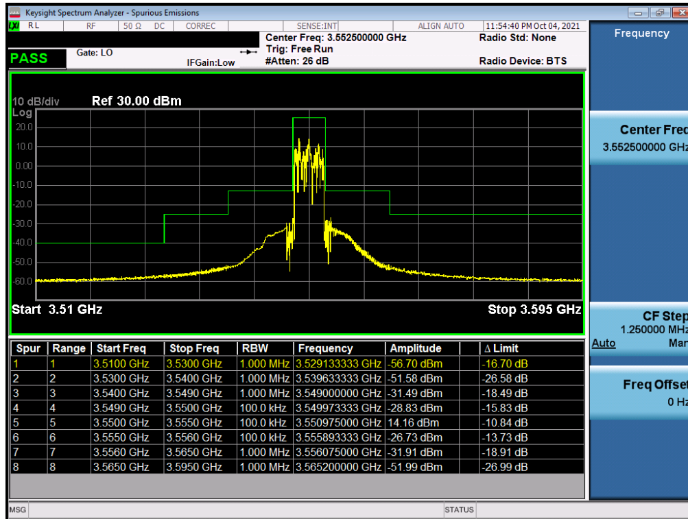
Plot 7-47. Channel Edge Plot (LTE Band 48 - 5MHz QPSK - Low Channel)
