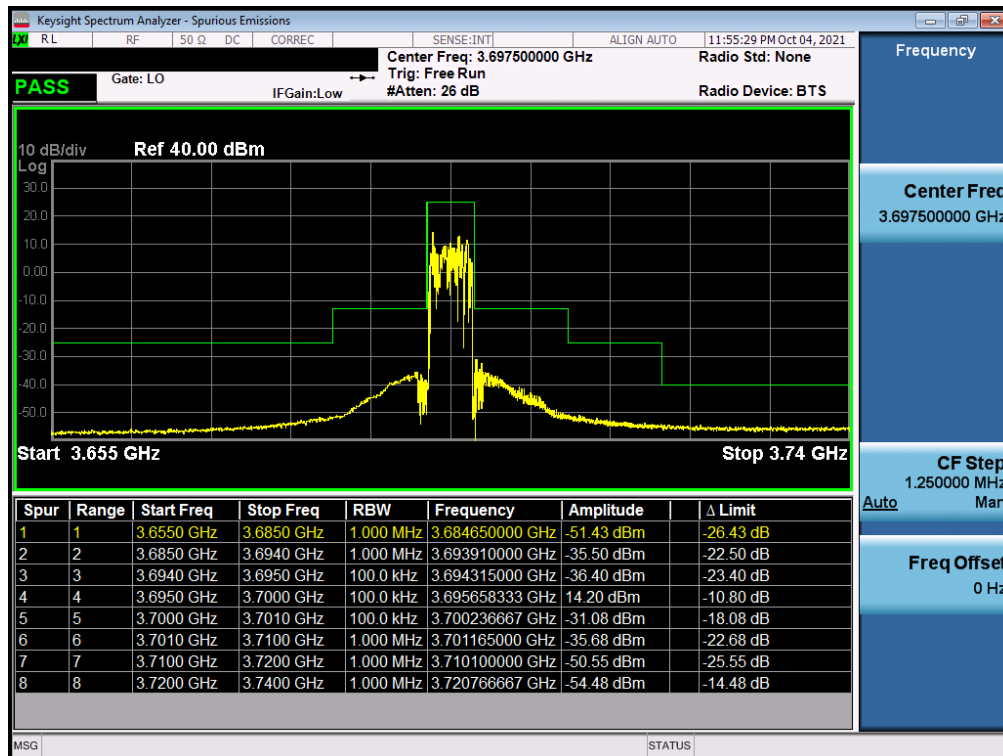
Plot 7-48. Channel Edge Plot (LTE Band 48 - 5MHz QPSK - High Channel)
