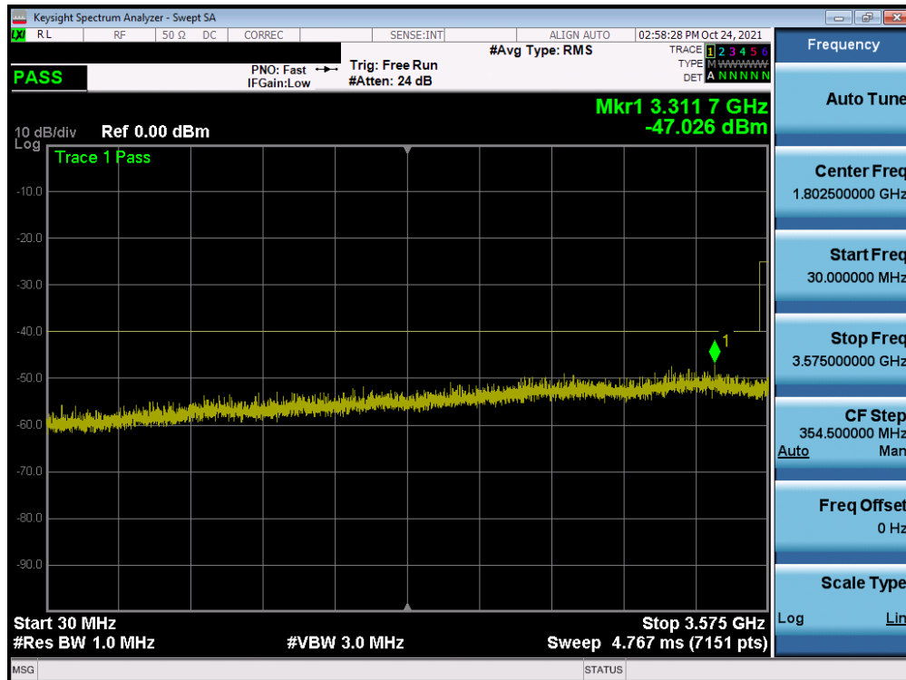
Plot 7-57. Conducted Spurious Plot (ULCA LB48 - 20+20MHz QPSK - Mid Channel)
