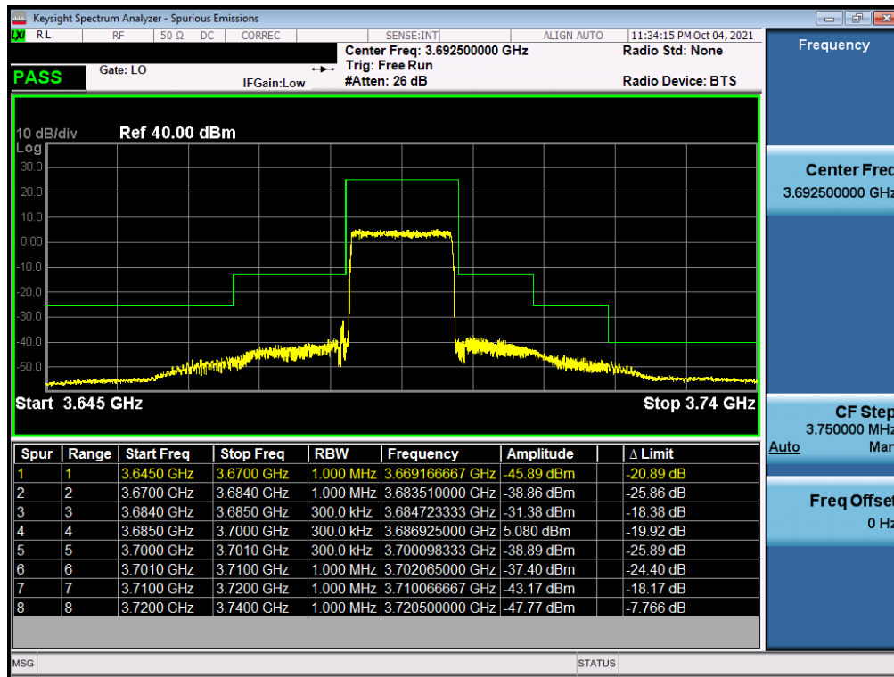
Plot 7-44. Channel Edge Plot (LTE Band 48 - 15MHz QPSK - High Channel)
