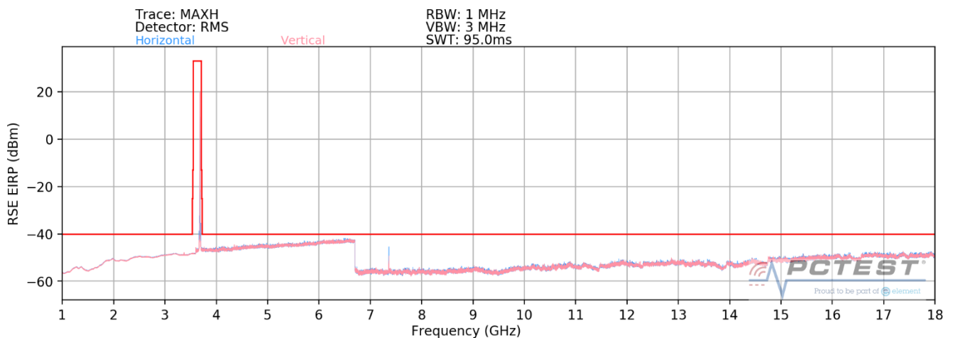
Plot 7-75. Radiated Spurious Plot (ULCA LB48 – High)
