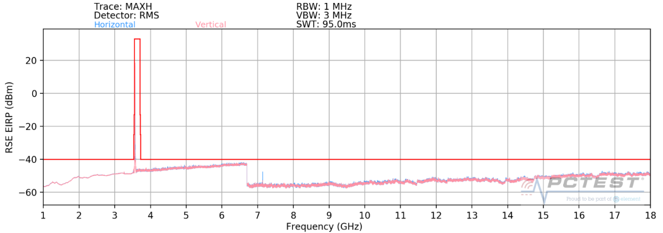
Plot 7-73. Radiated Spurious Plot (ULCA LB48 – Low)
