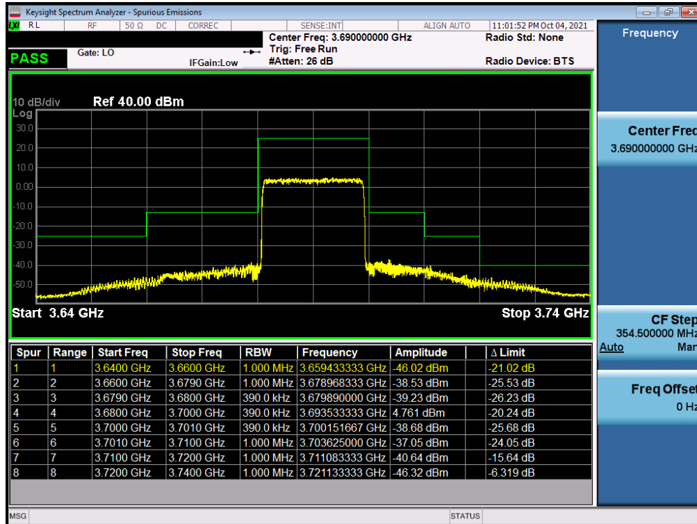
Plot 7-42. Channel Edge Plot (LTE Band 48 - 20MHz QPSK - High Channel)
