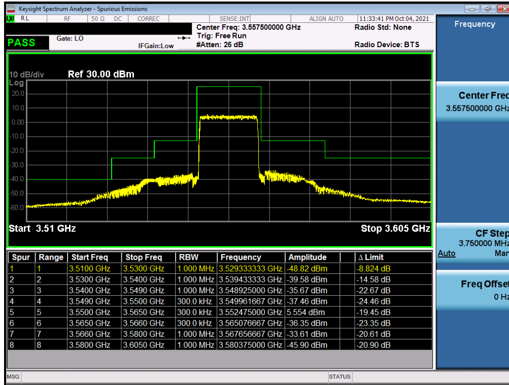
Plot 7-43. Channel Edge Plot (LTE Band 48 - 15MHz QPSK - Low Channel)
