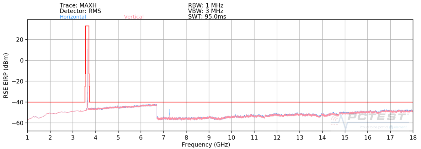
Plot 7-74. Radiated Spurious Plot (ULCA LB48 – Mid)
