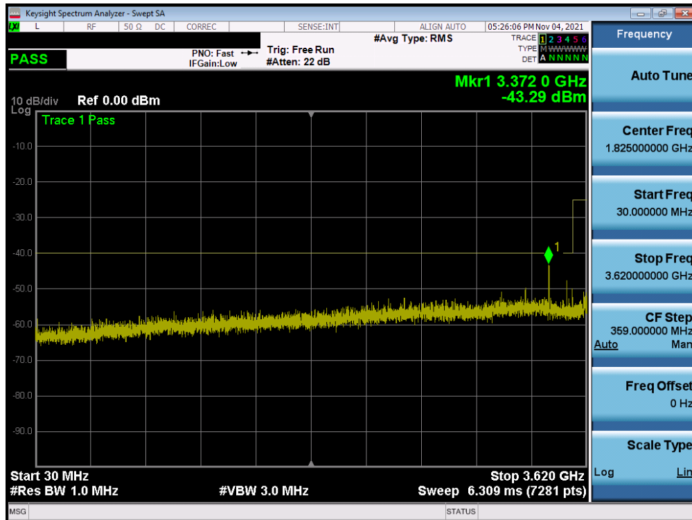
Plot 7-62. Conducted Spurious Plot (ULCA LB48 - 20+20MHz QPSK - High Channel)
