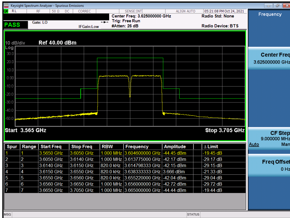
Plot 7-68. Channel Edge Plot (LTE Band 48 – 20+20MHz QPSK - Mid Channel)
