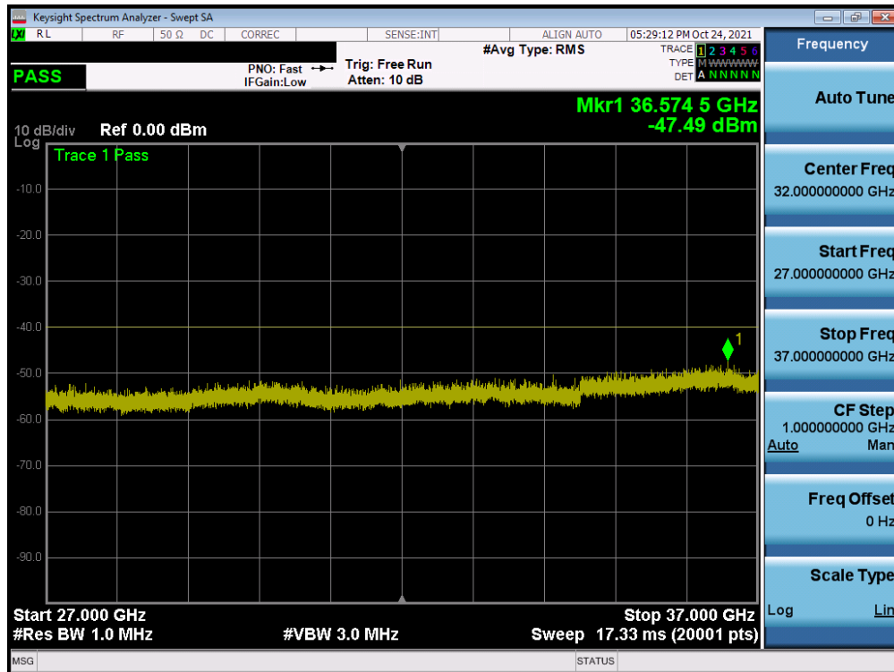
Plot 7-66. Conducted Spurious Plot (ULCA LB48 - 20+20MHz QPSK - High Channel)
