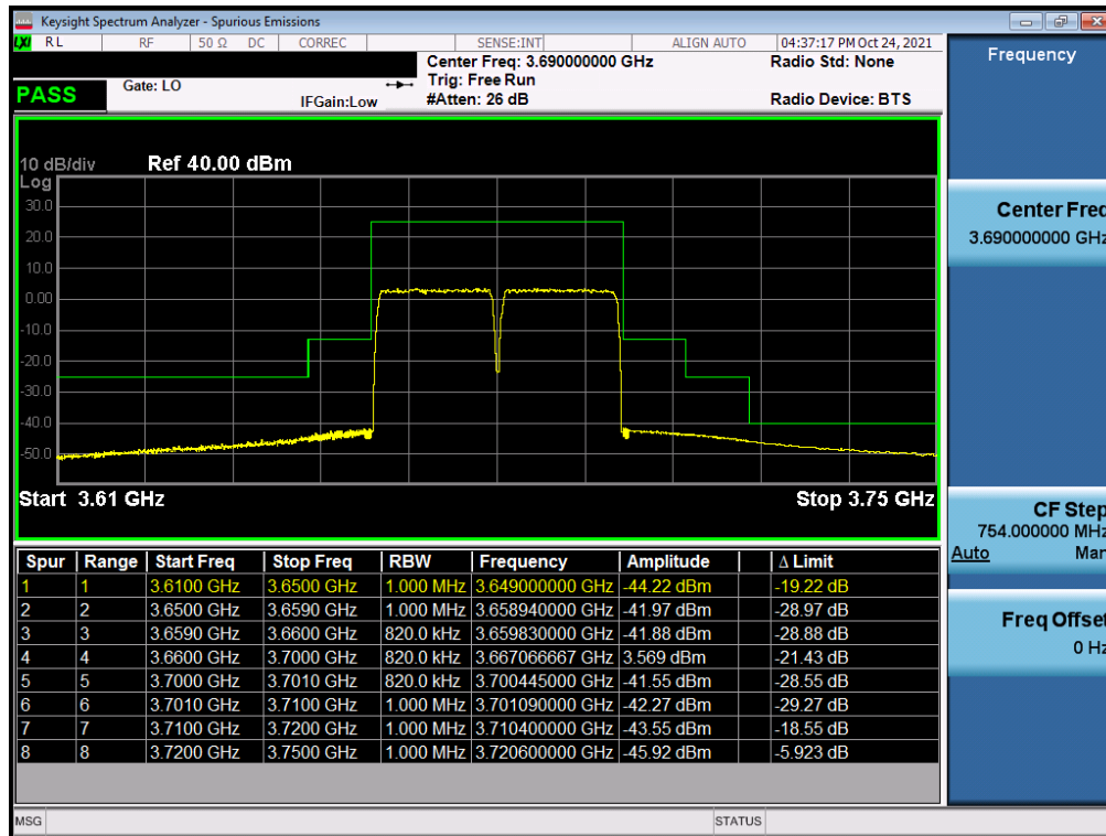
Plot 7-51. Channel Edge Plot (LTE Band 48 – 20+20MHz QPSK - High Channel)
