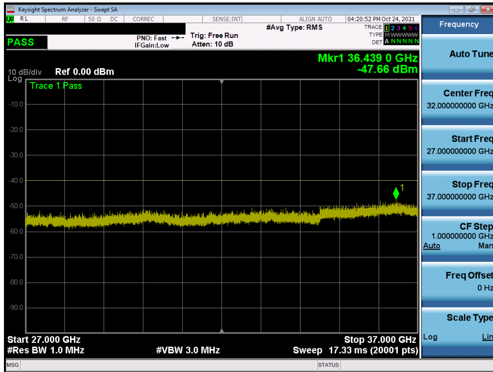
Plot 7-56. Conducted Spurious Plot (ULCA LB48 - 20+20MHz QPSK - Low Channel)
