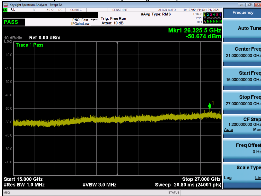
Plot 7-65. Conducted Spurious Plot (ULCA LB48 - 20+20MHz QPSK - High Channel)
