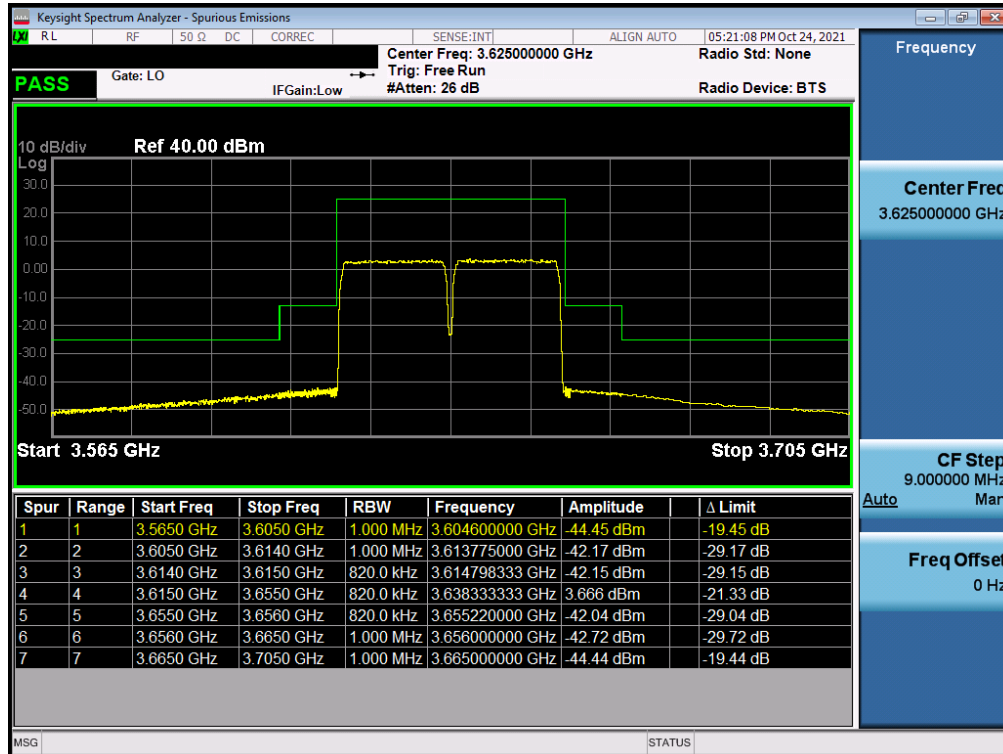
Plot 7-50. Channel Edge Plot (LTE Band 48 – 20+20MHz QPSK - Mid Channel)
