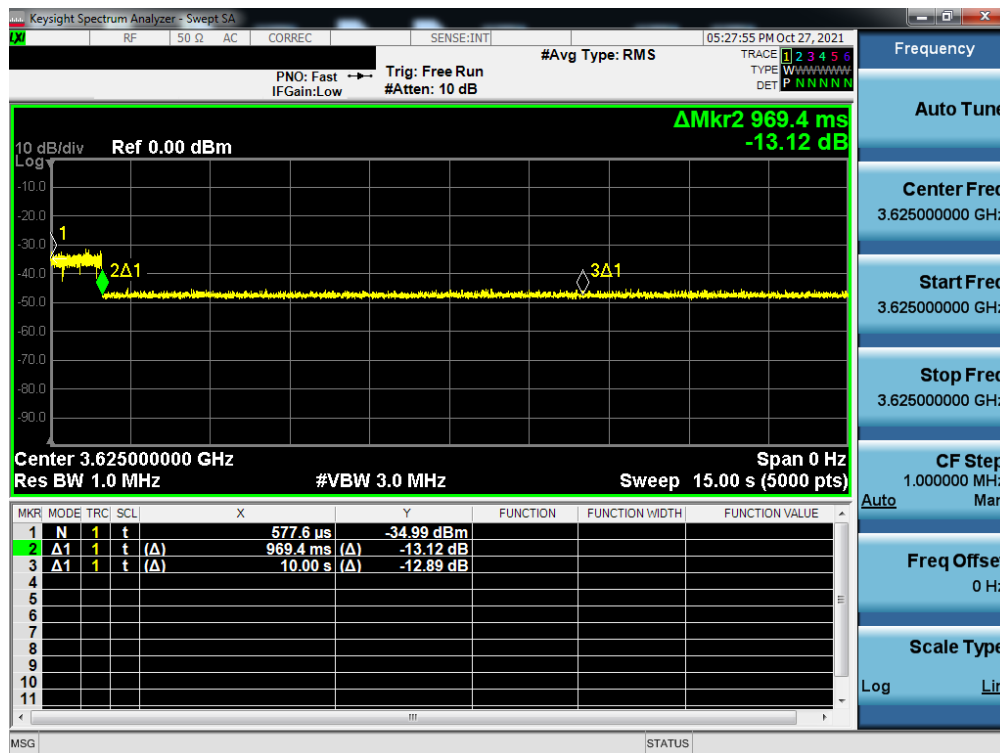
Plot 7-80. Run#1 End User Device Discontinues Operations within 10s
