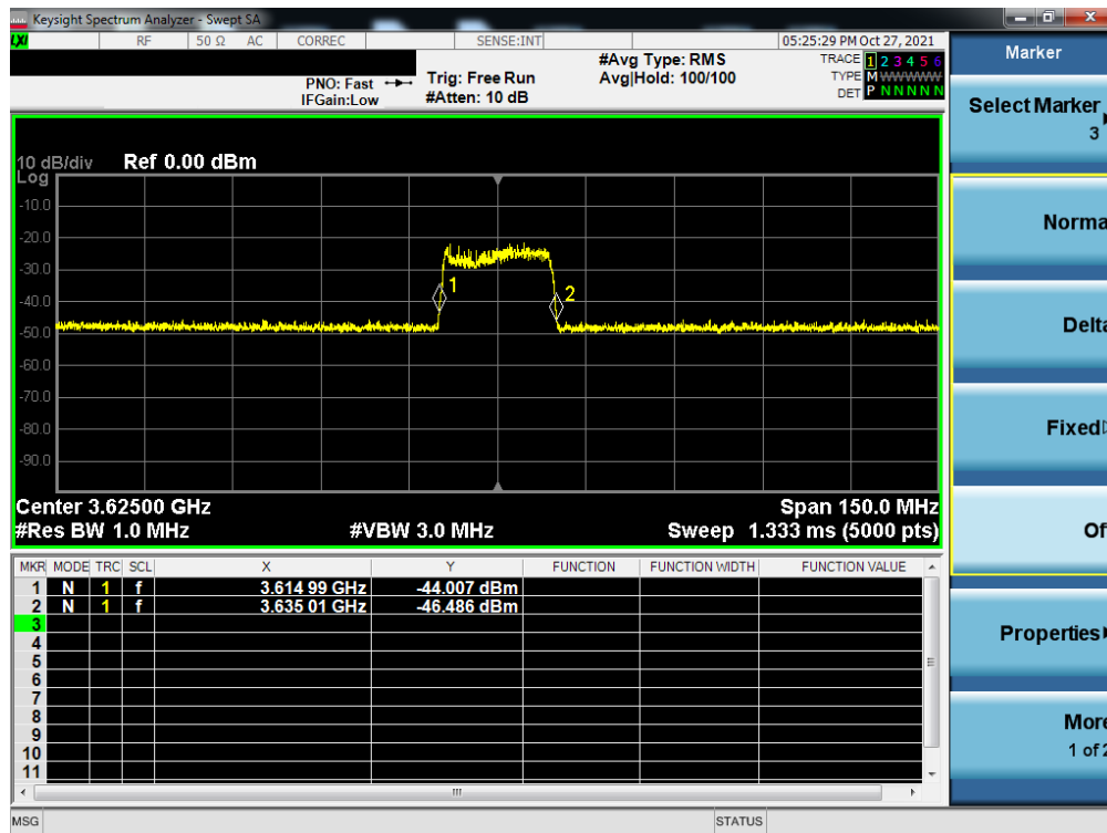
Plot 7-79. Run#1 End User Device Frequency of Operations
