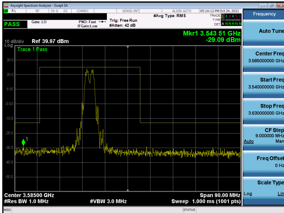
Plot 7-53. Conducted Spurious Plot (ULCA LB48 - 20+20MHz QPSK - Low Channel)
