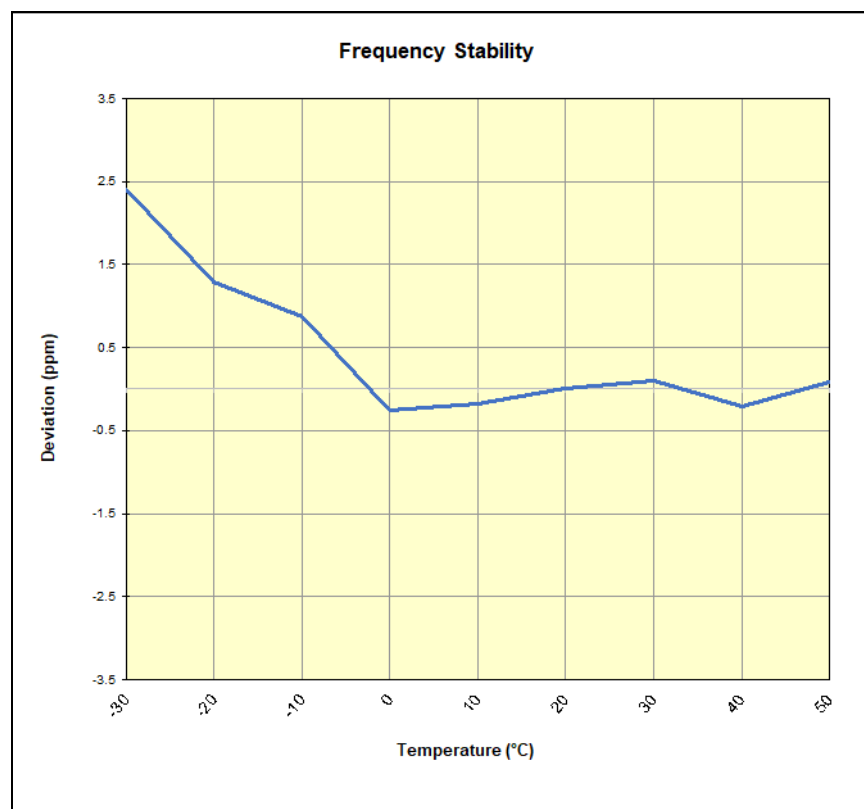
Plot 7-78. LTE Band 48 Frequency Stability Chart
