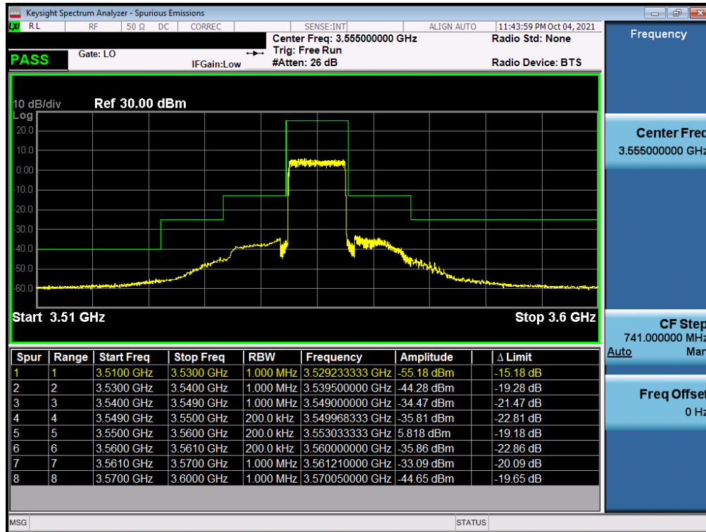
Plot 7-45. Channel Edge Plot (LTE Band 48 - 10MHz QPSK - Low Channel)
