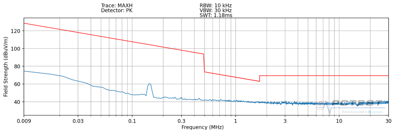
Plot 7-5Radiated Spurious Plot 9kHz – 30MHz (Pol. Y – Device to Device WPT – Config 2)
