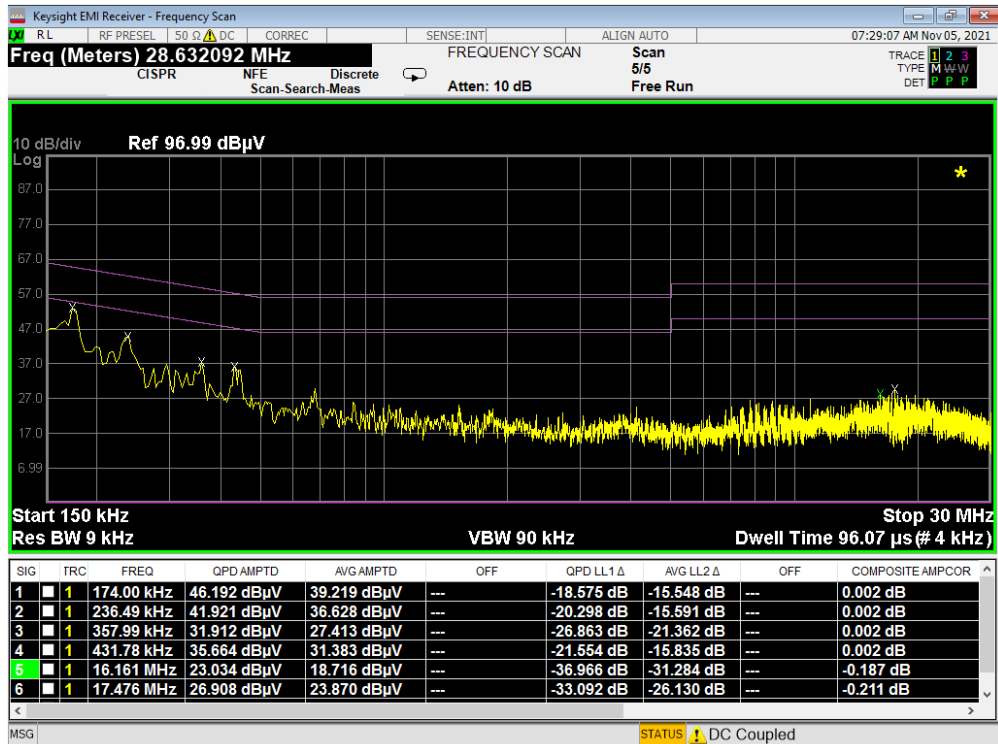
Plot 7-11. Line-Conducted Test Plot (N) - Device to Device – Config 1
