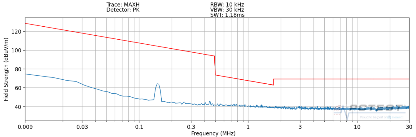
Plot 7-7. Radiated Spurious Plot 9kHz – 30MHz (Pol. X – Device to Device WPT – Config 3)
