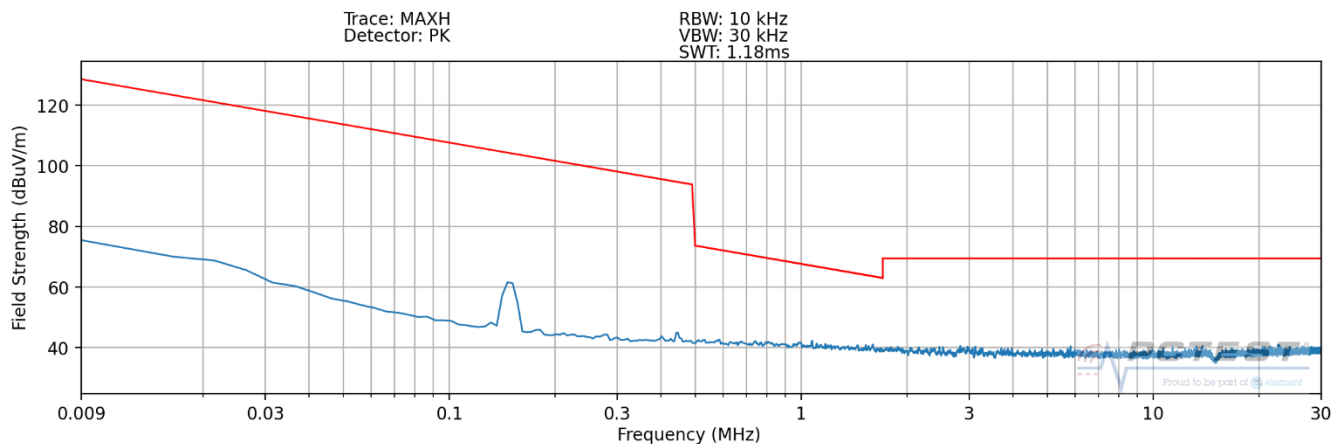
Plot 7-8 Radiated Spurious Plot 9kHz – 30MHz (Pol. Y – Device to Device WPT – Config 3)
