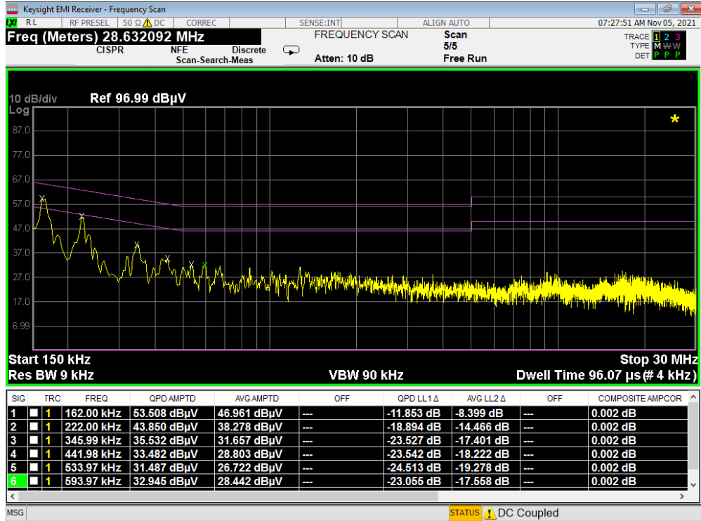
Plot 7-10. Line-Conducted Test Plot (L1) - Device to Device – Config 1
