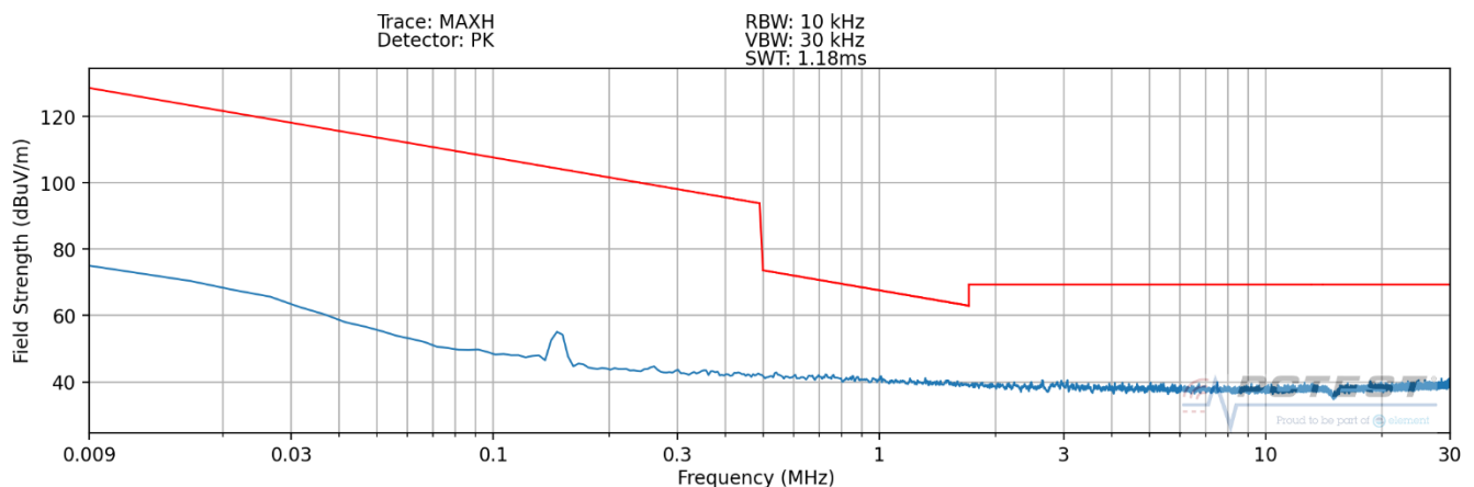
Plot 7-3. Radiated Spurious Plot 9kHz – 30MHz (Pol. Z – Device to Device WPT – Config 1)
