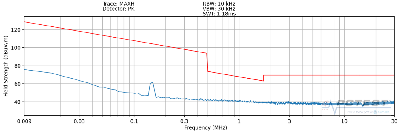
Plot 7-1. Radiated Spurious Plot 9kHz – 30MHz (Pol. X – Device to Device WPT – Config 1)
