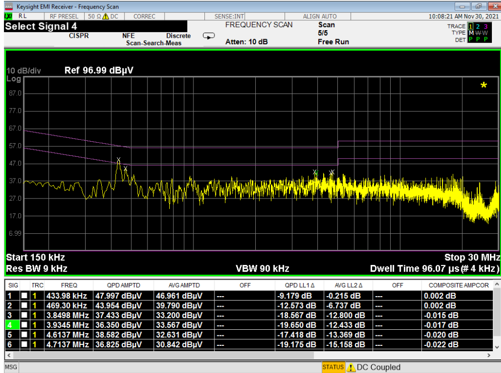
Plot 7-12. Line-Conducted Test Plot (L1) - Device to Device – Config 2
