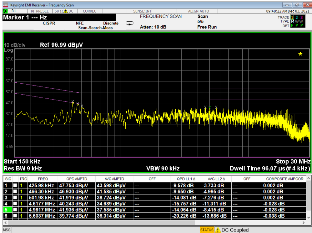
Plot 7-15. Line-Conducted Test Plot (N) - Device to Device – Config 3
