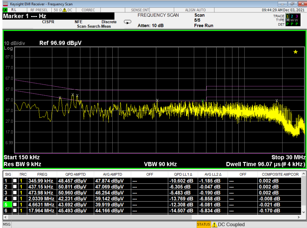
Plot 7-14. Line-Conducted Test Plot (L1) - Device to Device – Config 3
