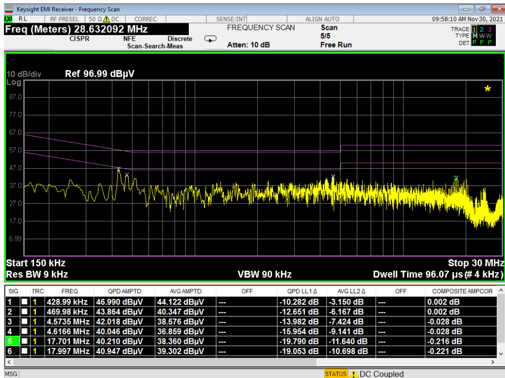
Plot 7-13. Line-Conducted Test Plot (N) - Device to Device – Config 2
