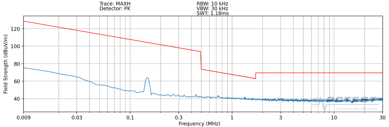
Plot 7-4. Radiated Spurious Plot 9kHz – 30MHz (Pol. X – Device to Device WPT – Config 2)
