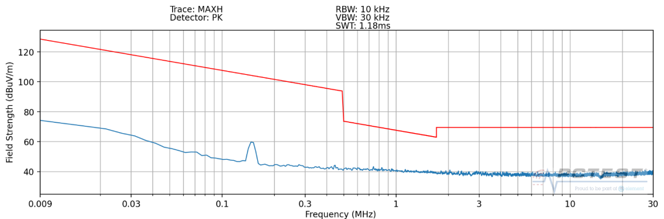
Plot 7-9. Radiated Spurious Plot 9kHz – 30MHz (Pol. Z – Device to Device WPT – Config 3)
