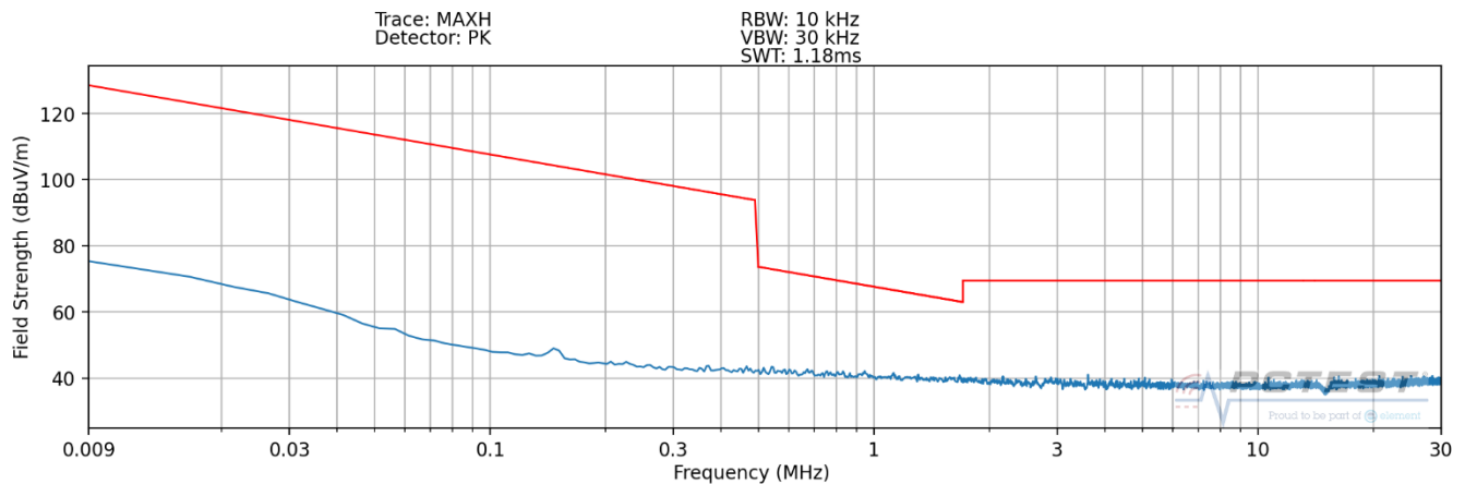
Plot 7-2 Radiated Spurious Plot 9kHz – 30MHz (Pol. Y – Device to Device WPT – Config 1)
