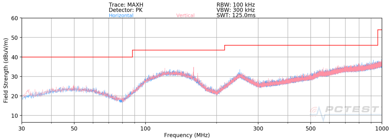
Plot 7-25. 30MHz - 1 GHz Pre-Scan Plots ANT1 – CH 5
