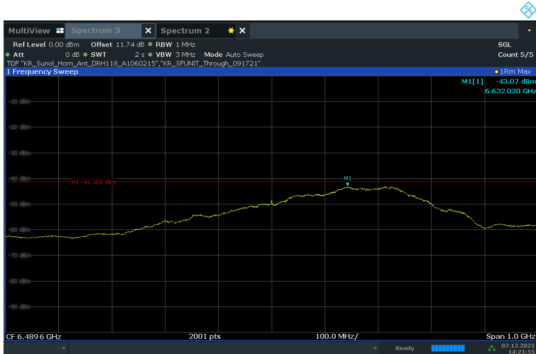
Plot 7-17. UWB Average Power Measurement - ANT 1 - CH.5 – BPRF
