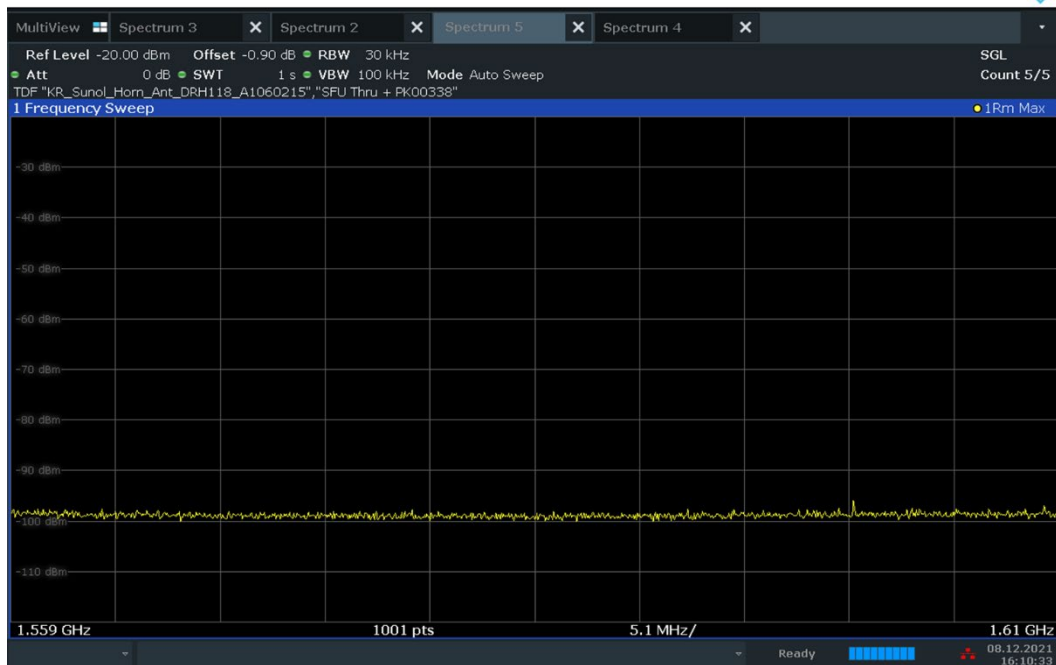
Plot 7-23. Radiated Spurious Pre-Scan 1559 - 1610 MHz - CH.5 - ANT 1 – GPS band
