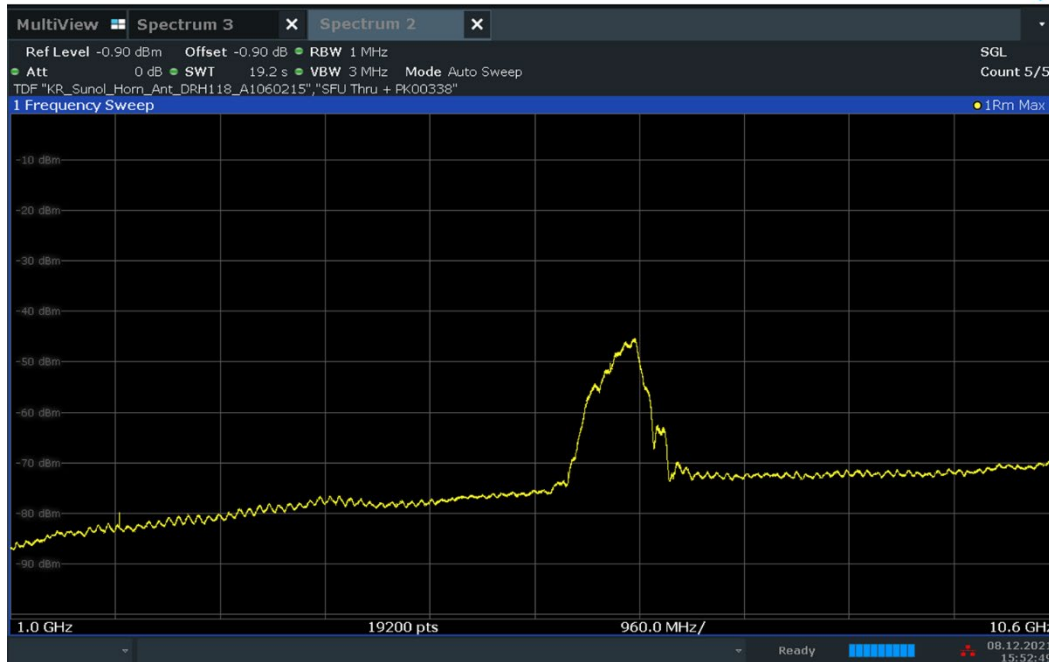
Plot 7-20. Radiated Spurious Pre-Scan 1000 - 10600 MHz - CH.5 - ANT 1
