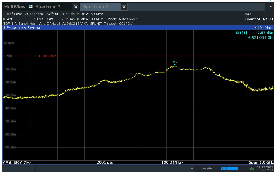
Plot 7-18. UWB Peak Power Measurement - ANT 1 - CH.5 – HPRF
