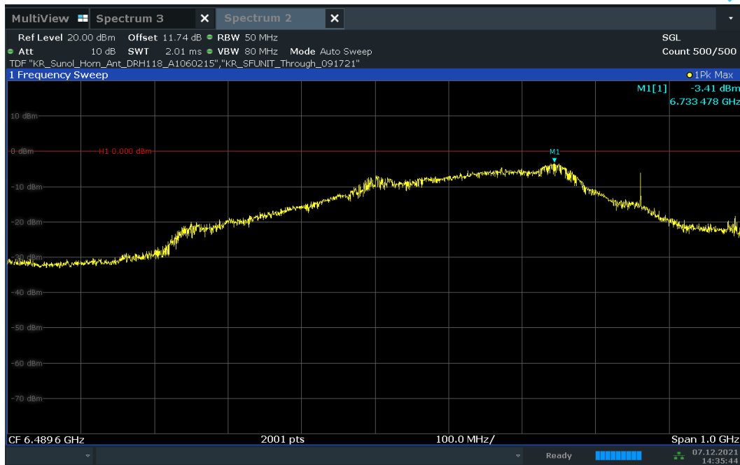
Plot 7-16. UWB Peak Power Measurement - ANT 1 - CH.5 – BPRF
