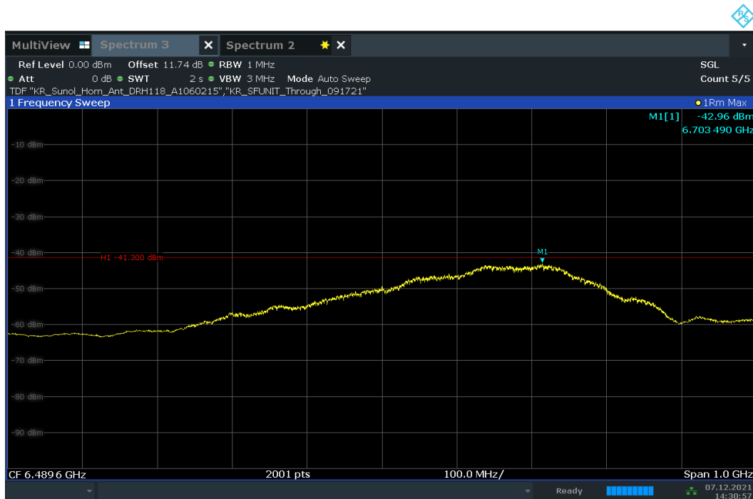
Plot 7-19. UWB Average Power Measurement - ANT 1 - CH.5 – HPRF
