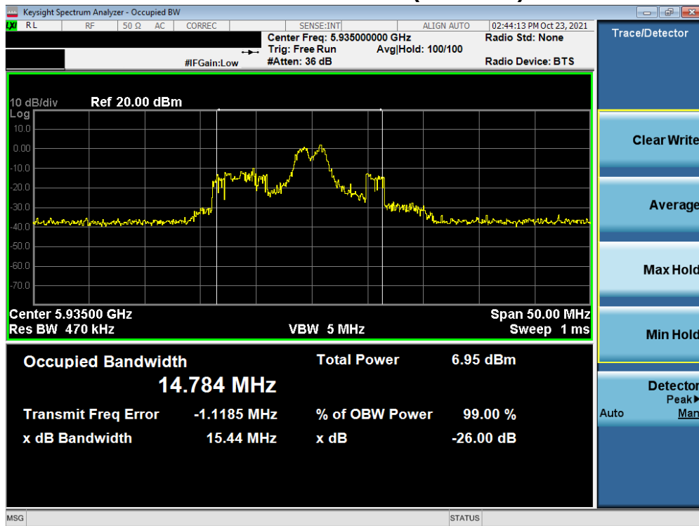
Plot 7-81. 26dB Bandwidth Plot MIMO ANT2 (20MHz BW 802.11ax (26 Tones) UNII Band 5) – Ch. 2)
