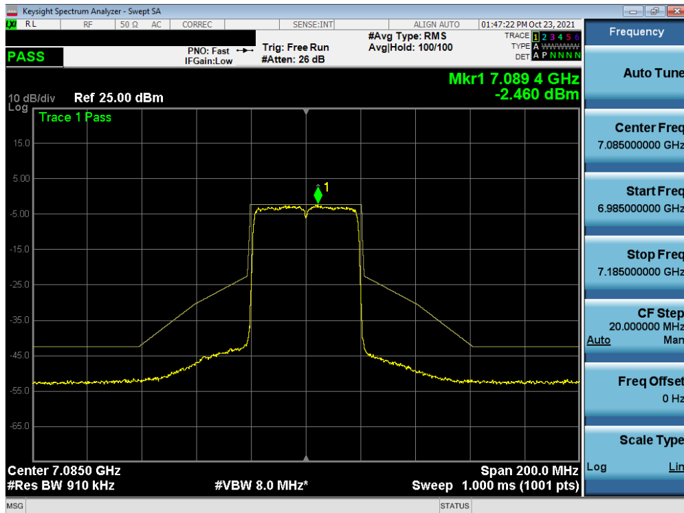
Plot 7-384. In-Band Emission Plot MIMO ANT1 (40MHz BW 802.11ax (Full Tones) (UNII Band 8) – Ch. 227)
