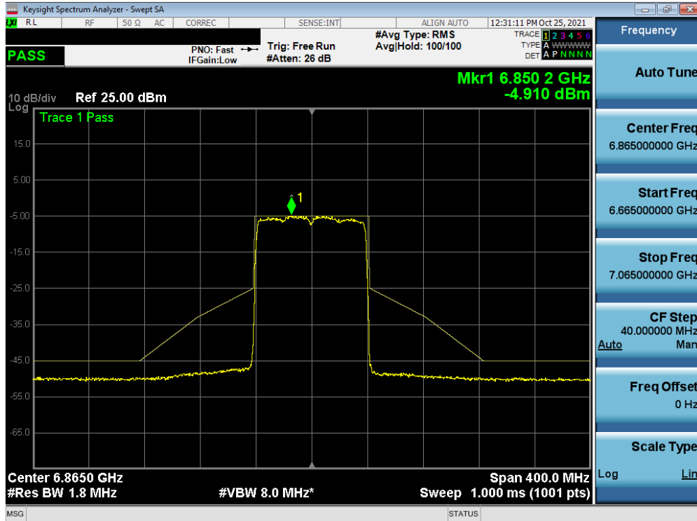
Plot 7-444. In-Band Emission Plot MIMO ANT2 (80MHz BW 802.11ax (Full Tones) (UNII Band 7) – Ch. 183)
