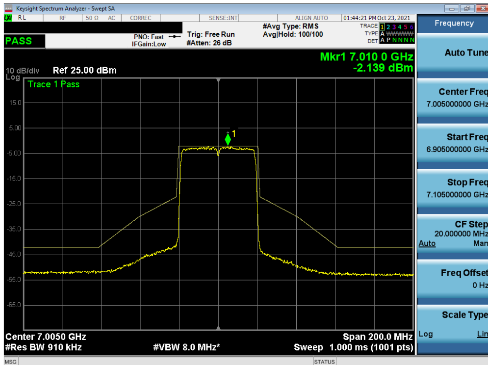
Plot 7-383. In-Band Emission Plot MIMO ANT1 (40MHz BW 802.11ax (Full Tones) (UNII Band 8) – Ch. 211)
