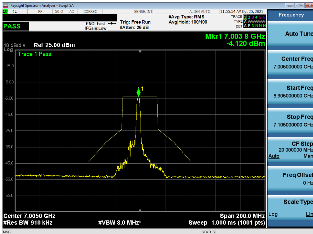
Plot 7-416. In-Band Emission Plot MIMO ANT2 (40MHz BW 802.11ax (26 Tones) (UNII Band 8) – Ch. 211)
