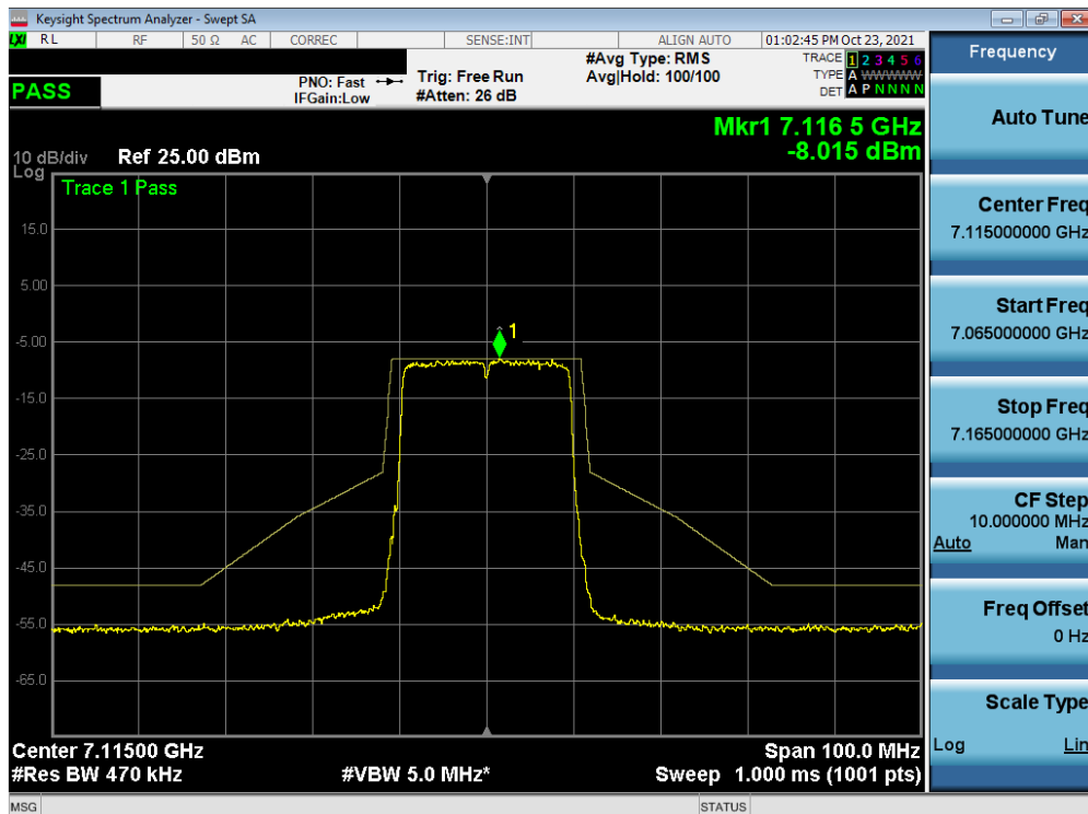
Plot 7-381. In-Band Emission Plot MIMO ANT1 (20MHz BW 802.11ax (Full Tones) (UNII Band 8) – Ch. 233)
