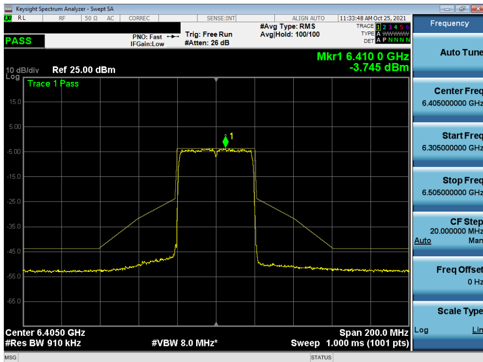
Plot 7-425. In-Band Emission Plot MIMO ANT2 (40MHz BW 802.11ax (Full Tones) (UNII Band 5) – Ch. 91)
