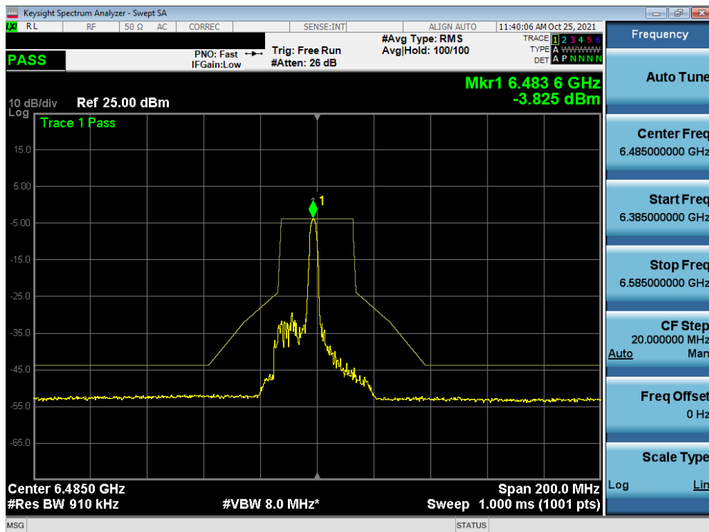
Plot 7-400. In-Band Emission Plot MIMO ANT2 (40MHz BW 802.11ax (26 Tones) (UNII Band 6) – Ch. 107)
