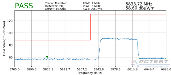
Plot 7-465. Radiated Lower Band Edge Plot MIMO (Peak – UNII Band 5)
