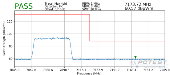
Plot 7-464. Radiated Upper Band Edge Plot MIMO (Peak – UNII Band 8)
