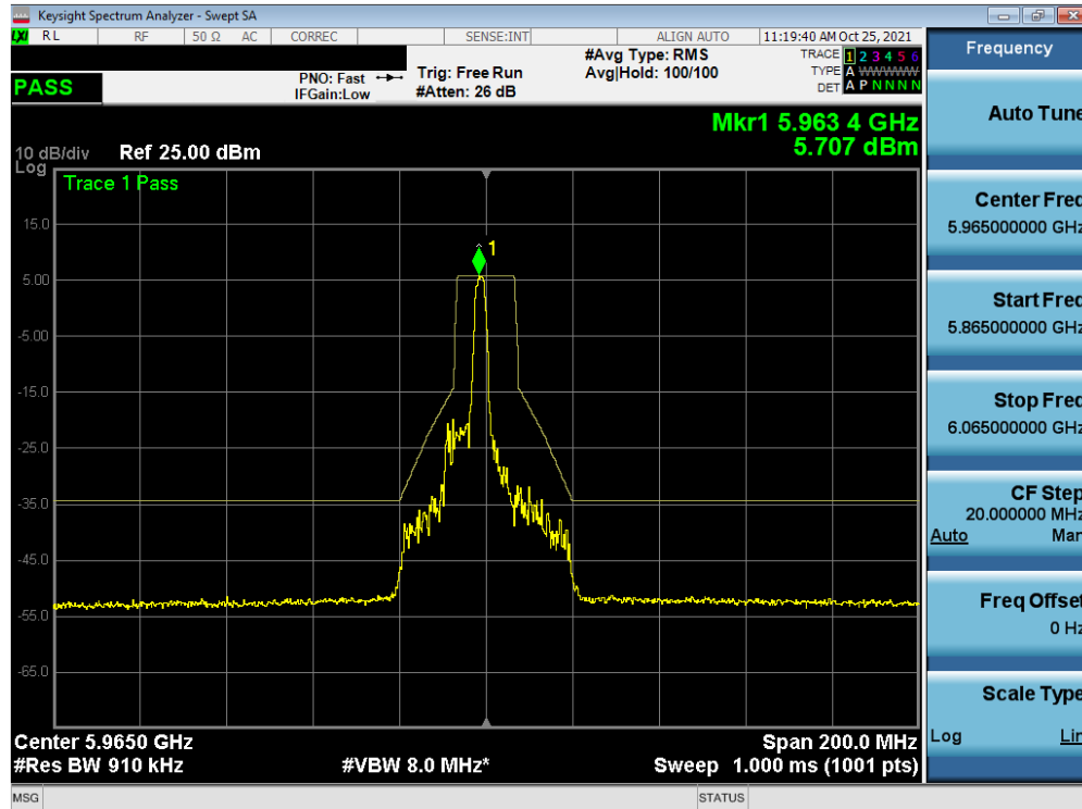
Plot 7-390. In-Band Emission Plot MIMO ANT2 (40MHz BW 802.11ax (26 Tones) (UNII Band 5) – Ch. 3)
