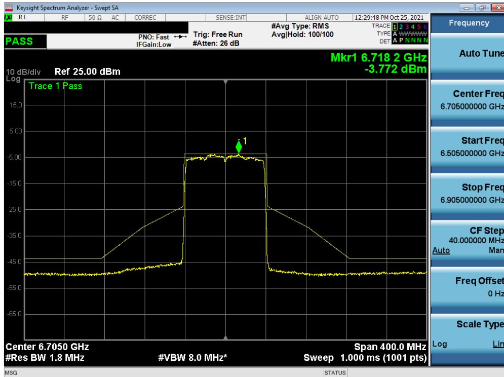
Plot 7-443. In-Band Emission Plot MIMO ANT2 (80MHz BW 802.11ax (Full Tones) (UNII Band 7) – Ch. 151)
