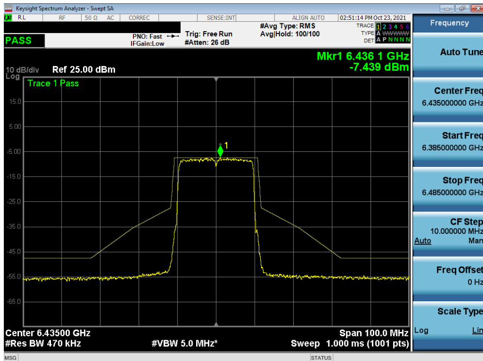
Plot 7-429. In-Band Emission Plot MIMO ANT2 (20MHz BW 802.11ax (Full Tones) (UNII Band 6) – Ch. 97)
