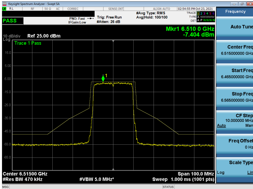
Plot 7-431. In-Band Emission Plot MIMO ANT2 (20MHz BW 802.11ax (Full Tones) (UNII Band 6) – Ch. 113)
