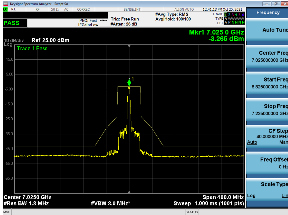
Plot 7-419. In-Band Emission Plot MIMO ANT2 (80MHz BW 802.11ax (26 Tones) (UNII Band 8) – Ch. 215)
