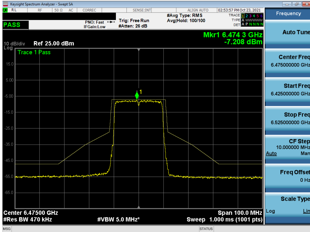
Plot 7-430. In-Band Emission Plot MIMO ANT2 (20MHz BW 802.11ax (Full Tones) (UNII Band 6) – Ch. 105)
