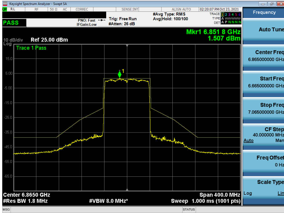
Plot 7-378. In-Band Emission Plot MIMO ANT1 (80MHz BW 802.11ax (Full Tones) (UNII Band 7) – Ch. 183)
