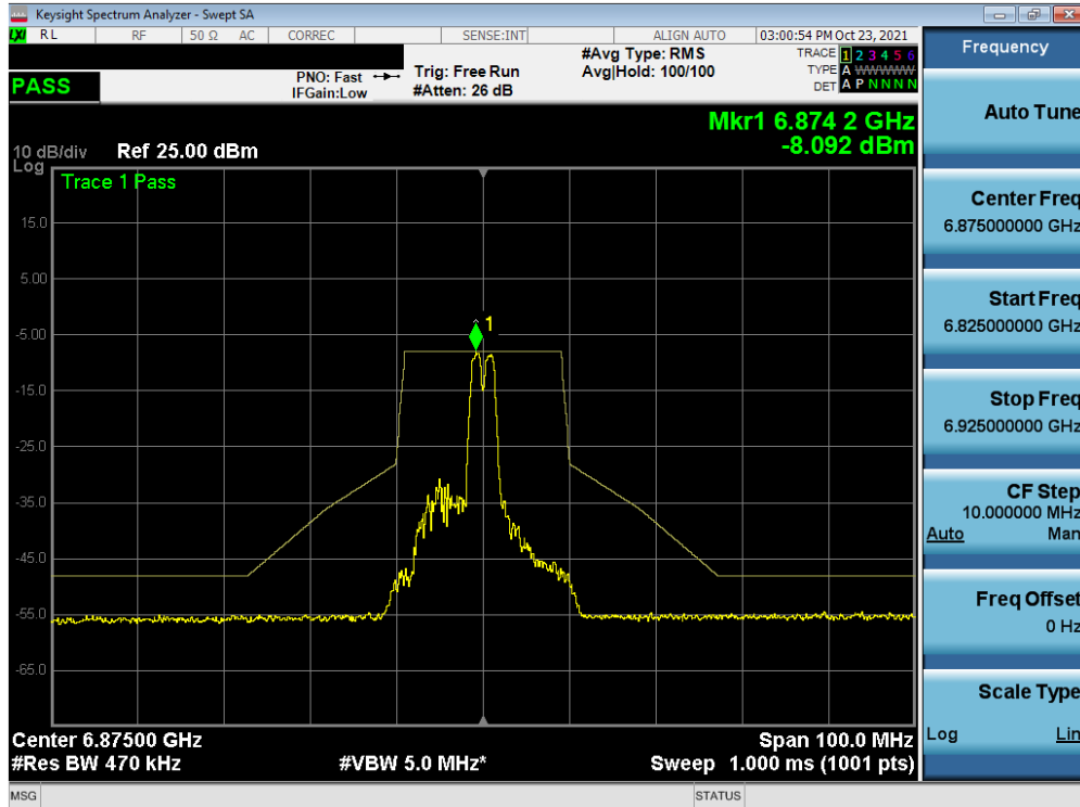
Plot 7-405. In-Band Emission Plot MIMO ANT2 (20MHz BW 802.11ax (26 Tones) (UNII Band 7) – Ch. 185)
