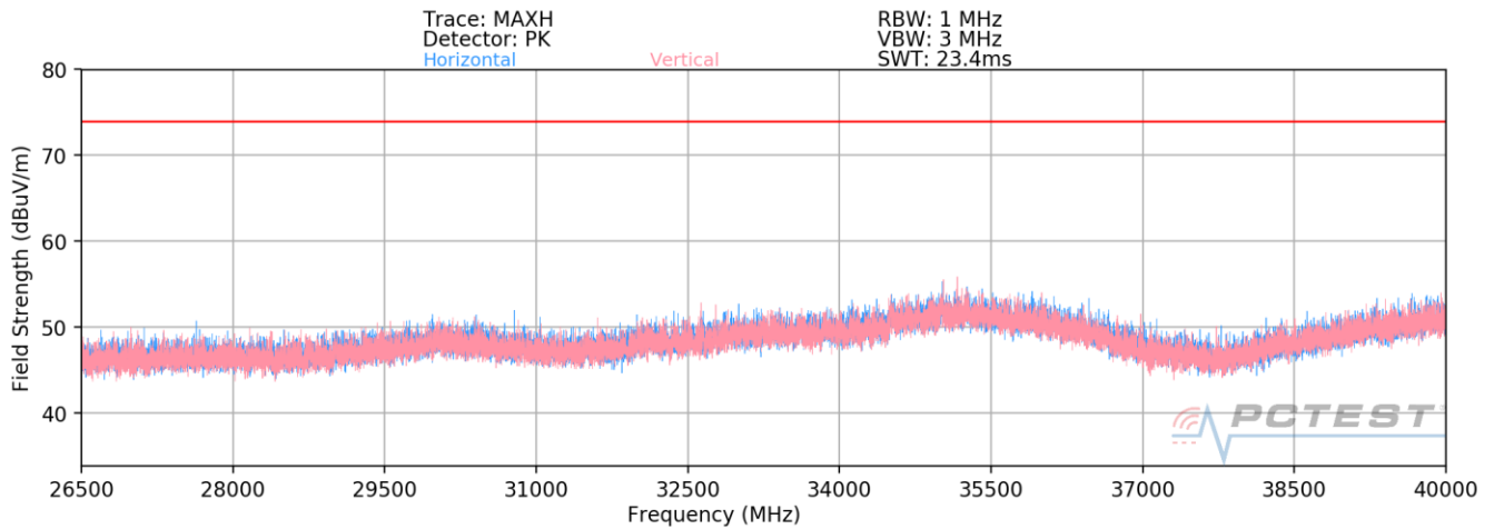
Plot 7-458. Radiated Spurious Plot 26.5GHz - 40GHz MIMO (802.11ax – Partial Tones)
