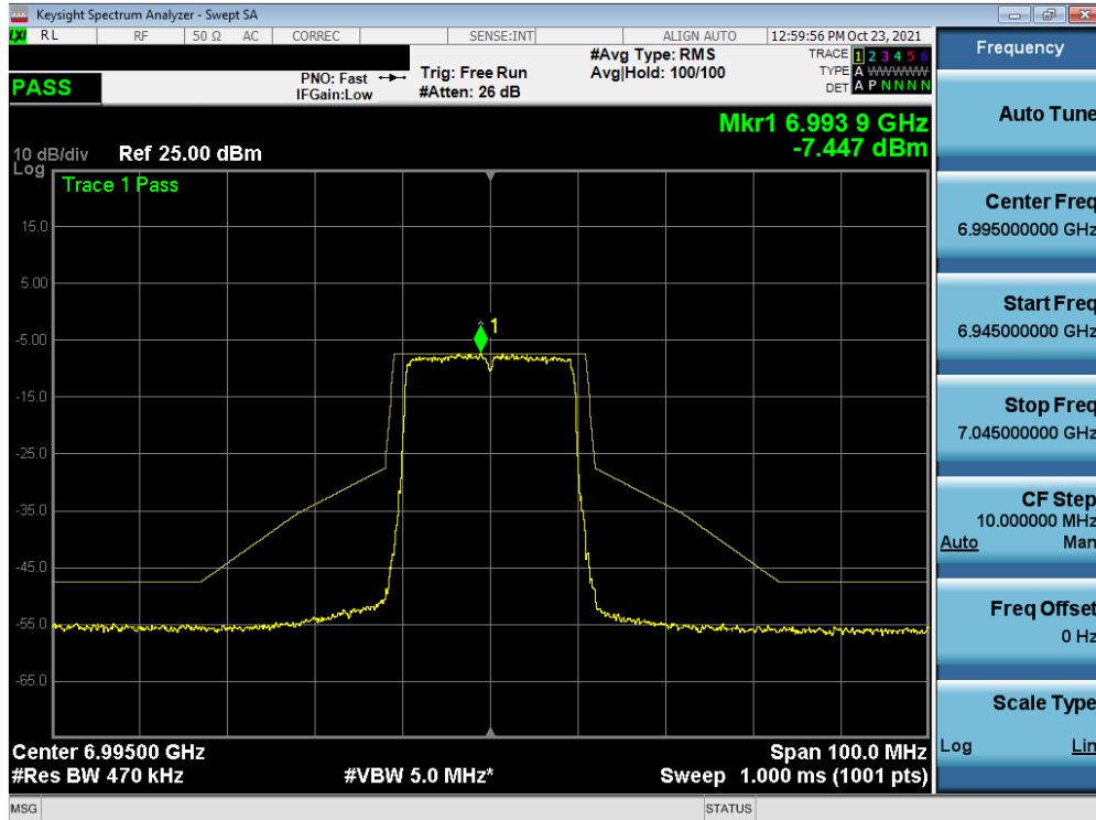
Plot 7-380. In-Band Emission Plot MIMO ANT1 (20MHz BW 802.11ax (Full Tones) (UNII Band 8) – Ch. 209)
