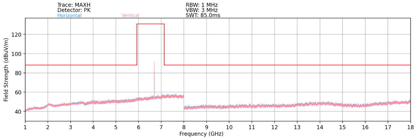
Plot 7-455. Radiated Spurious Plot above 1GHz MIMO (802.11ax)
