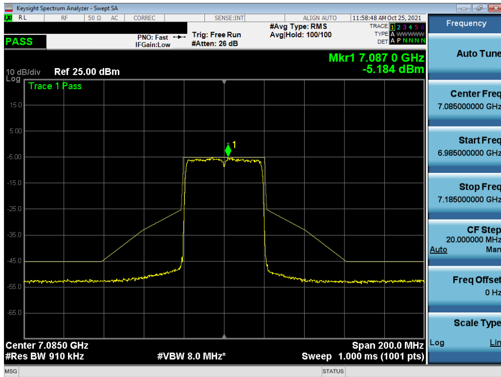
Plot 7-450. In-Band Emission Plot MIMO ANT2 (40MHz BW 802.11ax (Full Tones) (UNII Band 8) – Ch. 227)
