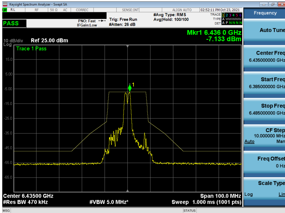
Plot 7-396. In-Band Emission Plot MIMO ANT2 (20MHz BW 802.11ax (26 Tones) (UNII Band 6) – Ch. 97)
