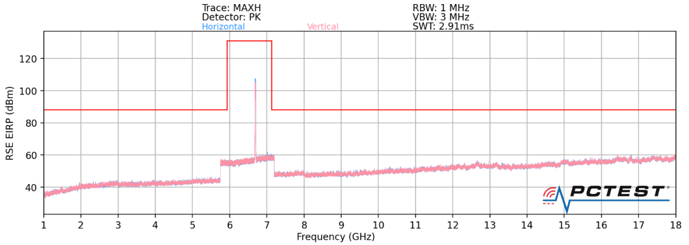
Plot 7-456. Radiated Spurious Plot above 1GHz MIMO (802.11ax)
