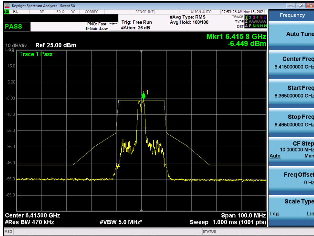
Plot 7-389. In-Band Emission Plot MIMO ANT2 (20MHz BW 802.11ax (26 Tones) UNII Band 5) – Ch. 93)
