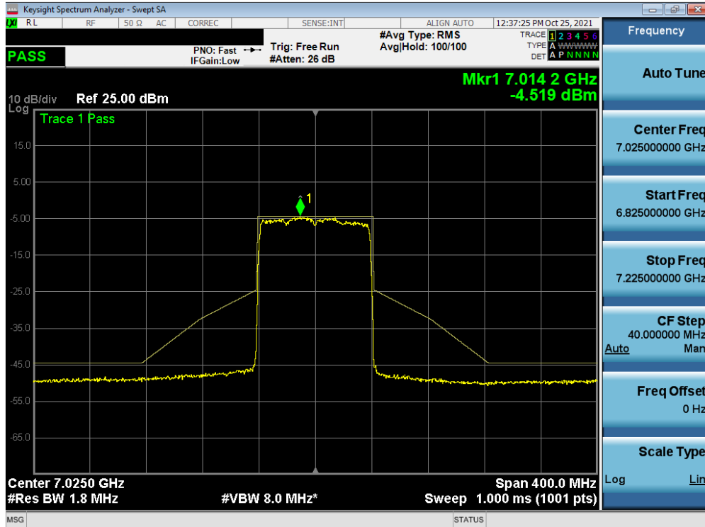
Plot 7-452. In-Band Emission Plot MIMO ANT2 (80MHz BW 802.11ax (Full Tones) (UNII Band 8) – Ch. 215)
