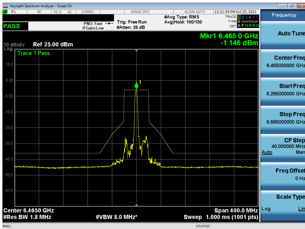
Plot 7-402. In-Band Emission Plot MIMO ANT2 (80MHz BW 802.11ax (26 Tones) (UNII Band 6) – Ch. 103)
