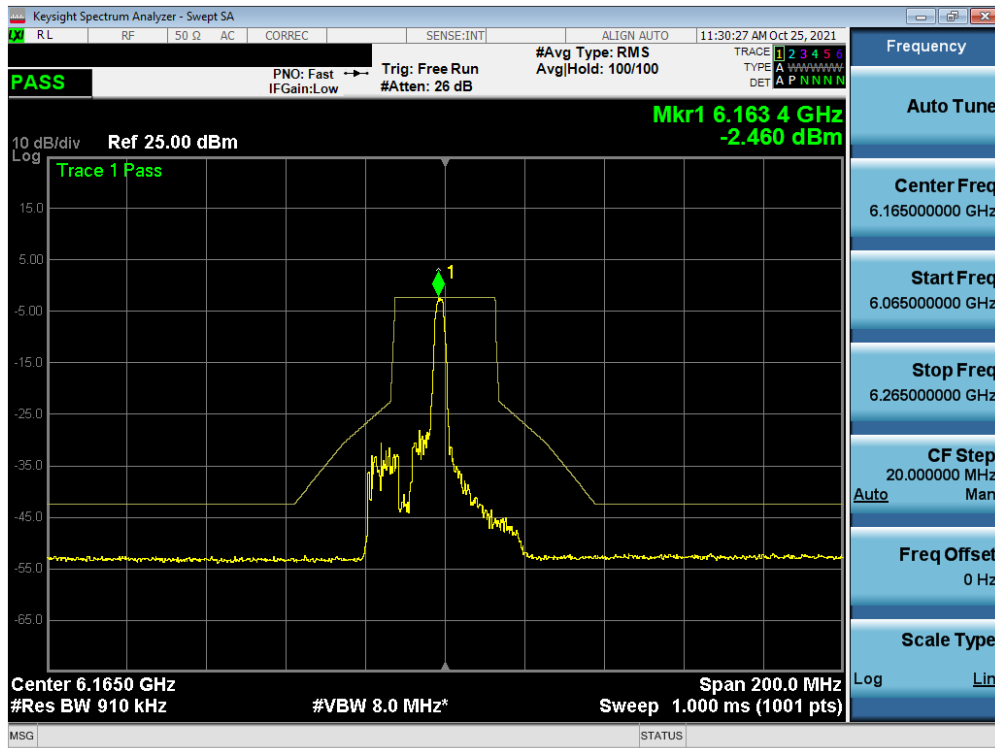
Plot 7-391. In-Band Emission Plot MIMO ANT2 (40MHz BW 802.11ax (26 Tones) (UNII Band 5) – Ch. 43)
