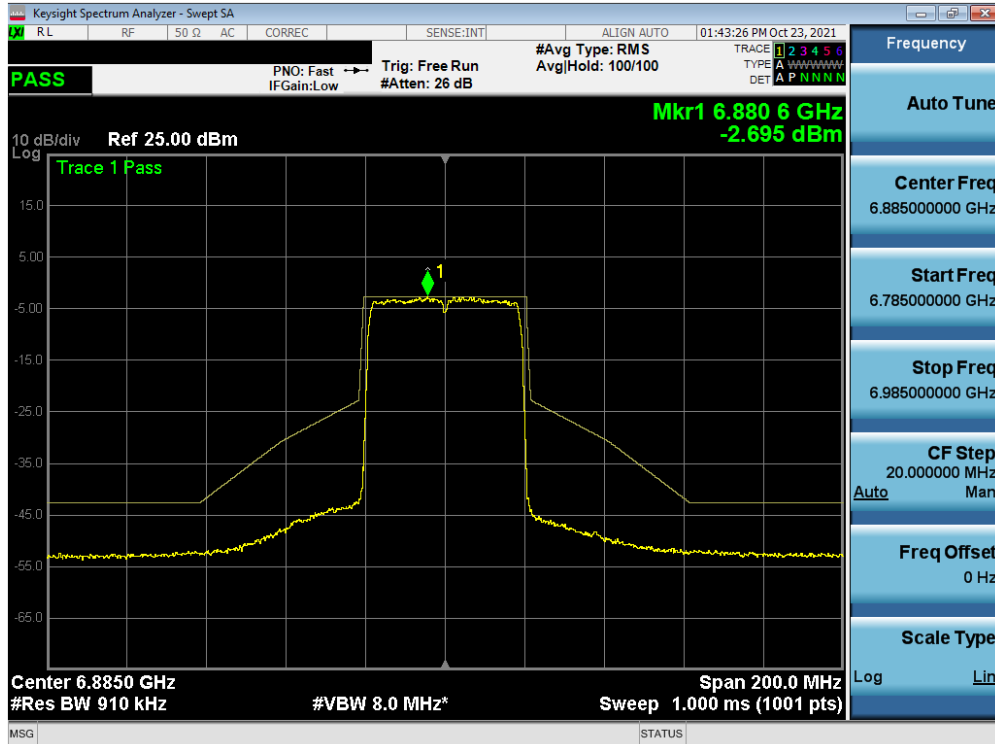
Plot 7-382. In-Band Emission Plot MIMO ANT1 (40MHz BW 802.11ax (Full Tones) (UNII Band 8) – Ch. 187)
