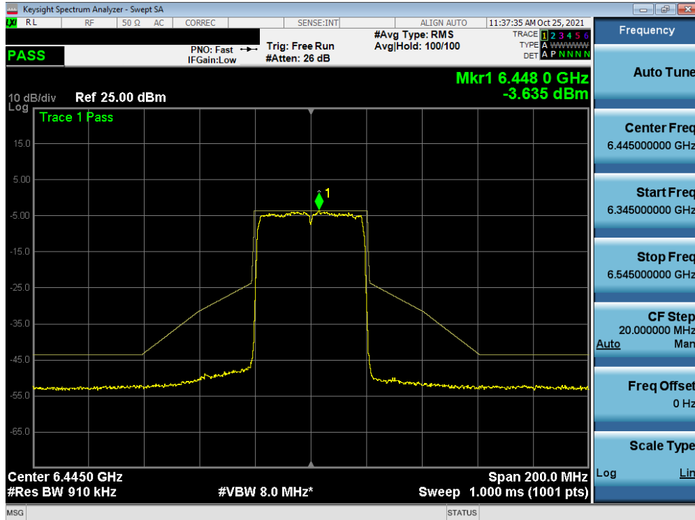
Plot 7-432. In-Band Emission Plot MIMO ANT2 (40MHz BW 802.11ax (Full Tones) (UNII Band 6) – Ch. 99)
