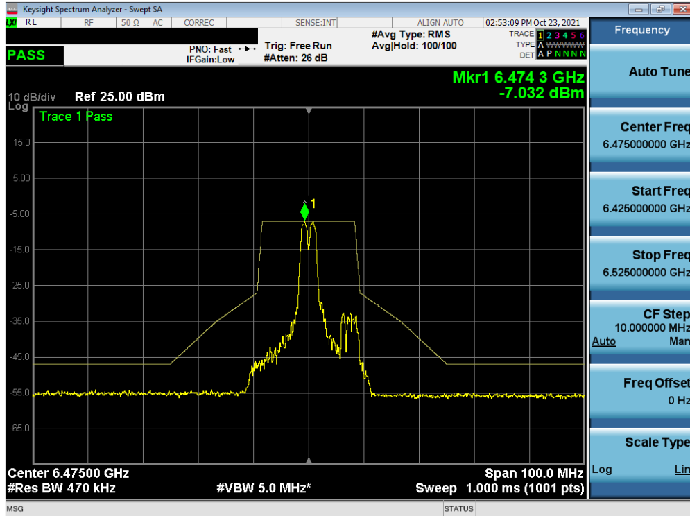
Plot 7-397. In-Band Emission Plot MIMO ANT2 (20MHz BW 802.11ax (26 Tones) (UNII Band 6) – Ch. 105)
