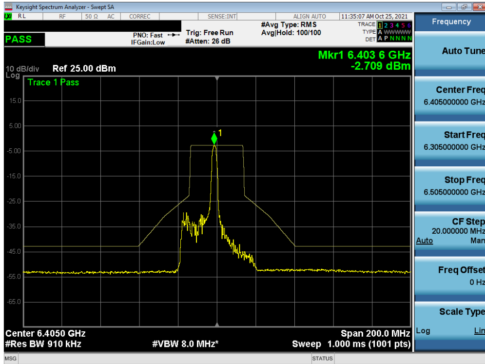
Plot 7-392. In-Band Emission Plot MIMO ANT2 (40MHz BW 802.11ax (26 Tones) (UNII Band 5) – Ch. 91)
