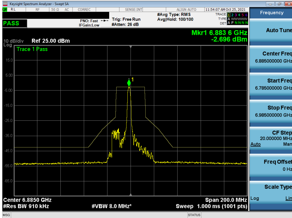
Plot 7-415. In-Band Emission Plot MIMO ANT2 (40MHz BW 802.11ax (26 Tones) (UNII Band 8) – Ch. 187)
