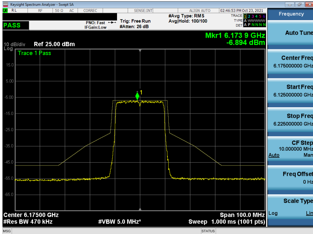
Plot 7-421. In-Band Emission Plot MIMO ANT2 (20MHz BW 802.11ax (Full Tones) (UNII Band 5) – Ch. 45)
