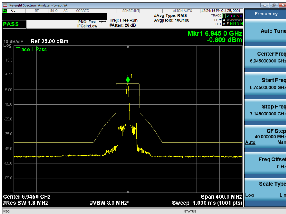
Plot 7-418. In-Band Emission Plot MIMO ANT2 (80MHz BW 802.11ax (26 Tones) (UNII Band 8) – Ch. 199)
