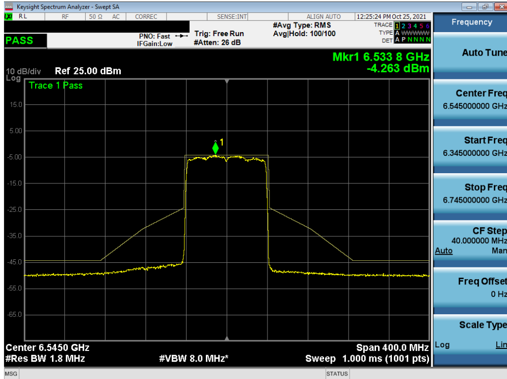
Plot 7-442. In-Band Emission Plot MIMO ANT2 (80MHz BW 802.11ax (Full Tones) (UNII Band 7) – Ch. 119)
