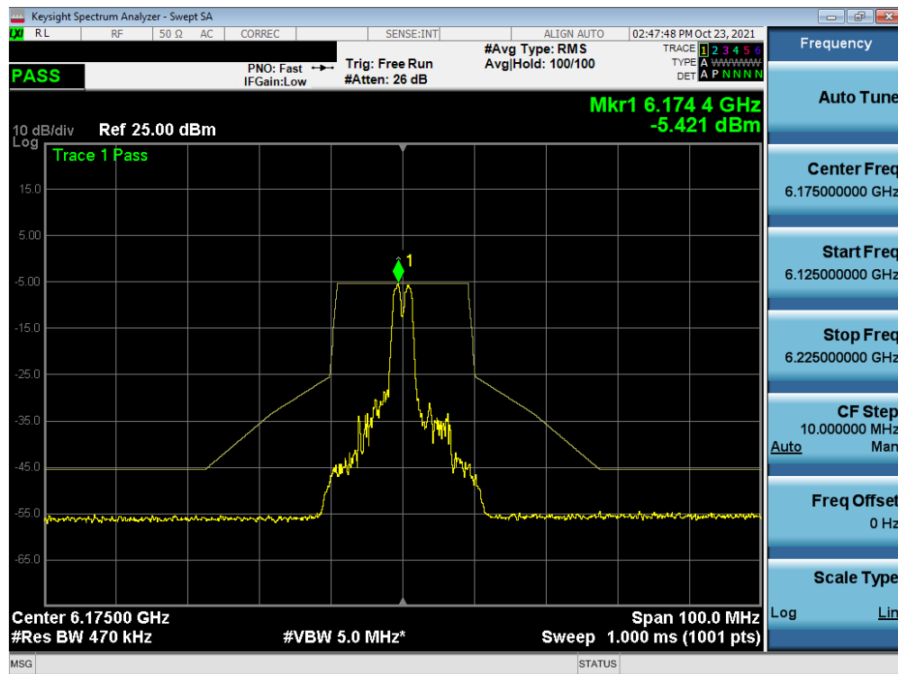
Plot 7-388. In-Band Emission Plot MIMO ANT2 (20MHz BW 802.11ax (26 Tones) (UNII Band 5) – Ch. 45)
