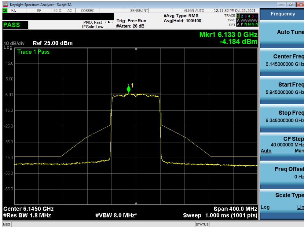
Plot 7-427. In-Band Emission Plot MIMO ANT2 (80MHz BW 802.11ax (Full Tones) (UNII Band 5) – Ch. 39)
