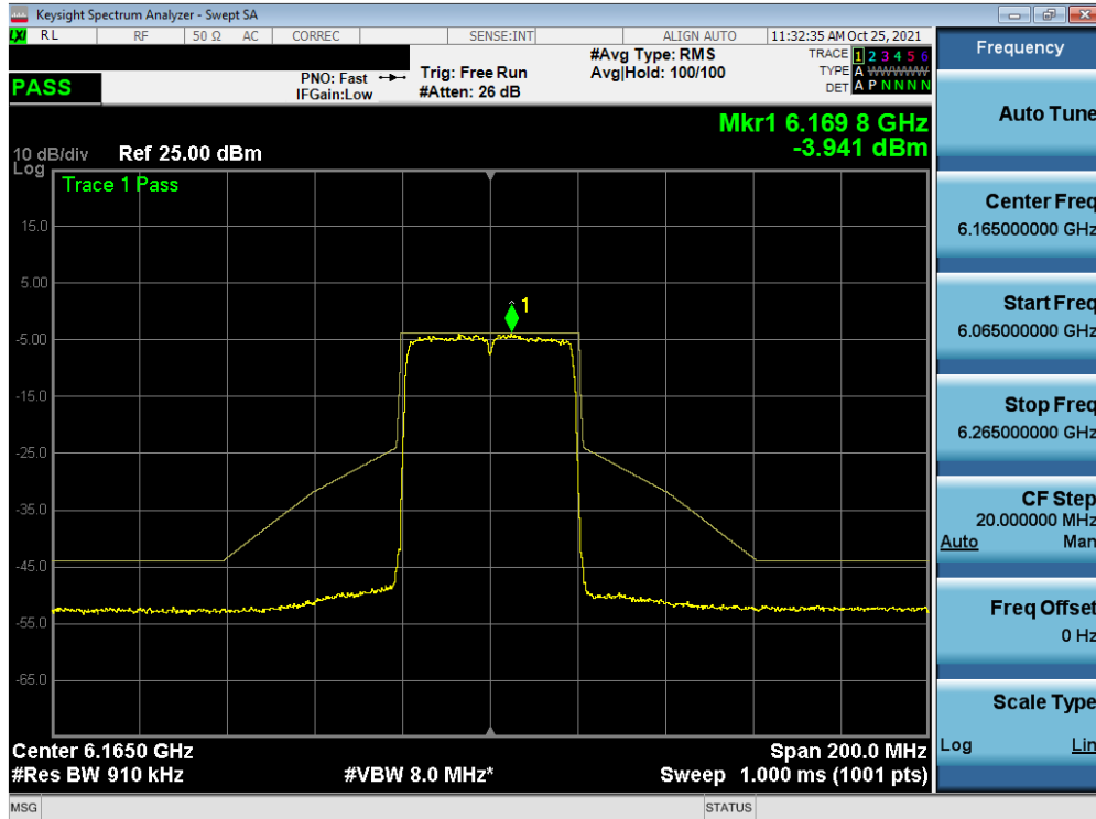
Plot 7-424. In-Band Emission Plot MIMO ANT2 (40MHz BW 802.11ax (Full Tones) (UNII Band 5) – Ch. 43)
