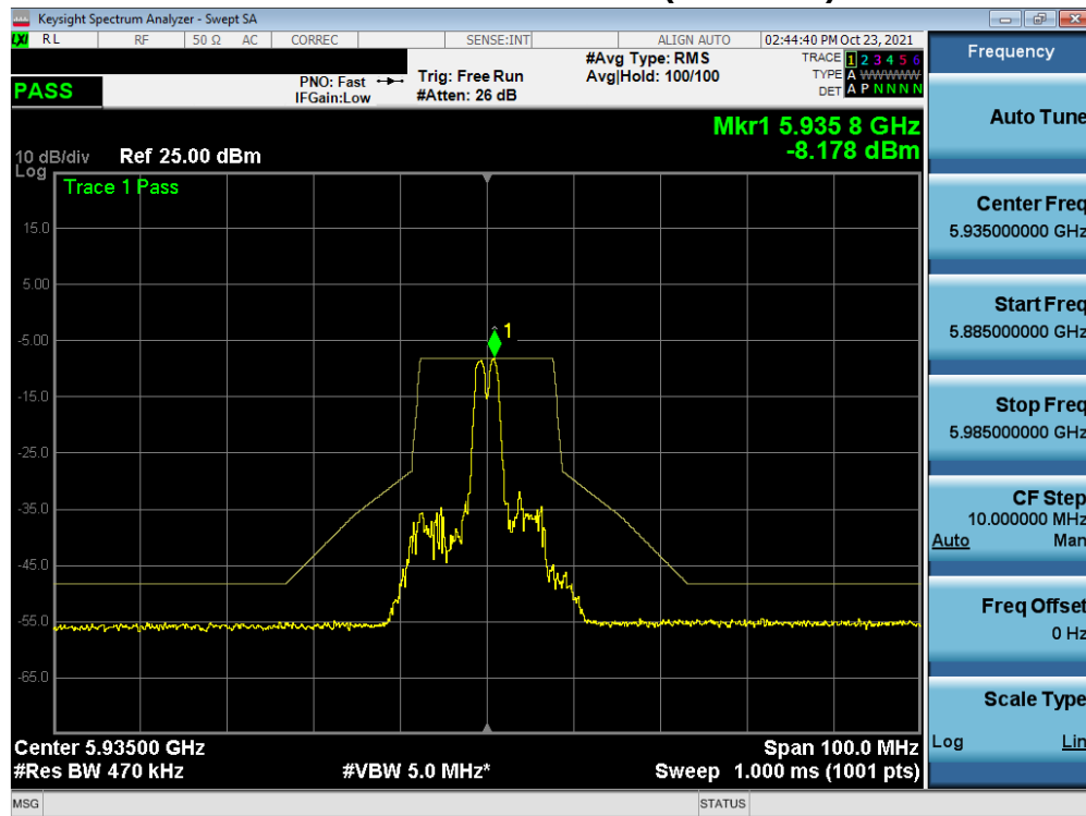
Plot 7-387. In-Band Emission Plot MIMO ANT2 (20MHz BW 802.11ax (26 Tones) UNII Band 5) – Ch. 2)
