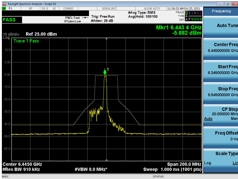
Plot 7-399. In-Band Emission Plot MIMO ANT2 (40MHz BW 802.11ax (26 Tones) (UNII Band 6) – Ch. 99)
