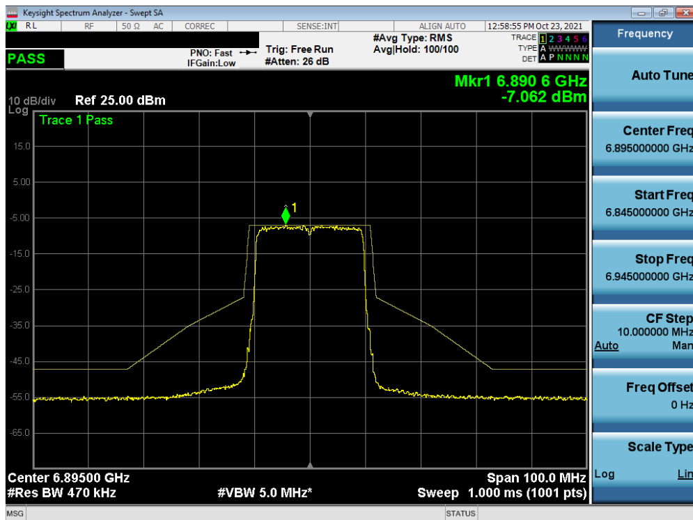
Plot 7-379. In-Band Emission Plot MIMO ANT1 (20MHz BW 802.11ax (Full Tones) (UNII Band 8) – Ch. 189)
