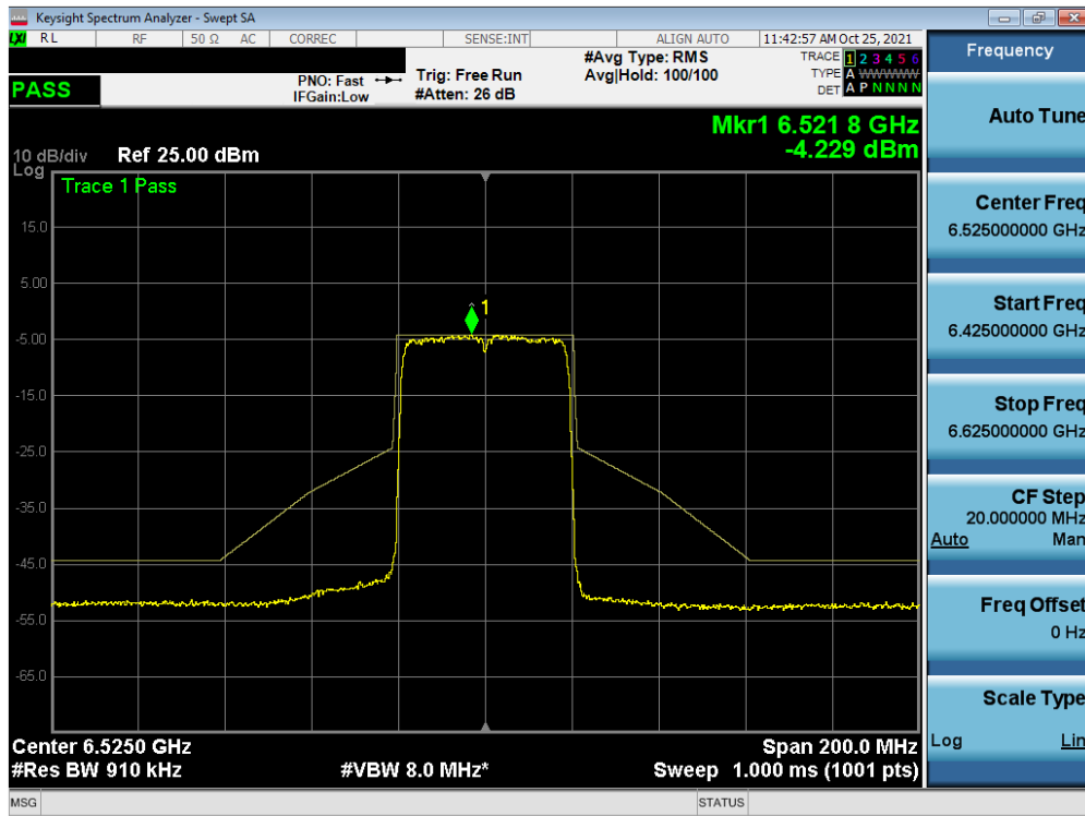
Plot 7-434. In-Band Emission Plot MIMO ANT2 (40MHz BW 802.11ax (Full Tones) (UNII Band 6) – Ch. 115)
