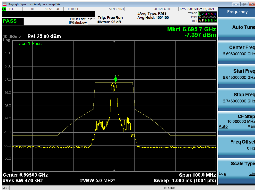
Plot 7-404. In-Band Emission Plot MIMO ANT2 (20MHz BW 802.11ax (26 Tones) (UNII Band 7) – Ch. 149)
