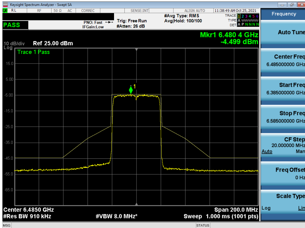
Plot 7-433. In-Band Emission Plot MIMO ANT2 (40MHz BW 802.11ax (Full Tones) (UNII Band 6) – Ch. 107)
