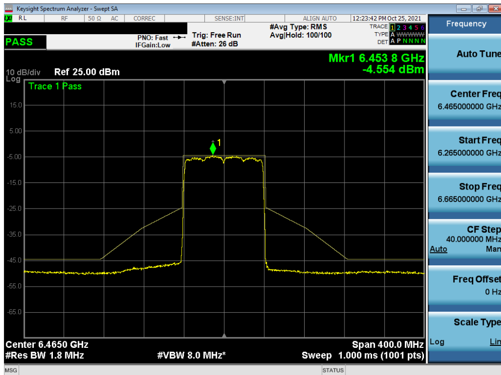
Plot 7-435. In-Band Emission Plot MIMO ANT2 (80MHz BW 802.11ax (Full Tones) (UNII Band 6) – Ch. 103)
