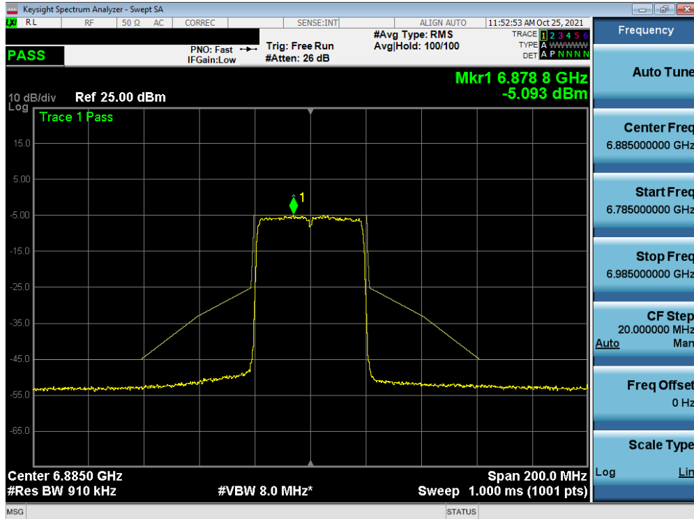
Plot 7-448. In-Band Emission Plot MIMO ANT2 (40MHz BW 802.11ax (Full Tones) (UNII Band 8) – Ch. 187)
