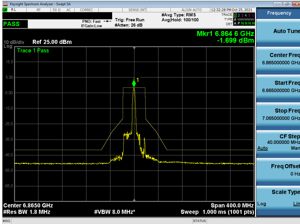
Plot 7-411. In-Band Emission Plot MIMO ANT2 (80MHz BW 802.11ax (26 Tones) (UNII Band 7) – Ch. 183)
