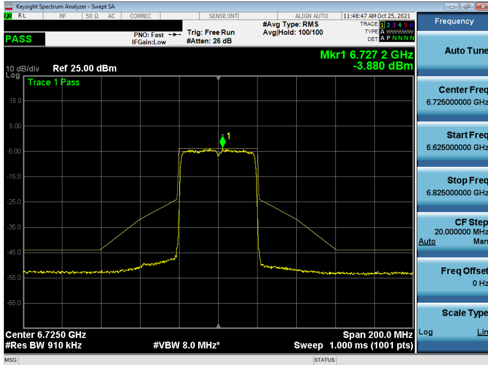
Plot 7-440. In-Band Emission Plot MIMO ANT2 (40MHz BW 802.11ax (Full Tones) (UNII Band 7) – Ch. 155)
