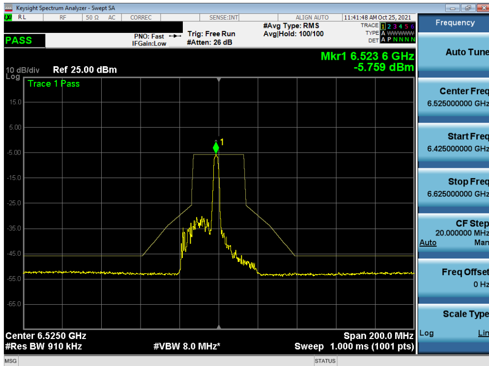
Plot 7-401. In-Band Emission Plot MIMO ANT2 (40MHz BW 802.11ax (26 Tones) (UNII Band 6) – Ch. 115)
