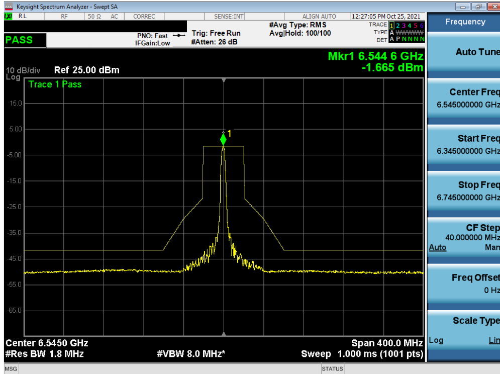
Plot 7-409. In-Band Emission Plot MIMO ANT2 (80MHz BW 802.11ax (26 Tones) (UNII Band 7) – Ch. 119)
