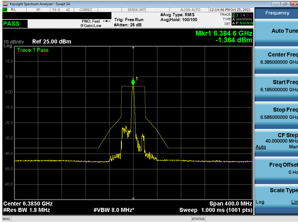
Plot 7-395. In-Band Emission Plot MIMO ANT2 (80MHz BW 802.11ax (26 Tones) (UNII Band 5) – Ch. 87)
