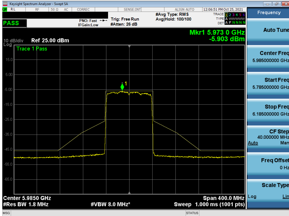
Plot 7-426. In-Band Emission Plot MIMO ANT2 (80MHz BW 802.11ax (Full Tones) (UNII Band 5) – Ch. 7)
