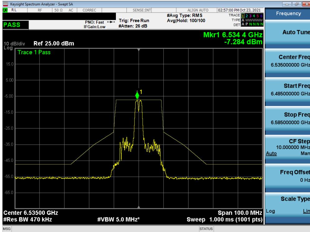
Plot 7-403. In-Band Emission Plot MIMO ANT2 (20MHz BW 802.11ax (26 Tones) (UNII Band 7) – Ch. 117)
