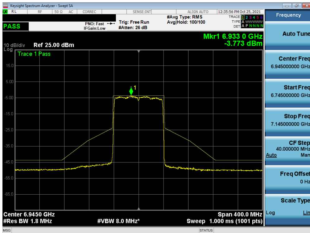
Plot 7-451. In-Band Emission Plot MIMO ANT2 (80MHz BW 802.11ax (Full Tones) (UNII Band 8) – Ch. 199)
