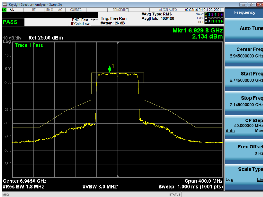
Plot 7-385. In-Band Emission Plot MIMO ANT1 (80MHz BW 802.11ax (Full Tones) (UNII Band 8) – Ch. 199)
