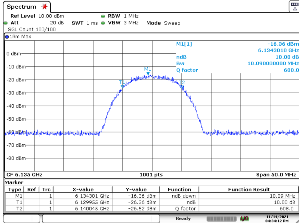
Plot 7-453. AWGN Sample Signal
