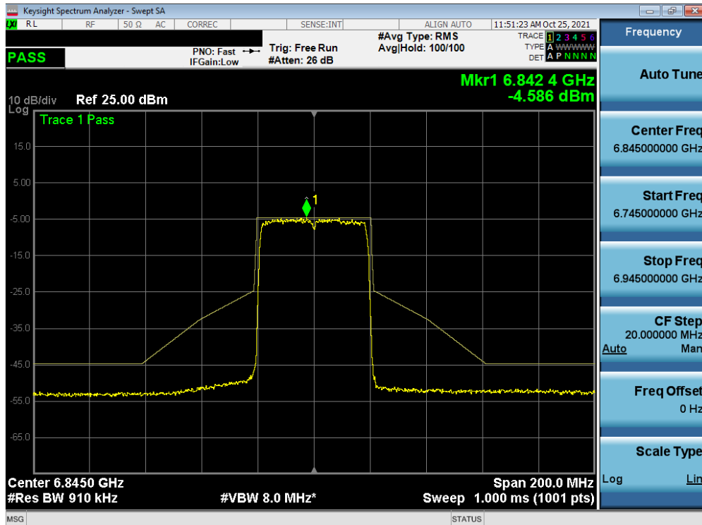
Plot 7-441. In-Band Emission Plot MIMO ANT2 (40MHz BW 802.11ax (Full Tones) (UNII Band 7) – Ch. 179)
