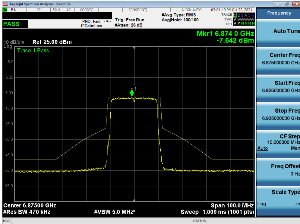
Plot 7-438. In-Band Emission Plot MIMO ANT2 (20MHz BW 802.11ax (Full Tones) (UNII Band 7) – Ch. 185)
