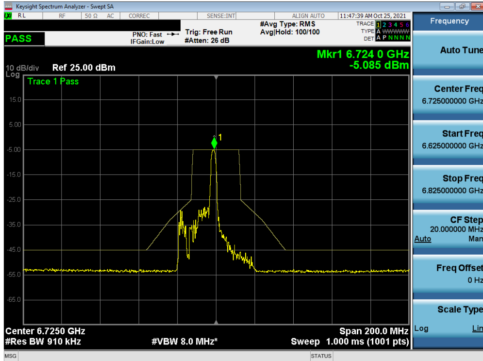
Plot 7-407. In-Band Emission Plot MIMO ANT2 (40MHz BW 802.11ax (26 Tones) (UNII Band 7) – Ch. 155)
