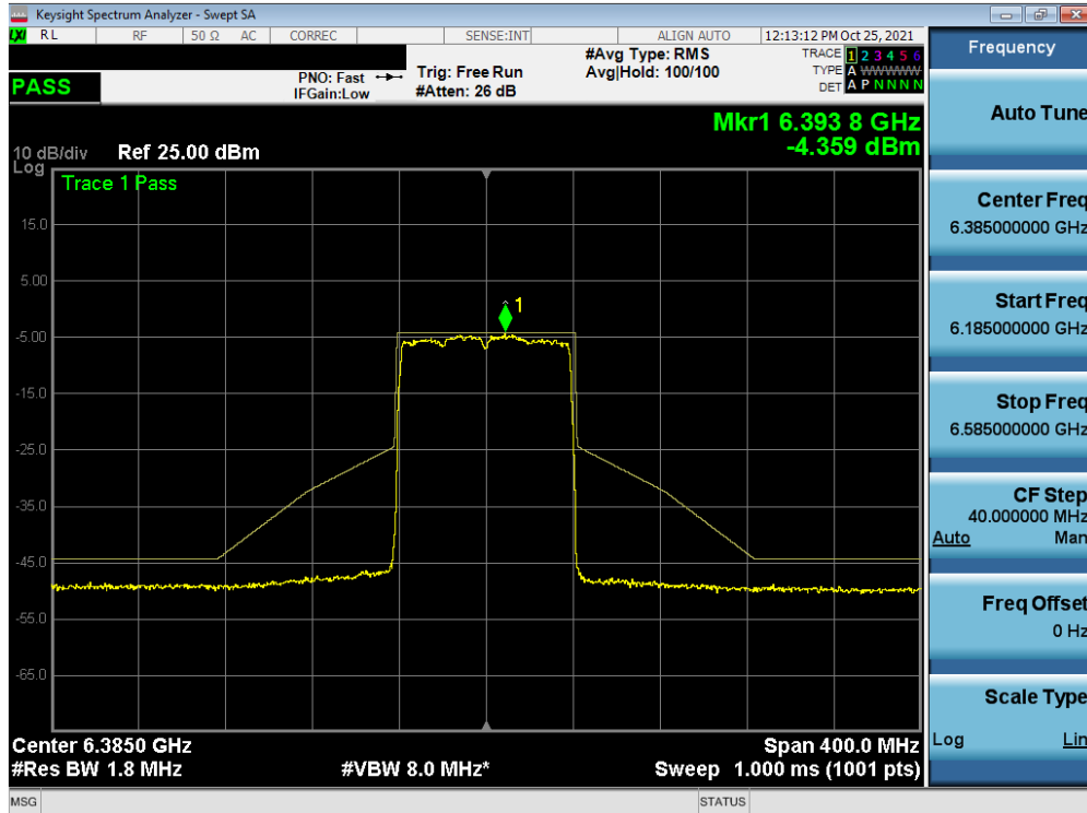
Plot 7-428. In-Band Emission Plot MIMO ANT2 (80MHz BW 802.11ax (Full Tones) (UNII Band 5) – Ch. 87)
