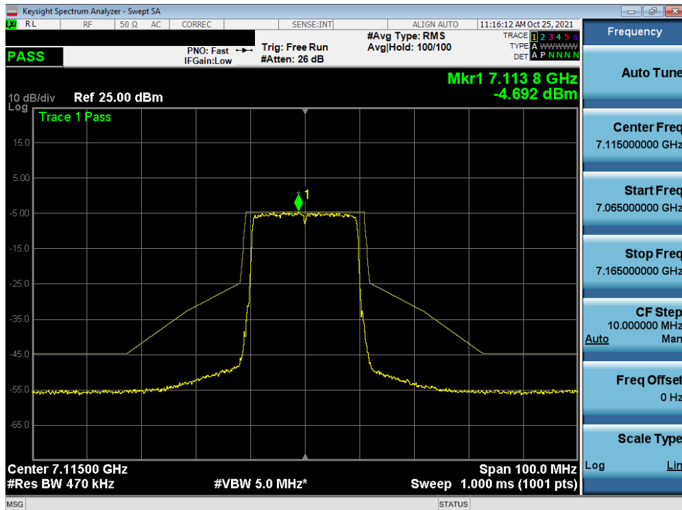
Plot 7-447. In-Band Emission Plot MIMO ANT2 (20MHz BW 802.11ax (Full Tones) (UNII Band 8) – Ch. 233)
