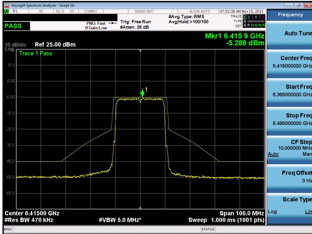
Plot 7-422. In-Band Emission Plot MIMO ANT2 (20MHz BW 802.11ax (Full Tones) UNII Band 5) – Ch. 93)
