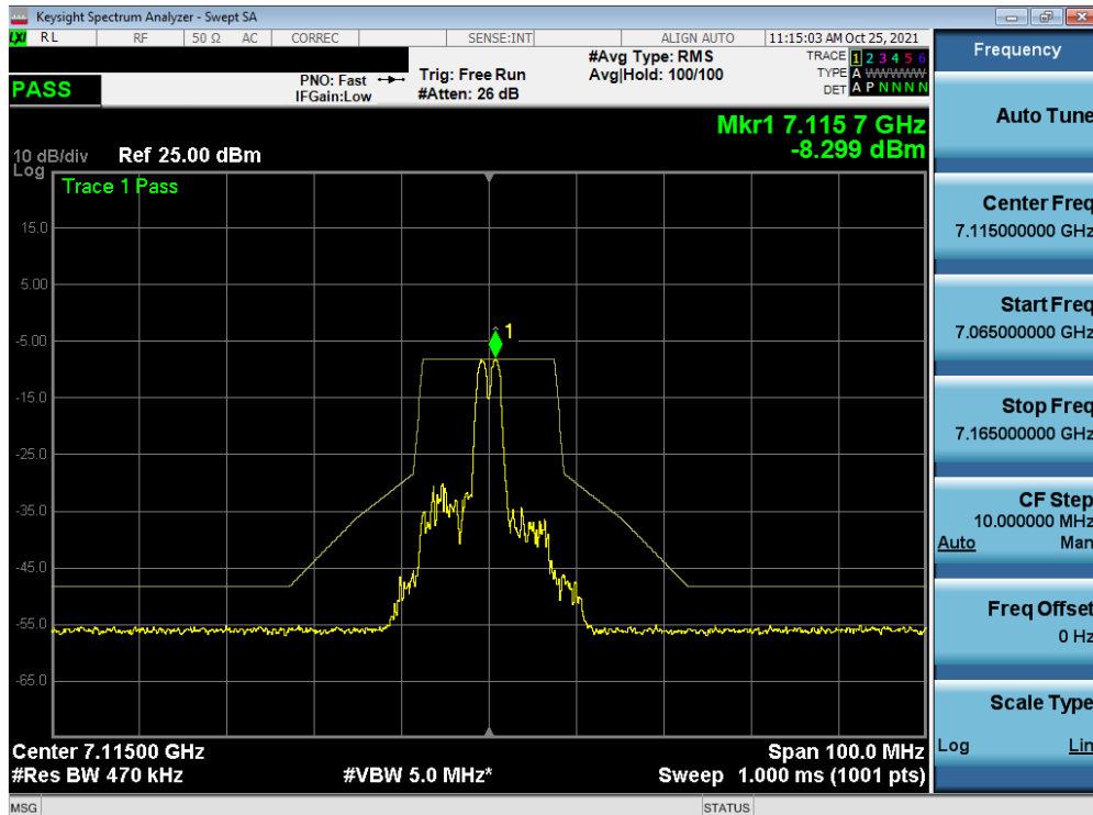
Plot 7-414. In-Band Emission Plot MIMO ANT2 (20MHz BW 802.11ax (26 Tones) (UNII Band 8) – Ch. 233)
