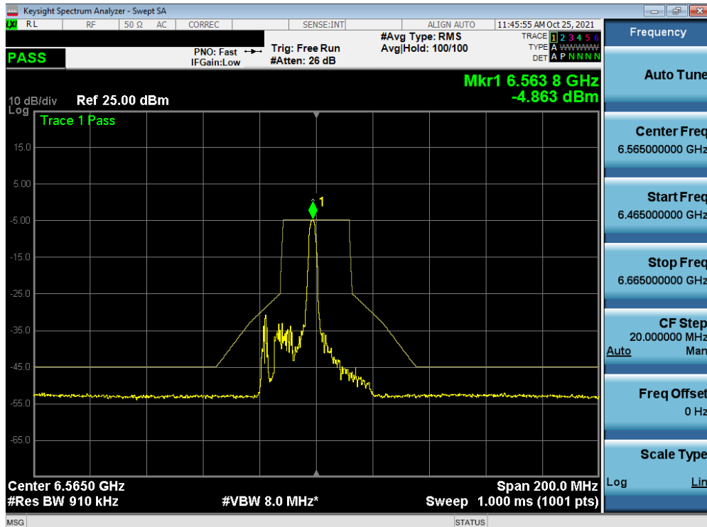
Plot 7-406. In-Band Emission Plot MIMO ANT2 (40MHz BW 802.11ax (26 Tones) (UNII Band 7) – Ch. 123)
