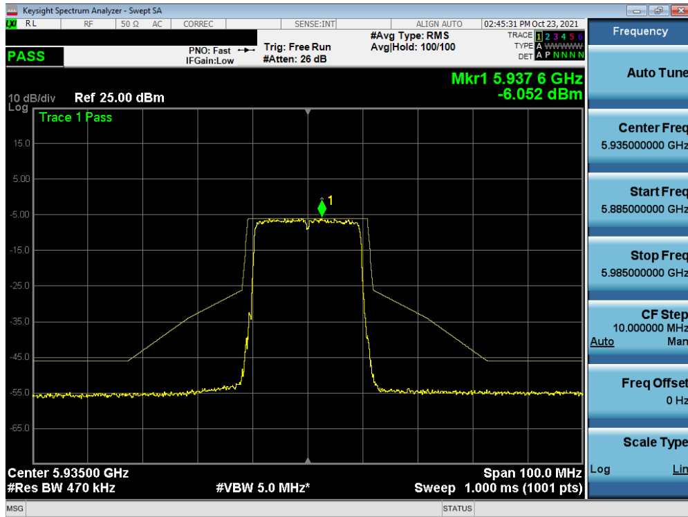
Plot 7-420. In-Band Emission Plot MIMO ANT2 (20MHz BW 802.11ax (Full Tones) UNII Band 5) – Ch. 2)
