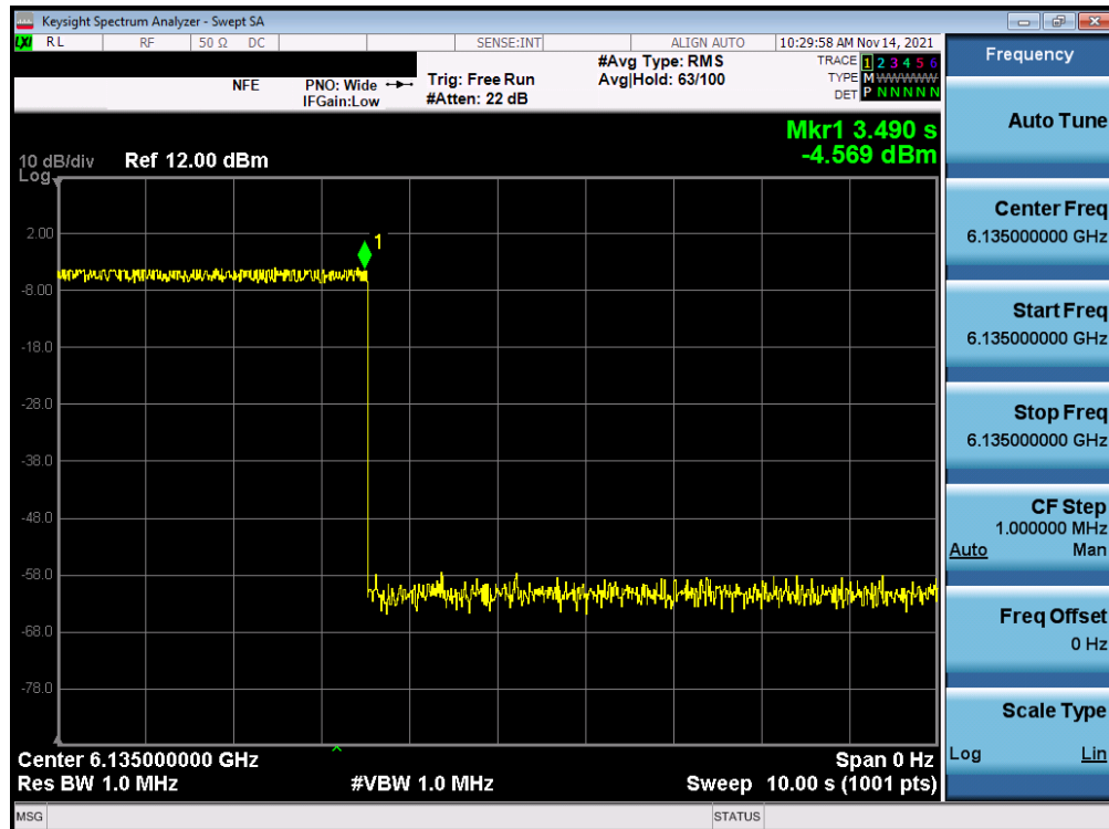
Plot 7-454. Contention Based Protocol Timing Plot
