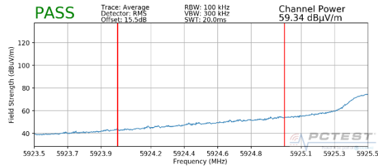
Plot 7-459. Radiated Lower Band Edge Plot MIMO (Average – UNII Band 5)
