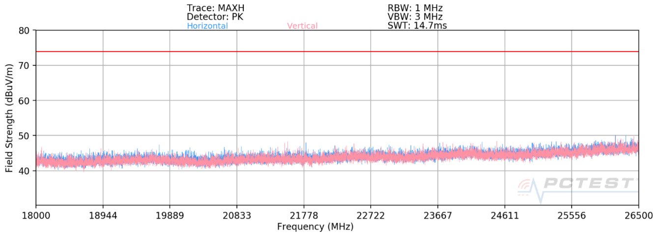
Plot 7-457. Radiated Spurious Plot above 18GHz - 26.5GHz MIMO (802.11ax – Partial Tones)
