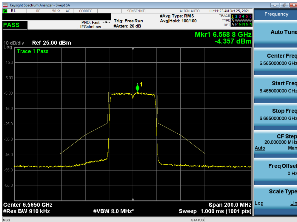
Plot 7-439. In-Band Emission Plot MIMO ANT2 (40MHz BW 802.11ax (Full Tones) (UNII Band 7) – Ch. 123)
