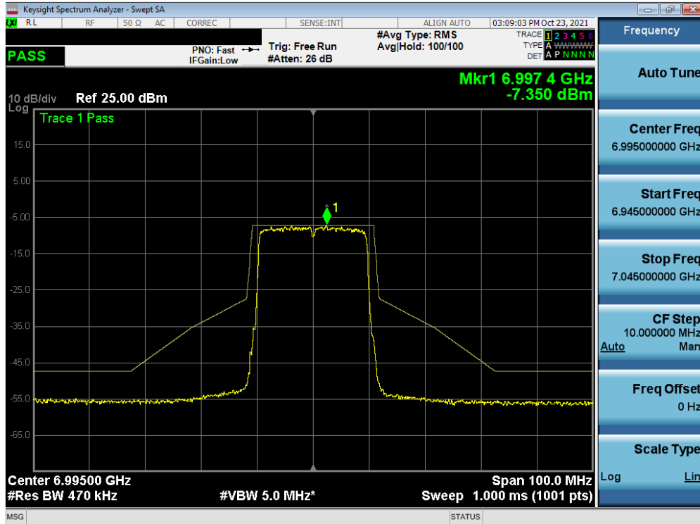
Plot 7-446. In-Band Emission Plot MIMO ANT2 (20MHz BW 802.11ax (Full Tones) (UNII Band 8) – Ch. 209)
