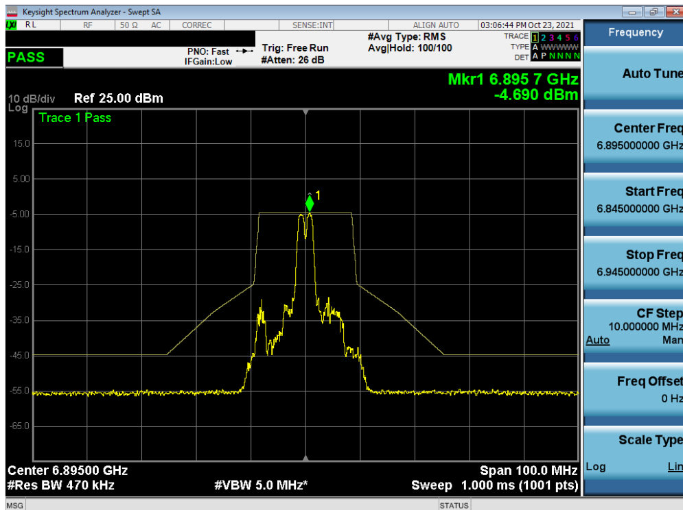
Plot 7-412. In-Band Emission Plot MIMO ANT2 (20MHz BW 802.11ax (26 Tones) (UNII Band 8) – Ch. 189)
