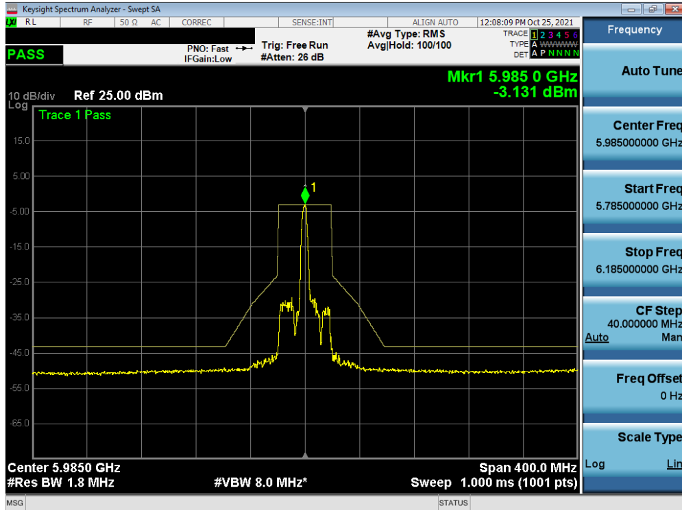
Plot 7-393. In-Band Emission Plot MIMO ANT2 (80MHz BW 802.11ax (26 Tones) (UNII Band 5) – Ch. 7)
