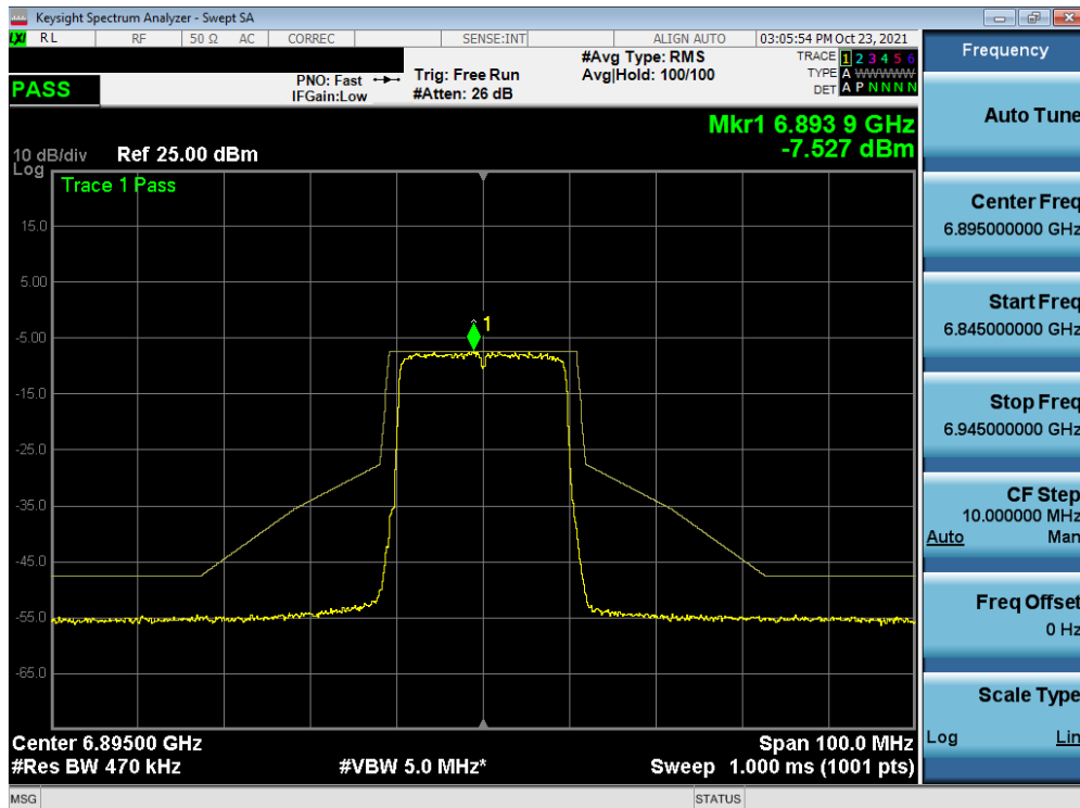
Plot 7-445. In-Band Emission Plot MIMO ANT2 (20MHz BW 802.11ax (Full Tones) (UNII Band 8) – Ch. 189)
