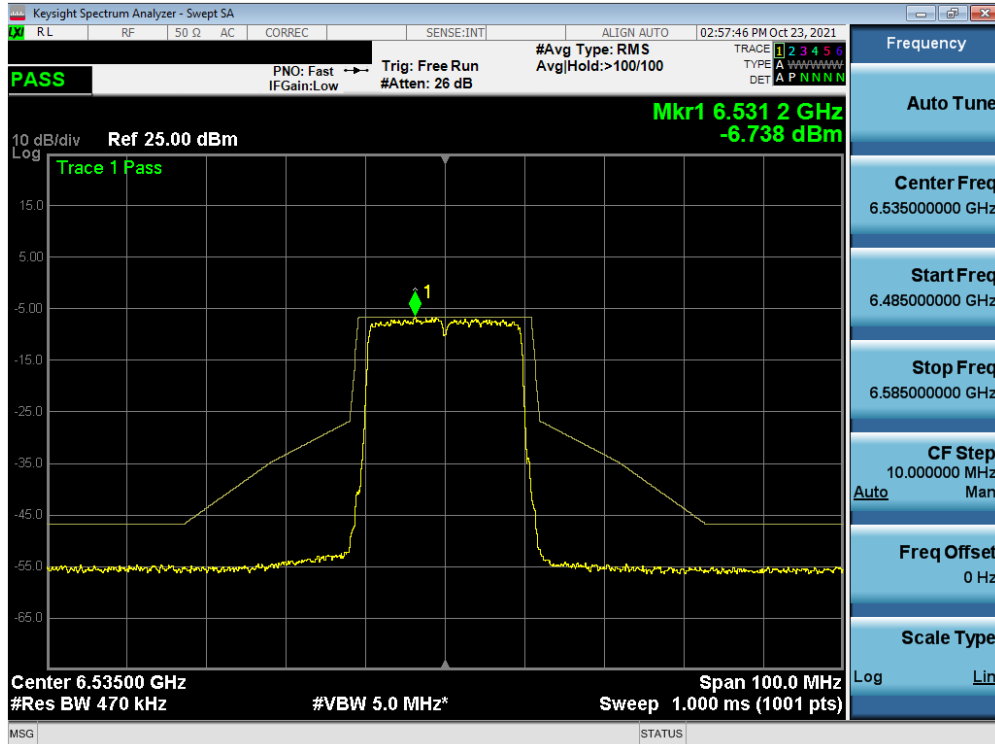
Plot 7-436. In-Band Emission Plot MIMO ANT2 (20MHz BW 802.11ax (Full Tones) (UNII Band 7) – Ch. 117)
