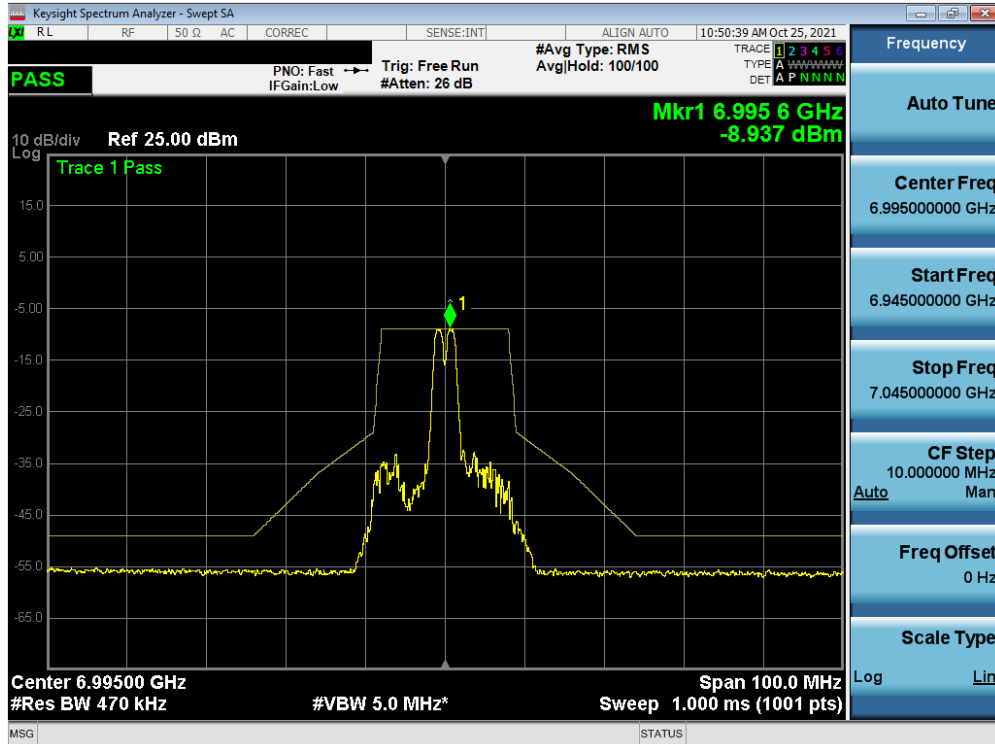
Plot 7-413. In-Band Emission Plot MIMO ANT2 (20MHz BW 802.11ax (26 Tones) (UNII Band 8) – Ch. 209)
