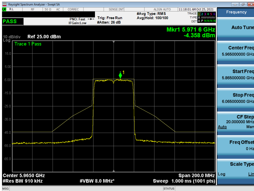
Plot 7-423. In-Band Emission Plot MIMO ANT2 (40MHz BW 802.11ax (Full Tones) UNII Band 5) – Ch. 3)
