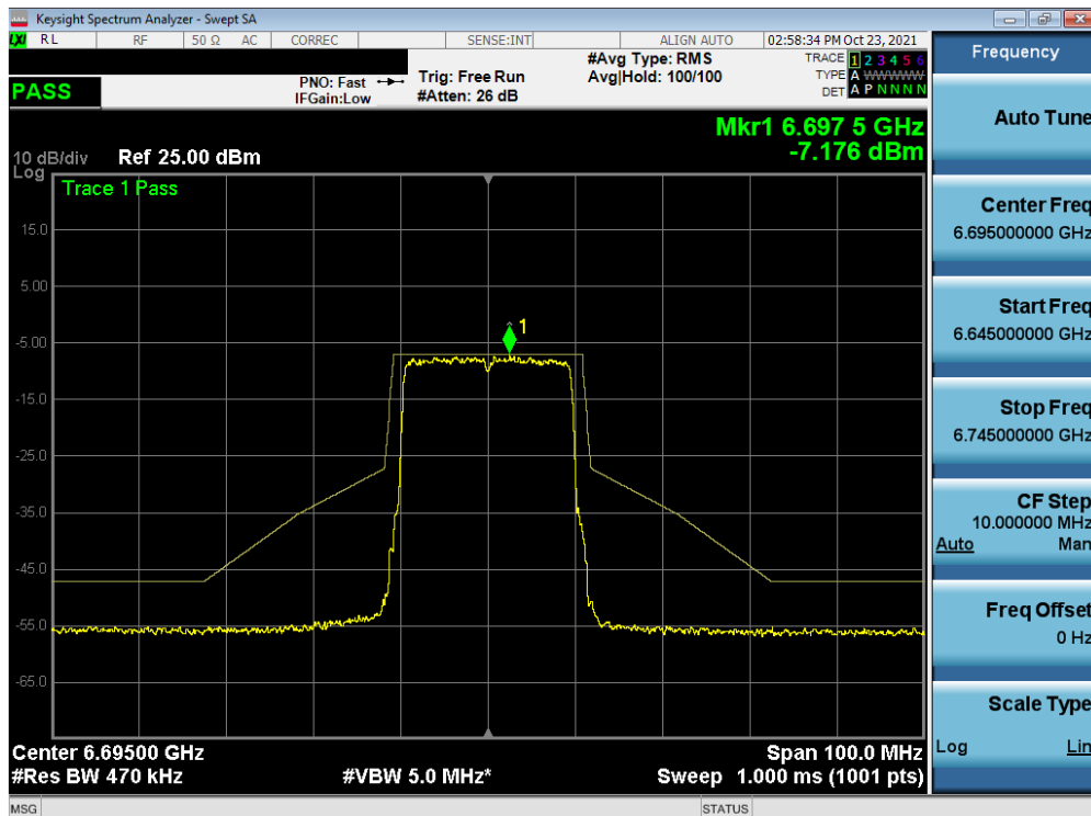
Plot 7-437. In-Band Emission Plot MIMO ANT2 (20MHz BW 802.11ax (Full Tones) (UNII Band 7) – Ch. 149)
