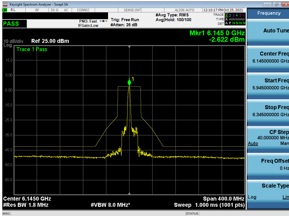
Plot 7-394. In-Band Emission Plot MIMO ANT2 (80MHz BW 802.11ax (26 Tones) (UNII Band 5) – Ch. 39)
