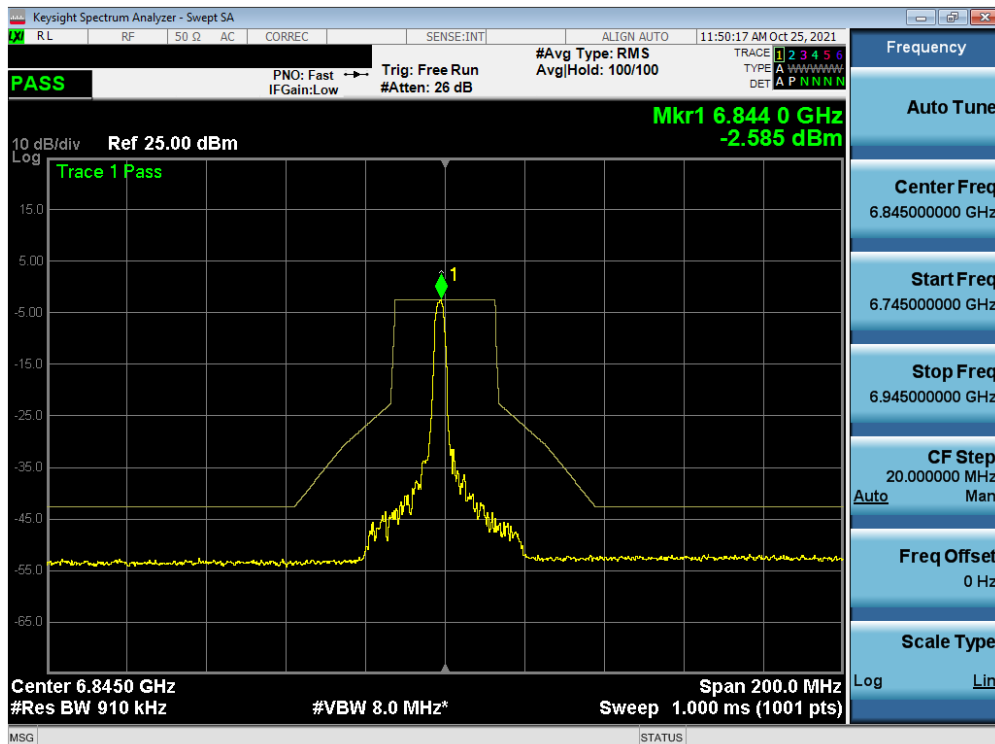
Plot 7-408. In-Band Emission Plot MIMO ANT2 (40MHz BW 802.11ax (26 Tones) (UNII Band 7) – Ch. 179)
