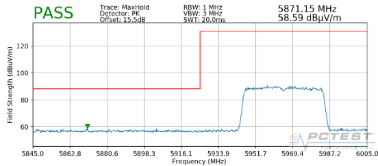
Plot 7-463. Radiated Lower Band Edge Plot MIMO (Peak – UNII Band 5)
