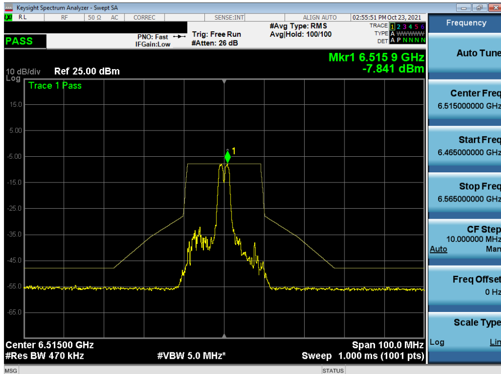
Plot 7-398. In-Band Emission Plot MIMO ANT2 (20MHz BW 802.11ax (26 Tones) (UNII Band 6) – Ch. 113)
