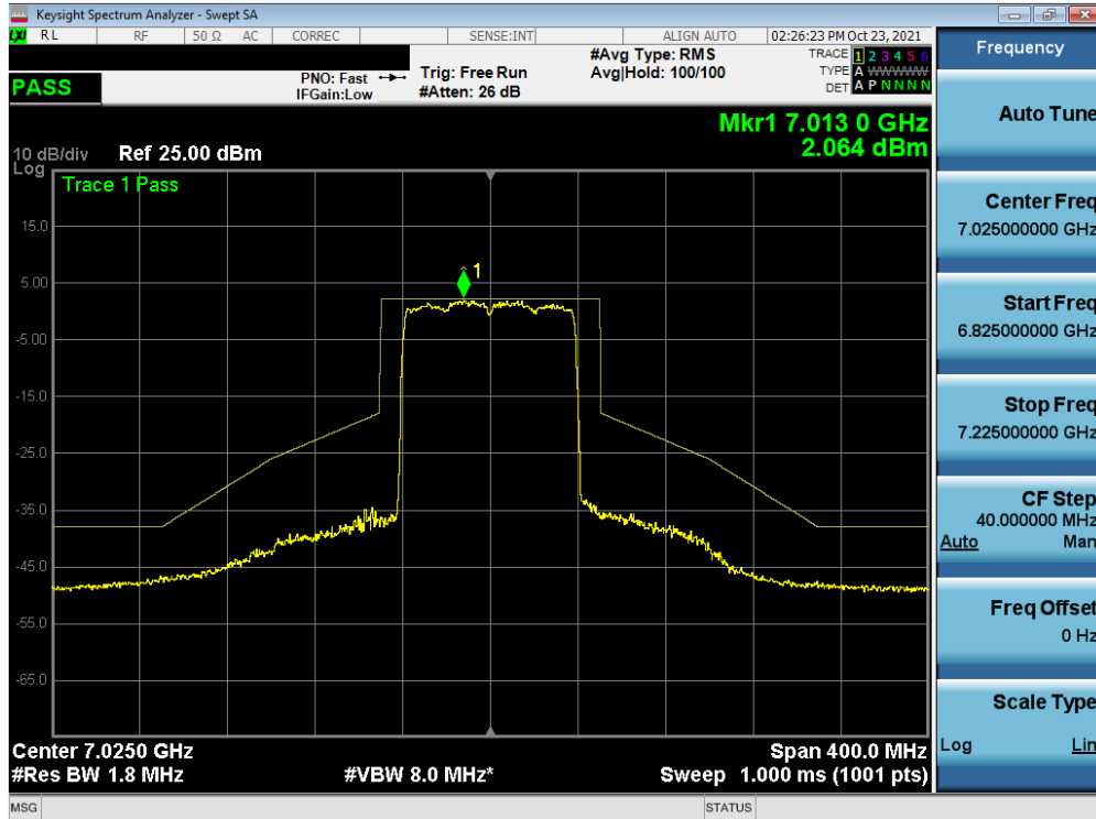
Plot 7-386. In-Band Emission Plot MIMO ANT1 (80MHz BW 802.11ax (Full Tones) (UNII Band 8) – Ch. 215)
