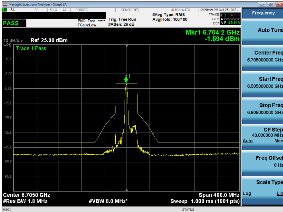
Plot 7-410. In-Band Emission Plot MIMO ANT2 (80MHz BW 802.11ax (26 Tones) (UNII Band 7) – Ch. 151)
