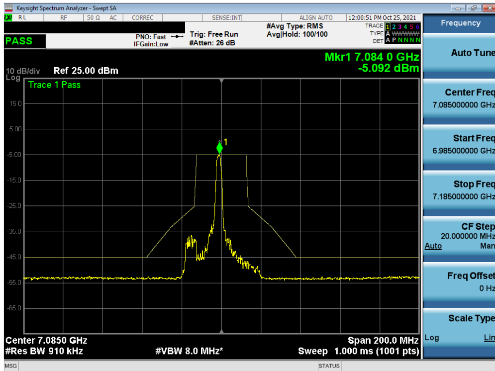
Plot 7-417. In-Band Emission Plot MIMO ANT2 (40MHz BW 802.11ax (26 Tones) (UNII Band 8) – Ch. 227)
