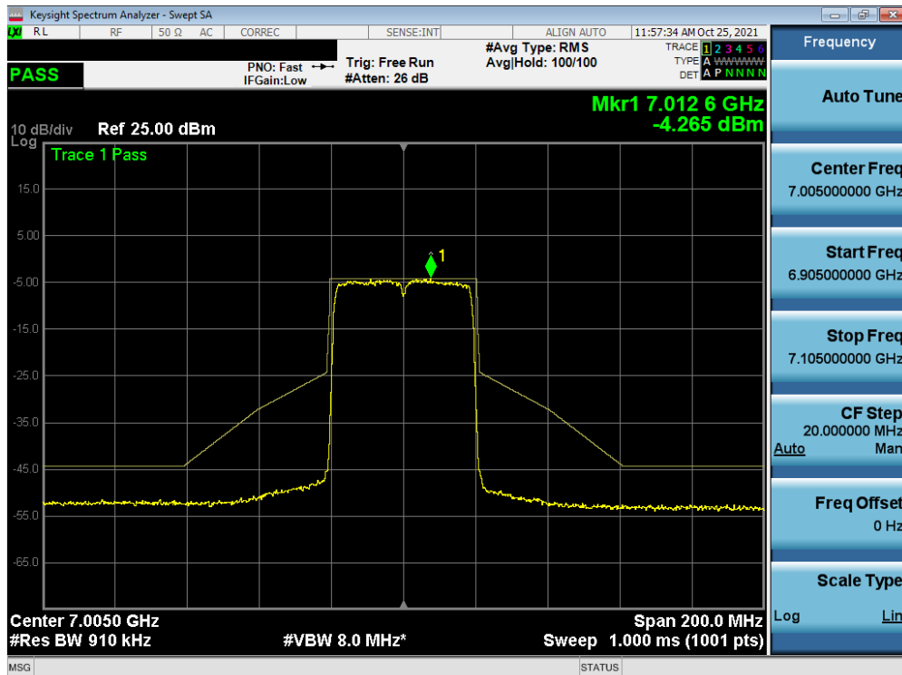
Plot 7-449. In-Band Emission Plot MIMO ANT2 (40MHz BW 802.11ax (Full Tones) (UNII Band 8) – Ch. 211)
