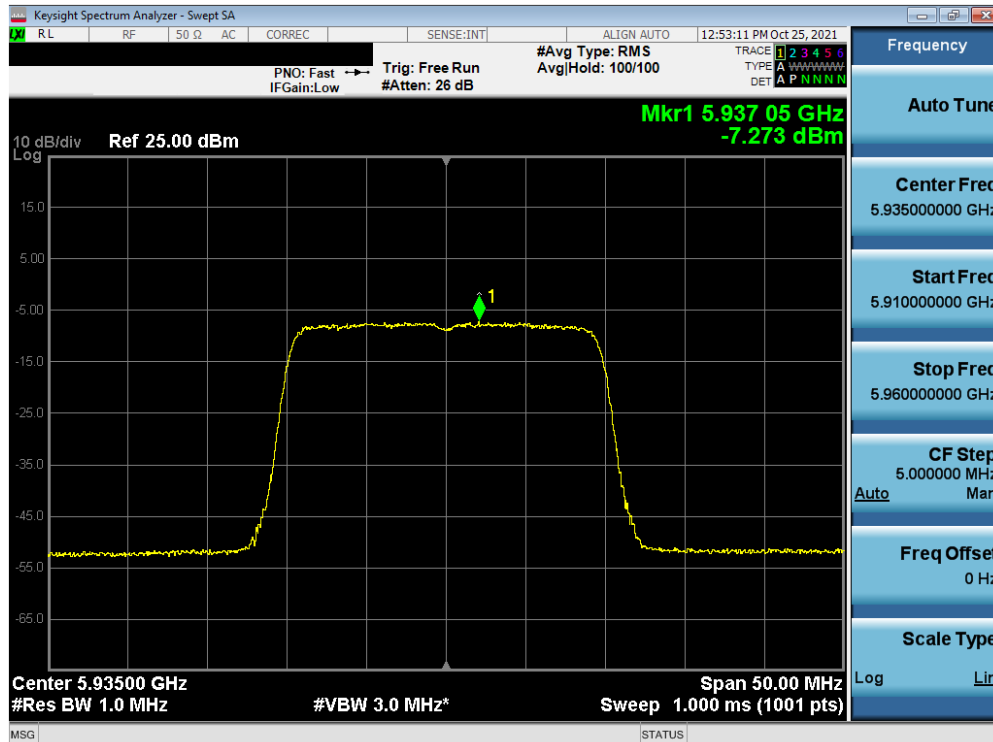
Plot 7-108. Power Spectral Density Measurement Plot MIMO ANT1 (20MHz 802.11a (UNII Band 5) – Ch. 2)
