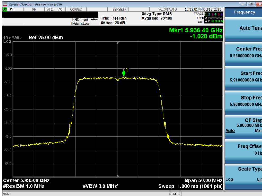
Plot 7-160. Power Spectral Density Measurement Plot MIMO ANT2 (20MHz 802.11a (UNII Band 5) – Ch. 2)
