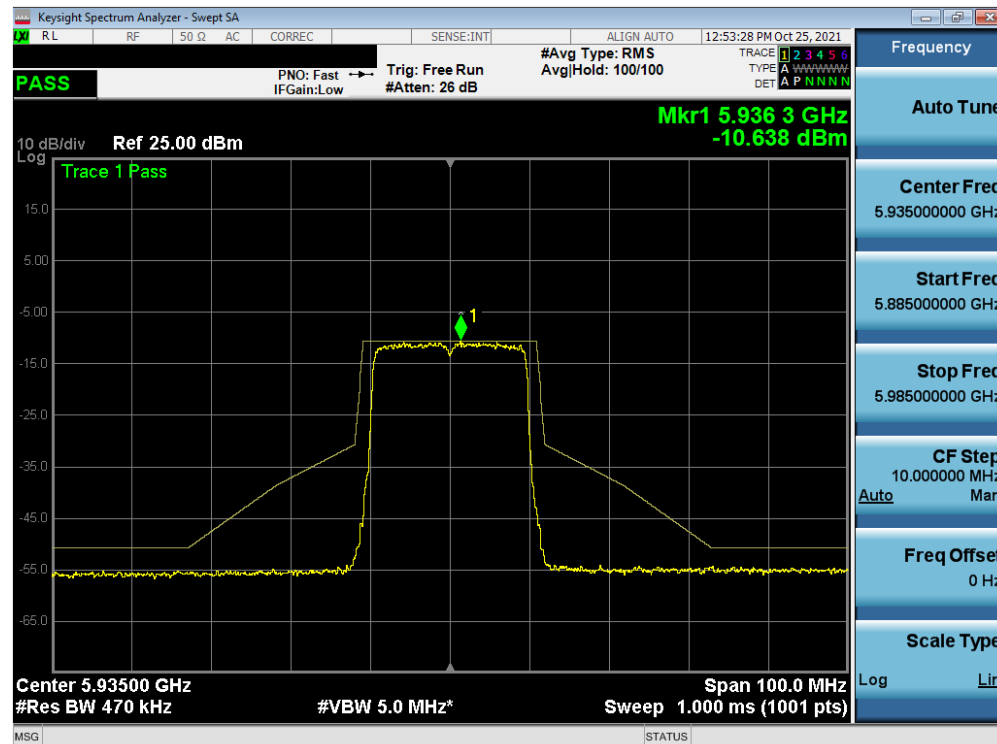
Plot 7-212. In-Band Emission Measurement Plot MIMO ANT1 (20MHz 802.11a (UNII Band 5) – Ch. 2)
