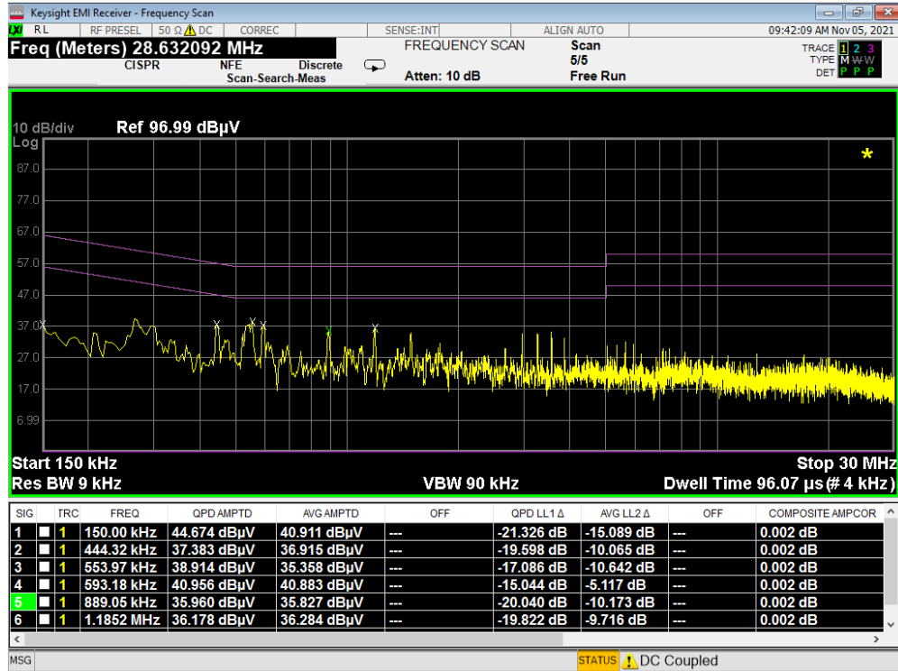
Plot 7-340. Line Conducted Plot with 802.11a UNII Band 5 (L1) with WCP
