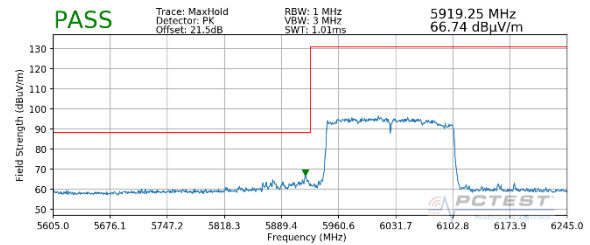
Plot 7-328. Radiated Lower Band Edge Plot MIMO (Peak – UNII Band 5)
