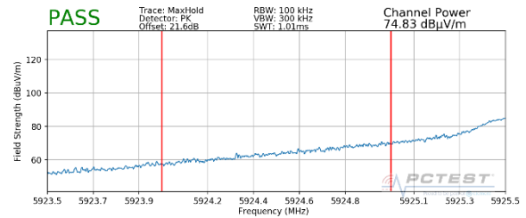
Plot 7-320. Radiated Lower Band Edge Plot MIMO (Peak – UNII Band 5)
