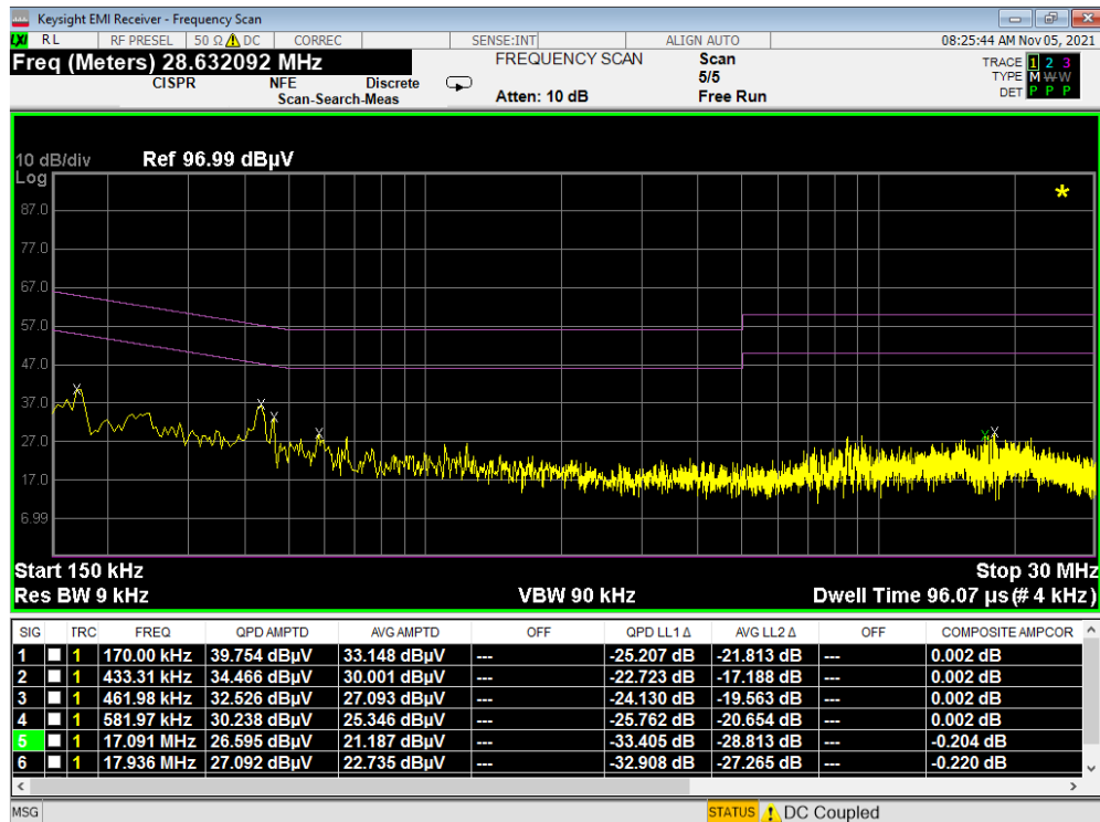
Plot 7-337. Line Conducted Plot with 802.11a UNII Band 7 (N)
