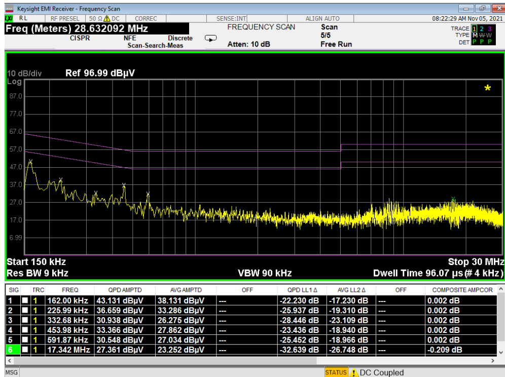
Plot 7-335. Line Conducted Plot with 802.11a UNII Band 6 (N)
