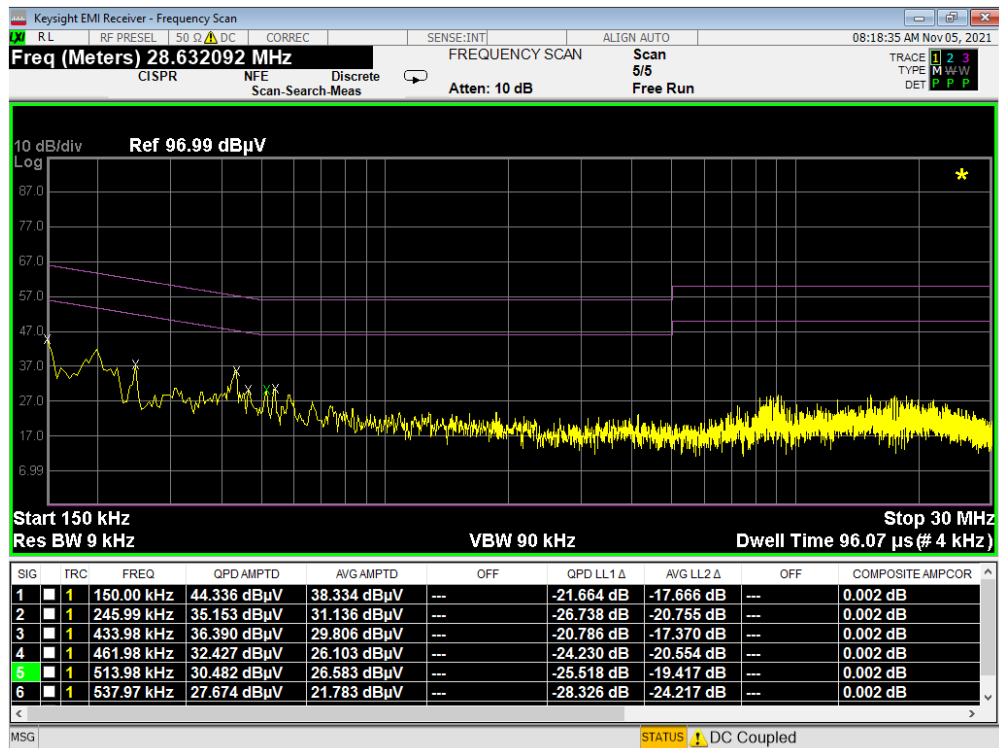
Plot 7-333. Line Conducted Plot with 802.11a UNII Band 5 (N)
