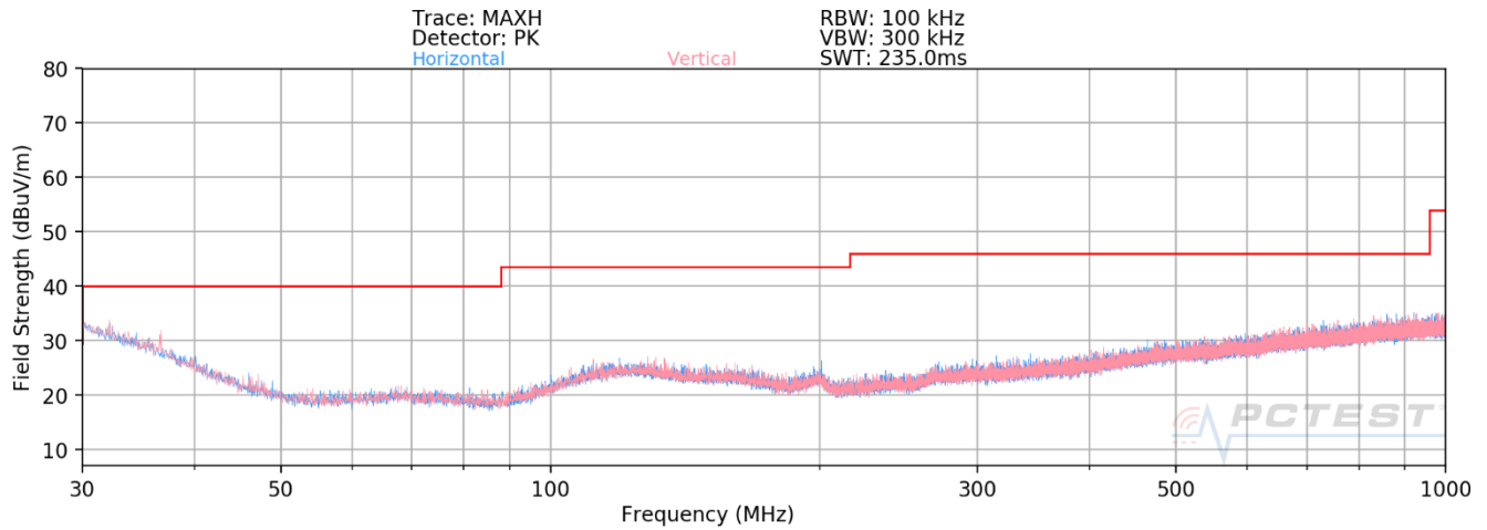
Plot 7-331. Radiated Spurious Plot below 1GHz
