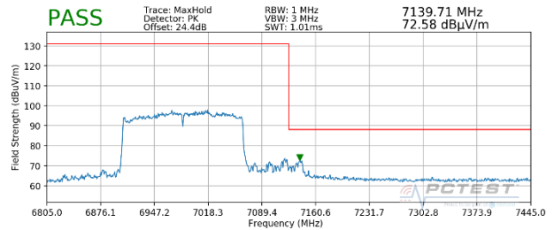
Plot 7-330. Radiated Upper Band Edge Plot MIMO (Peak – UNII Band 8)
