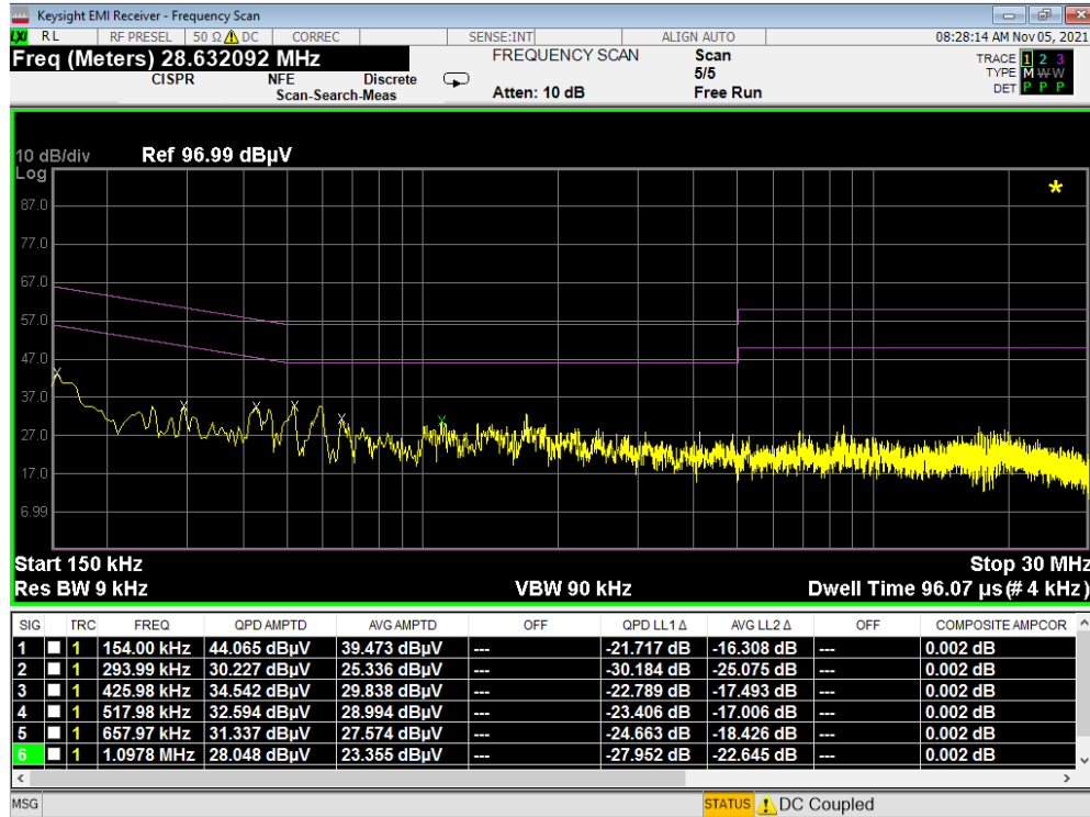
Plot 7-338. Line Conducted Plot with 802.11a UNII Band 8 (L1)
