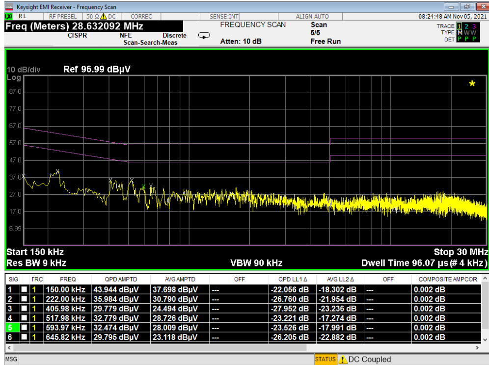
Plot 7-336. Line Conducted Plot with 802.11a UNII Band 7 (L1)
