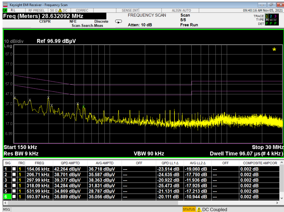
Plot 7-341. Line Conducted Plot with 802.11a UNII Band 5 (N) with WCP
