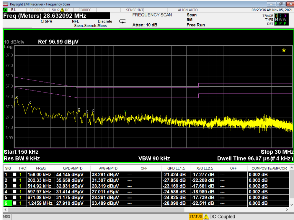
Plot 7-334. Line Conducted Plot with 802.11a UNII Band 6 (L1)
