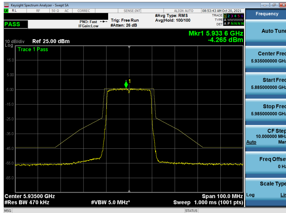
Plot 7-264. In-Band Emission Measurement Plot MIMO ANT2 (20MHz 802.11a (UNII Band 5) – Ch. 2)
