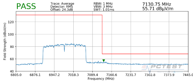
Plot 7-329. Radiated Upper Band Edge Plot MIMO (Average – UNII Band 8)
