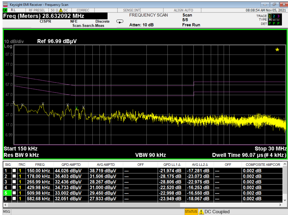
Plot 7-332. Line Conducted Plot with 802.11a UNII Band 5 (L1)
