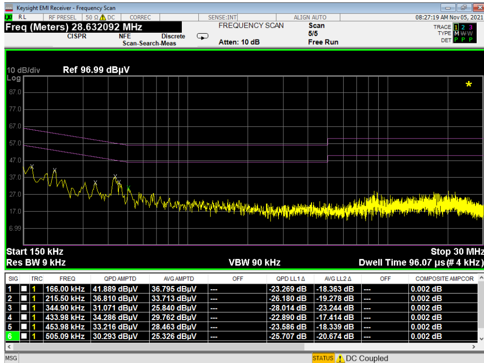
Plot 7-339. Line Conducted Plot with 802.11a UNII Band 8 (N)
