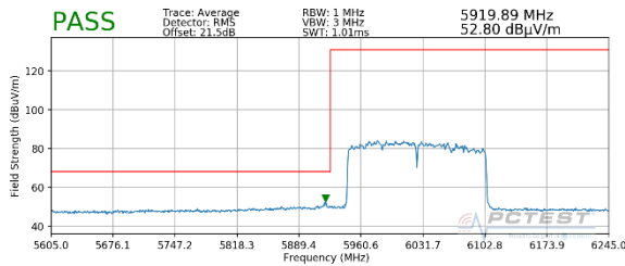
Plot 7-327. Radiated Lower Band Edge Plot MIMO (Average – UNII Band 5)
