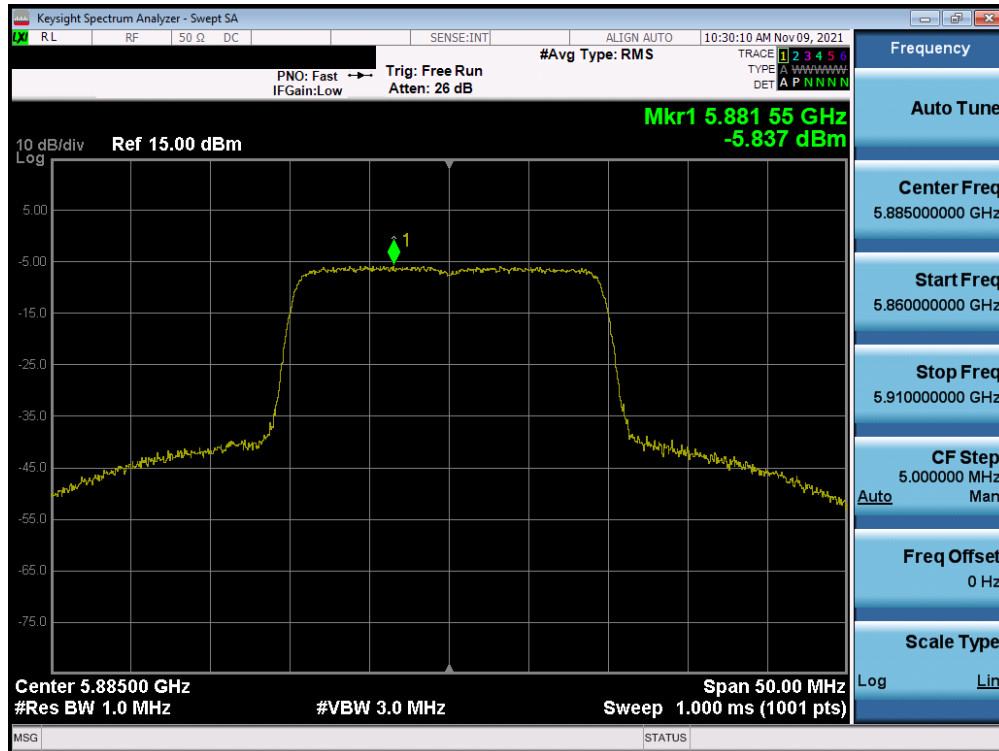
Plot 7-307. Power Spectral Density Plot MIMO ANT2 (20MHz BW 802.11ax – Full Tones (UNII Band 3/4) – Ch. 177)
