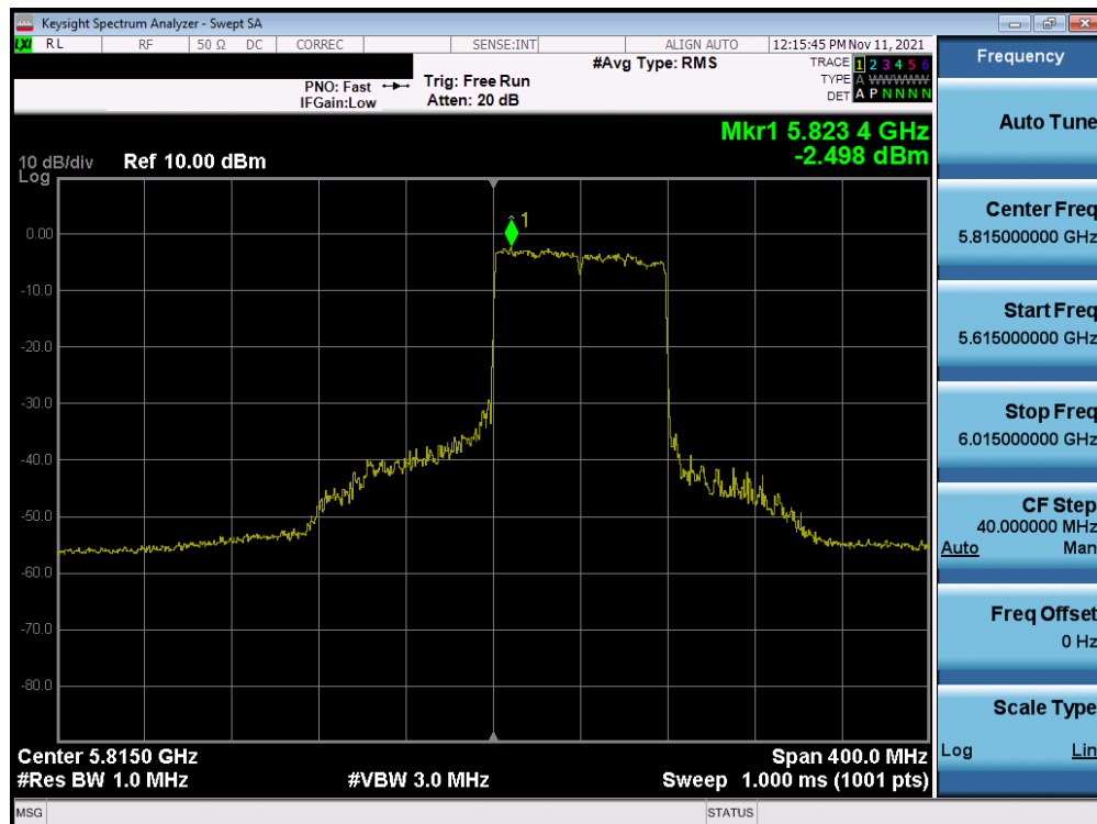
Plot 7-312. Power Spectral Density Plot MIMO ANT2 (160MHz BW (U) 802.11ax – Full Tones (UNII Band 3/4) – Ch. 171)
