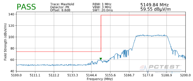
Plot 7-328. Radiated Lower Band Edge Plot MIMO (Peak - UNII Band 1 - 242 Tones)
