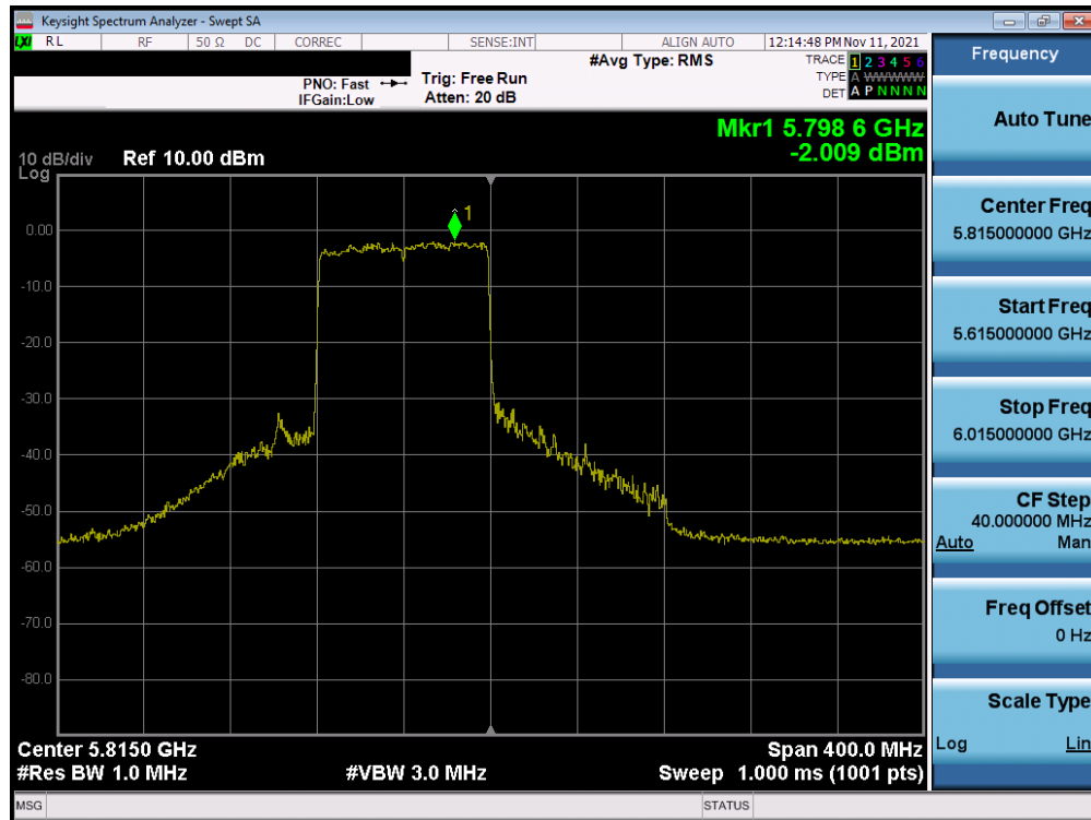
Plot 7-311. Power Spectral Density Plot MIMO ANT2 (160MHz BW (L) 802.11ax – Full Tones (UNII Band 3/4) – Ch. 163)
