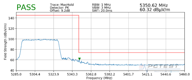
Plot 7-339. Radiated Upper Band Edge Plot MIMO (Peak – UNII Band 2A – 484 Tones)
