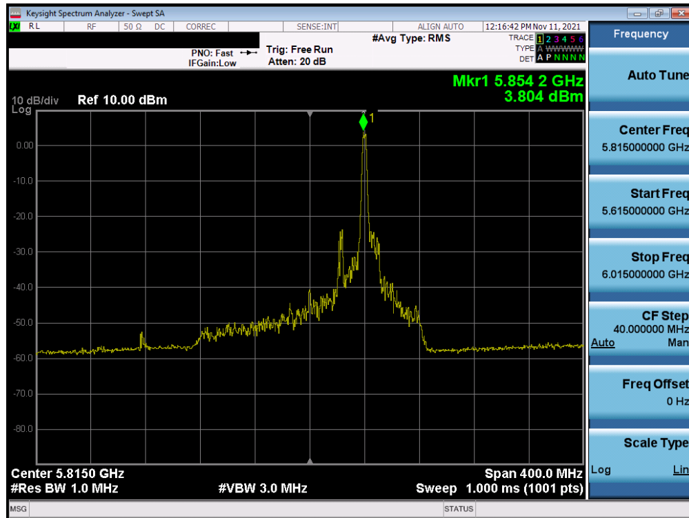
Plot 7-273. Power Spectral Density Plot MIMO ANT2 (160MHz BW (U) 802.11ax – 26 Tones (UNII Band 3/4) – Ch. 163)
