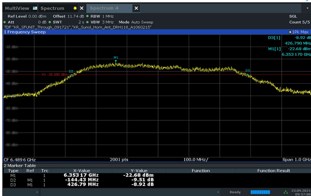
Plot 7-8. 10dBc Bandwidth – CH.5 – SP1 – Preamble 11
