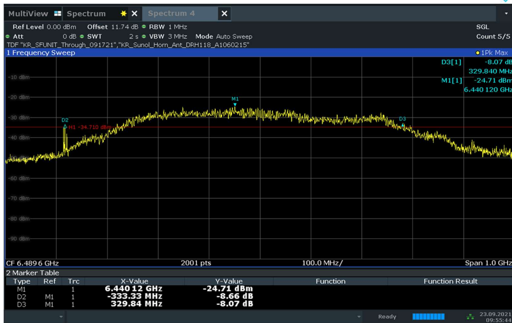
Plot 7-7. 10dBc Bandwidth – CH.5 - SP0 – Preamble 11
