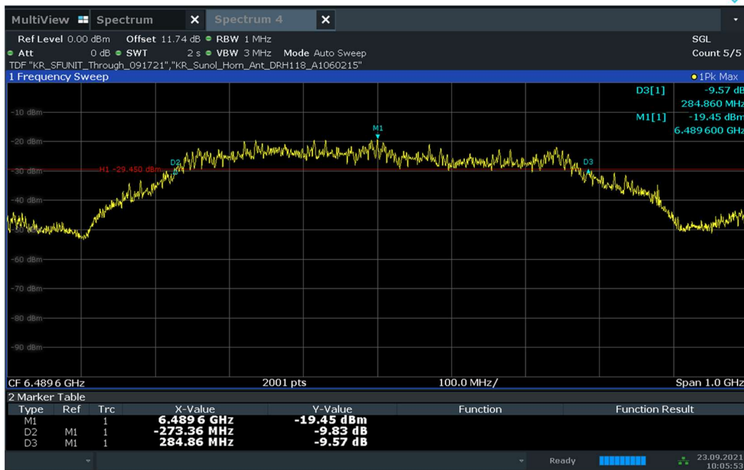
Plot 7-13. 10dBc Bandwidth – CH.5 - SP0 – Preamble 27
