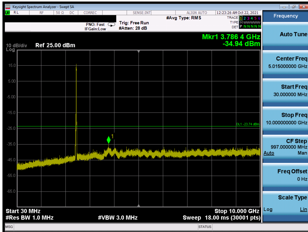
Plot 7-57. Conducted Spurious Plot MIMO ANT2 (802.11ax OFDMA – 242 Tones – Ch. 11)
