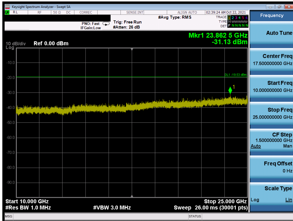
Plot 7-50. Conducted Spurious Plot MIMO ANT2 (802.11ax OFDMA – 26 Tones – Ch. 6)
