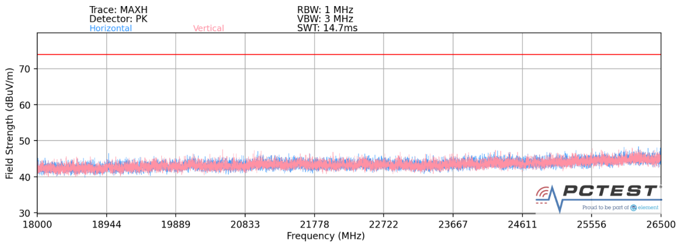
Plot 7-66. Radiated Spurious Plot above 18GHz MIMO (802.11ax OFDMA – 242 Tones)
