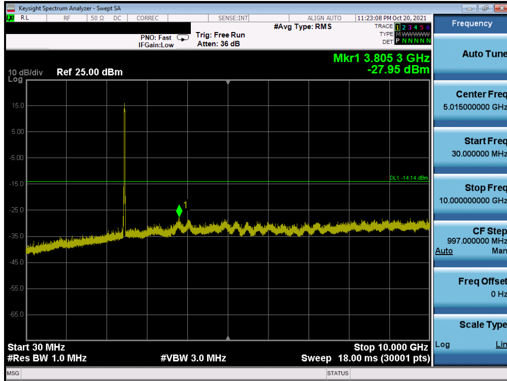
Plot 7-45. Conducted Spurious Plot MIMO ANT1 (802.11ax OFDMA – 242 Tones – Ch. 11)
