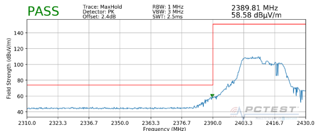
Plot 7-68. Radiated Restricted Lower Band Edge Measurement MIMO (Peak – 106 Tones)
