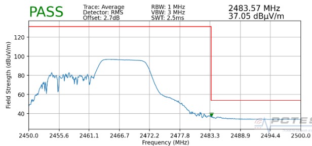
Plot 7-69. Radiated Restricted Upper Band Edge Measurement MIMO (Average – 106 Tones)
