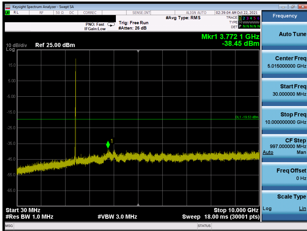
Plot 7-49. Conducted Spurious Plot MIMO ANT2 (802.11ax OFDMA – 26 Tones – Ch. 6)
