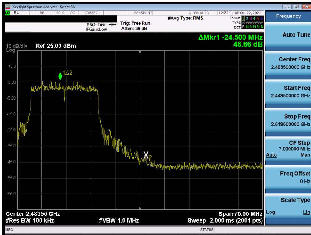
Plot 7-34. Band Edge Plot MIMO ANT2 (802.11ax OFDMA – 242 Tones – Ch. 11)
