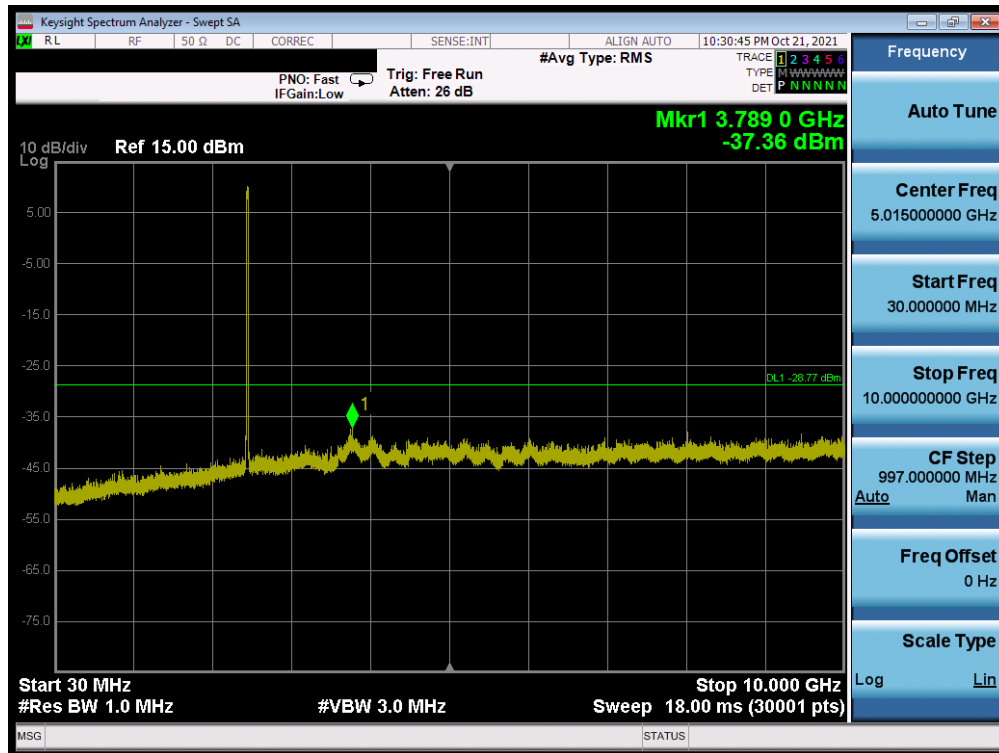
Plot 7-39. Conducted Spurious Plot MIMO ANT1 (802.11ax OFDMA – 26 Tones – Ch. 11)
