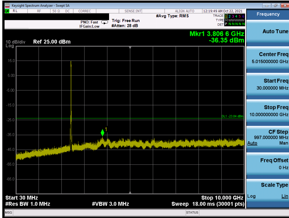
Plot 7-55. Conducted Spurious Plot MIMO ANT2 (802.11ax OFDMA – 242 Tones – Ch. 6)
