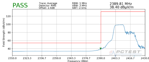
Plot 7-67. Radiated Restricted Lower Band Edge Measurement MIMO (Average – 106 Tones)
