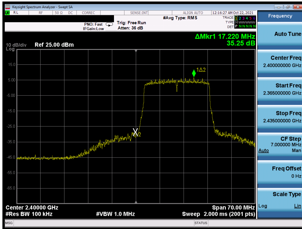
Plot 7-32. Band Edge Plot MIMO ANT2 (802.11ax OFDMA – 242 Tones – Ch. 1)
