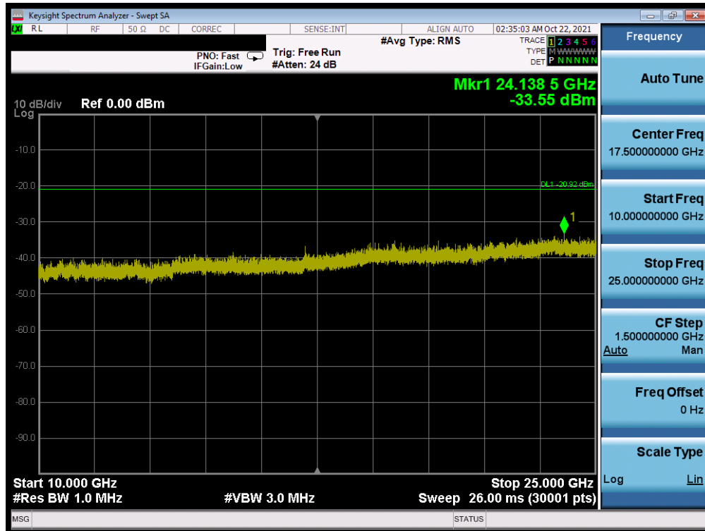
Plot 7-48. Conducted Spurious Plot MIMO ANT2 (802.11ax OFDMA – 26 Tones – Ch. 1)
