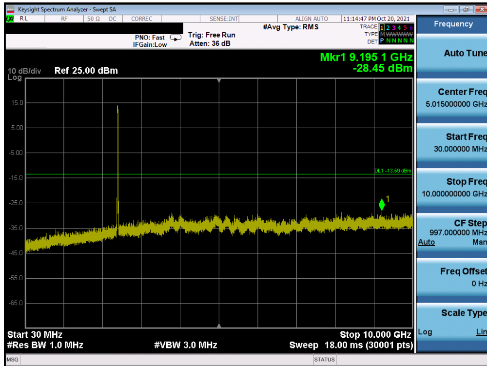
Plot 7-41. Conducted Spurious Plot MIMO ANT1 (802.11ax OFDMA – 242 Tones – Ch. 1)
