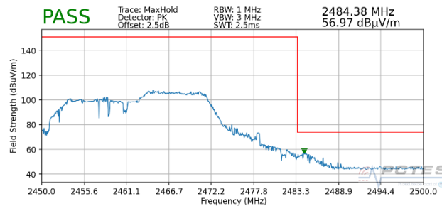
Plot 7-70. Radiated Restricted Upper Band Edge Measurement MIMO (Peak – 106 Tones)
