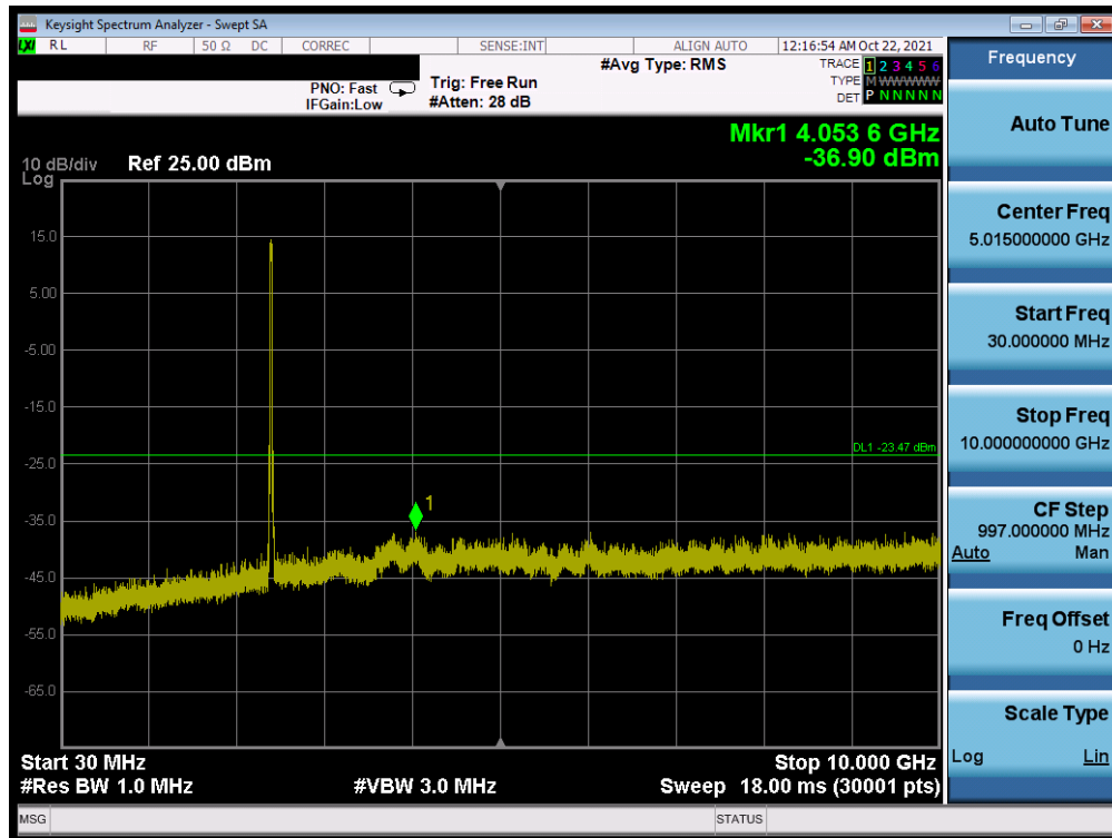
Plot 7-53. Conducted Spurious Plot MIMO ANT2 (802.11ax OFDMA – 242 Tones – Ch. 1)
