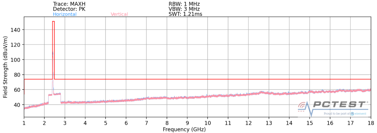
Plot 7-62. Radiated Spurious Plot above 1GHz MIMO (802.11ax OFDMA – 242 Tones – Ch. 1)
