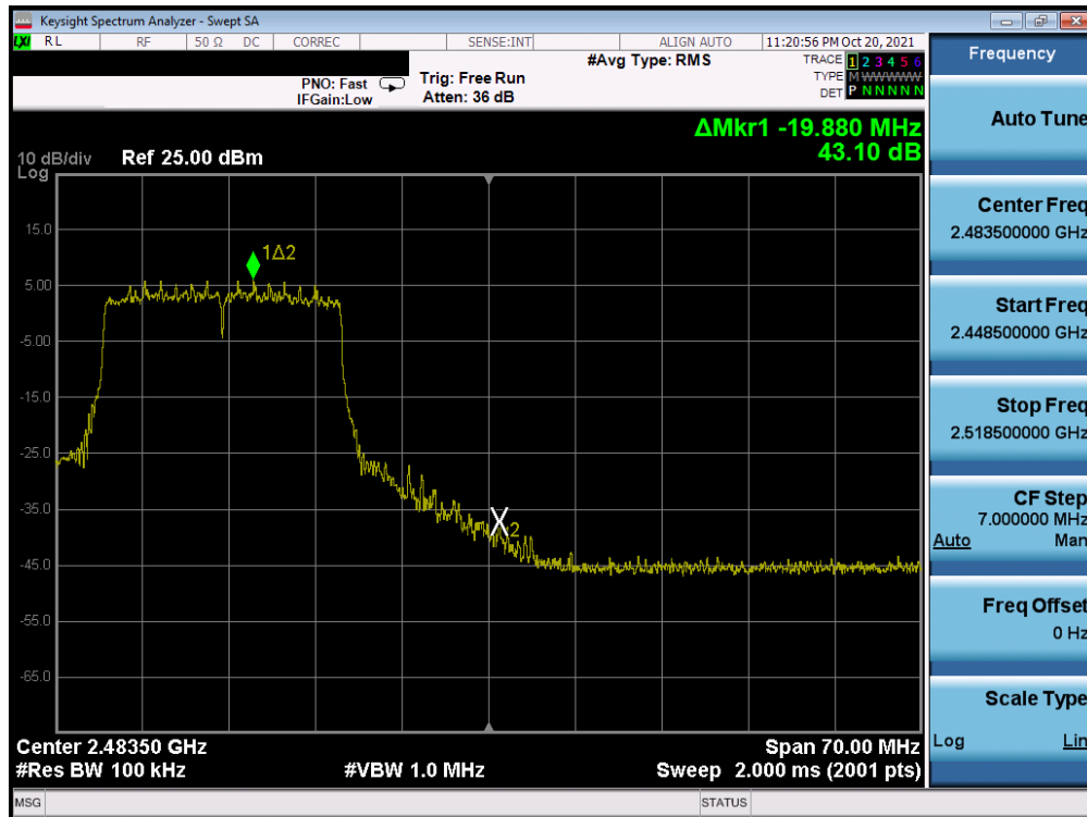
Plot 7-29. Band Edge Plot MIMO ANT1 (802.11ax OFDMA – 242 Tones – Ch. 11)
