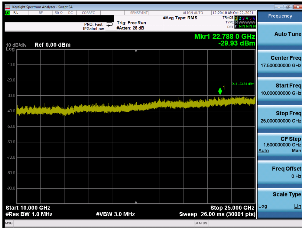
Plot 7-56. Conducted Spurious Plot MIMO ANT2 (802.11ax OFDMA – 242 Tones – Ch. 6)
