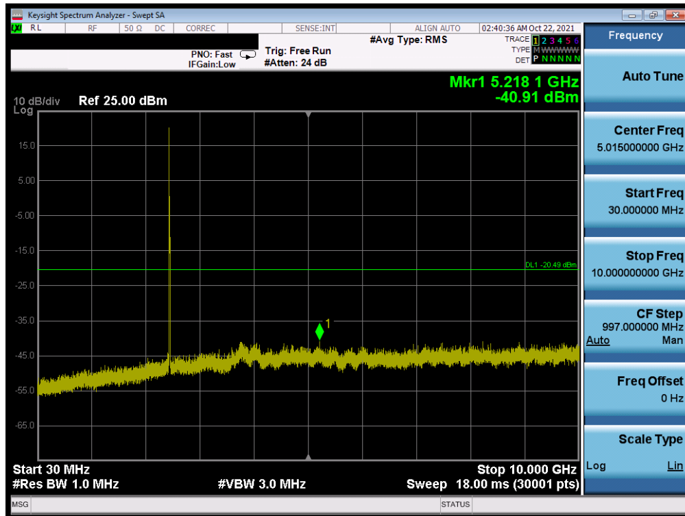
Plot 7-51. Conducted Spurious Plot MIMO ANT2 (802.11ax OFDMA - 26 Tones - Ch. 11)
