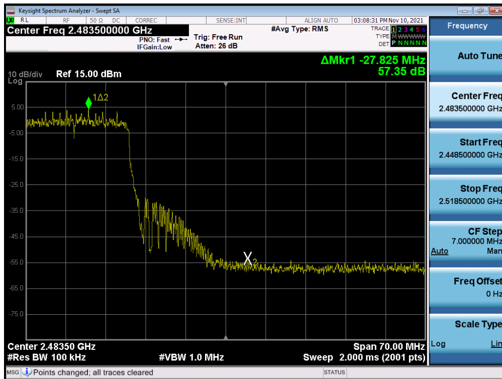
Plot 7-33. Band Edge Plot MIMO ANT2 (802.11ax OFDMA – 242 Tones – Ch. 10)
