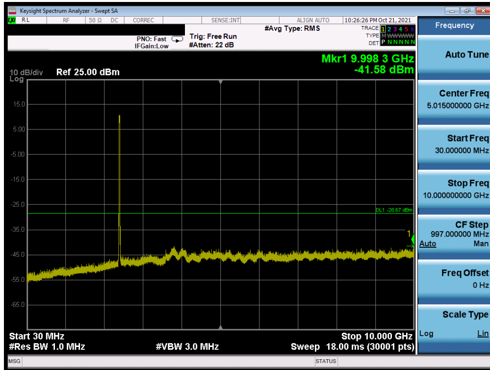
Plot 7-35. Conducted Spurious Plot MIMO ANT1 (802.11ax OFDMA – 26 Tones – Ch. 1)
