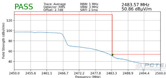
Plot 7-73. Radiated Restricted Upper Band Edge Measurement MIMO (Average – 242 Tones)
