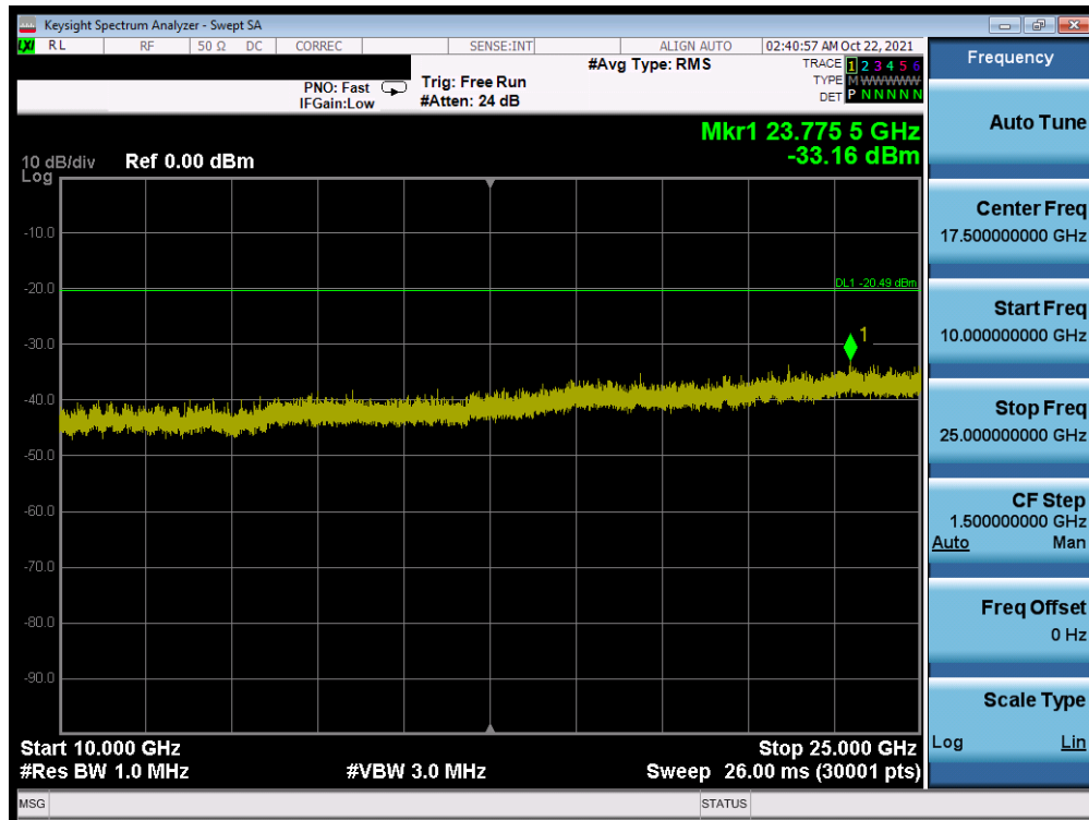
Plot 7-52. Conducted Spurious Plot MIMO ANT2 (802.11ax OFDMA - 26 Tones - Ch. 11)
