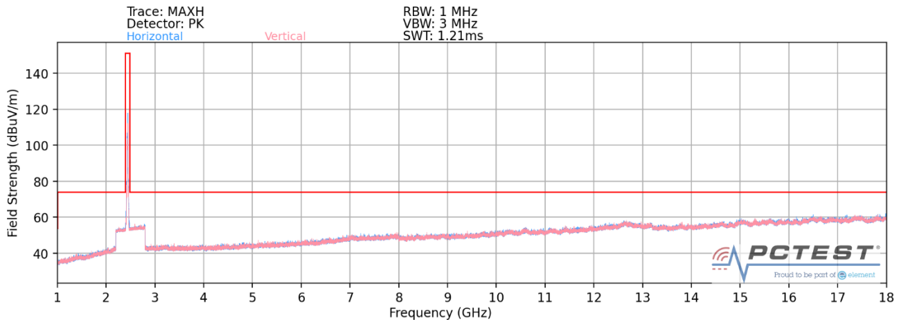
Plot 7-60. Radiated Spurious Plot above 1GHz MIMO (802.11ax OFDMA – 26 Tones – Ch. 6)
