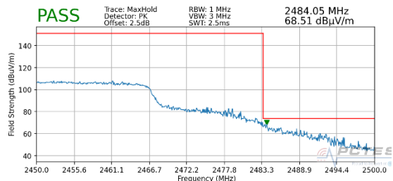
Plot 7-74. Radiated Restricted Upper Band Edge Measurement MIMO (Peak – 242 Tones)
