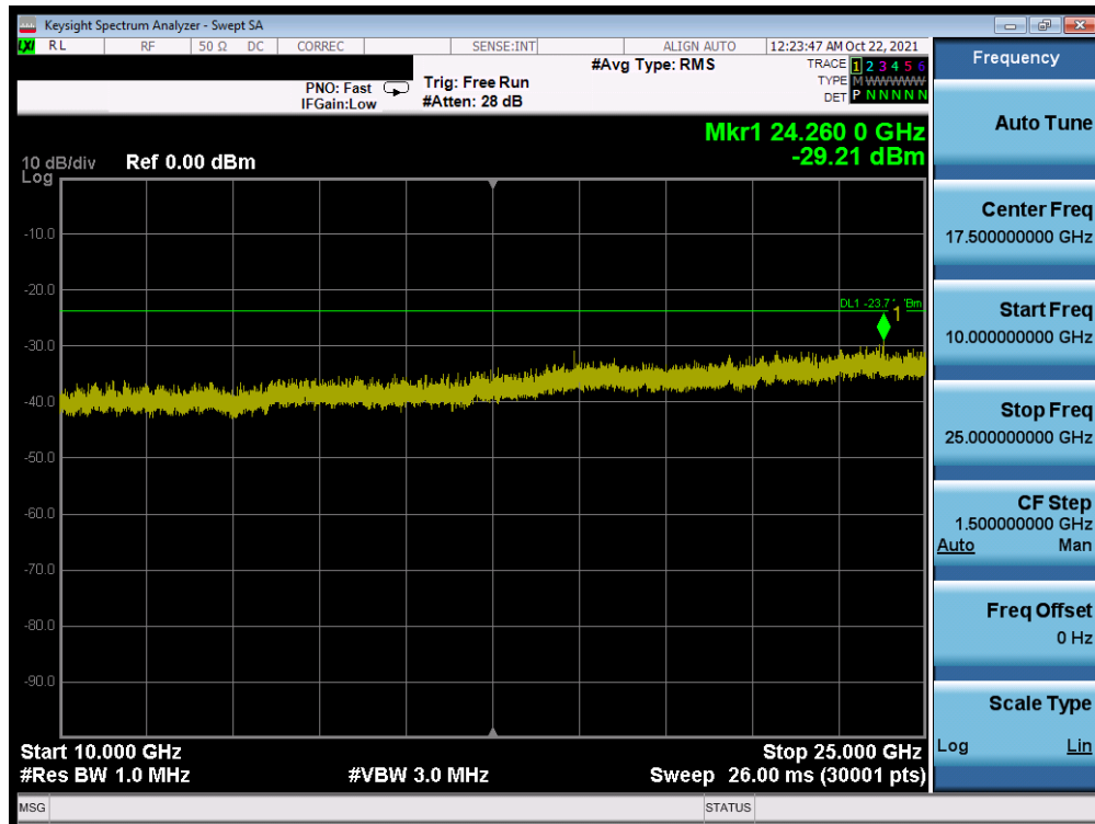
Plot 7-58. Conducted Spurious Plot MIMO ANT2 (802.11ax OFDMA – 242 Tones – Ch. 11)
