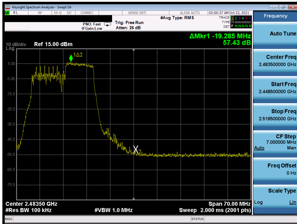
Plot 7-31. Band Edge Plot MIMO ANT2 (802.11ax OFDMA – 106 Tones – Ch. 11)
