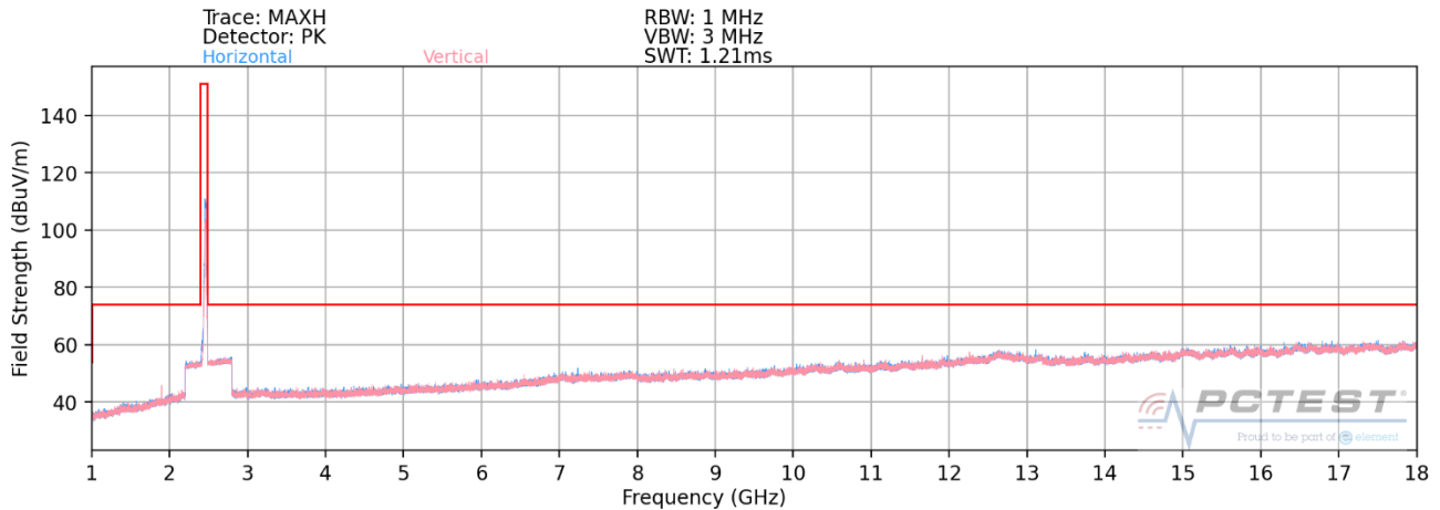
Plot 7-64. Radiated Spurious Plot above 1GHz MIMO (802.11ax OFDMA – 242 Tones – Ch. 11)
