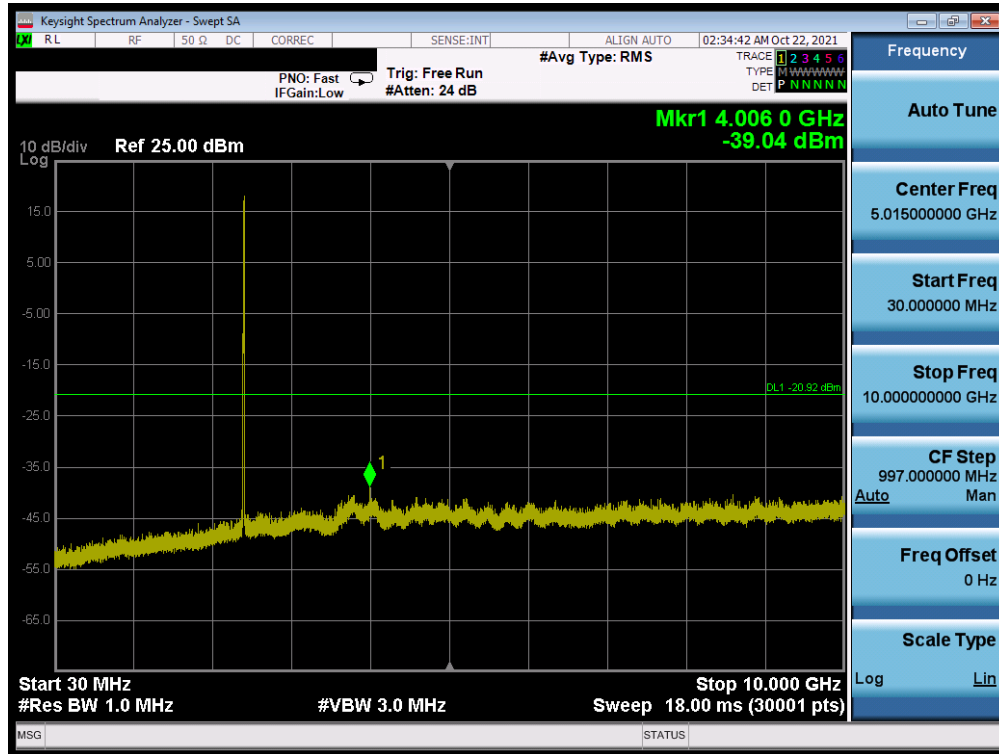
Plot 7-47. Conducted Spurious Plot MIMO ANT2 (802.11ax OFDMA – 26 Tones – Ch. 1)
