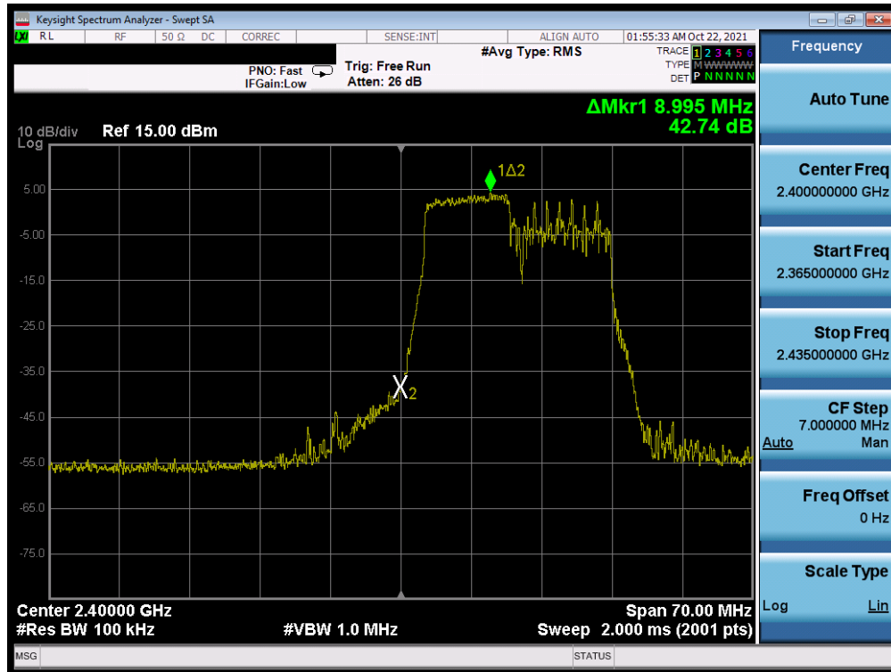
Plot 7-30. Band Edge Plot MIMO ANT2 (802.11ax OFDMA – 106 Tones – Ch. 1)
