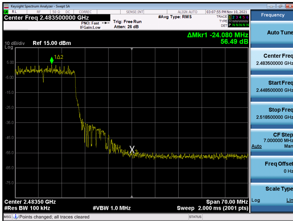
Plot 7-28. Band Edge Plot MIMO ANT1 (802.11ax OFDMA – 242 Tones – Ch. 10)
