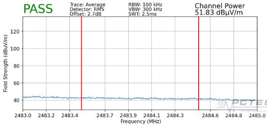
Plot 7-75. Radiated Restricted Upper Band Edge Measurement MIMO (Average – 242 Tones)
