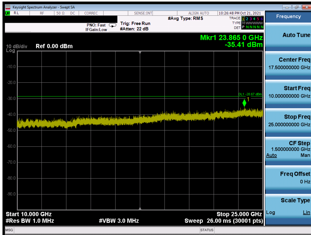
Plot 7-36. Conducted Spurious Plot MIMO ANT1 (802.11ax OFDMA – 26 Tones – Ch. 1)
