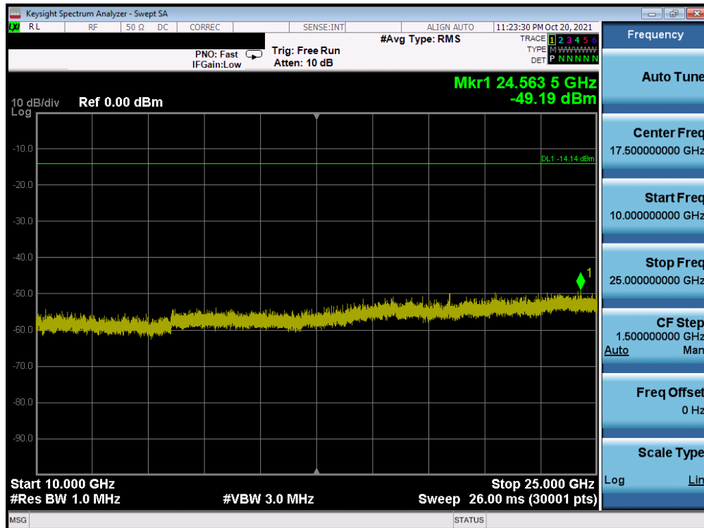
Plot 7-46. Conducted Spurious Plot MIMO ANT1 (802.11ax OFDMA – 242 Tones – Ch. 11)
