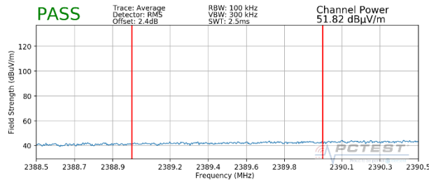
Plot 7-71. Radiated Restricted Lower Band Edge Measurement MIMO (Average – 242 Tones)
