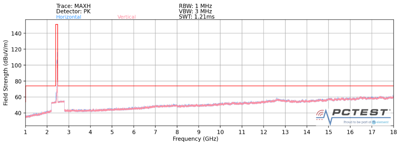
Plot 7-61. Radiated Spurious Plot above 1GHz MIMO (802.11ax OFDMA – 26 Tones – Ch. 11)
