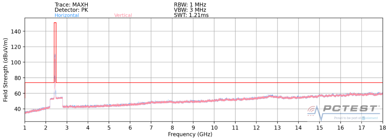
Plot 7-63. Radiated Spurious Plot above 1GHz MIMO (802.11ax OFDMA – 242 Tones – Ch. 6)
