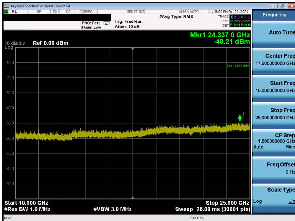
Plot 7-42. Conducted Spurious Plot MIMO ANT1 (802.11ax OFDMA – 242 Tones – Ch. 1)
