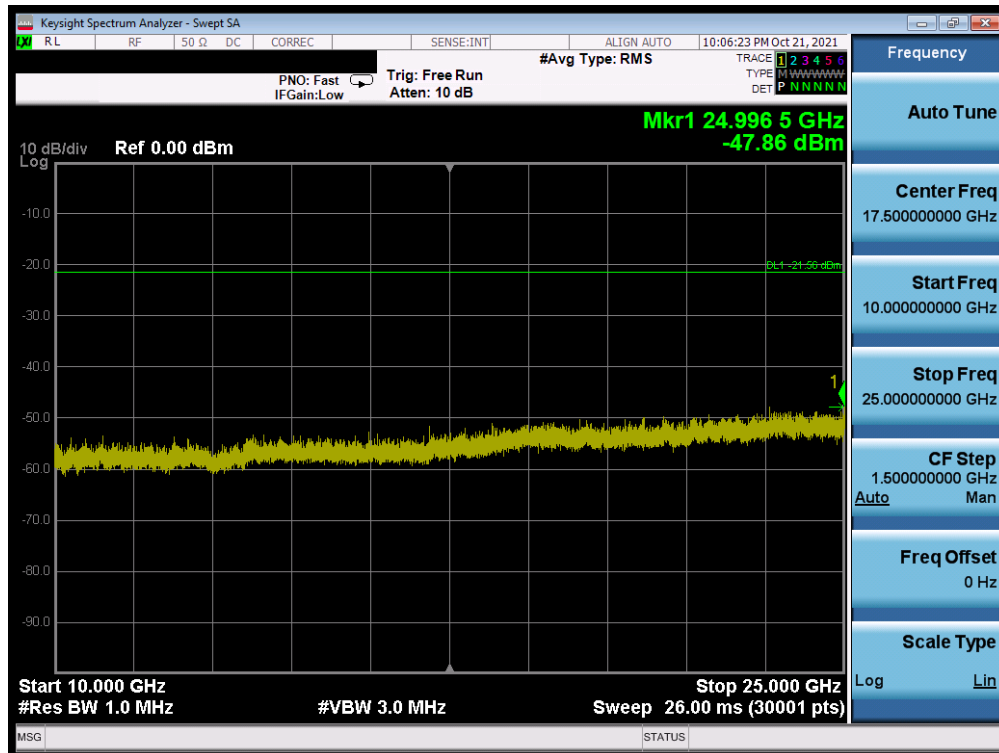
Plot 7-38. Conducted Spurious Plot MIMO ANT1 (802.11ax OFDMA – 26 Tones – Ch. 6)
