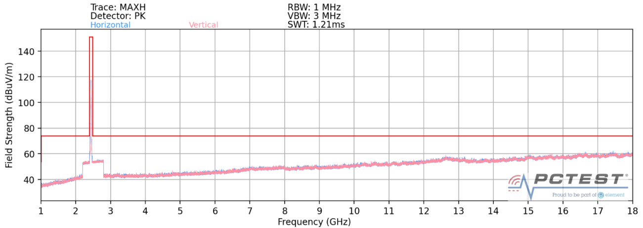
Plot 7-59. Radiated Spurious Plot above 1GHz MIMO (802.11ax OFDMA – 26 Tones – Ch. 1)
