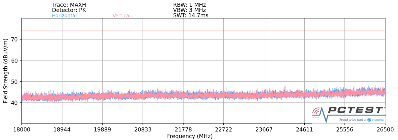
Plot 7-65. Radiated Spurious Plot above 18GHz MIMO (802.11ax OFDMA – 26 Tones)
