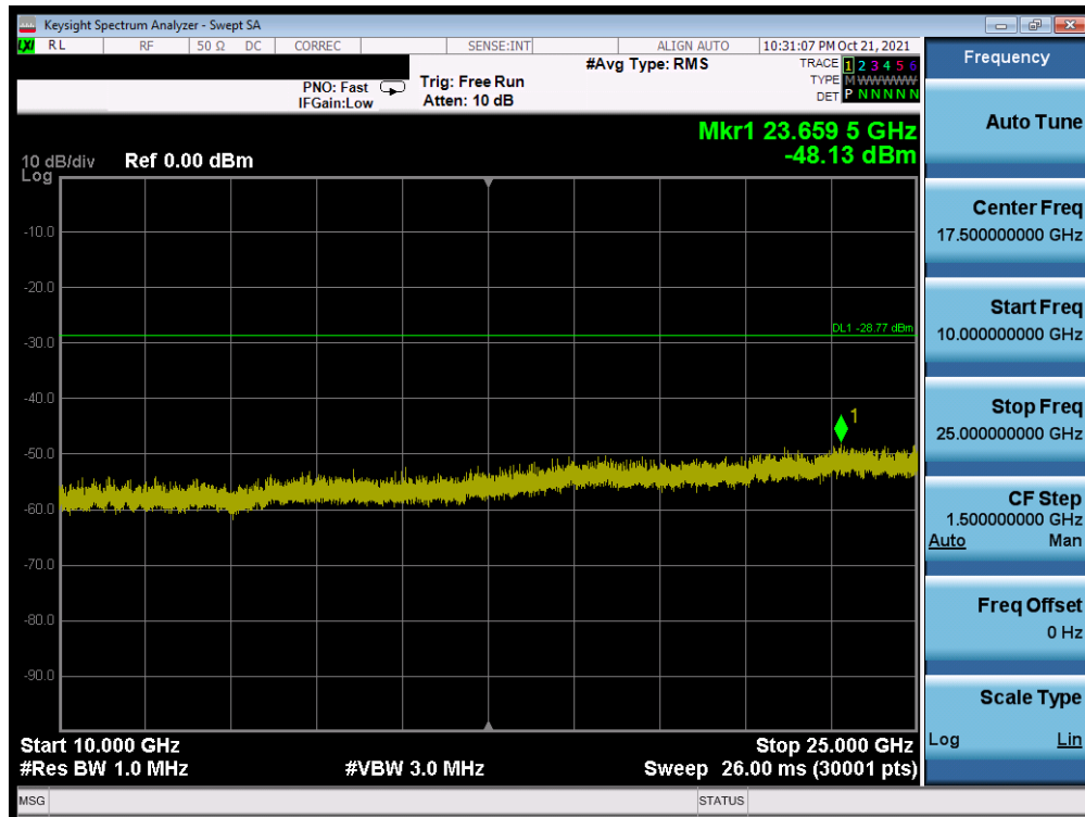
Plot 7-40. Conducted Spurious Plot MIMO ANT1 (802.11ax OFDMA – 26 Tones – Ch. 11)
