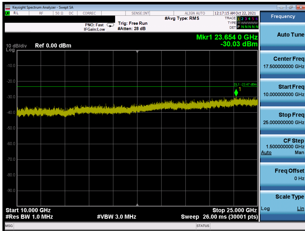
Plot 7-54. Conducted Spurious Plot MIMO ANT2 (802.11ax OFDMA – 242 Tones – Ch. 1)
