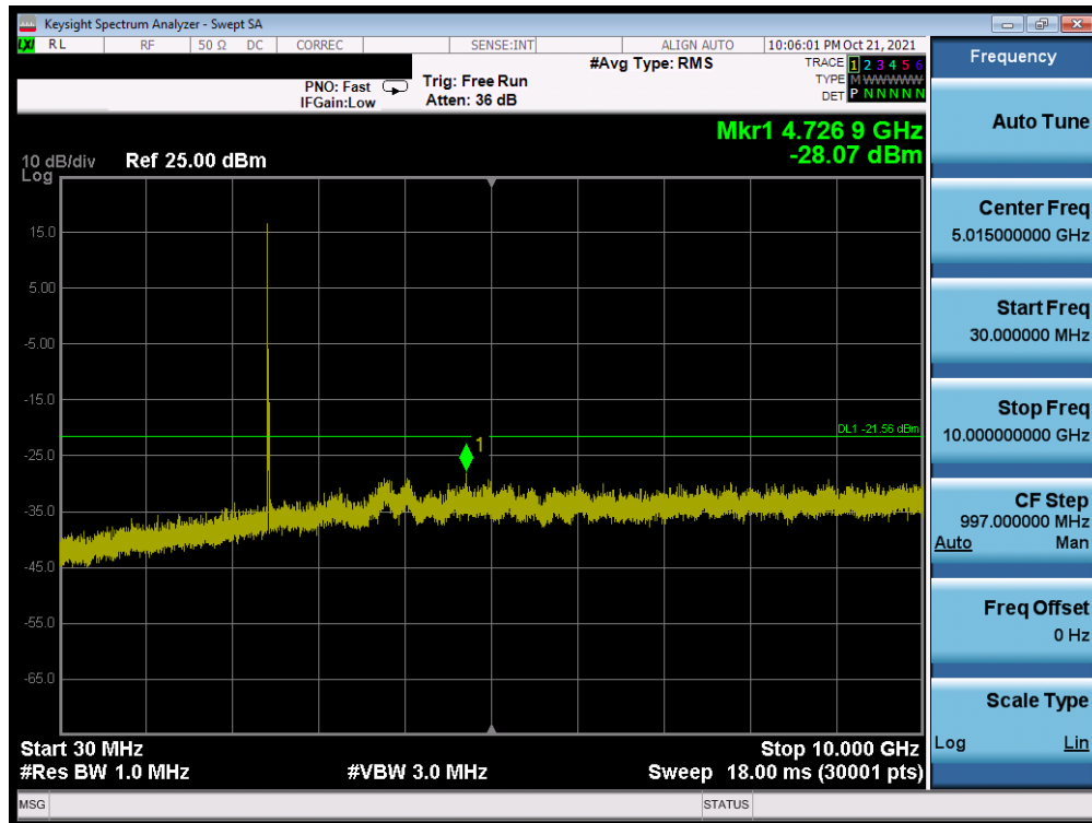
Plot 7-37. Conducted Spurious Plot MIMO ANT1 (802.11ax OFDMA – 26 Tones – Ch. 6)
