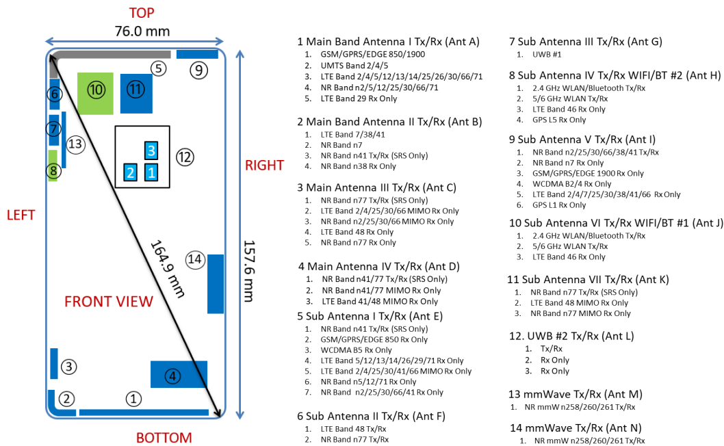
Figure C-1 DUT Antenna Locations
