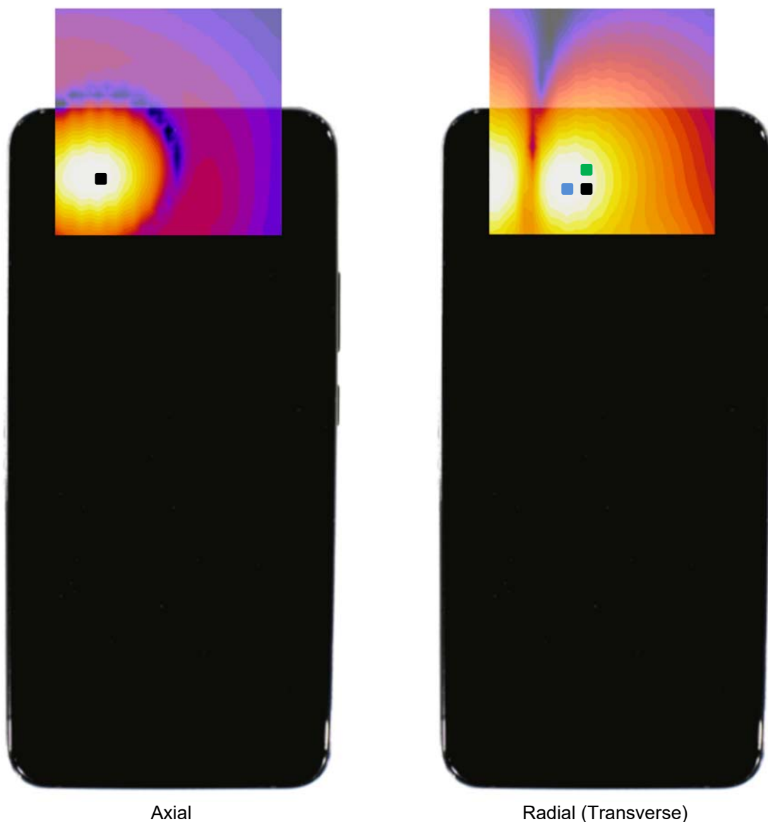
Figure 17-3 T-Coil Scan Overlay Magnetic Field Distributions
