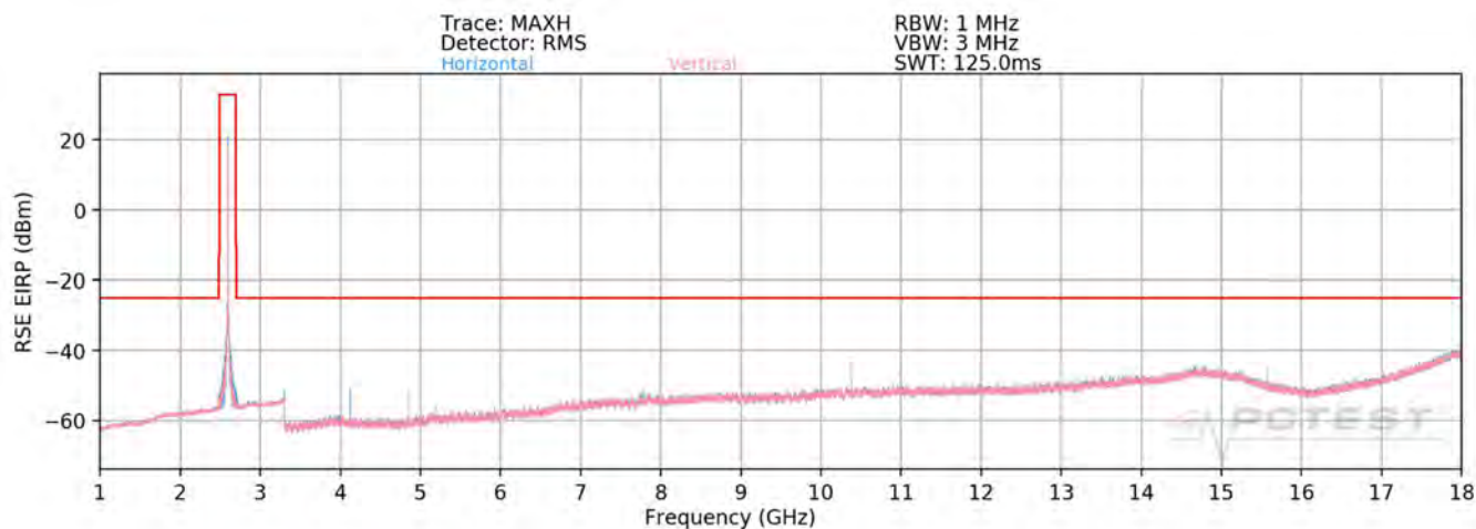
Plot 7-26. Radiated Spurious Plot (LTE Band 41(PC2))
