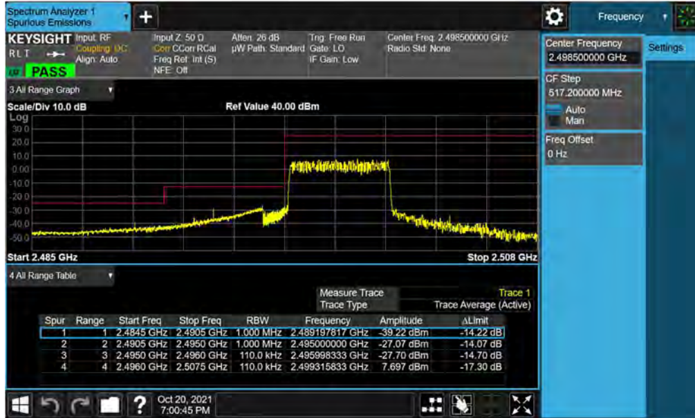
Plot 7-24. Lower ACP Plot (LTE Band 41(PC2) - 5MHz QPSK – Full RB)
