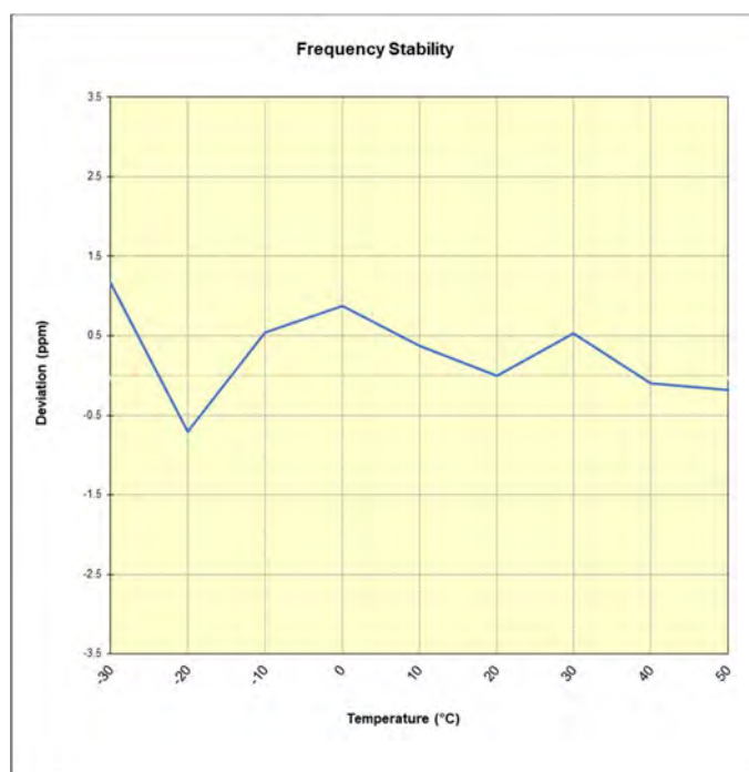
Plot 7-27. LTE Band 41(PC2) Frequency Stability Chart
