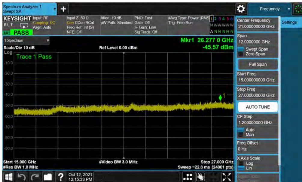
Plot 7-14. Conducted Spurious Plot (LTE Band 41(PC2) - 20MHz QPSK - RB Size 1, RB Offset 0 - Mid Channel)
