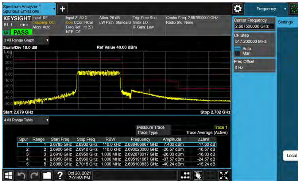
Plot 7-25. Upper ACP Plot (LTE Band 41(PC2) - 5MHz QPSK – Full RB)
