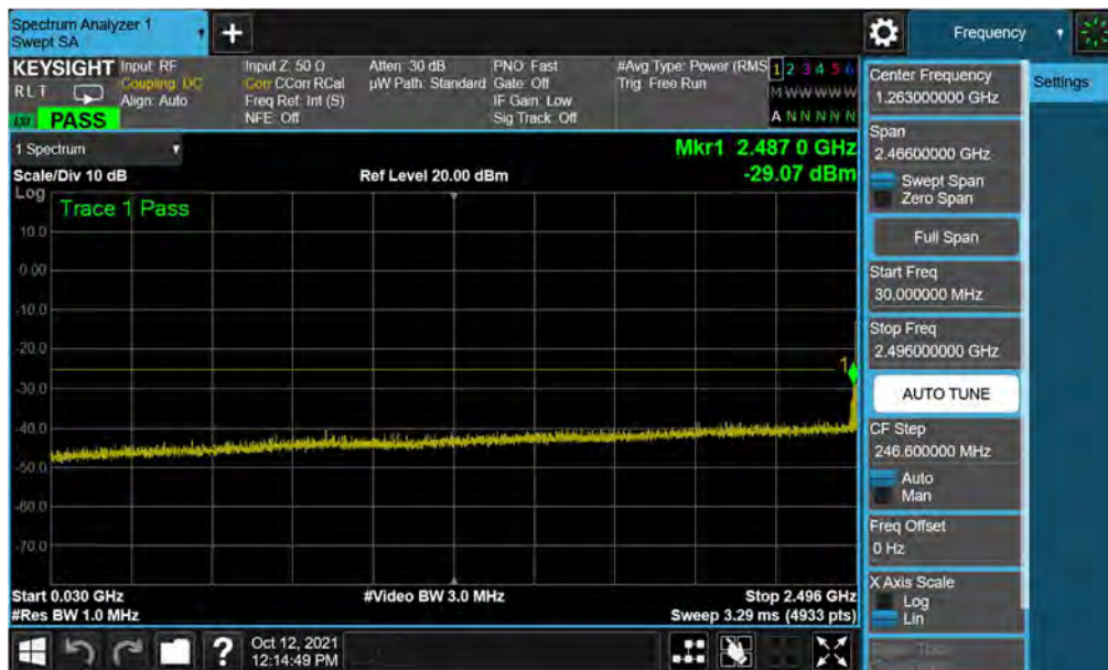
Plot 7-12. Conducted Spurious Plot (LTE Band 41(PC2) - 20MHz QPSK - RB Size 1, RB Offset 0 - Mid Channel)
