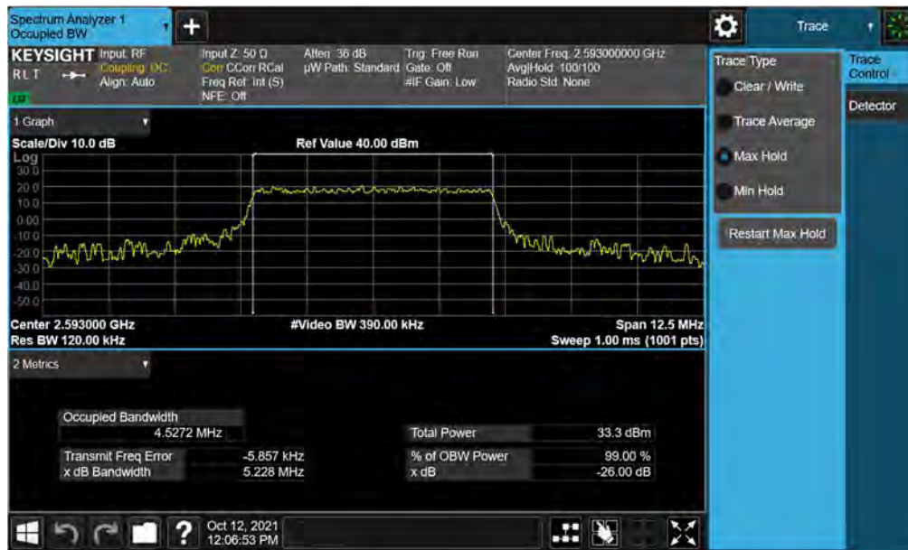
Plot 7-7. Occupied Bandwidth Plot (LTE Band 41(PC2) - 5MHz QPSK - Full RB)
