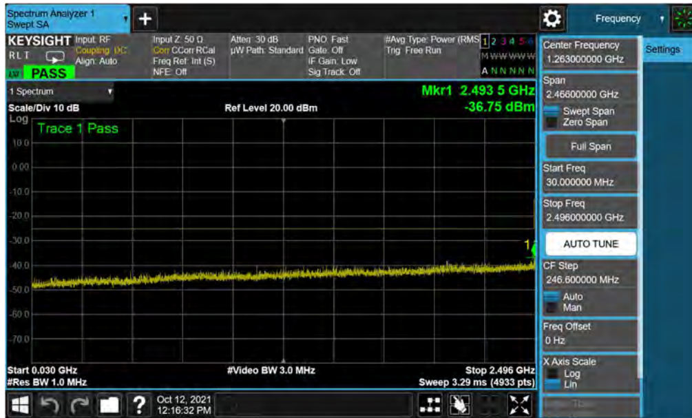
Plot 7-15. Conducted Spurious Plot (LTE Band 41(PC2) - 20MHz QPSK - RB Size 1, RB Offset 0 - High Channel)
