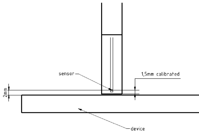
Figure C-2 EUmWVx Probe
