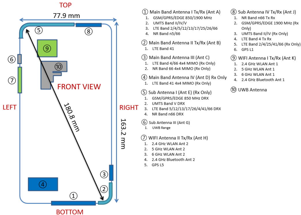
Figure C-1 DUT Antenna Locations
