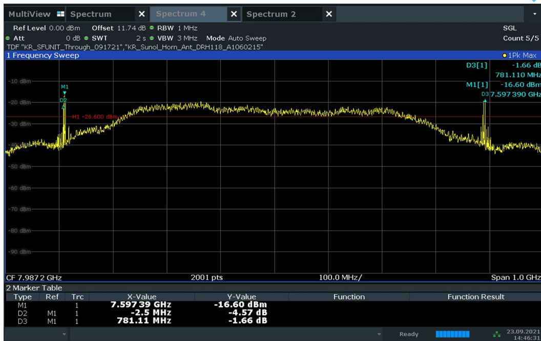
Plot 7-23. 10dBc Bandwidth – CH.9 – SP1 – Preamble 11
