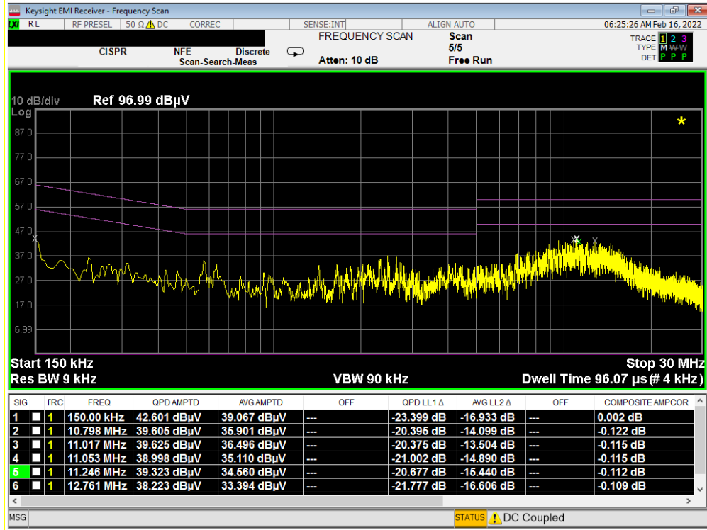
Plot 7-18. Line-Conducted Test Plot (L1) - Device to Device – Config 2
