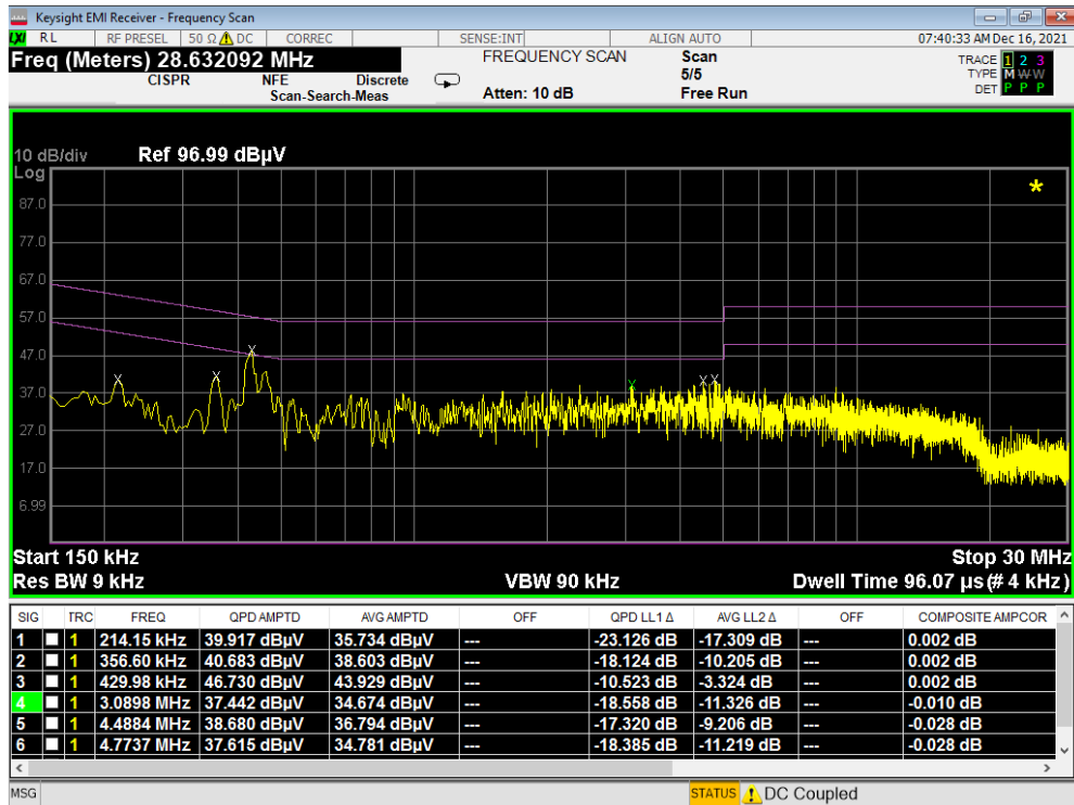
Plot 7-23. Line-Conducted Test Plot (N) - Digitizer - Hover
