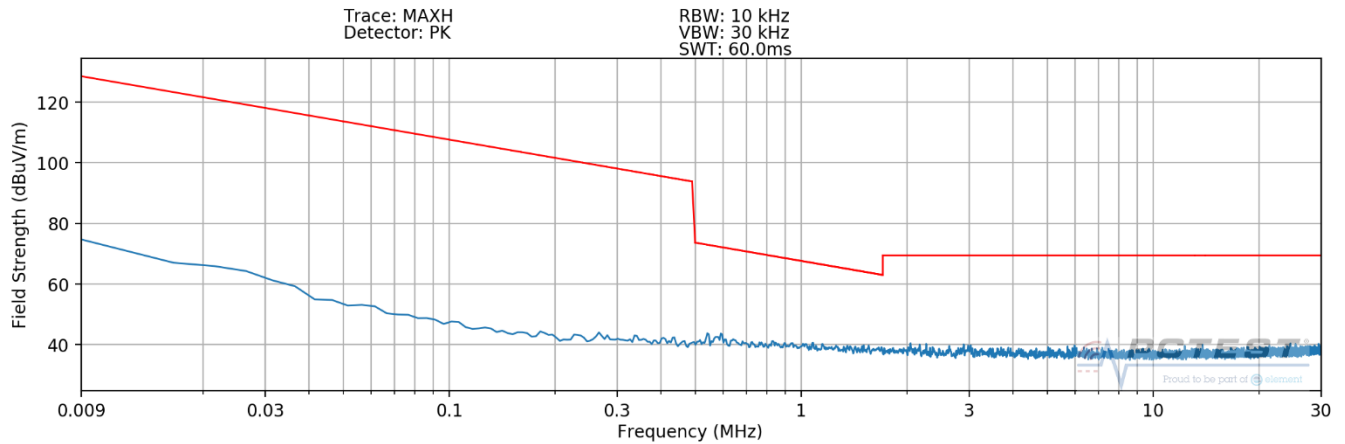
Plot 7-8. Radiated Spurious Plot 9kHz – 30MHz (Pol. Y – Device to S-Pen)
