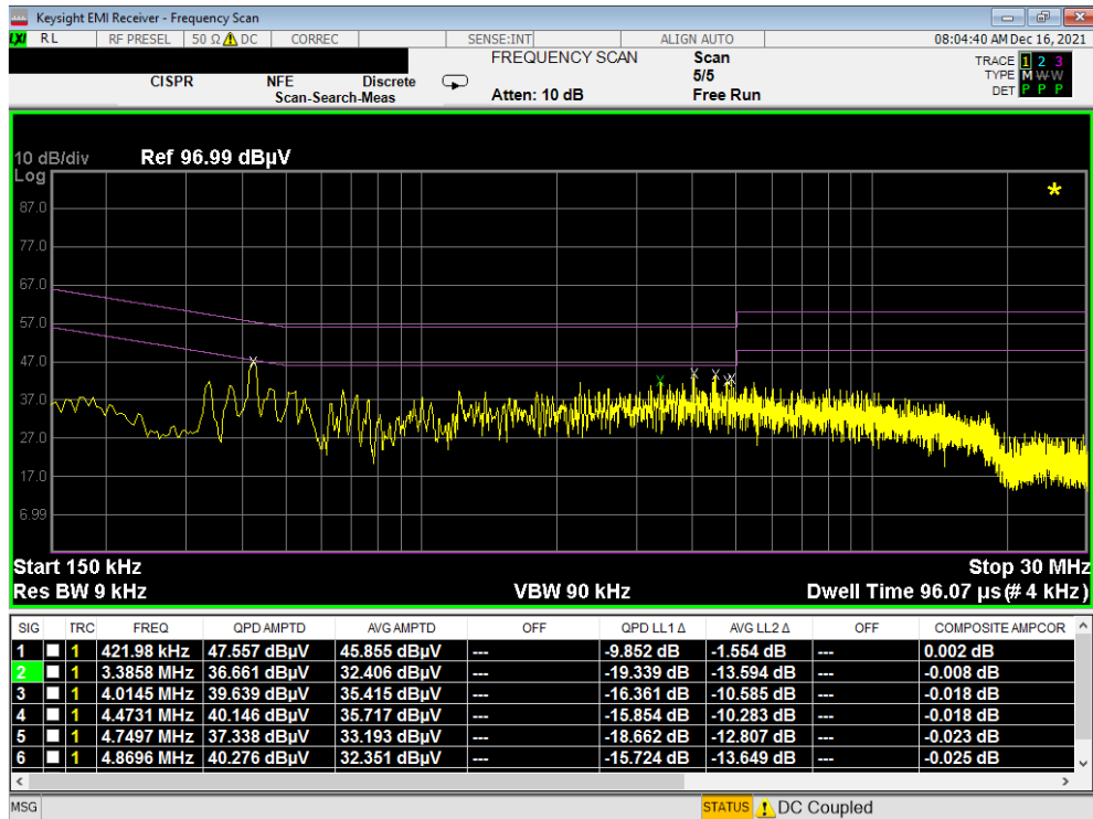
Plot 7-21. Line-Conducted Test Plot (N) - Device to S-Pen
