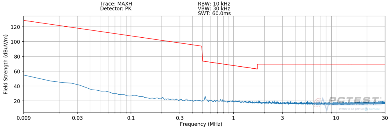
Plot 7-13. Radiated Spurious Plot 9kHz – 30MHz (Pol. X – WPT – Digitizer Click)
