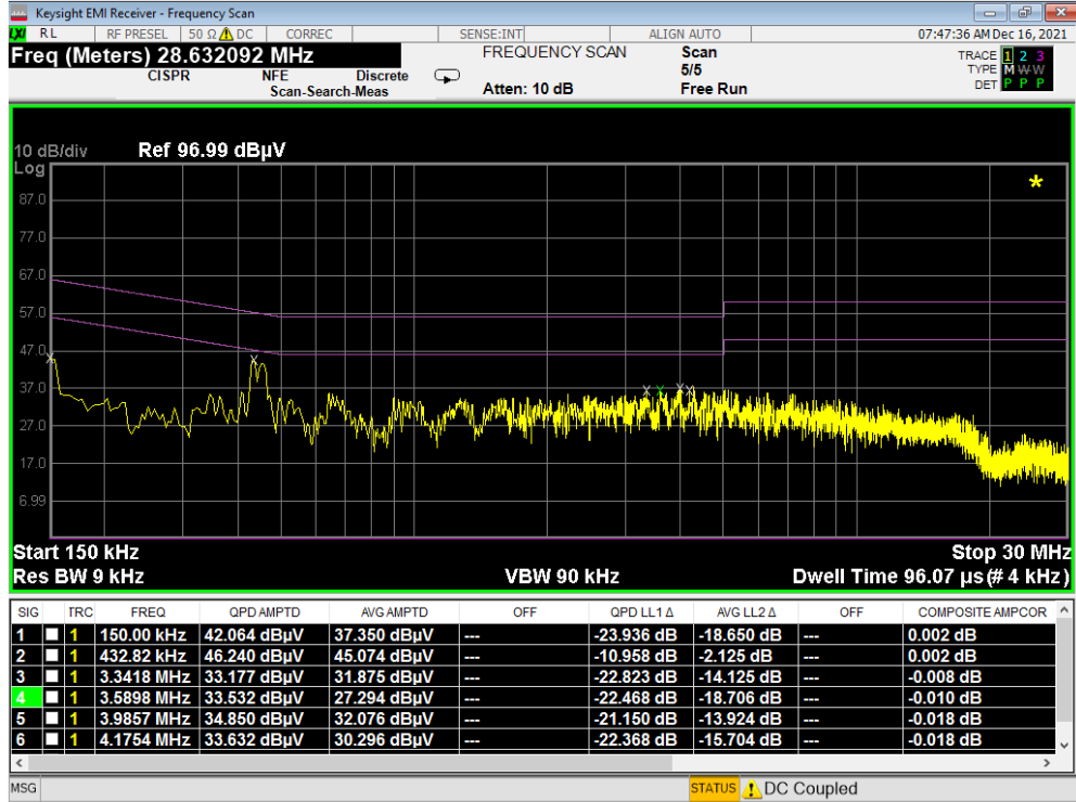
Plot 7-24. Line-Conducted Test Plot (L1) – Digitizer - Click
