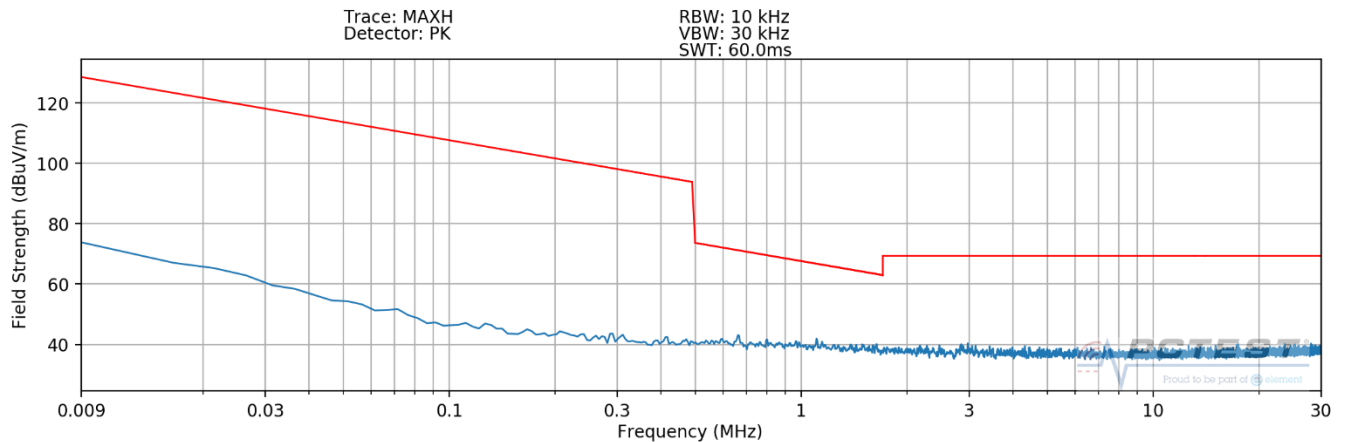
Plot 7-9. Radiated Spurious Plot 9kHz – 30MHz (Pol. Z – Device to S-Pen)
