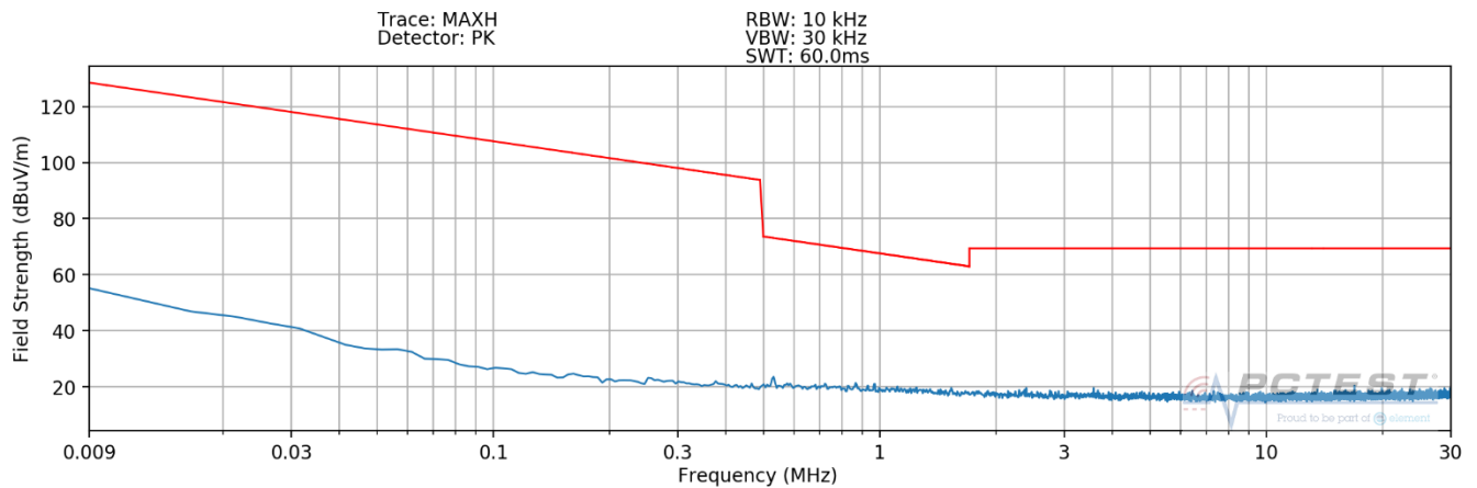
Plot 7-15. Radiated Spurious Plot 9kHz – 30MHz (Pol. Z – WPT – Digitizer Click)
