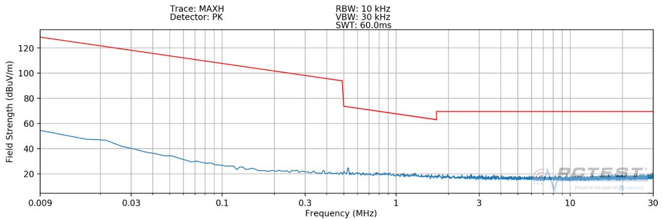
Plot 7-14. Radiated Spurious Plot 9kHz – 30MHz (Pol. Y – WPT – Digitizer Click)
