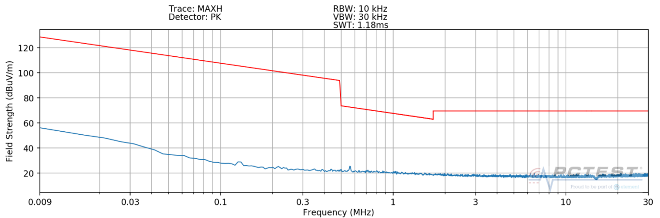
Plot 7-12. Radiated Spurious Plot 9kHz – 30MHz (Pol. Z – WPT – Digitizer Hover)
