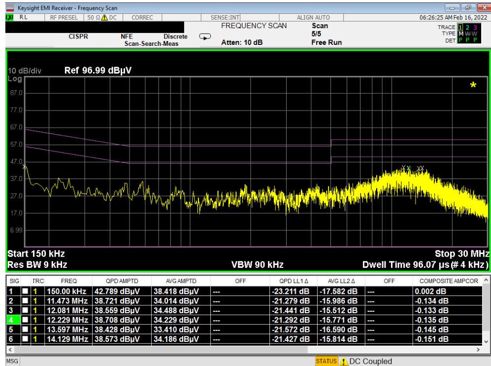
Plot 7-19. Line-Conducted Test Plot (N) - Device to Device – Config 2
