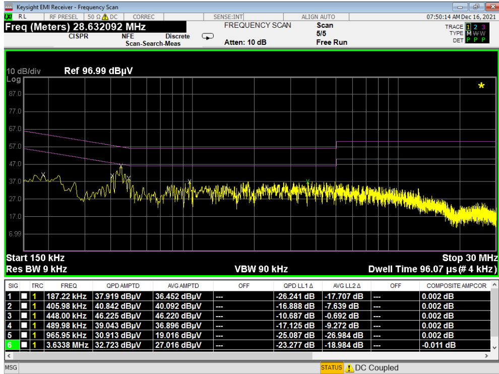
Plot 7-22. Line-Conducted Test Plot (L1) – Digitizer - Hover
