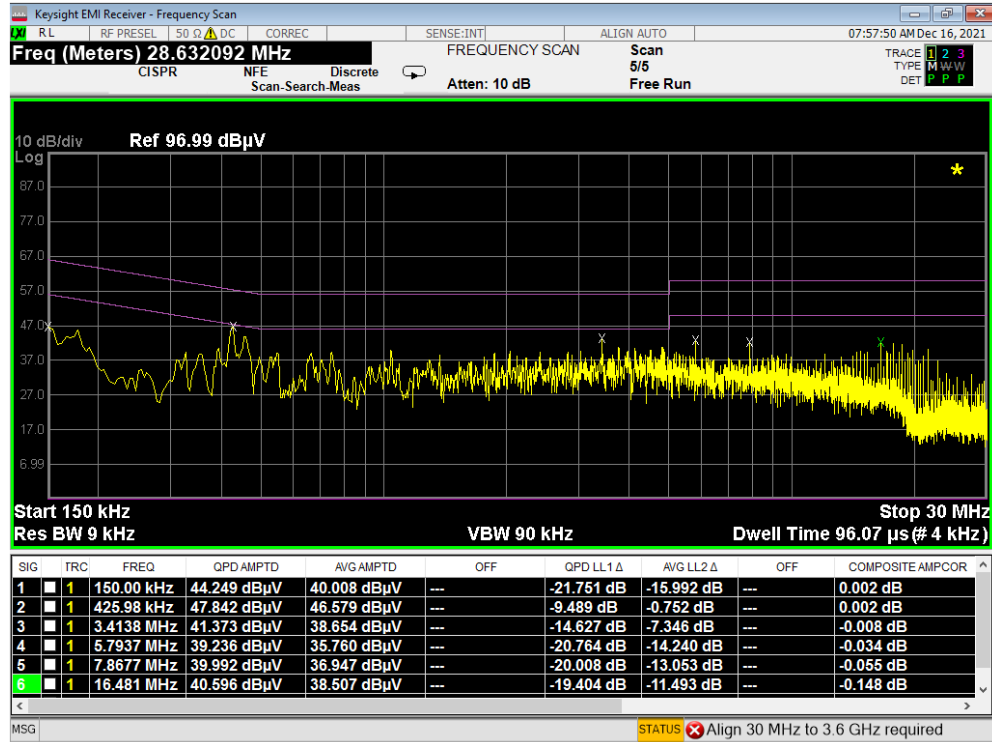
Plot 7-16. Line-Conducted Test Plot (L1) - Device to Device – Config 1
