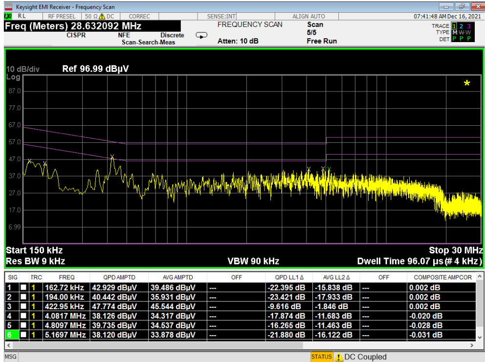
Plot 7-25. Line-Conducted Test Plot (N) - Digitizer - Click
