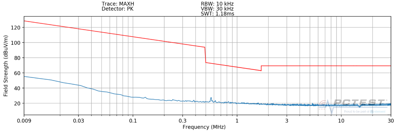
Plot 7-10. Radiated Spurious Plot 9kHz – 30MHz (Pol. X – WPT – Digitizer Hover)
