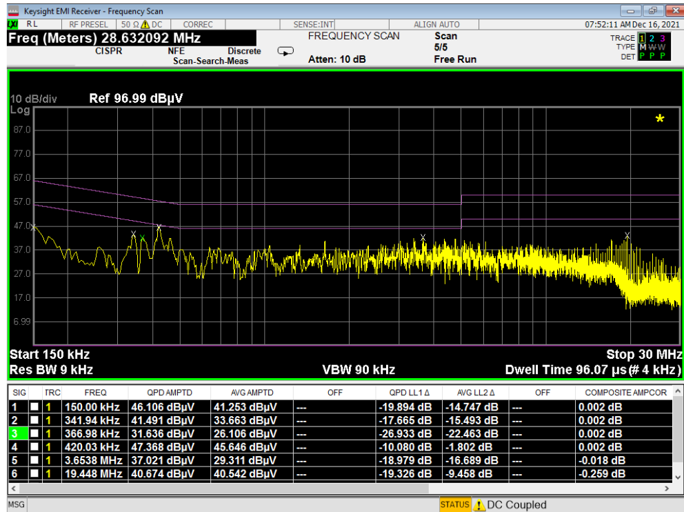
Plot 7-17. Line-Conducted Test Plot (N) - Device to Device – Config 1
