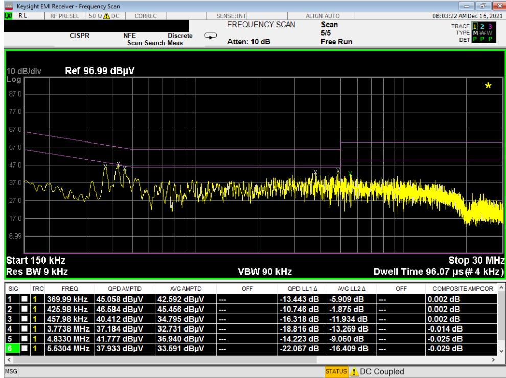
Plot 7-20. Line-Conducted Test Plot (L1) - Device to S-Pen
