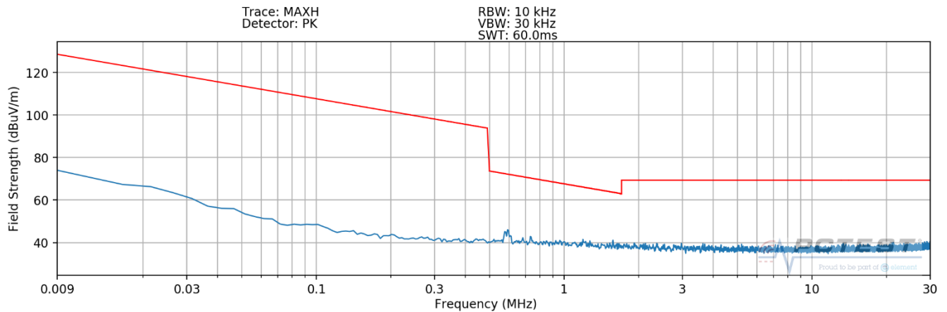
Plot 7-7. Radiated Spurious Plot 9kHz – 30MHz (Pol. X – Device to S-Pen)
