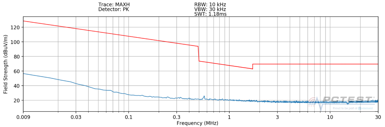
Plot 7-11. Radiated Spurious Plot 9kHz – 30MHz (Pol. Y – WPT – Digitizer Hover)
