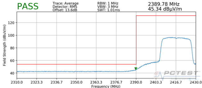
Plot 7-173. Radiated Restricted Lower Band Edge Measurement MIMO (Average)
