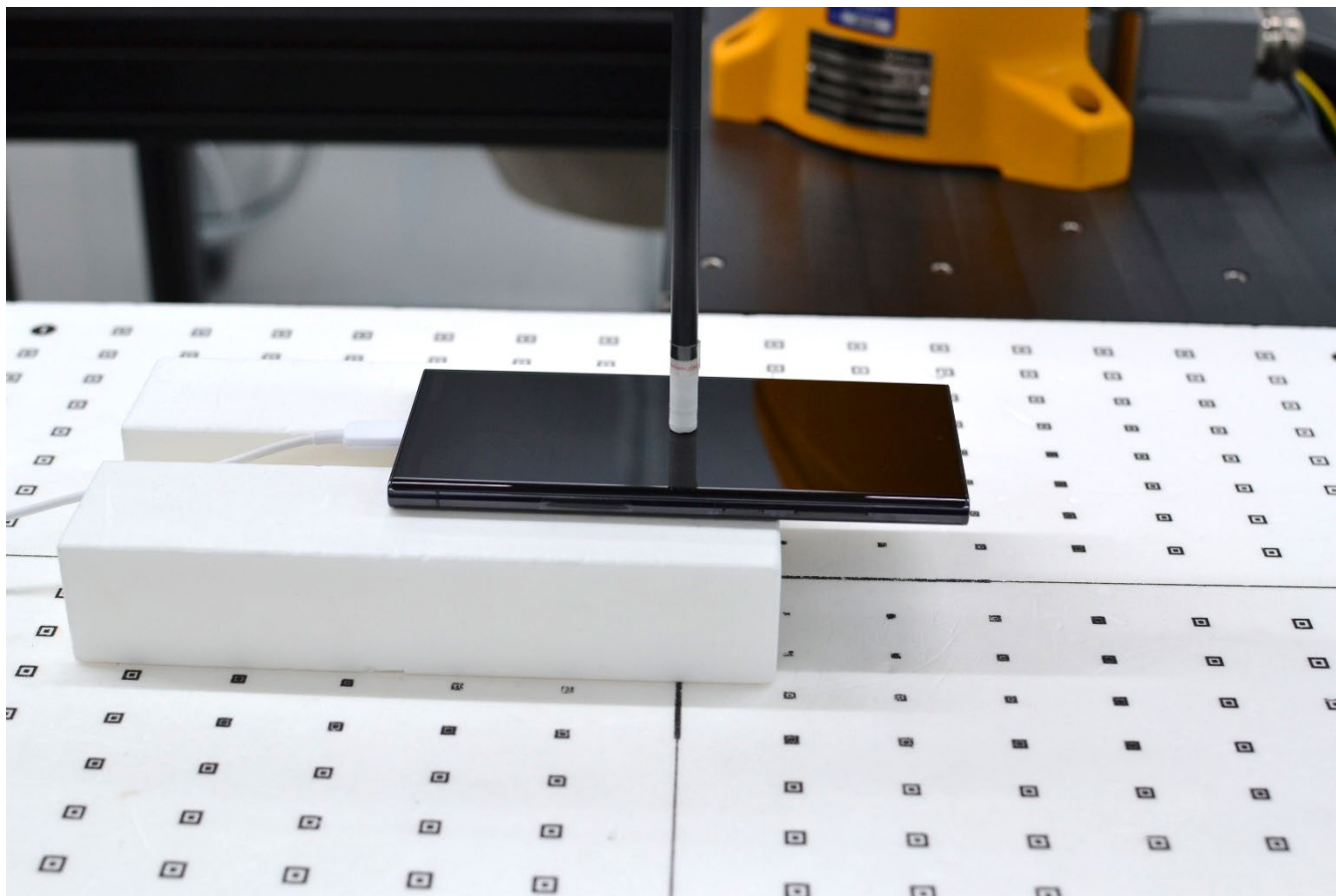
Figure C-14 Near Field Power Density Test Setup Photo – Front Side at 2 mm
