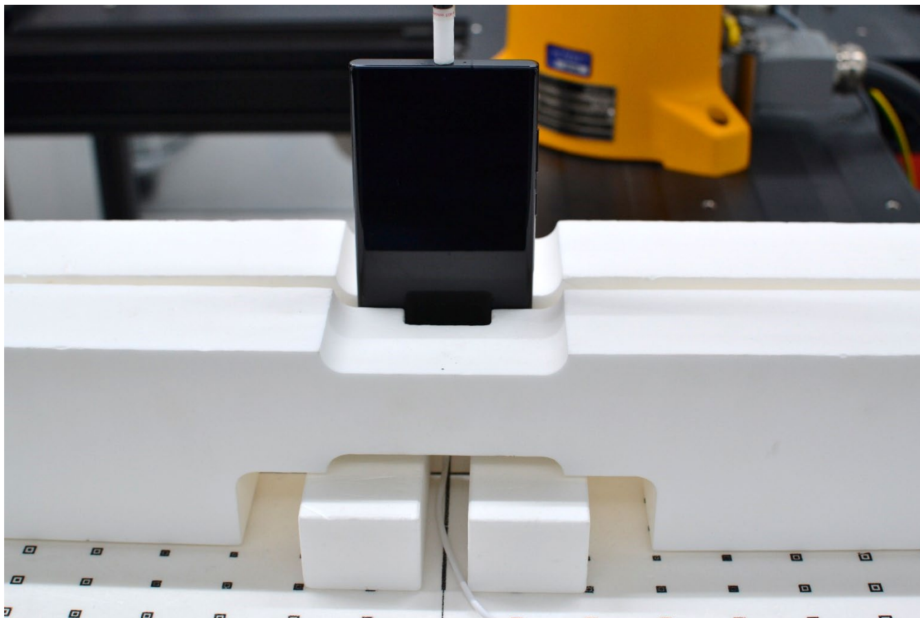
Figure C-16 Near Field Power Density Test Setup Photo – Top Edge at 2 mm
