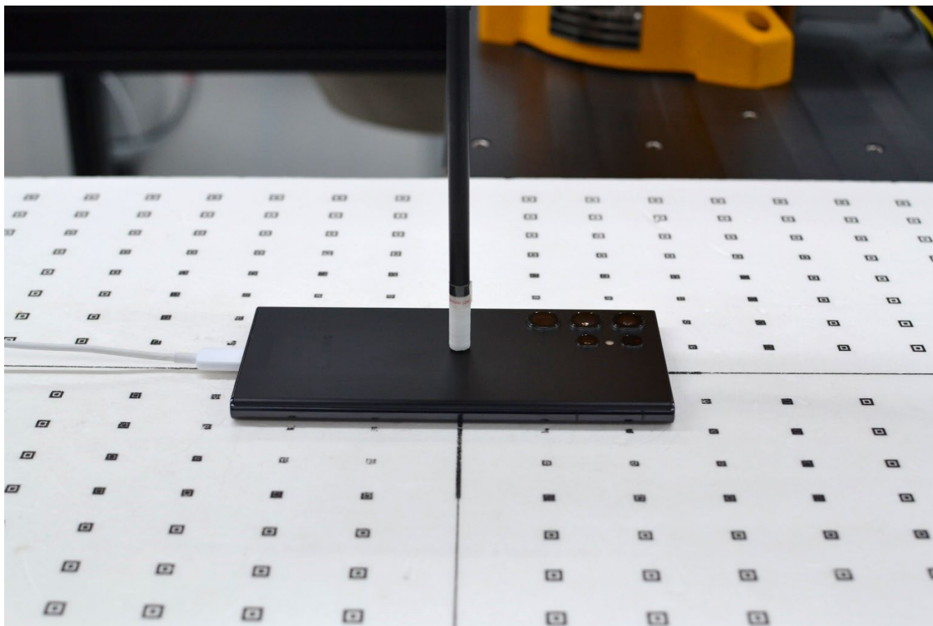
Figure C-13 Near Field Power Density Test Setup Photo – Back Side at 2 mm
