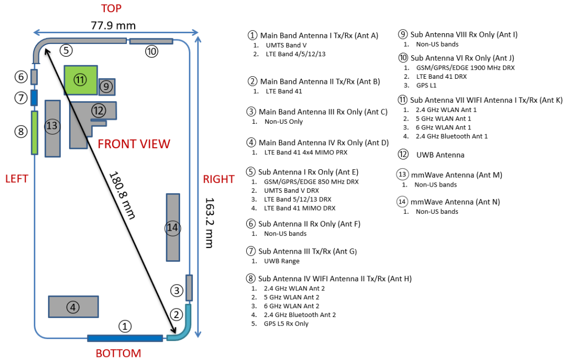
Figure C-1 DUT Antenna Locations
