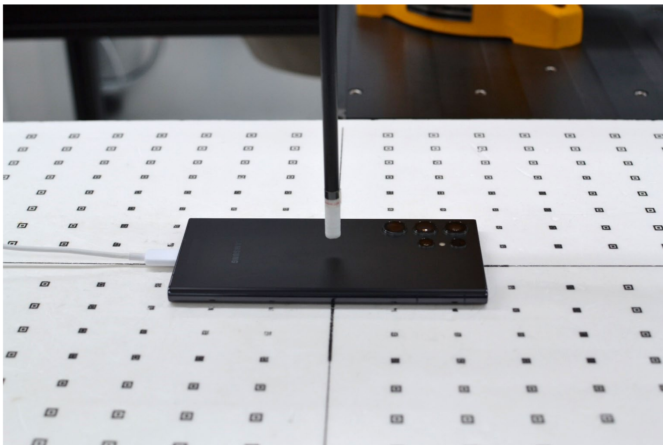
Figure C-17 Near Field Power Density Test Setup Photo – Back Side at 9.51 mm
