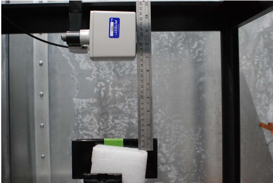
Test Setup Photo 29 E-field, Right edge, 15cm
