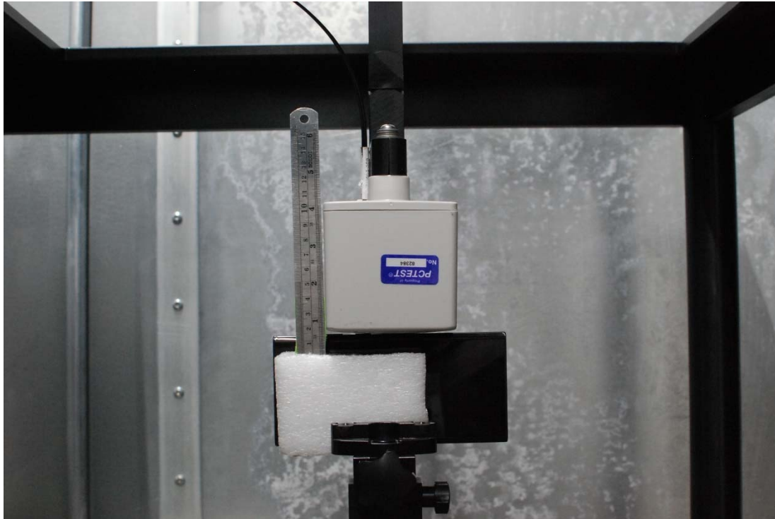
Test Setup Photo 41 H-field, Right edge, 0cm
