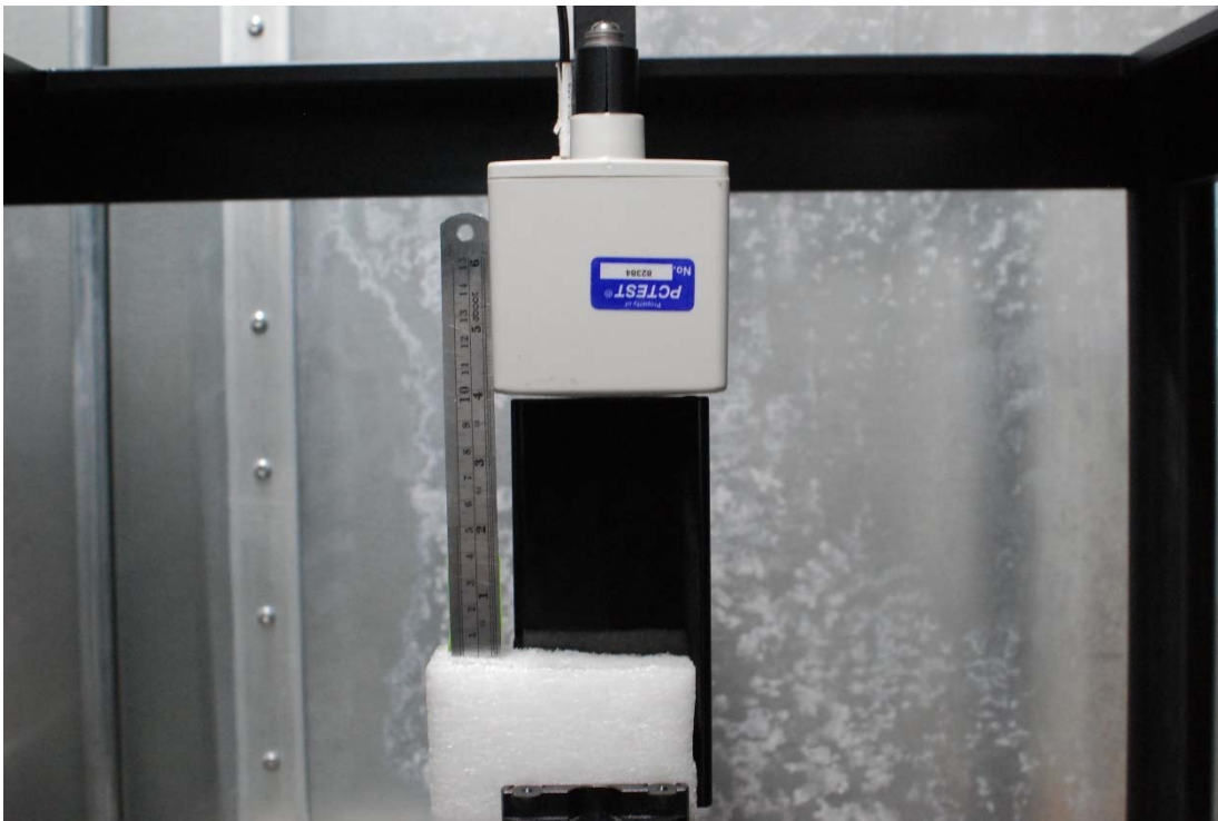
Test Setup Photo 40 H-field, Bottom edge, 0cm
