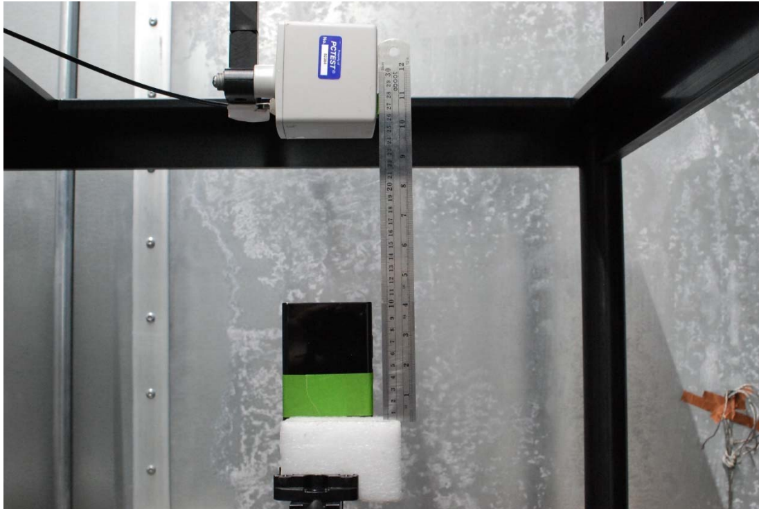
Test Setup Photo 15 E-field, Top edge, 15cm
