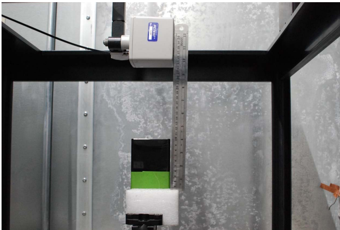
Test Setup Photo 16 E-field, Bottom edge, 15cm
