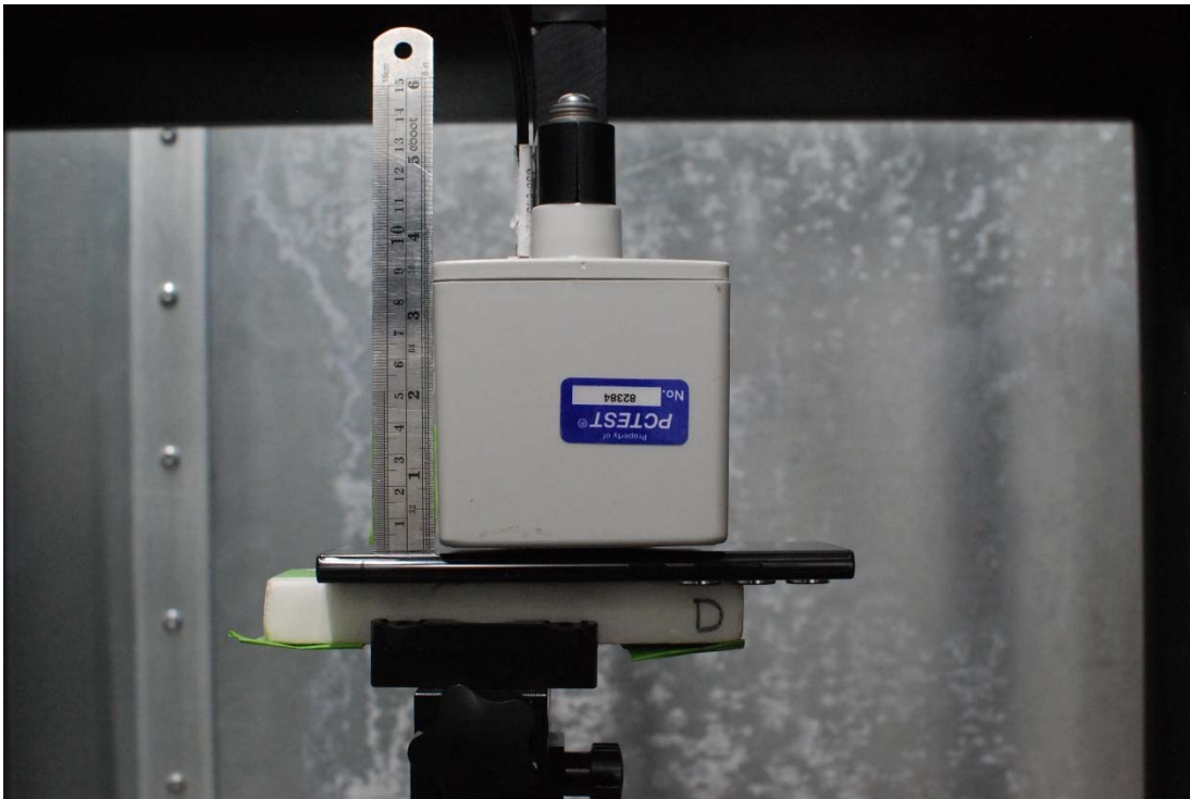
Test Setup Photo 38 H-field, Front side, 0cm
