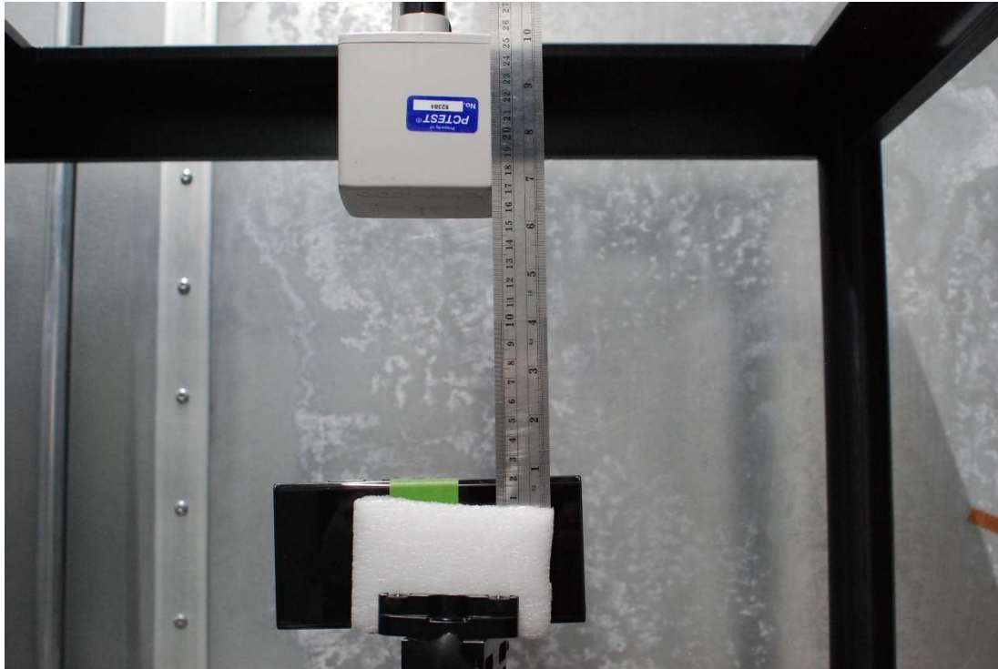
Test Setup Photo 35 H-field, Right edge, 15cm
