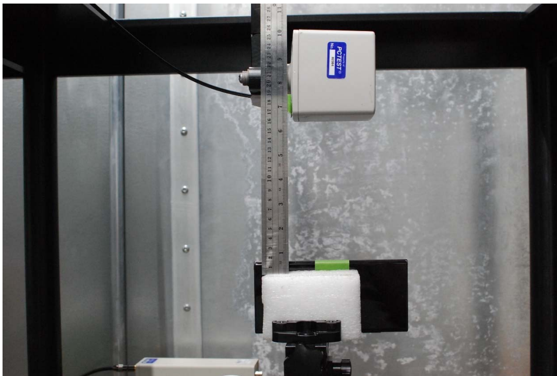
Test Setup Photo 30 E-field, Left edge, 15cm
