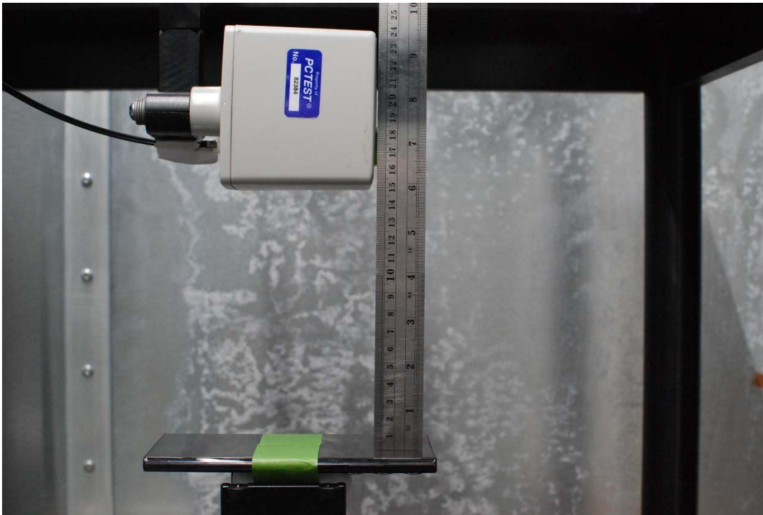
Test Setup Photo 26 E-field, Front side, 15cm
