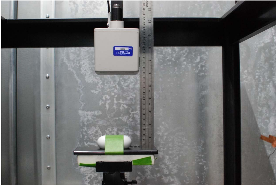
Test Setup Photo 31 H-field, Back side, 15cm
