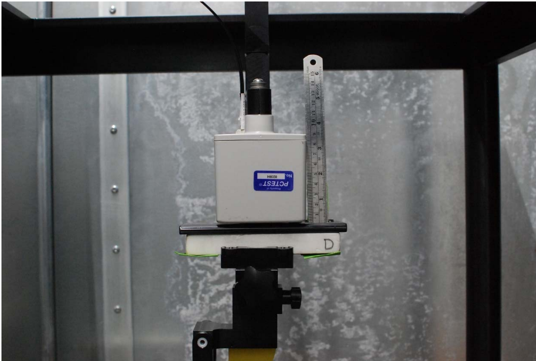
Test Setup Photo 37 H-field, Back side, 0cm
