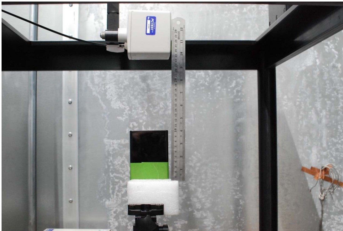
Test Setup Photo 28 E-field, Bottom edge, 15cm
