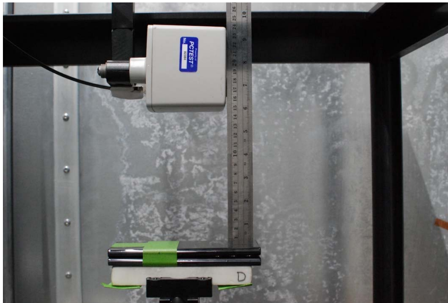
Test Setup Photo 2 E-field, Front side, 15cm
