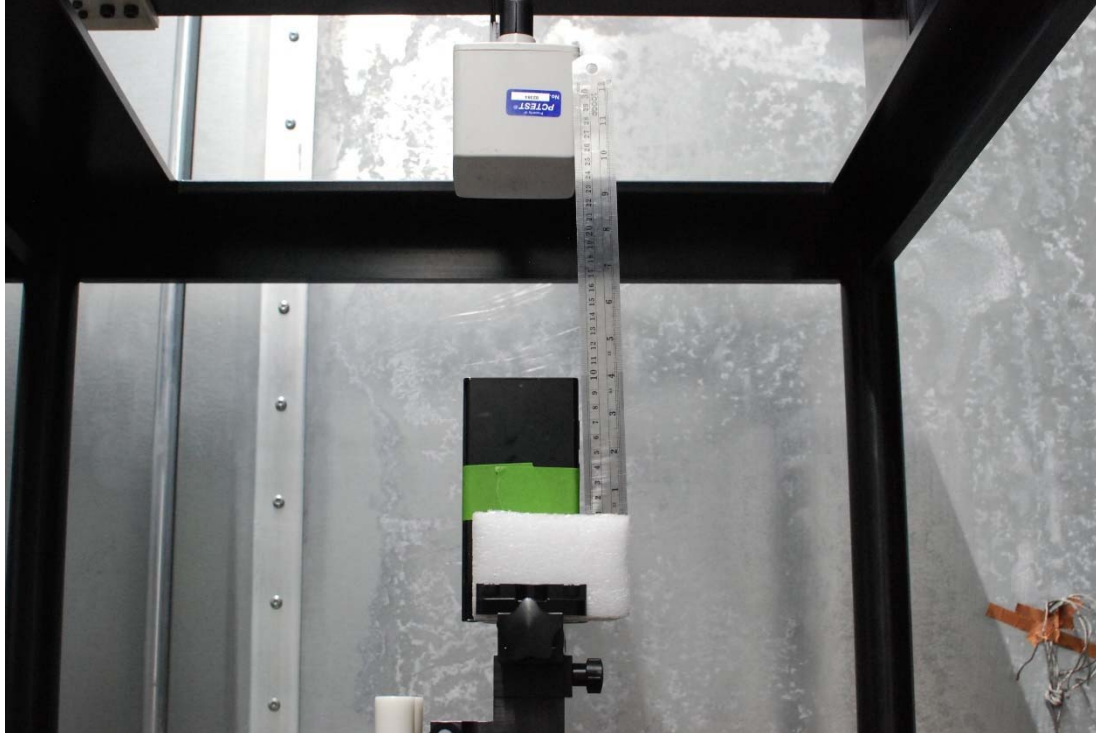
Test Setup Photo 33 H-field, Top edge, 15cm
