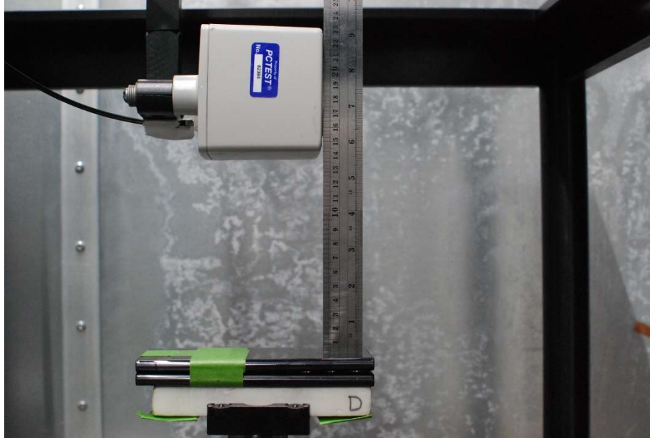
Test Setup Photo 1 E-field, Back side, 15cm
