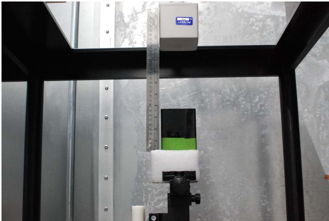
Test Setup Photo 34 H-field, Bottom edge, 15cm
