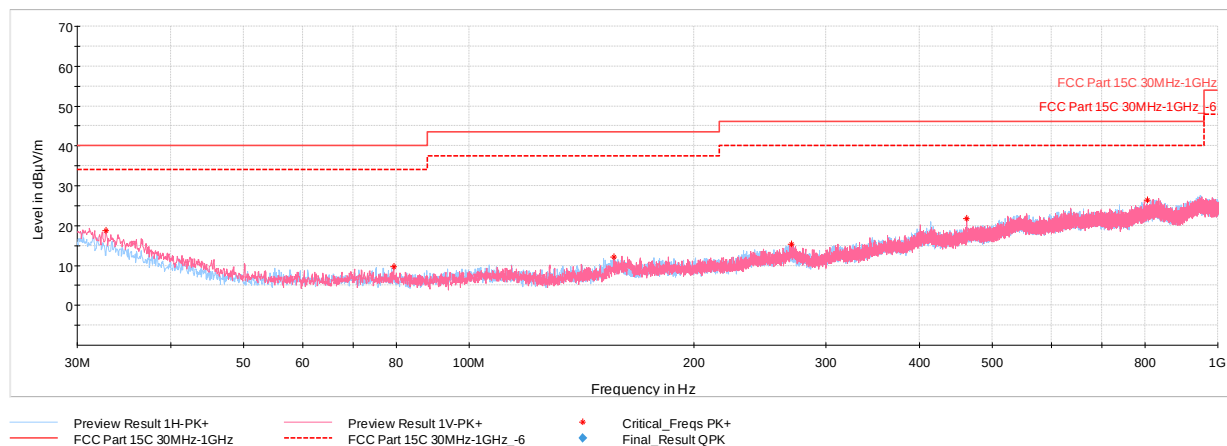
Plot 7-165. Radiated Spurious Emissions Below 1GHz (Antenna 2)
