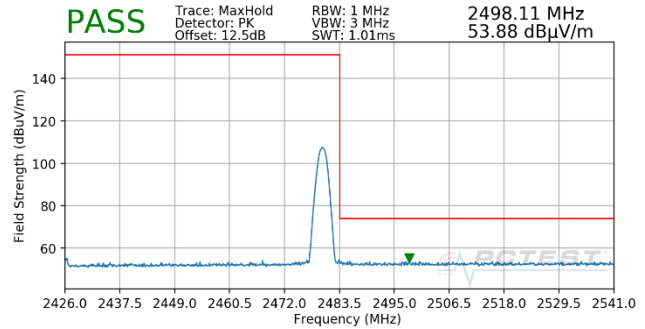
Plot 7-177. Radiated Restricted Upper Band Edge Measurement (Peak) – Dual
