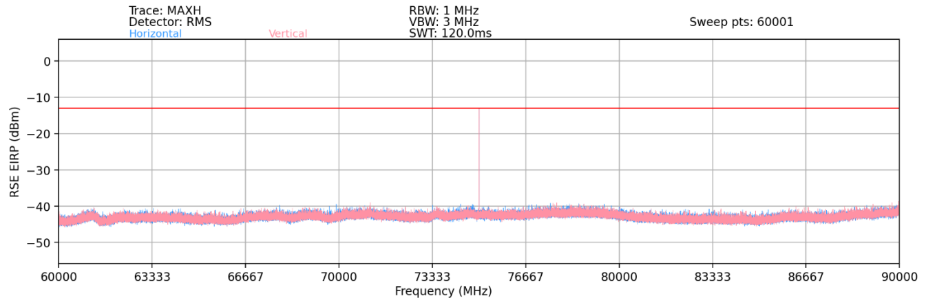
Plot 7-84. Ant1-n258-R2 Radiated Spurious Plot (1CC QPSK Mid Channel 2Tx – EN-DC Anchor B2)
