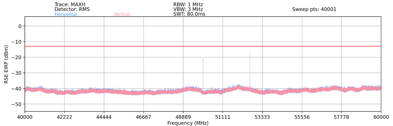
Plot 7-83. Ant1-n258-R2 Radiated Spurious Plot (1CC QPSK Mid Channel 2Tx – EN-DC Anchor B2)
