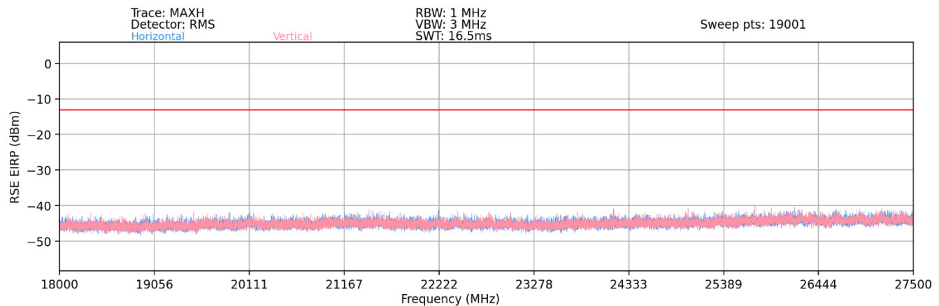
Plot 7-95. Ant1-n261 Radiated Spurious Plot (1CC QPSK Mid Channel 2Tx – EN-DC Anchor B2)
