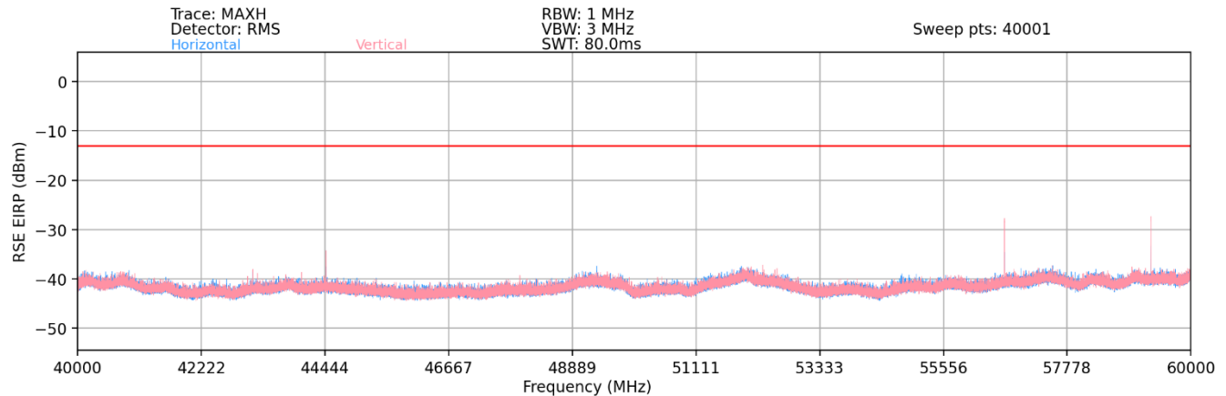
Plot 7-97. Ant1-n261 Radiated Spurious Plot (1CC QPSK Mid Channel 2Tx – EN-DC Anchor B2)
