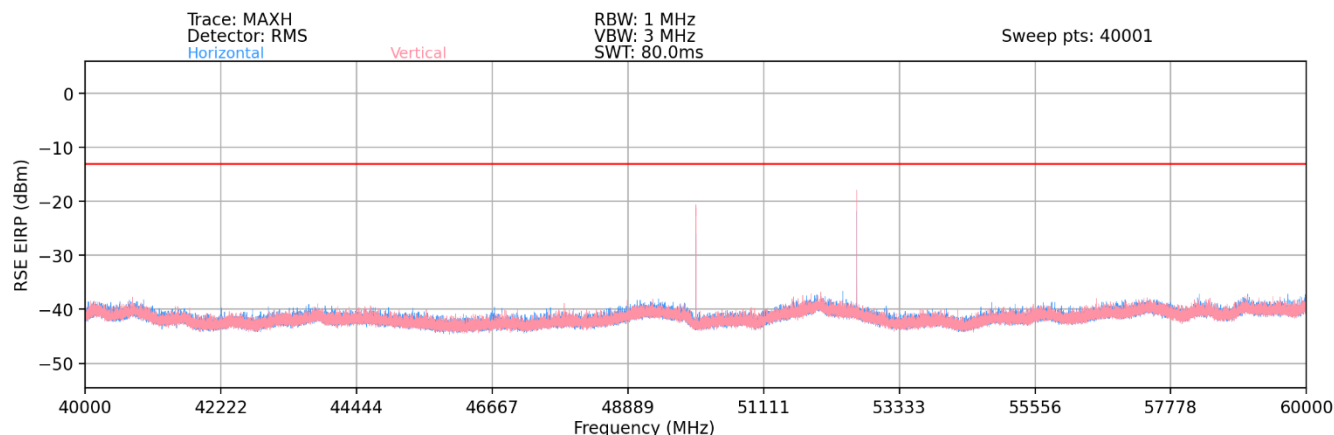
Plot 7-90. Ant2-n258-R2 Radiated Spurious Plot (1CC QPSK Mid Channel 2Tx – EN-DC Anchor B2)
