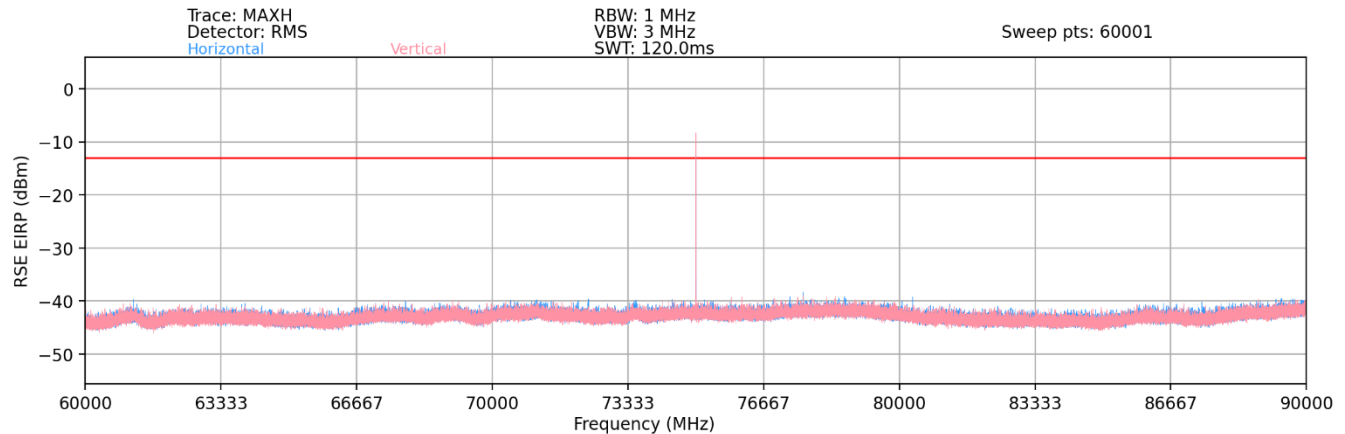
Plot 7-91. Ant2-n258-R2 Radiated Spurious Plot (1CC QPSK Mid Channel 2Tx – EN-DC Anchor B2)
