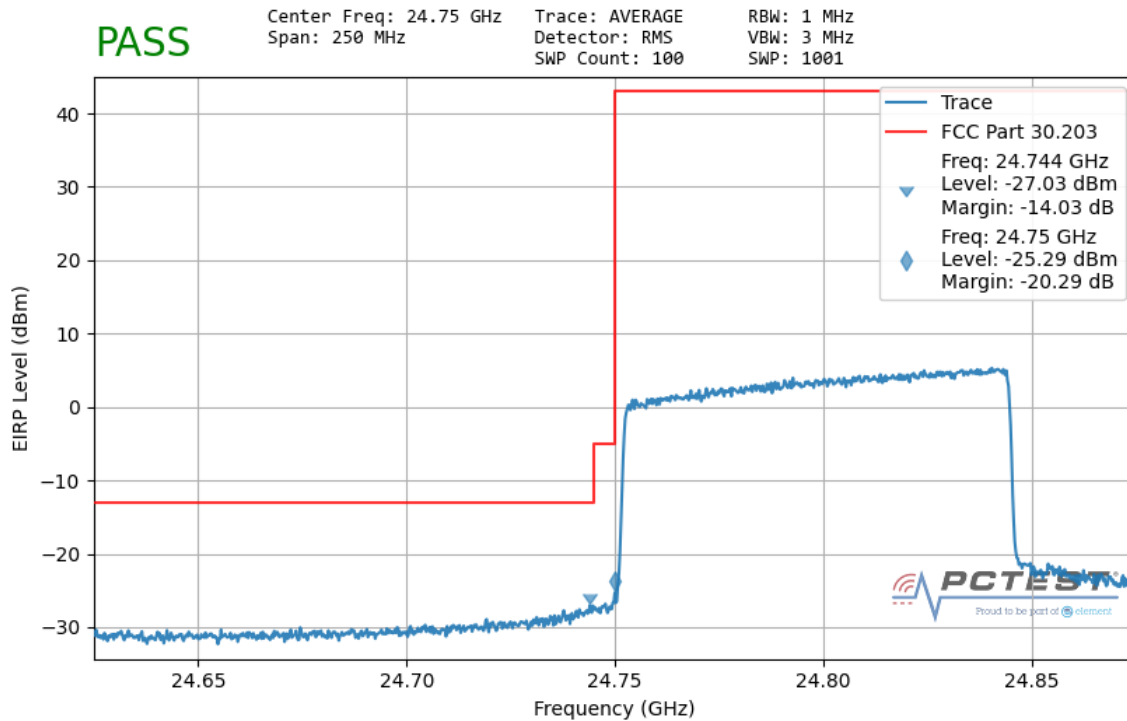
Plot 7-143. Ant1 Lower Band Edge (100MHz-1CC – QPSK Full RB)
