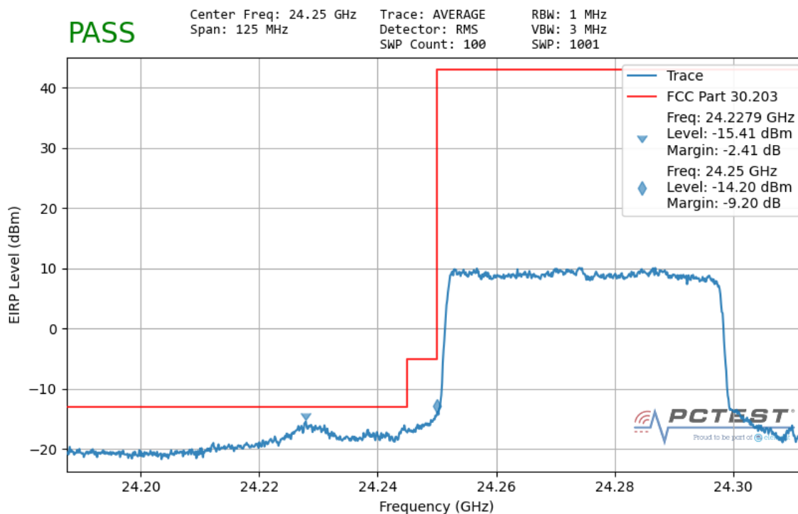
Plot 7-123. Ant1 Lower Band Edge (50MHz-1CC – \pi/2 -BPSK Full RB)
