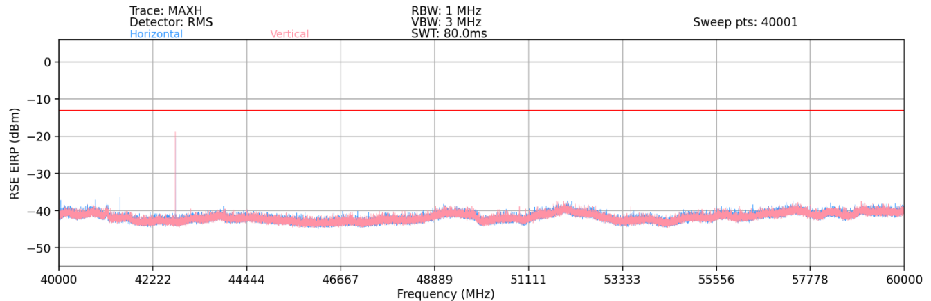
Plot 7-110. Ant1-n260 Radiated Spurious Plot (1CC QPSK Mid Channel 2Tx – EN-DC Anchor Band 2)
