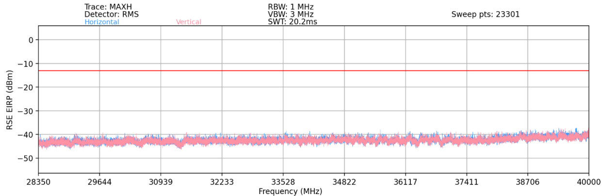
Plot 7-103. Ant2-n261 Radiated Spurious Plot (1CC QPSK Mid Channel 2Tx – EN-DC Anchor B2)
