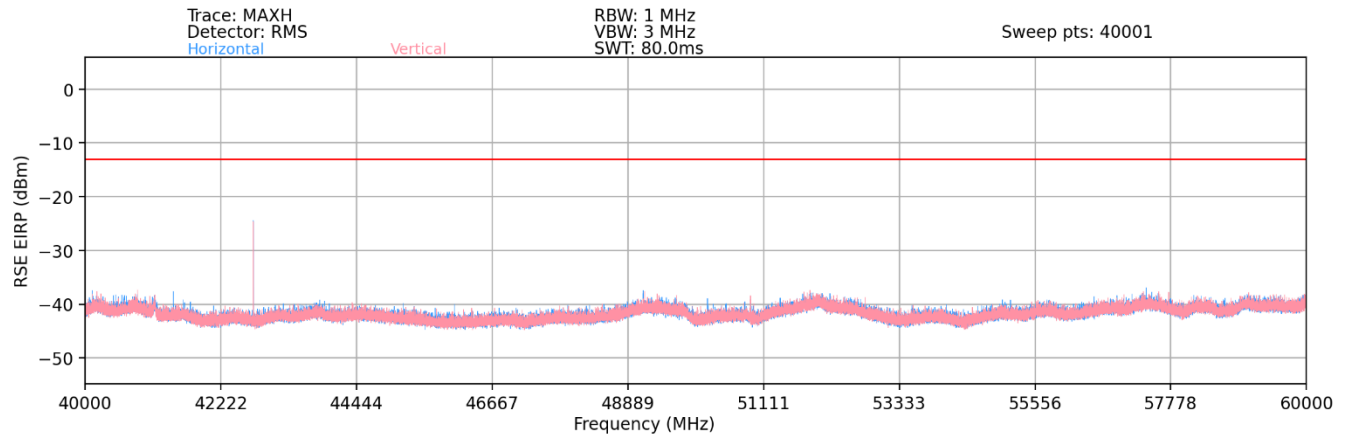
Plot 7-118. Ant2-n260 Radiated Spurious Plot (1CC QPSK Mid Channel 2Tx – EN-DC Anchor Band 2)
