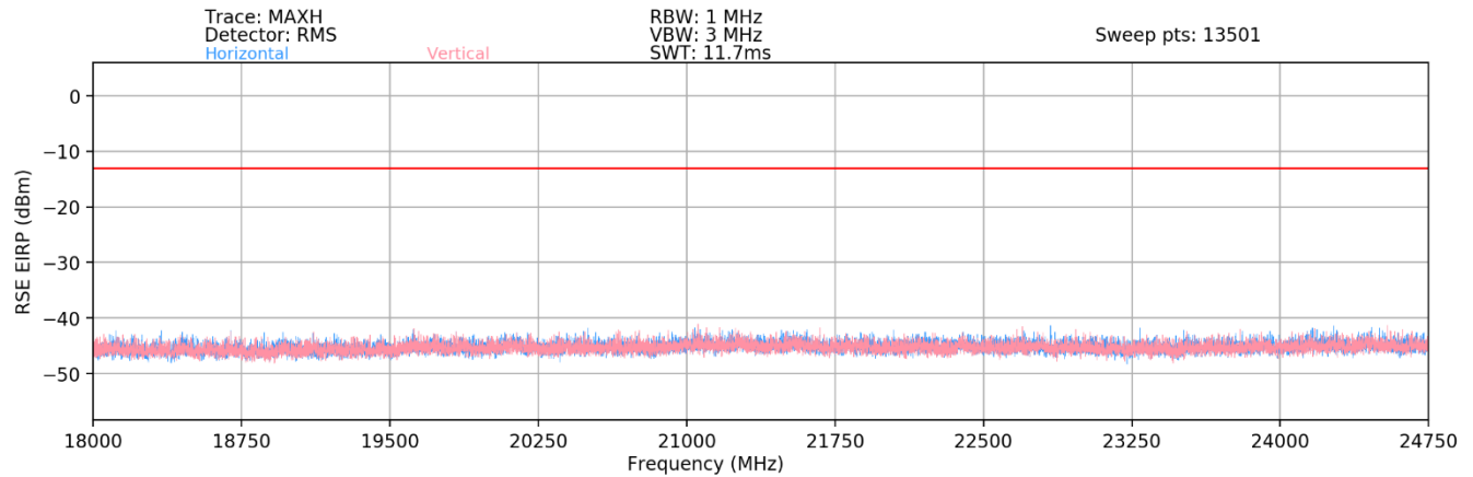
Plot 7-88. Ant2-n258-R2 Radiated Spurious Plot (1CC QPSK Mid Channel 2Tx – EN-DC Anchor B2)
