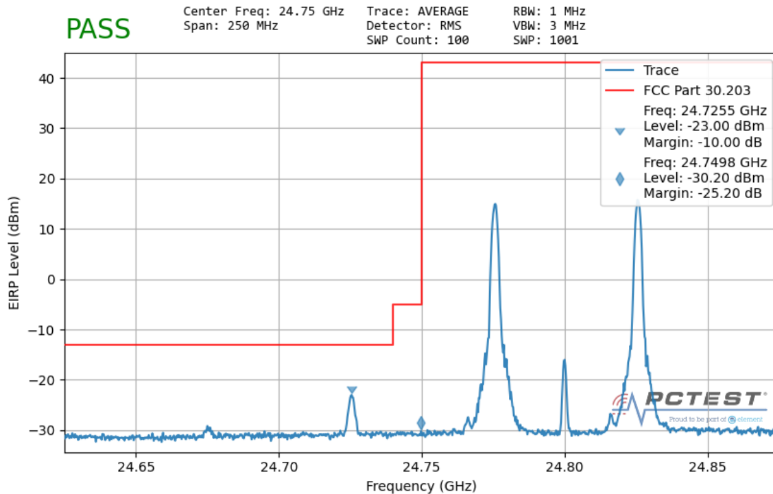
Plot 7-140. Ant1 Lower Band Edge (50MHz-2CC – QPSK 1 RB)
