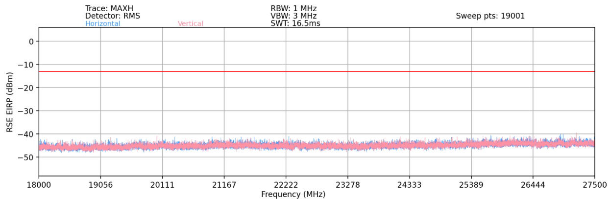
Plot 7-102. Ant2-n261 Radiated Spurious Plot (1CC QPSK Mid Channel 2Tx – EN-DC Anchor B2)
