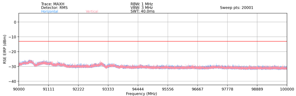
Plot 7-106. Ant2-n261 Radiated Spurious Plot (1CC QPSK Mid Channel 2Tx – EN-DC Anchor B2)
