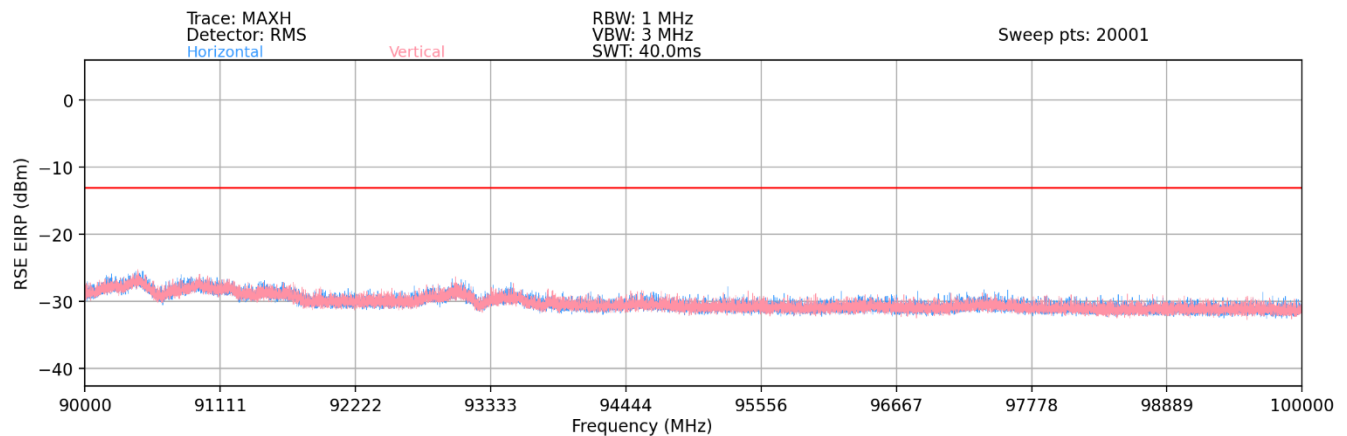
Plot 7-85. Ant1-n258-R2 Radiated Spurious Plot (1CC QPSK Mid Channel 2Tx – EN-DC Anchor B2)
