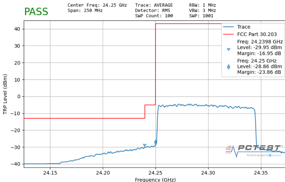
Plot 7-127. Ant1 Lower Band Edge – TRP (100MHz-1CC – QPSK Full RB)
