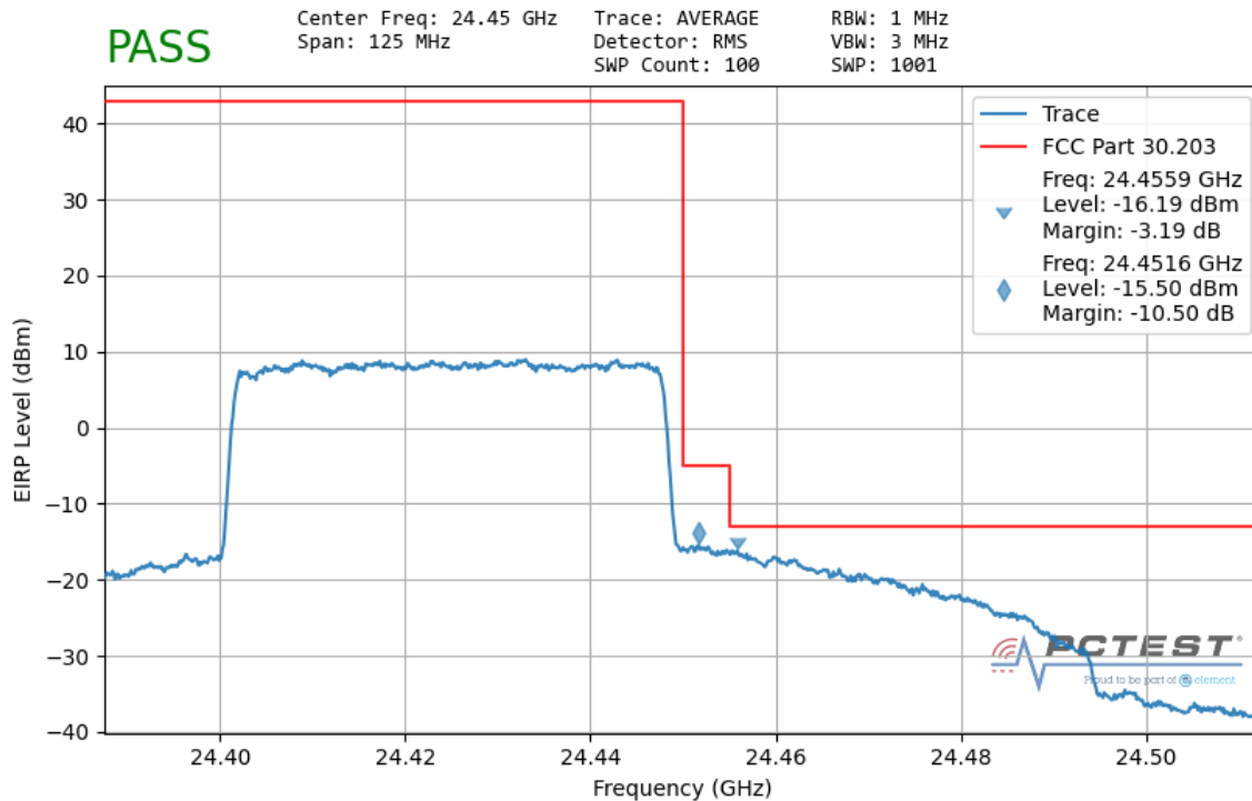
Plot 7-125. Ant1 Upper Band Edge (50MHz-1CC – QPSK Full RB)
