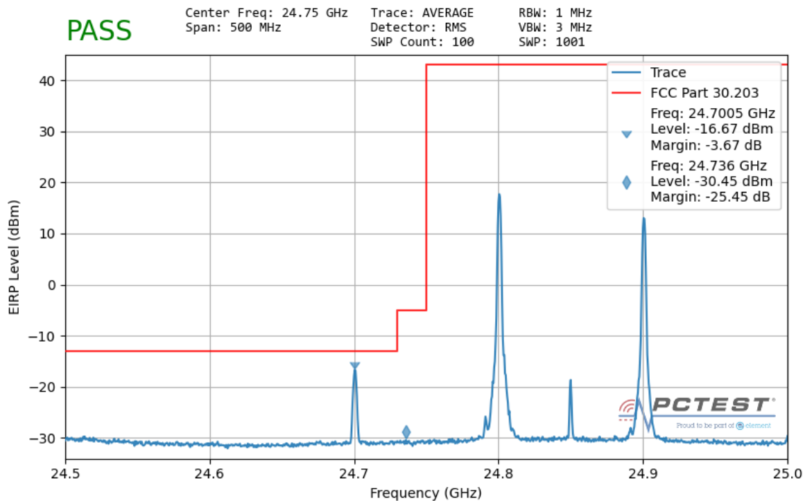
Plot 7-144. Ant1 Lower Band Edge (100MHz-2CC – QPSK 1 RB)
