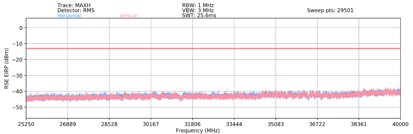
Plot 7-89. Ant2-n258-R2 Radiated Spurious Plot (1CC QPSK Mid Channel 2Tx – EN-DC Anchor B2)
