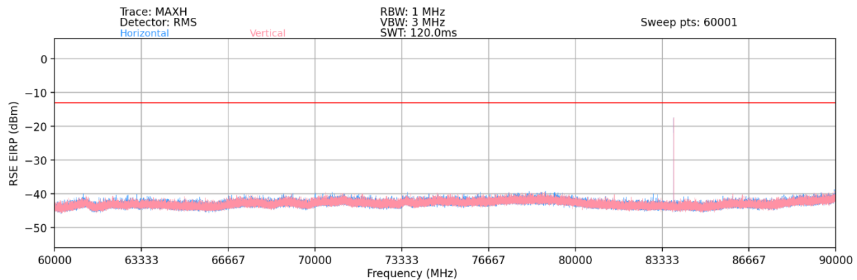
Plot 7-105. Ant2-n261 Radiated Spurious Plot (1CC QPSK Mid Channel 2Tx – EN-DC Anchor B2)
