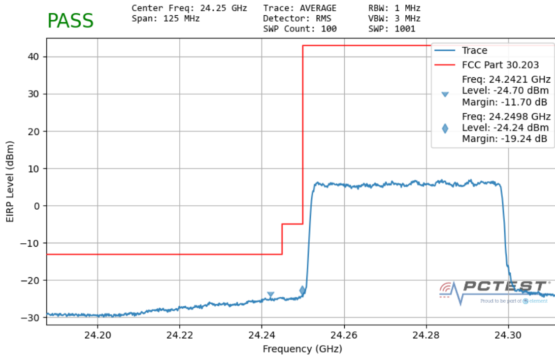
Plot 7-131. Ant2 Lower Band Edge (50MHz-1CC – QPSK Full RB)
