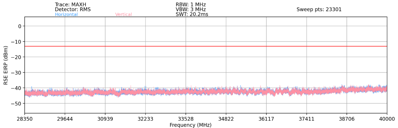
Plot 7-96. Ant1-n261 Radiated Spurious Plot (1CC QPSK Mid Channel 2Tx – EN-DC Anchor B2)
