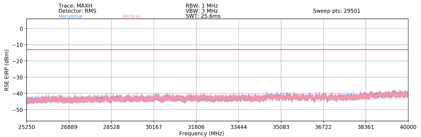
Plot 7-82. Ant1-n258-R2 Radiated Spurious Plot (1CC QPSK Mid Channel 2Tx – EN-DC Anchor B2)
