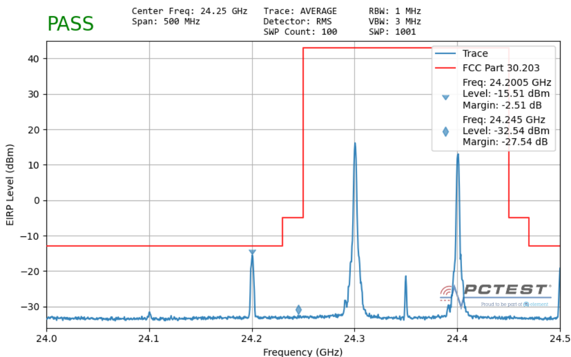
Plot 7-128. Ant1 Lower Band Edge (100MHz-2CC – QPSK 1 RB)
