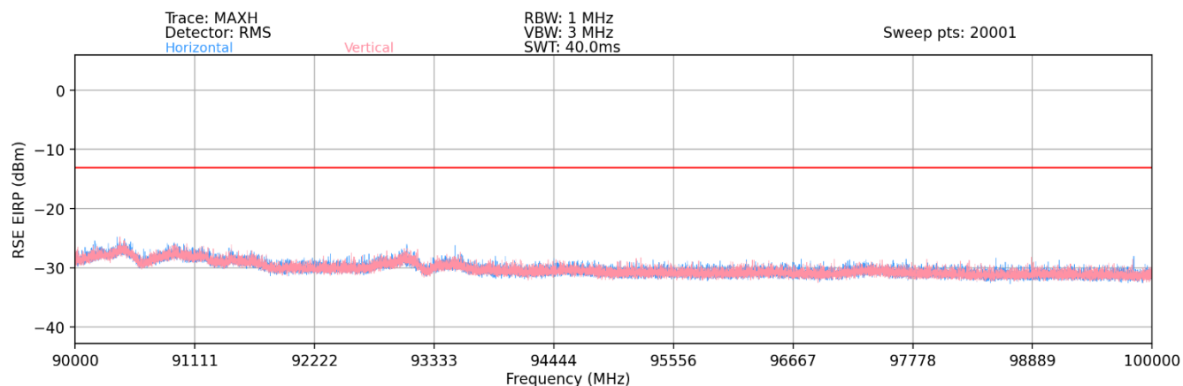
Plot 7-99. Ant1-n261 Radiated Spurious Plot (1CC QPSK Mid Channel 2Tx – EN-DC Anchor B2)
