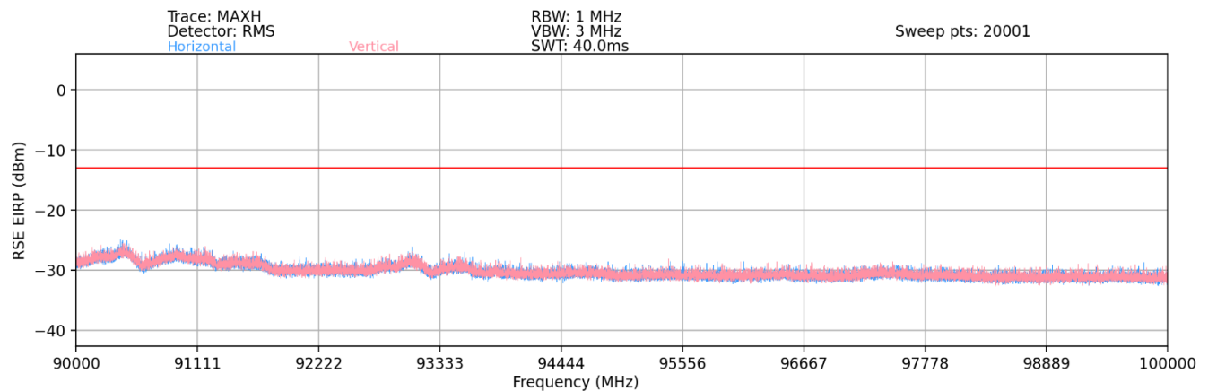
Plot 7-92. Ant2-n258-R2 Radiated Spurious Plot (1CC QPSK Mid Channel 2Tx – EN-DC Anchor B2)
