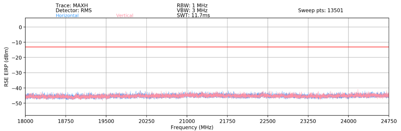
Plot 7-81. Ant1-n258-R2 Radiated Spurious Plot (1CC QPSK Mid Channel 2Tx – EN-DC Anchor B2)
