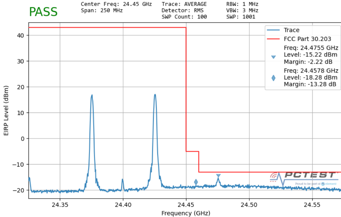
Plot 7-126. Ant1 Upper Band Edge (50MHz-2CC – QPSK 1 RB)
