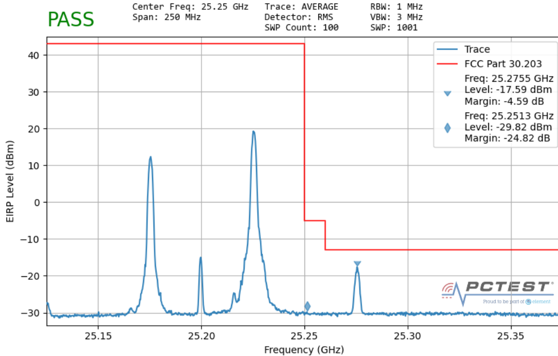
Plot 7-142. Ant1 Upper Band Edge (50MHz-2CC – QPSK 1 RB)
