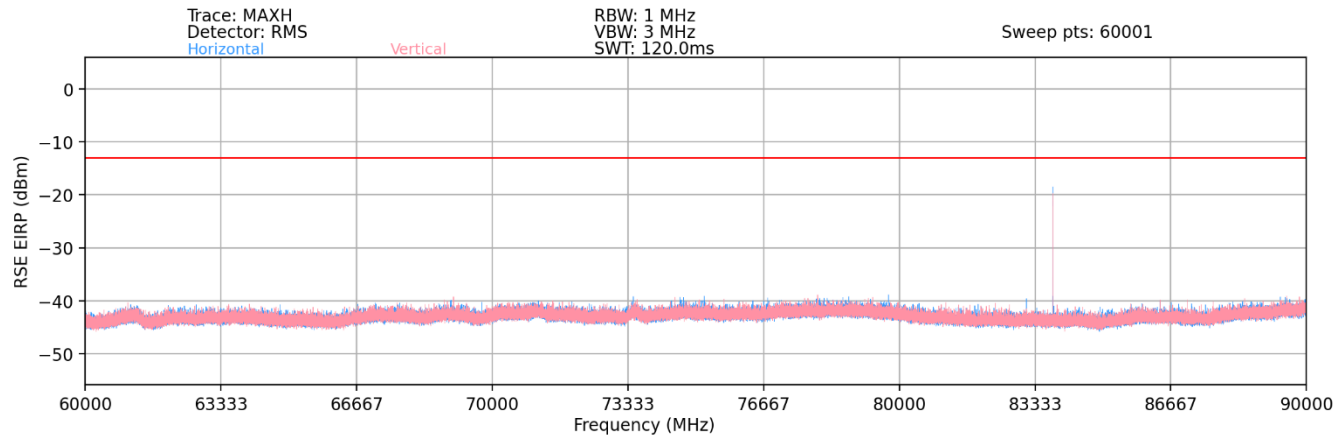
Plot 7-98. Ant1-n261 Radiated Spurious Plot (1CC QPSK Mid Channel 2Tx – EN-DC Anchor B2)
