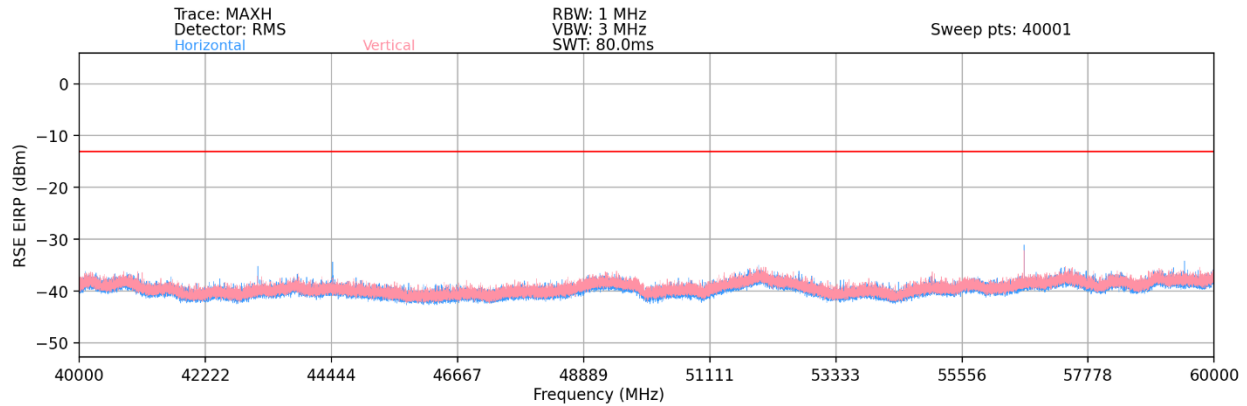
Plot 7-104. Ant2-n261 Radiated Spurious Plot (1CC QPSK Mid Channel 2Tx – EN-DC Anchor B2)
