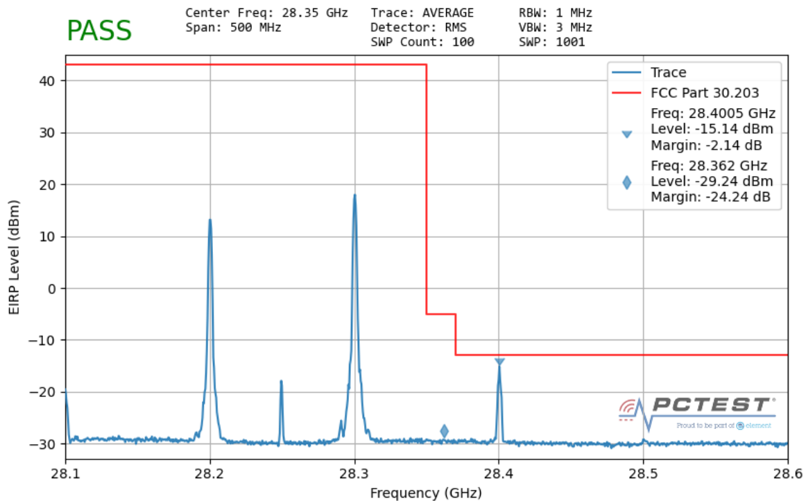
Plot 7-170. Ant2 Upper Band Edge (100MHz-2CC – QPSK 1 RB)
