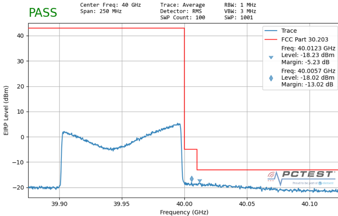
Plot 7-177. Ant1 Upper Band Edge (100MHz-1CC – QPSK Full RB)
