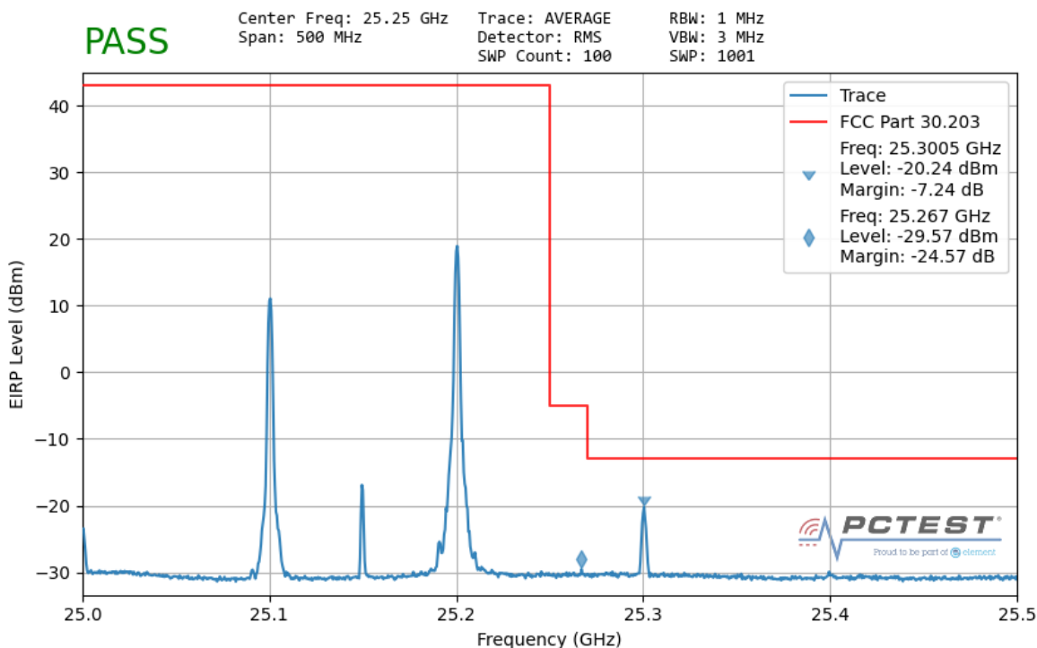
Plot 7-146. Ant1 Upper Band Edge (100MHz-2CC – QPSK 1 RB)
