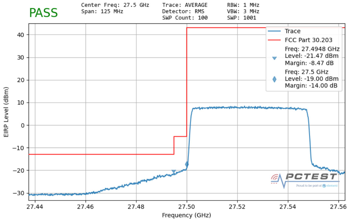
Plot 7-163. Ant2 Lower Band Edge (50MHz-1CC – \pi/2 -BPSK Full RB)
