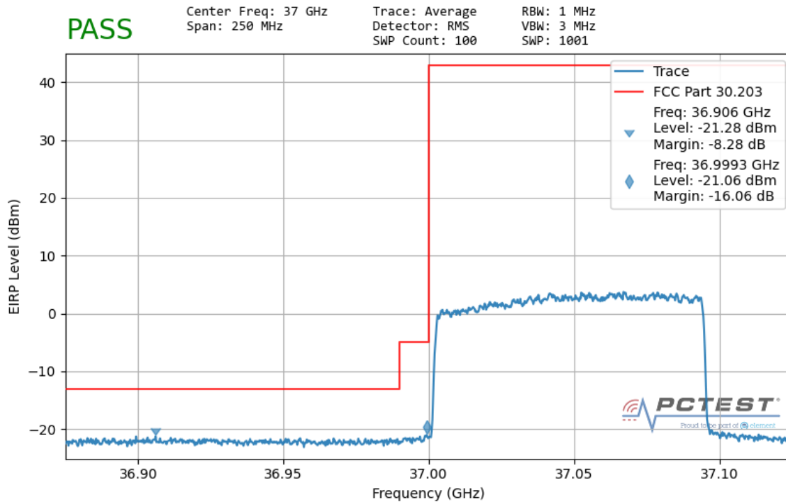
Plot 7-175. Ant1 Lower Band Edge (100MHz-1CC – QPSK Full RB)
