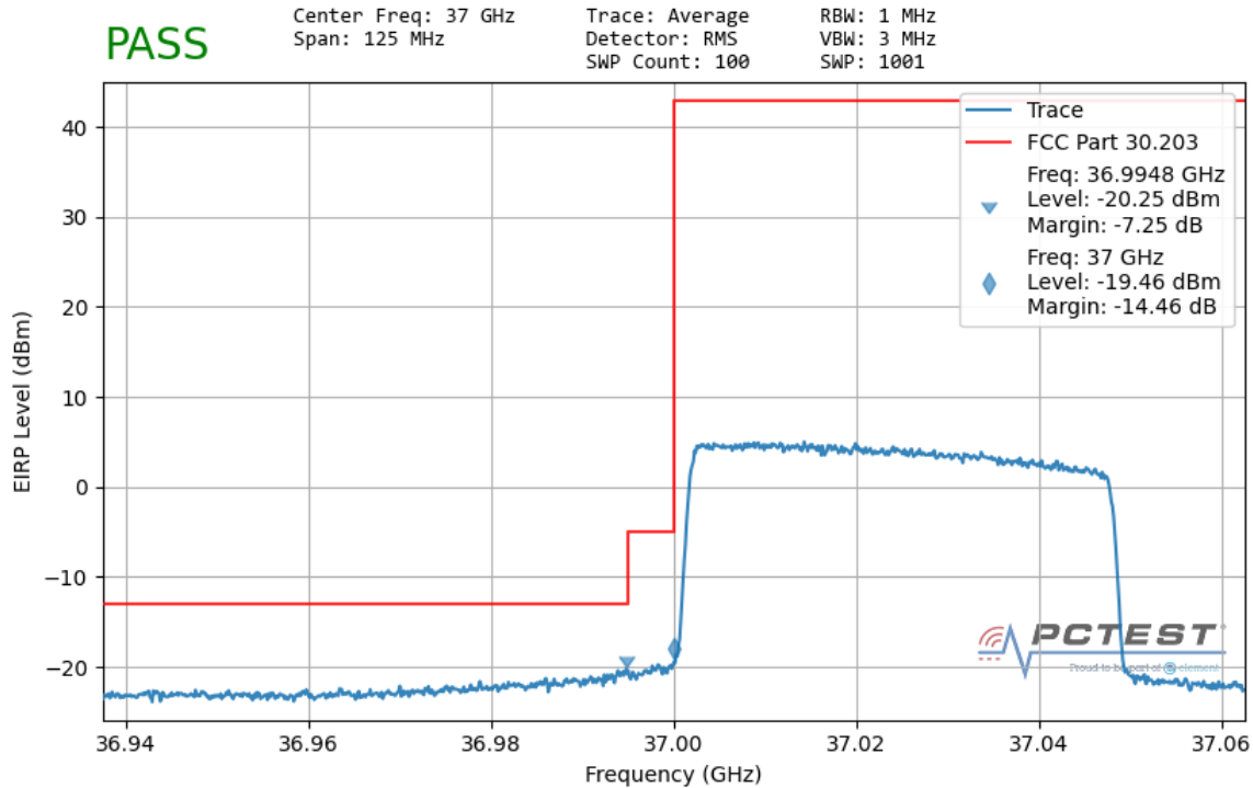
Plot 7-171. Ant1 Lower Band Edge (50MHz-1CC – QPSK Full RB)
