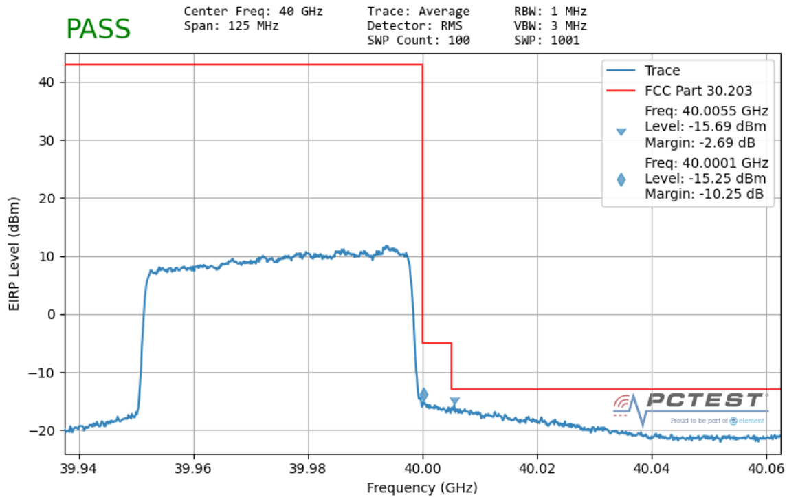
Plot 7-173. Ant1 Upper Band Edge (50MHz-1CC – QPSK Full RB)
