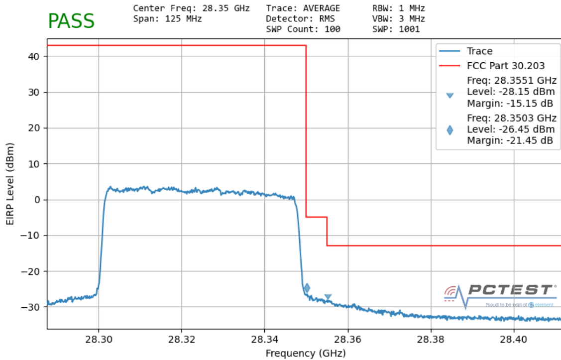
Plot 7-157. Ant1 Upper Band Edge (50MHz-1CC – QPSK Full RB)
