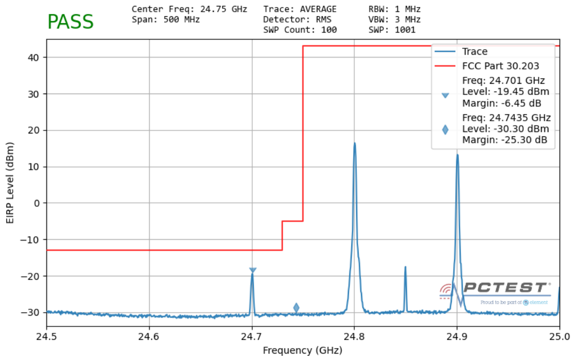
Plot 7-152. Ant2 Lower Band Edge – TRP (100MHz-2CC – QPSK 1 RB)
