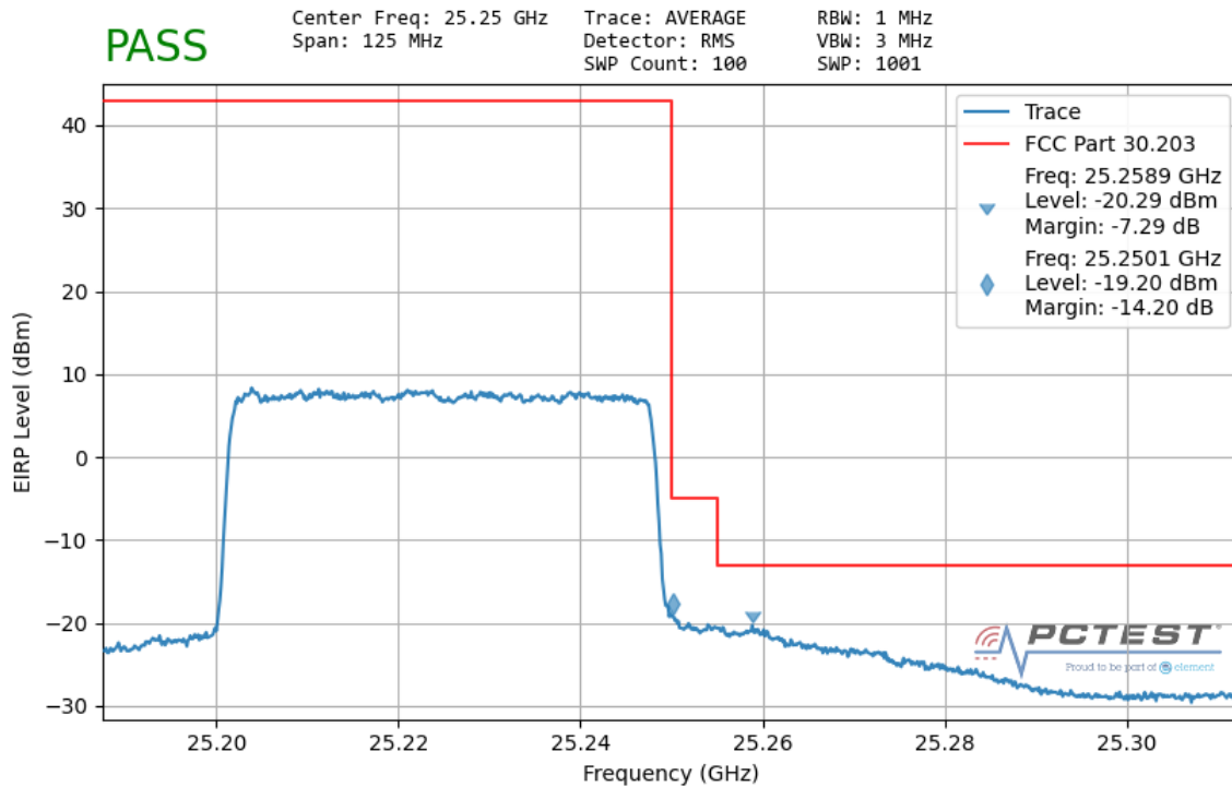
Plot 7-149. Ant2 Upper Band Edge (50MHz-1CC – QPSK Full RB)
