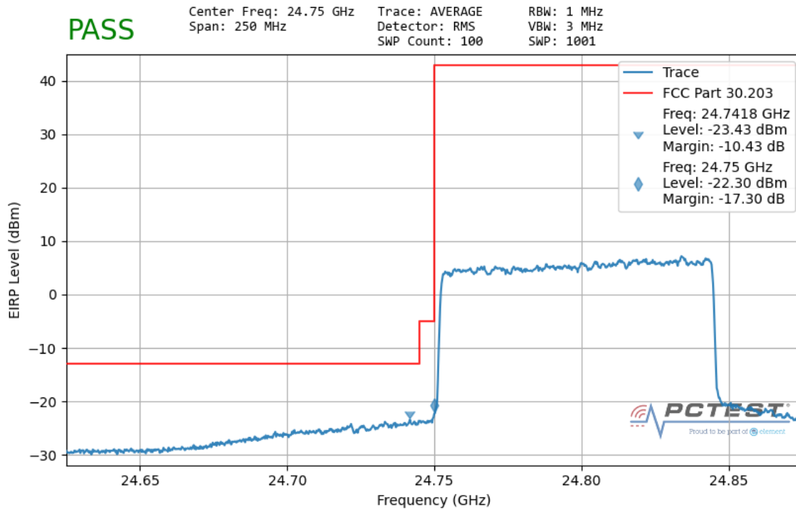
Plot 7-151. Ant2 Lower Band Edge (100MHz-1CC – QPSK Full RB)
