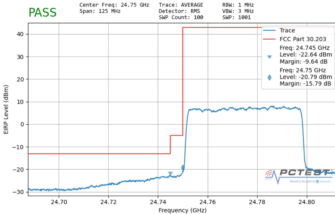
Plot 7-147. Ant2 Lower Band Edge (50MHz-1CC – \pi/2 -BPSK Full RB)
