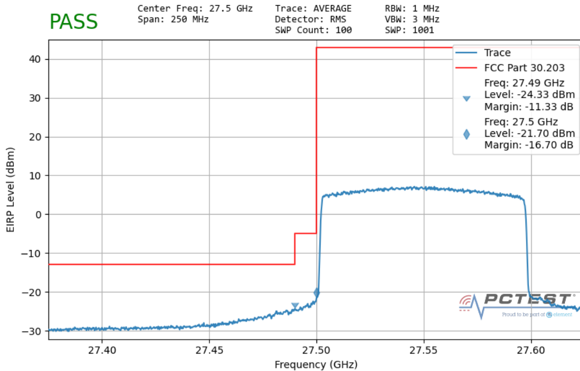
Plot 7-167. Ant2 Lower Band Edge (100MHz-1CC – QPSK Full RB)
