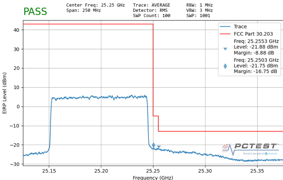
Plot 7-145. Ant1 Upper Band Edge (100MHz-1CC – QPSK Full RB)
