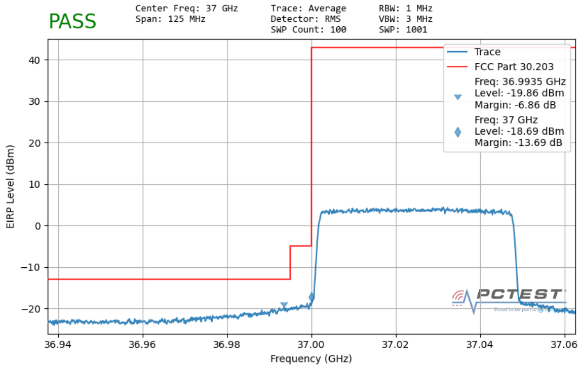
Plot 7-179. Ant2 Lower Band Edge (50MHz-1CC – \pi/2 -BPSK Full RB)
