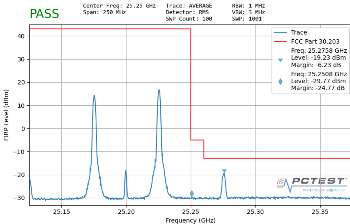
Plot 7-150. Ant2 Upper Band Edge (50MHz-2CC – QPSK 1 RB)
