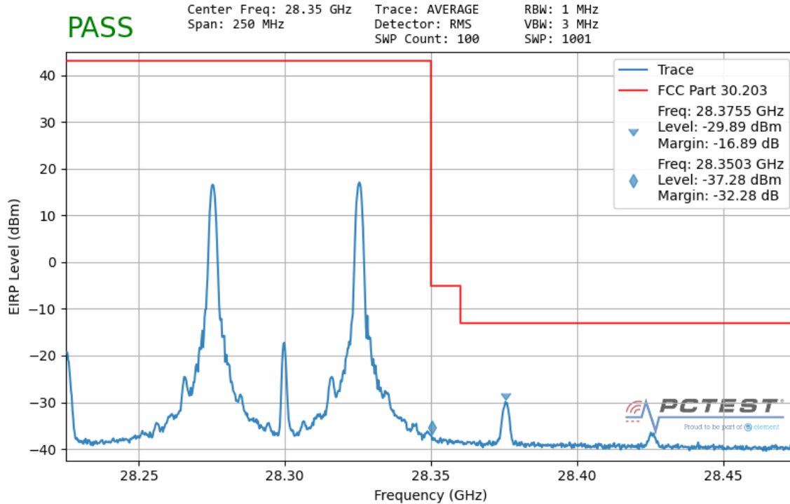
Plot 7-158. Ant1 Upper Band Edge (50MHz-2CC – QPSK 1 RB)
