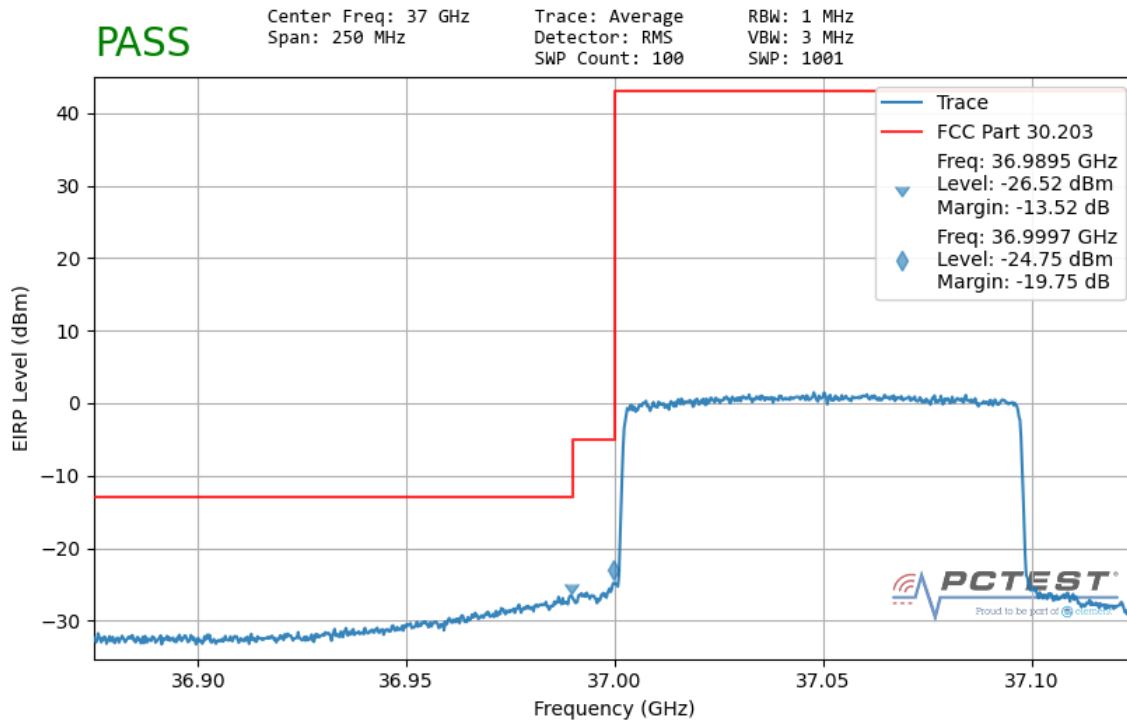
Plot 7-183. Ant2 Lower Band Edge (100MHz-1CC – QPSK Full RB)
