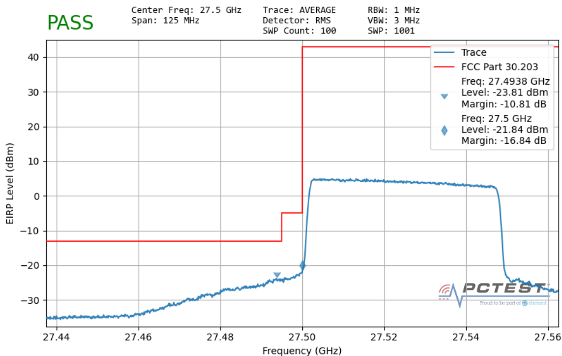
Plot 7-179. Ant1 Lower Band Edge (50MHz-1CC – QPSK Full RB)
