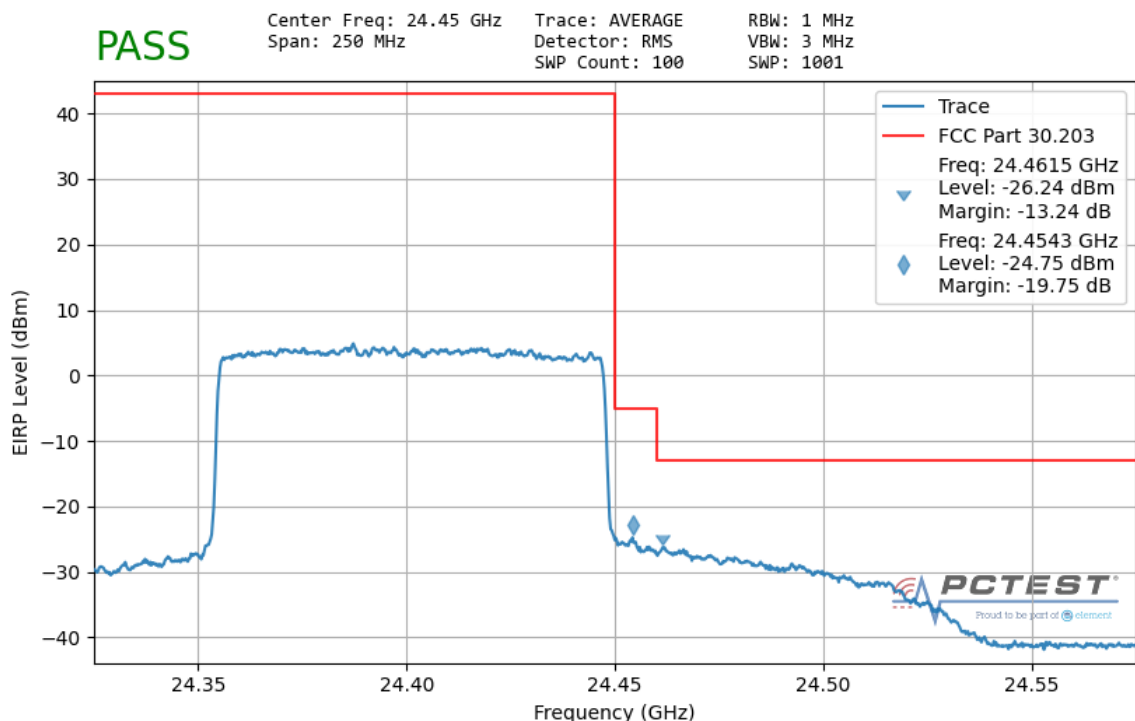
Plot 7-161. Ant2 Upper Band Edge (100MHz-1CC – QPSK Full RB)
