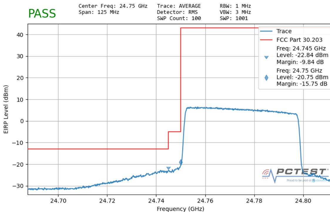
Plot 7-163. Ant1 Lower Band Edge (50MHz-1CC – QPSK Full RB)
