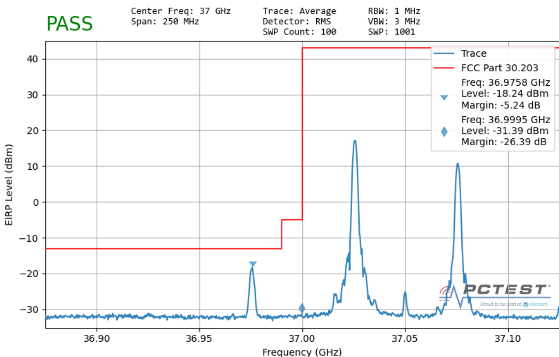
Plot 7-204. Ant2 Lower Band Edge (50MHz-2CC – QPSK 1 RB)
