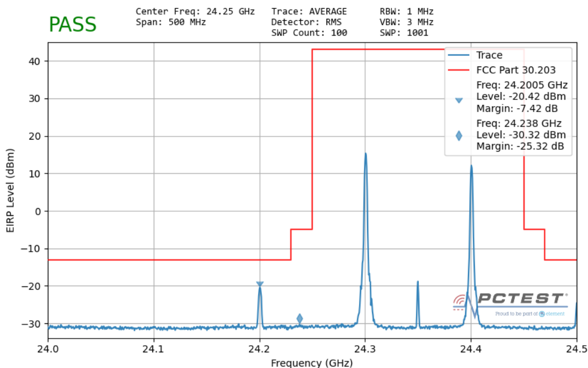
Plot 7-160. Ant2 Lower Band Edge – TRP (100MHz-2CC – QPSK 1 RB)
