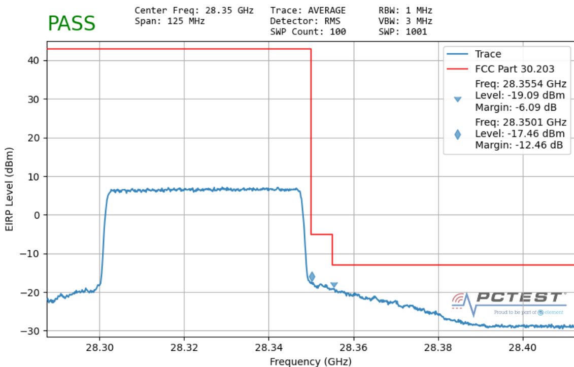
Plot 7-189. Ant2 Upper Band Edge (50MHz-1CC – QPSK Full RB)
