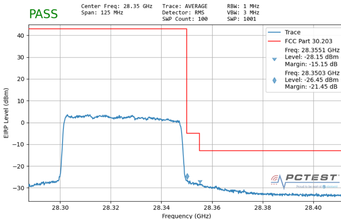
Plot 7-181. Ant1 Upper Band Edge (50MHz-1CC – QPSK Full RB)
