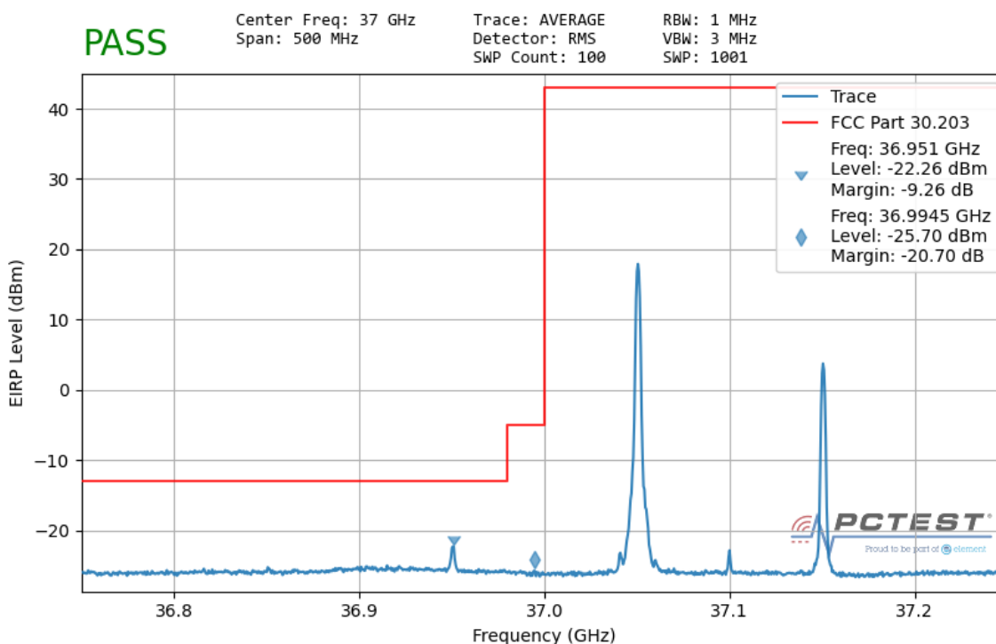
Plot 7-208. Ant2 Lower Band Edge – TRP (100MHz-2CC – QPSK 1 RB)
