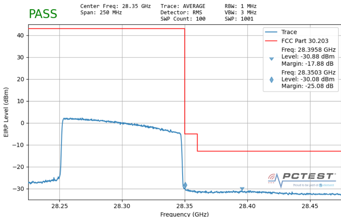
Plot 7-185. Ant1 Upper Band Edge (100MHz-1CC – QPSK Full RB)
