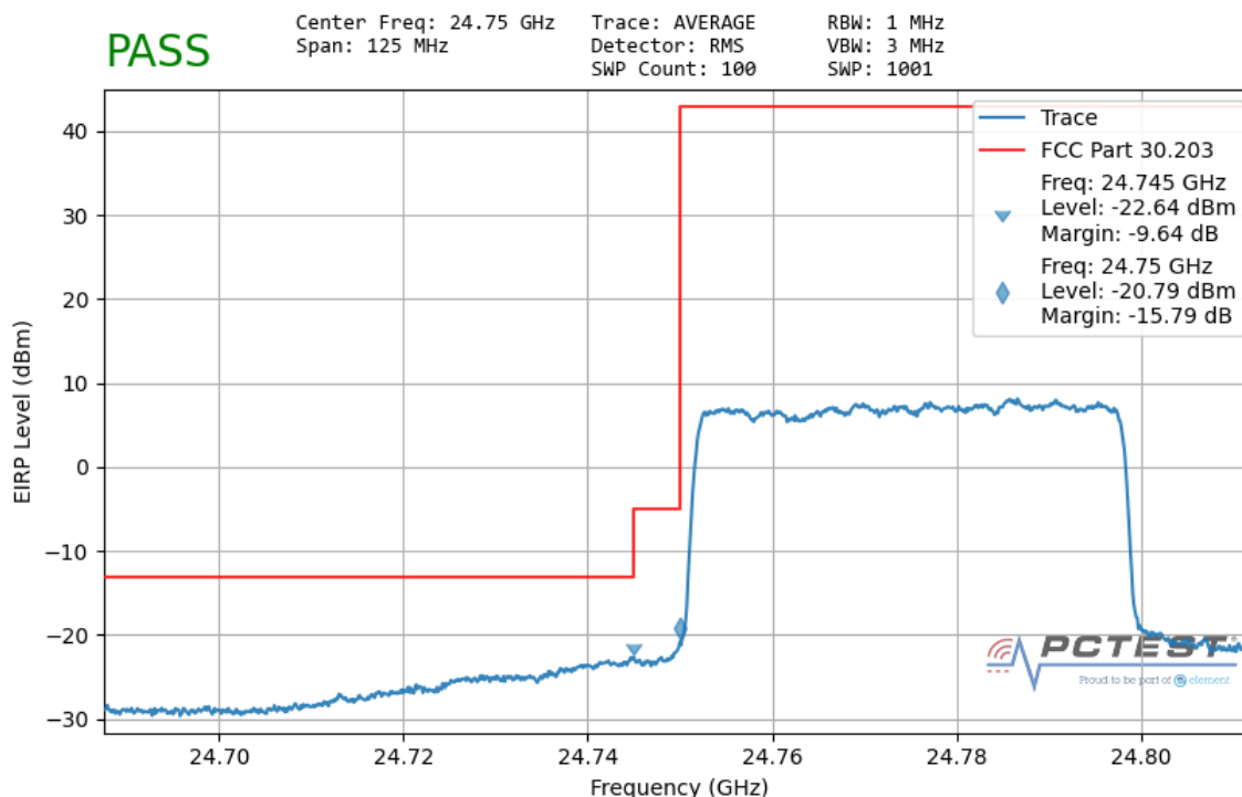
Plot 7-171. Ant2 Lower Band Edge (50MHz-1CC – \pi/2 -BPSK Full RB)
