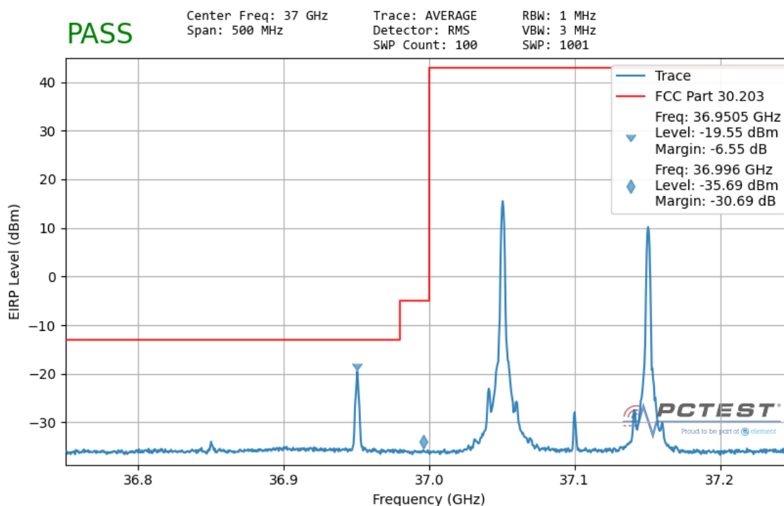
Plot 7-200. Ant1 Lower Band Edge (100MHz-2CC – QPSK 1 RB)
