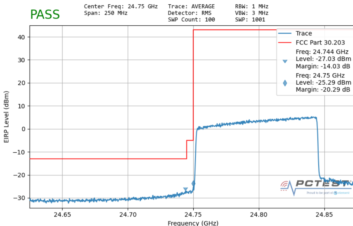
Plot 7-167. Ant1 Lower Band Edge (100MHz-1CC – QPSK Full RB)
