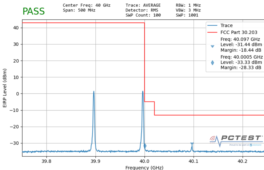
Plot 7-210. Ant2 Upper Band Edge (100MHz-2CC – QPSK 1 RB)
