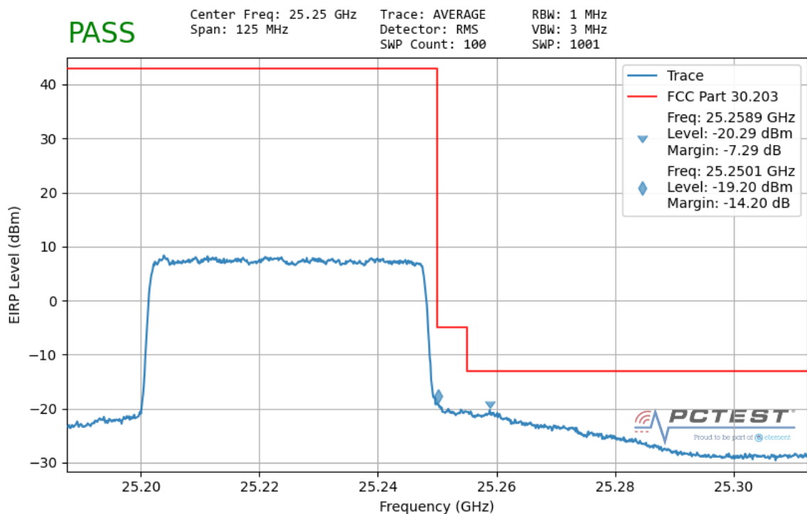
Plot 7-173. Ant2 Upper Band Edge (50MHz-1CC – QPSK Full RB)
