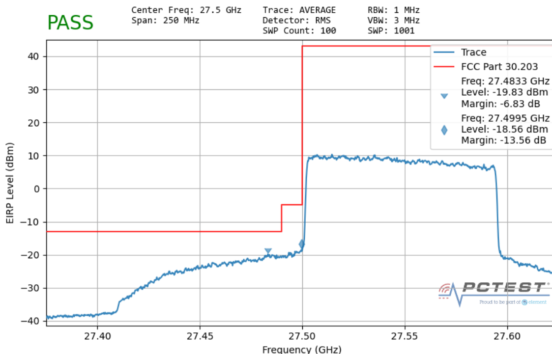
Plot 7-183. Ant1 Lower Band Edge (100MHz-1CC – QPSK Full RB)
