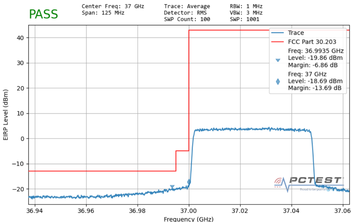
Plot 7-203. Ant2 Lower Band Edge (50MHz-1CC – \pi/2 -BPSK Full RB)
