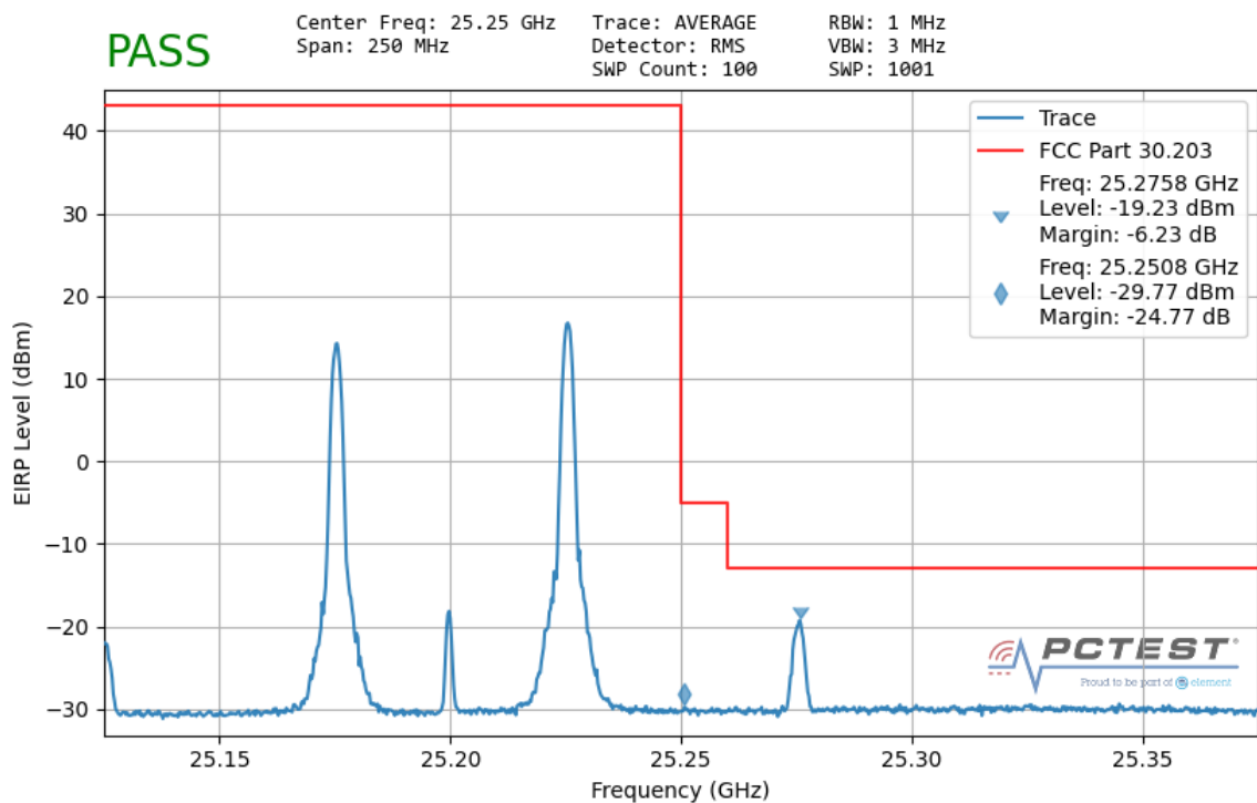
Plot 7-174. Ant2 Upper Band Edge (50MHz-2CC – QPSK 1 RB)
