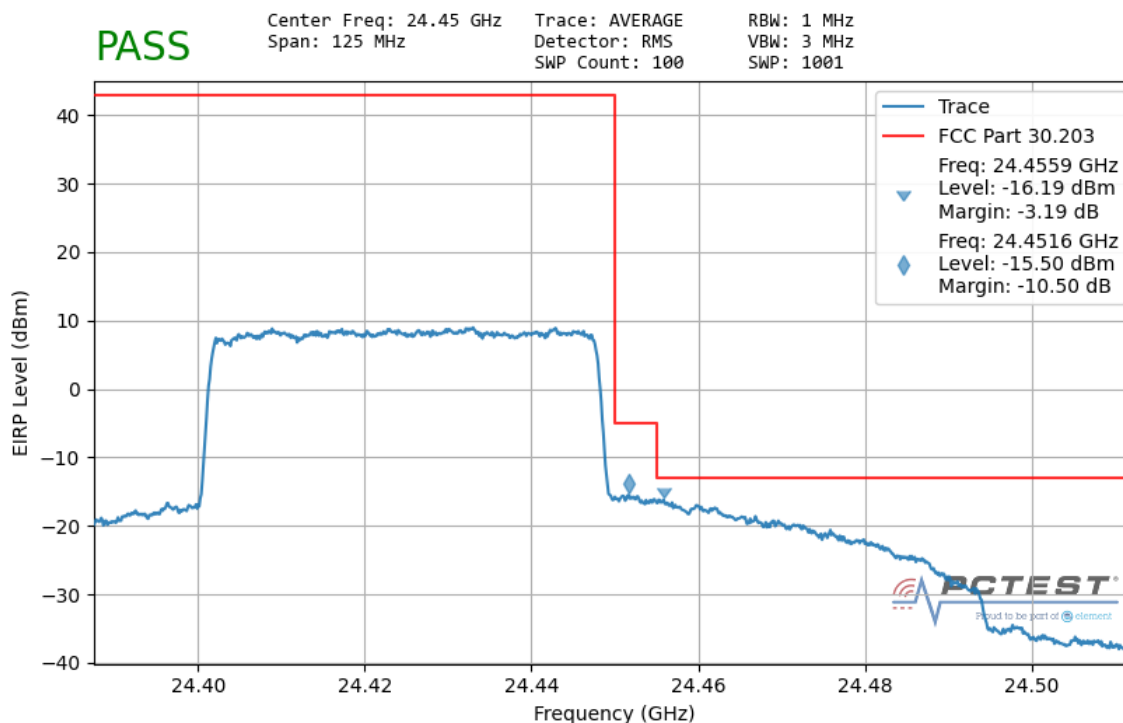
Plot 7-149. Ant1 Upper Band Edge (50MHz-1CC – QPSK Full RB)
