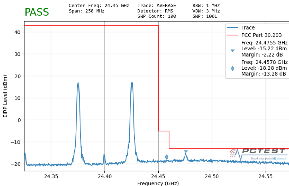
Plot 7-150. Ant1 Upper Band Edge (50MHz-2CC – QPSK 1 RB)
