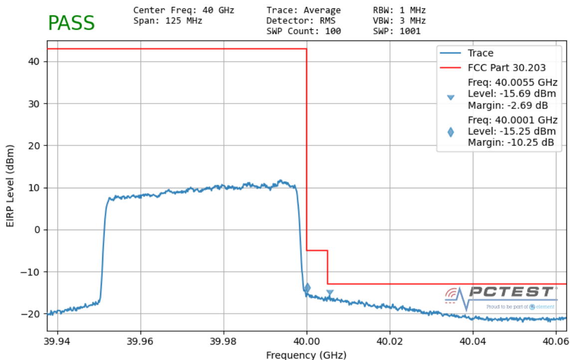
Plot 7-197. Ant1 Upper Band Edge (50MHz-1CC – QPSK Full RB)
