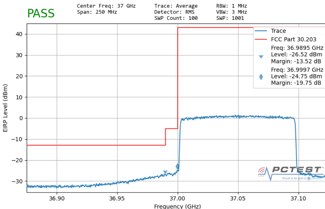
Plot 7-207. Ant2 Lower Band Edge (100MHz-1CC – QPSK Full RB)
