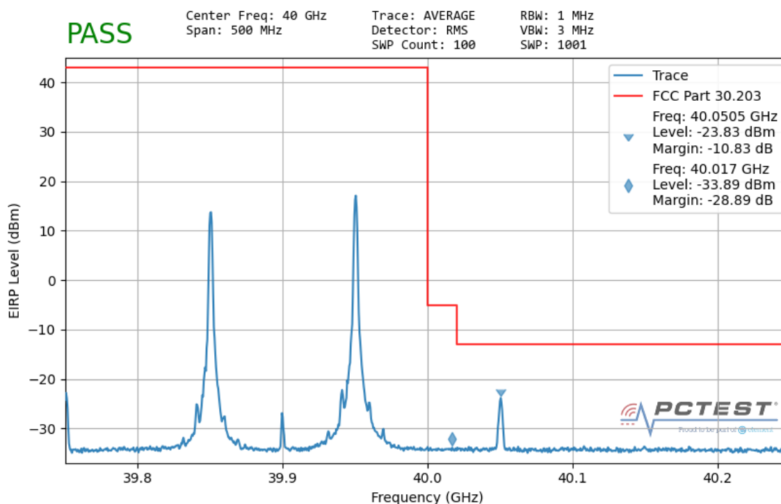
Plot 7-202. Ant1 Upper Band Edge (100MHz-2CC – QPSK 1 RB)
