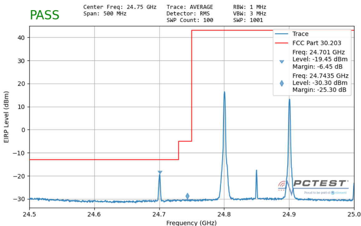
Plot 7-176. Ant2 Lower Band Edge – TRP (100MHz-2CC – QPSK 1 RB)
