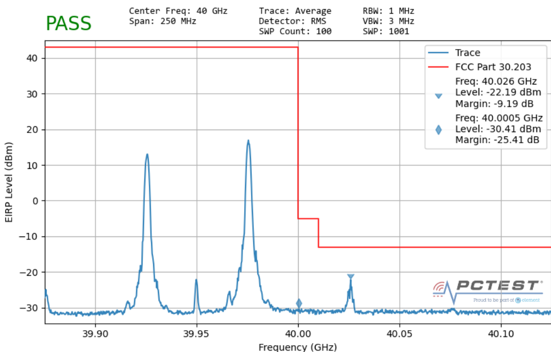
Plot 7-206. Ant2 Upper Band Edge (50MHz-2CC – QPSK 1 RB)
