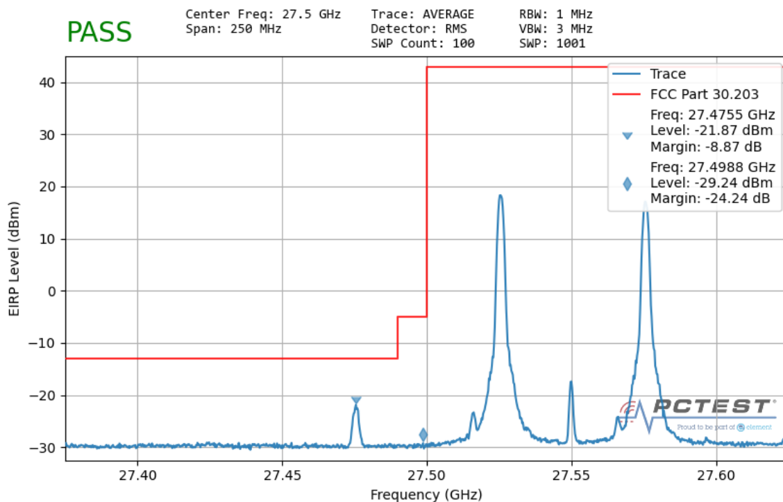
Plot 7-180. Ant1 Lower Band Edge (50MHz-2CC – QPSK 1 RB)
