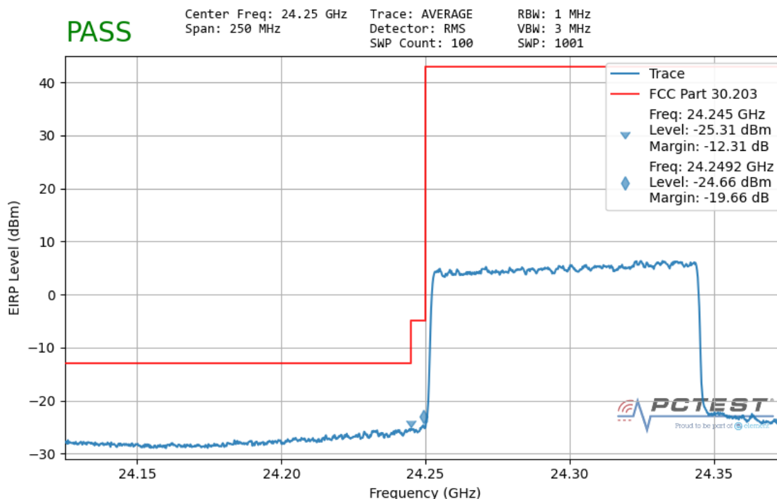
Plot 7-159. Ant2 Lower Band Edge (100MHz-1CC – QPSK Full RB)
