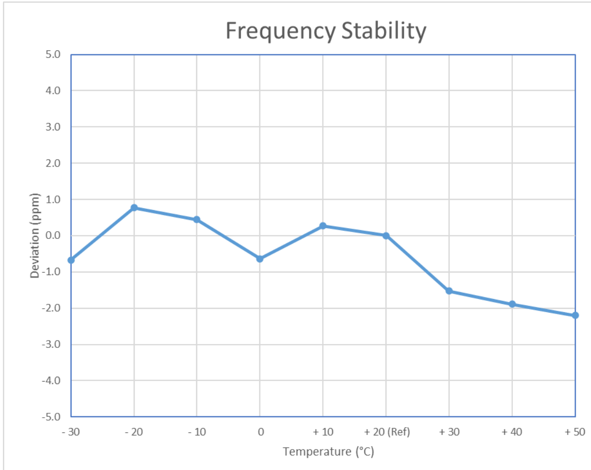
Figure 7-2. Frequency Stability Graph (n261)
