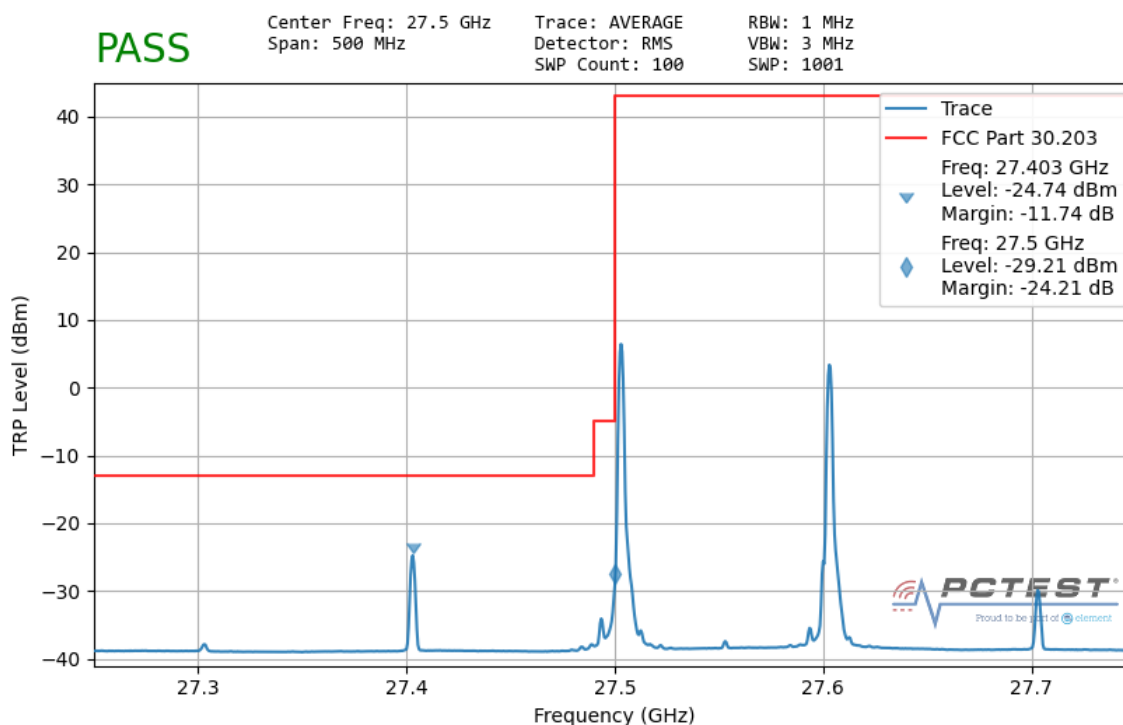
Plot 7-184. Ant1 Lower Band Edge – TRP (100MHz-2CC – QPSK 1 RB)
