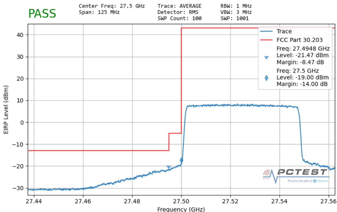
Plot 7-187. Ant2 Lower Band Edge (50MHz-1CC – \pi/2 -BPSK Full RB)
