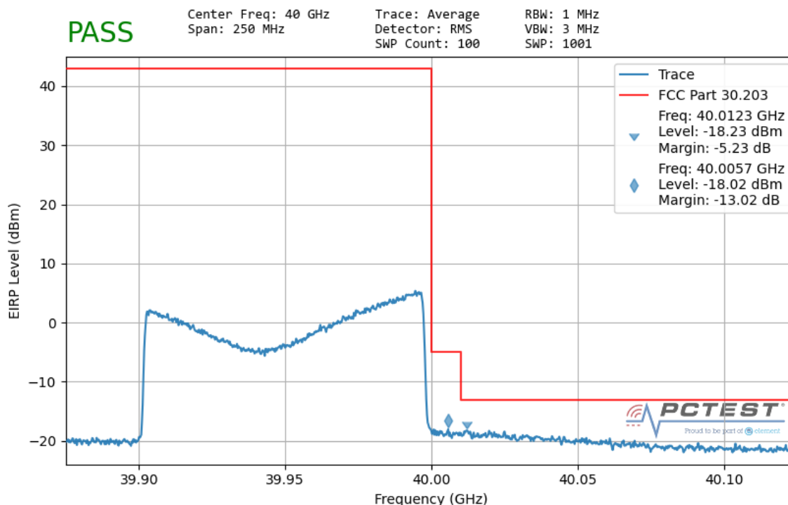
Plot 7-201. Ant1 Upper Band Edge (100MHz-1CC – QPSK Full RB)
