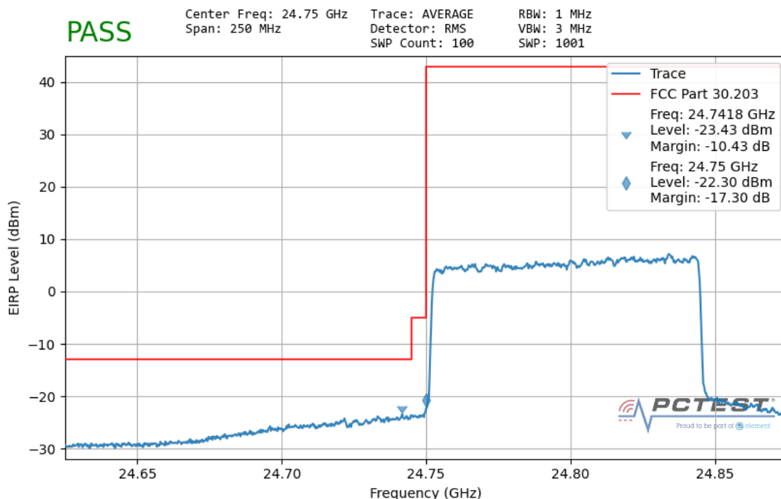
Plot 7-175. Ant2 Lower Band Edge (100MHz-1CC – QPSK Full RB)
