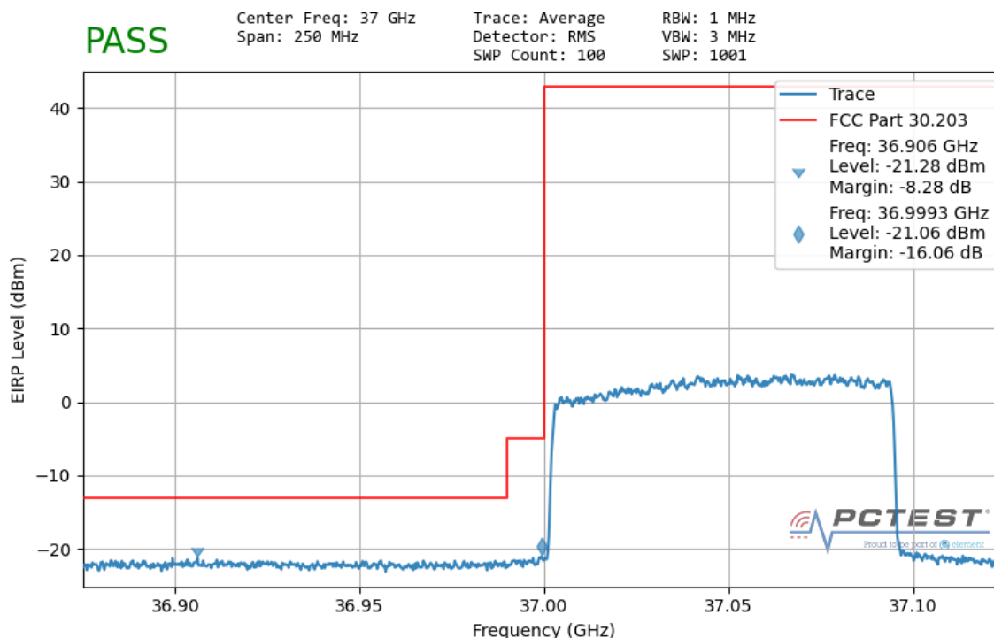
Plot 7-199. Ant1 Lower Band Edge (100MHz-1CC – QPSK Full RB)
