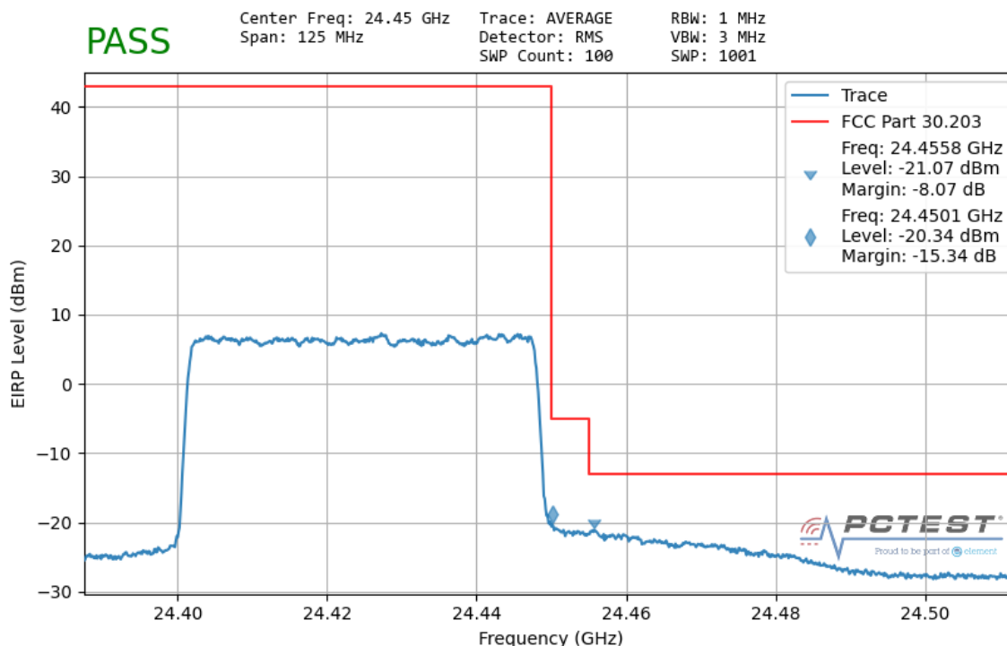
Plot 7-157. Ant2 Upper Band Edge (50MHz-1CC – QPSK Full RB)
