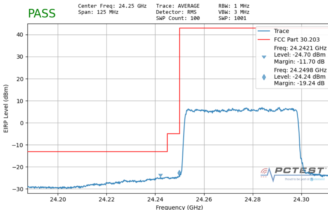
Plot 7-155. Ant2 Lower Band Edge (50MHz-1CC – QPSK Full RB)
