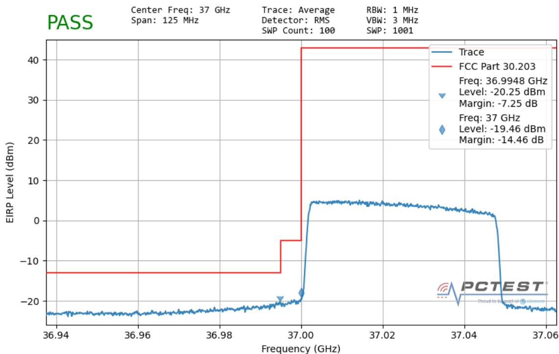
Plot 7-195. Ant1 Lower Band Edge (50MHz-1CC – QPSK Full RB)
