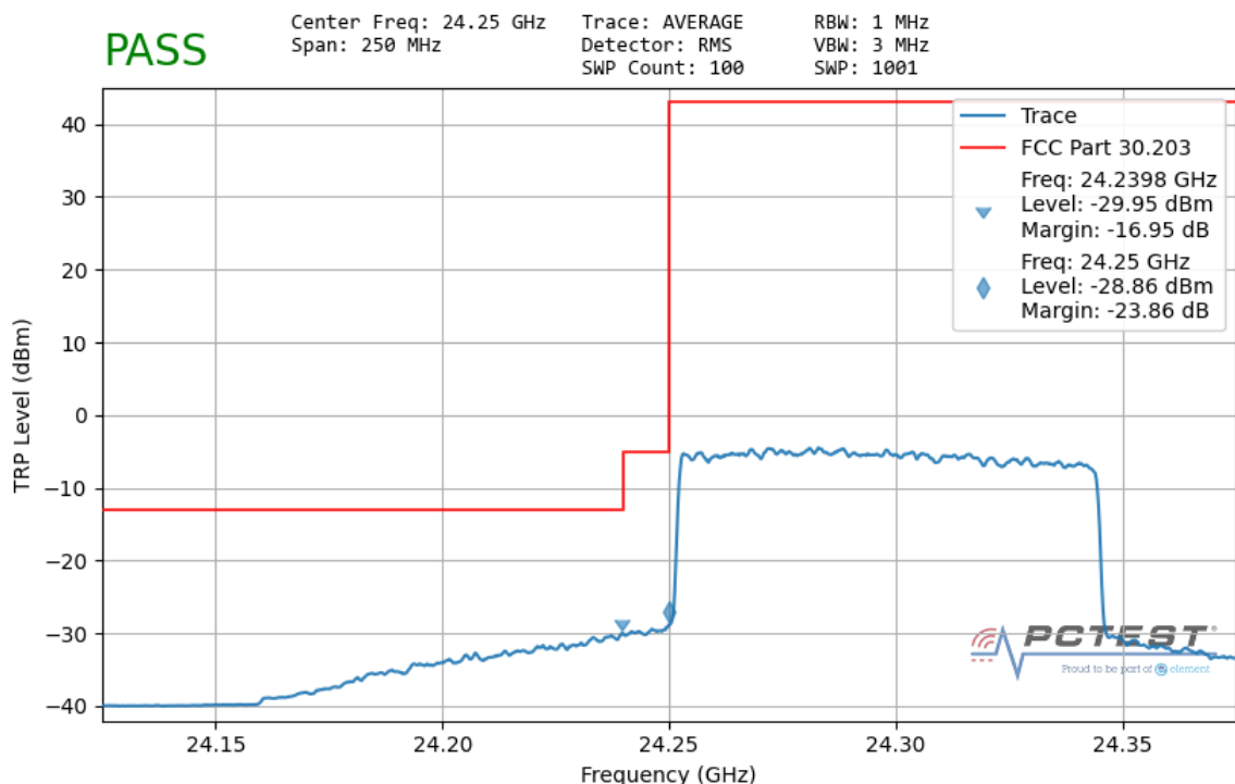
Plot 7-151. Ant1 Lower Band Edge – TRP (100MHz-1CC – QPSK Full RB)
