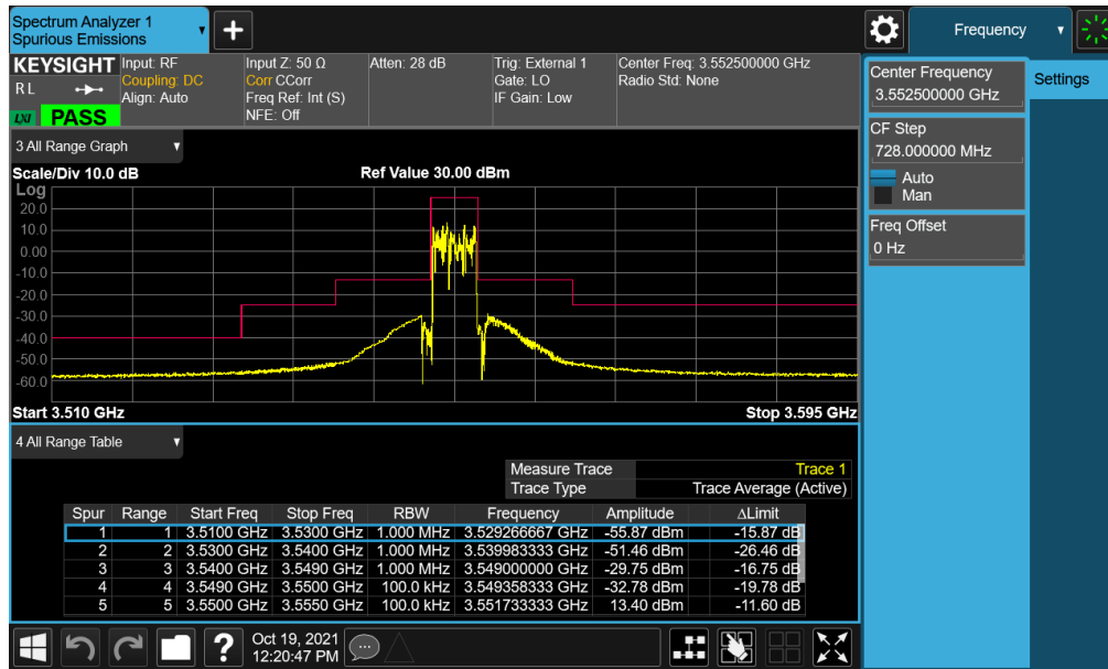
Plot 7-47. Channel Edge Plot (LTE Band 48 - 5MHz QPSK - Low Channel)
