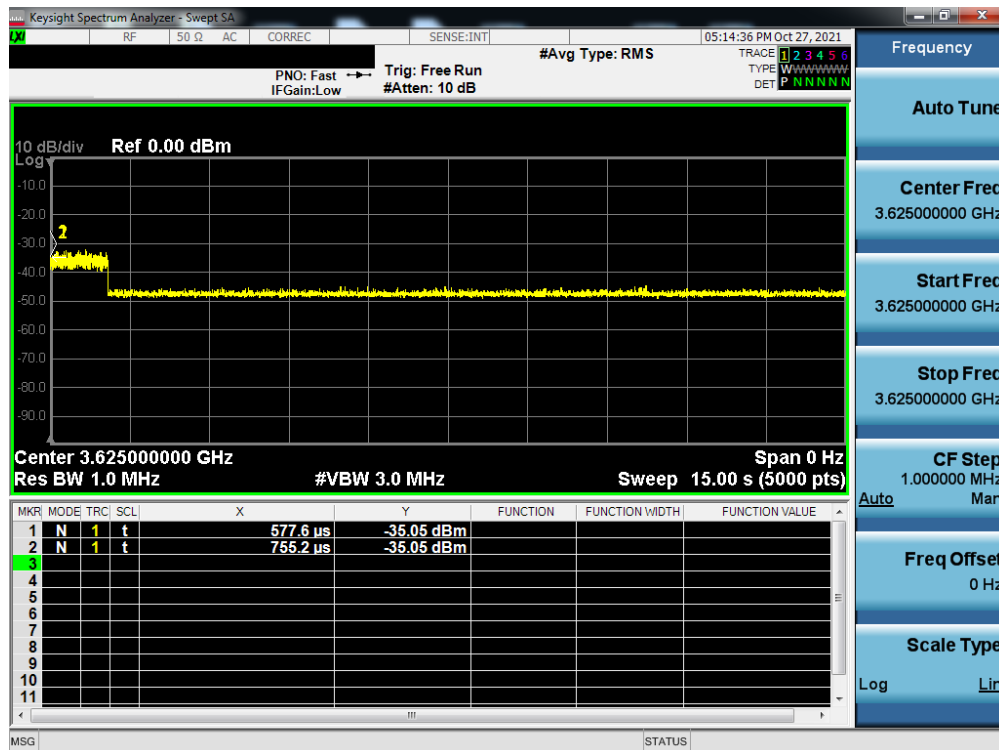
Plot 7-60. Run#1 End User Device Discontinues Operations within 10s
