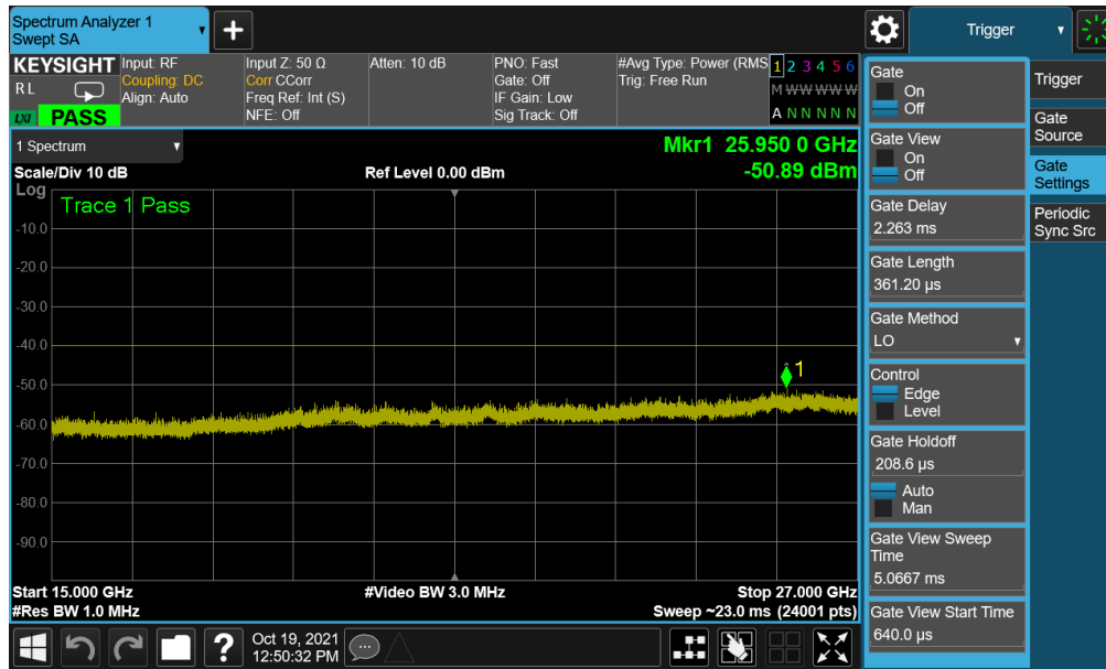
Plot 7-23. Conducted Spurious Plot (LTE Band 48 - 20MHz QPSK - Mid Channel)
