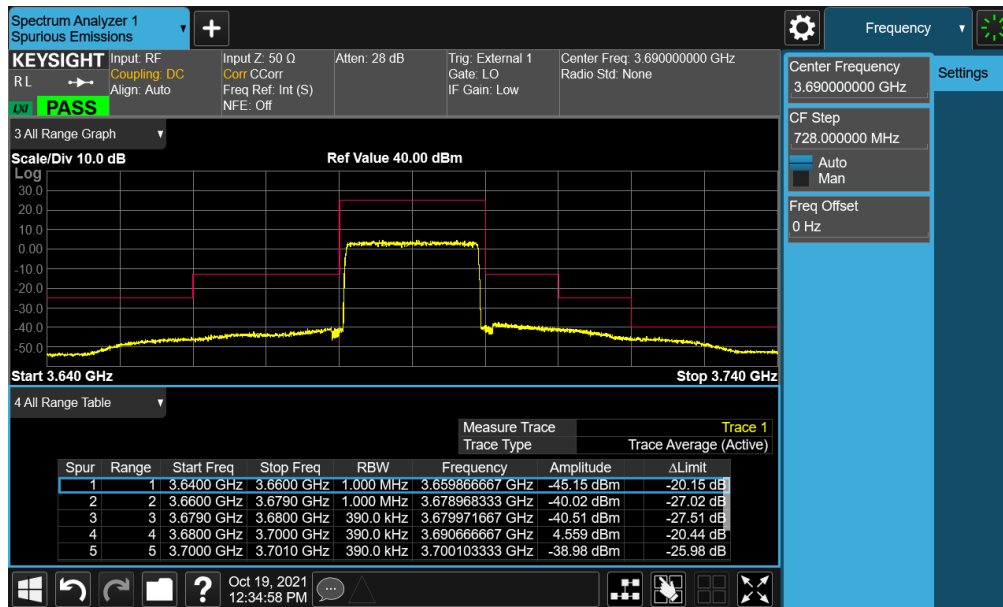
Plot 7-42. Channel Edge Plot (LTE Band 48 - 20MHz QPSK - High Channel)
