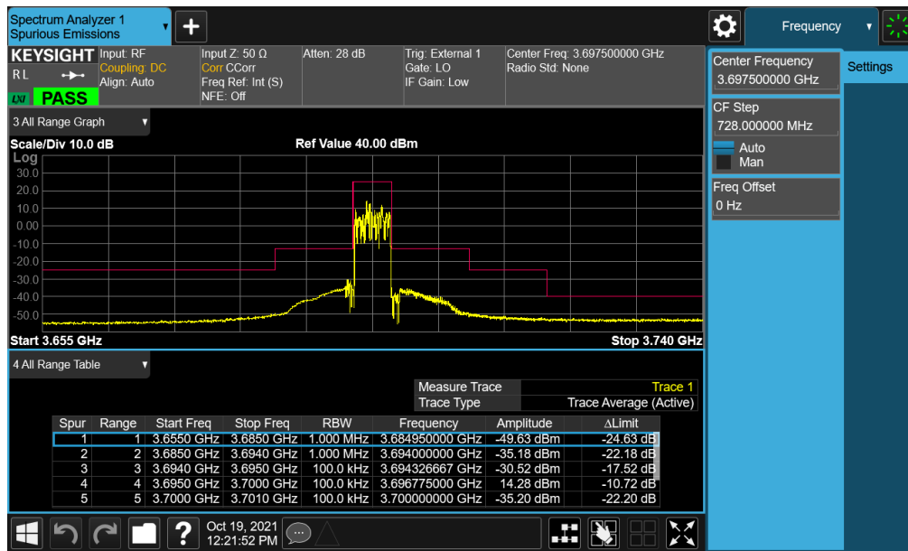
Plot 7-48. Channel Edge Plot (LTE Band 48 - 5MHz QPSK - High Channel)
