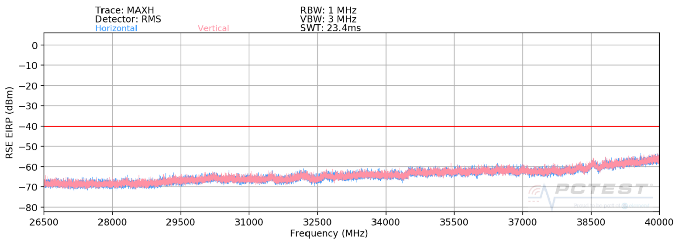
Plot 7-54. Radiated Spurious Plot 26.5-40GHz (LTE Band 48)
