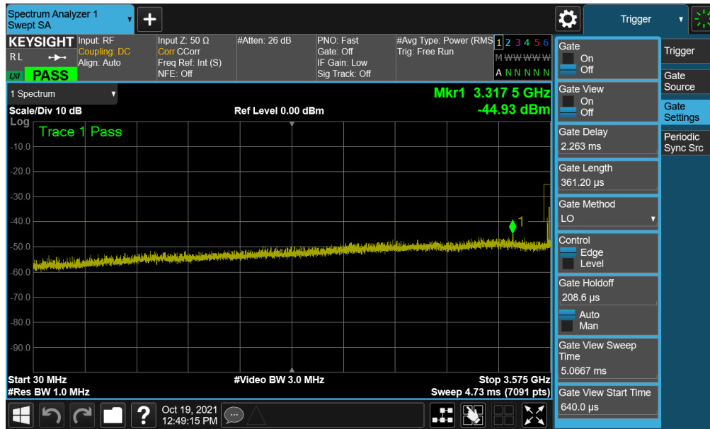
Plot 7-21. Conducted Spurious Plot (LTE Band 48 - 20MHz QPSK - Mid Channel)
