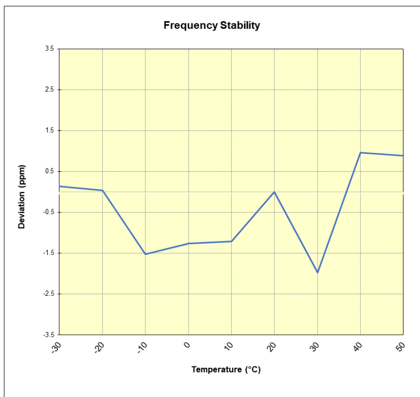
Plot 7-58. LTE Band 48 Frequency Stability Chart
