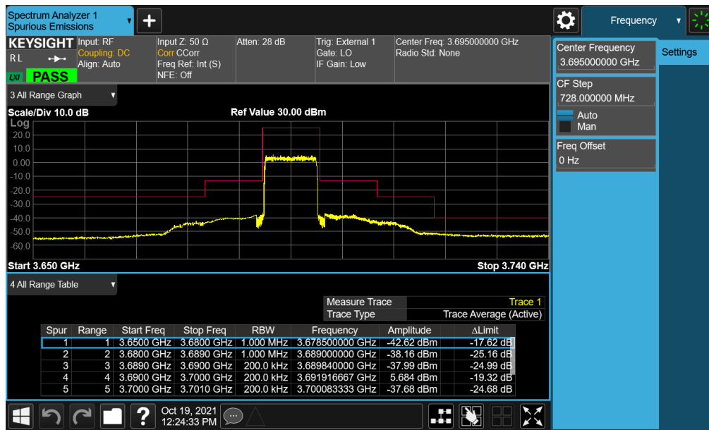
Plot 7-46. Channel Edge Plot (LTE Band 48 - 10MHz QPSK - High Channel)
