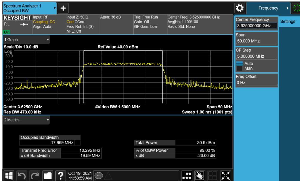
Plot 7-1. Occupied Bandwidth Plot (LTE Band 48 - 20MHz QPSK - Full RB Configuration)
