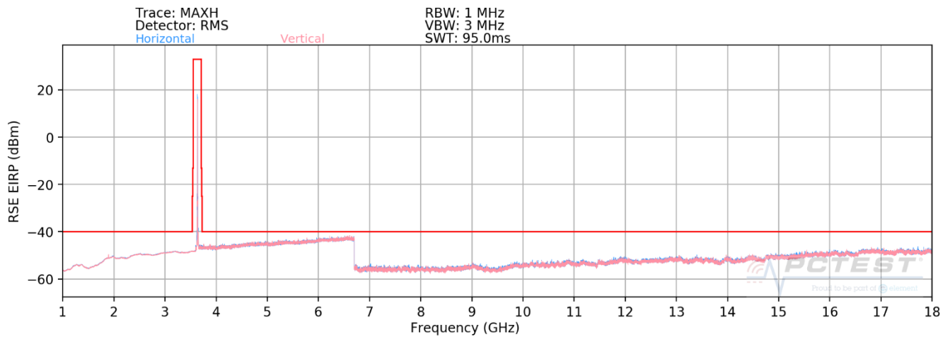
Plot 7-56. Radiated Spurious Plot (ULCA LB48) – Mid Channel
