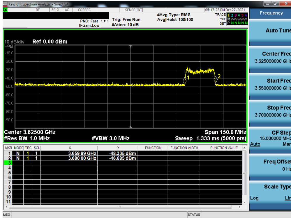
Plot 7-61. Run#2 End User Device Frequency of Operations
