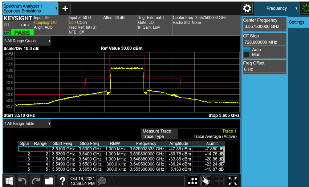
Plot 7-43. Channel Edge Plot (LTE Band 48 - 15MHz QPSK - Low Channel)
