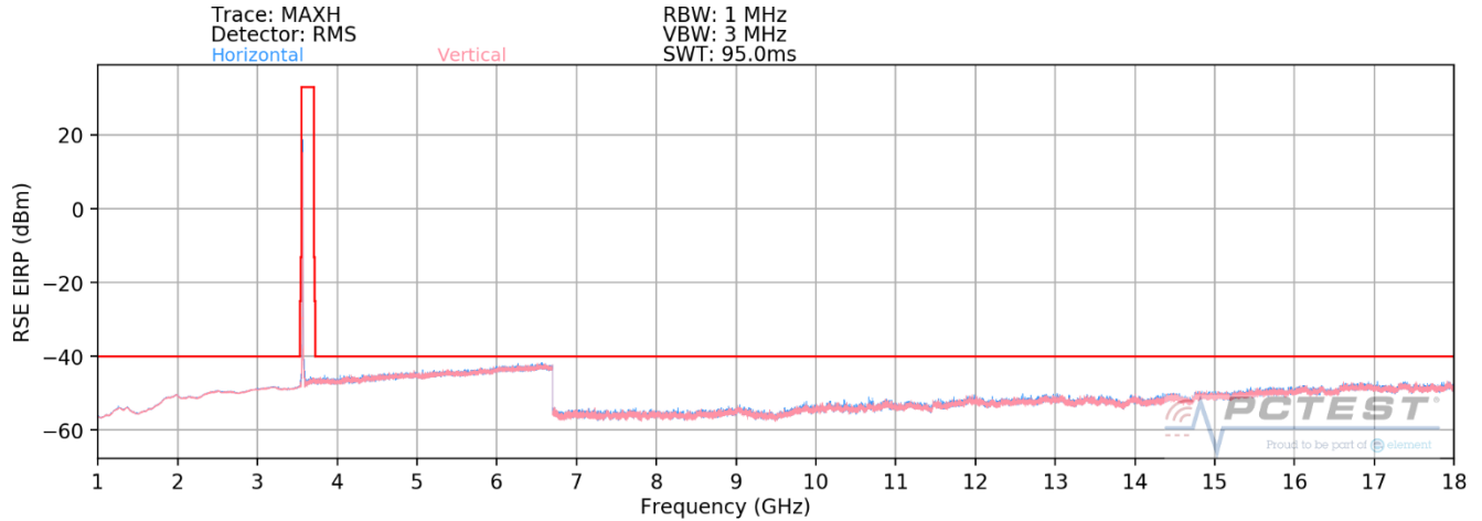
Plot 7-55. Radiated Spurious Plot (ULCA LB48) – Low Channel
