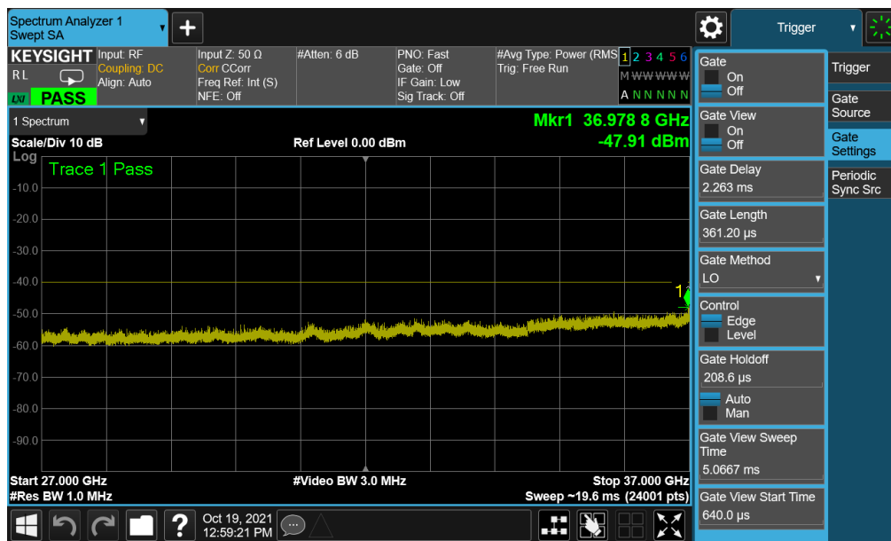
Plot 7-20. Conducted Spurious Plot (LTE Band 48 - 20MHz QPSK - Low Channel)
