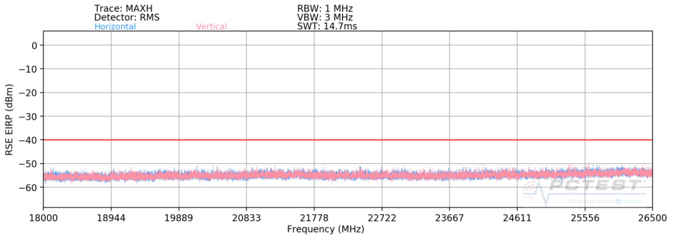
Plot 7-53. Radiated Spurious Plot 18-26.5GHz (LTE Band 48)
