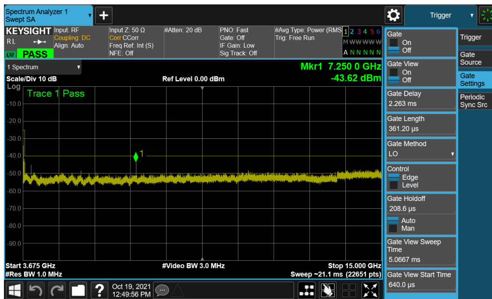
Plot 7-22. Conducted Spurious Plot (LTE Band 48 - 20MHz QPSK - Mid Channel)
