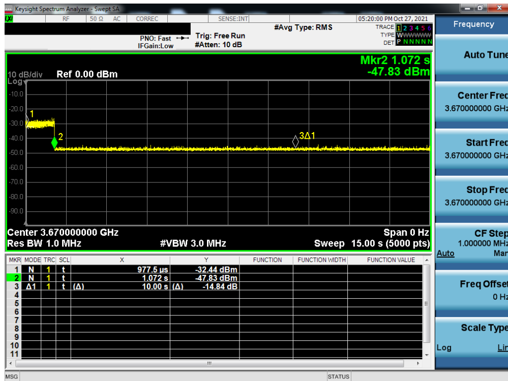
Plot 7-62. Run#2 End User Device Discontinues Operations within 10s
