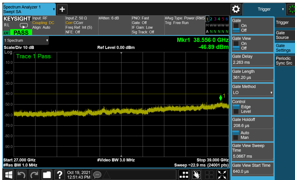
Plot 7-24. Conducted Spurious Plot (LTE Band 48 - 20MHz QPSK - Mid Channel)
