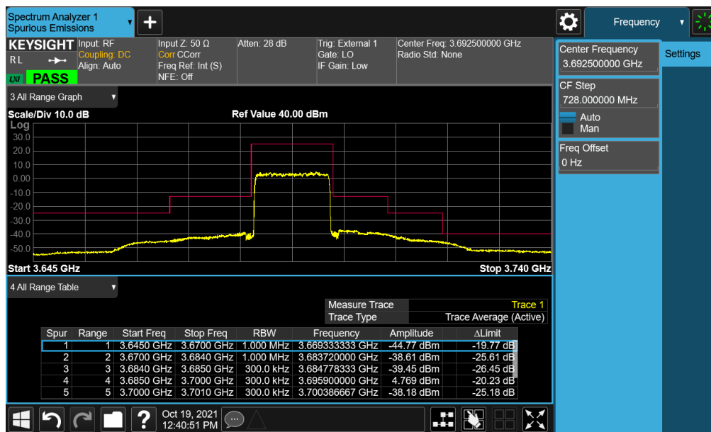
Plot 7-44. Channel Edge Plot (LTE Band 48 - 15MHz QPSK - High Channel)
