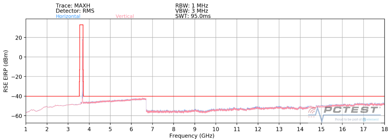
Plot 7-57. Radiated Spurious Plot (ULCA LB48) – High Channel
