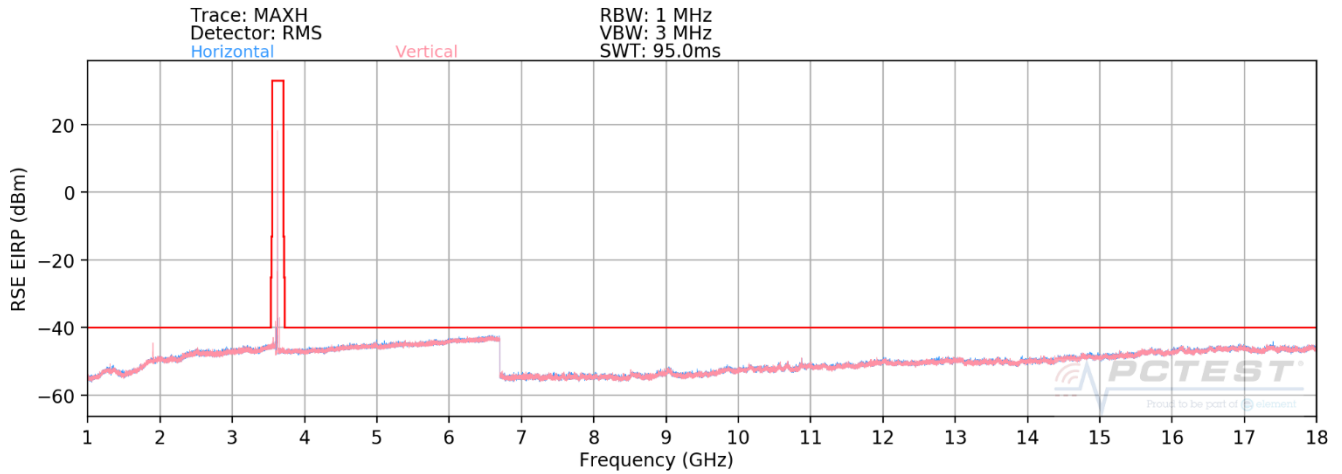
Plot 7-52. Radiated Spurious Plot 1-18GHz (LTE Band 48)
