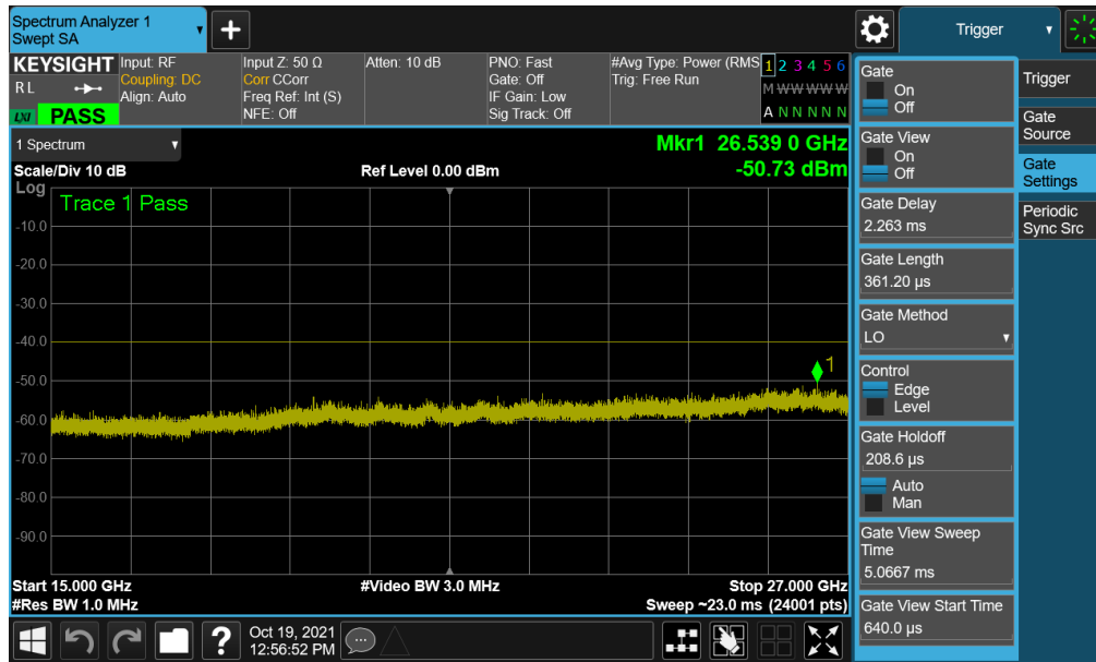
Plot 7-19. Conducted Spurious Plot (LTE Band 48 - 20MHz QPSK - Low Channel)
