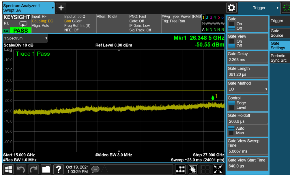
Plot 7-27. Conducted Spurious Plot (LTE Band 48 - 20MHz QPSK - High Channel)
