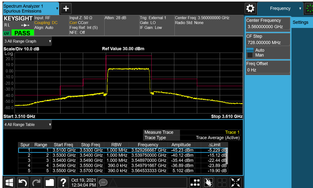
Plot 7-41. Channel Edge Plot (LTE Band 48 - 20MHz QPSK - Low Channel)
