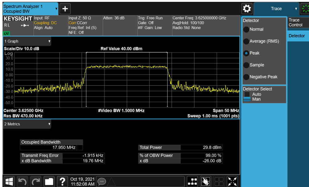
Plot 7-2. Occupied Bandwidth Plot (LTE Band 48 - 20MHz 16-QAM - Full RB Configuration)
