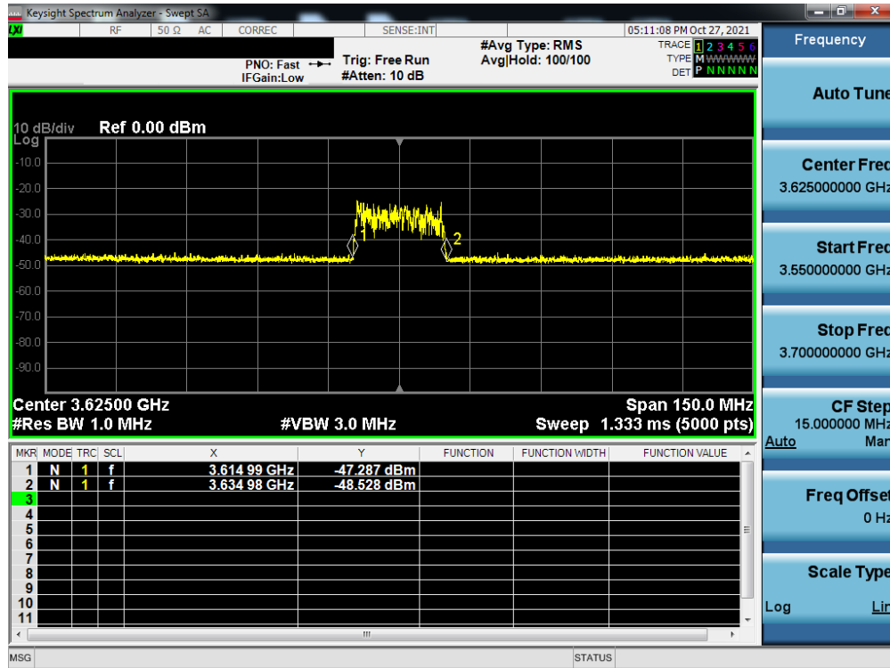
Plot 7-59. Run#1 End User Device Frequency of Operations
