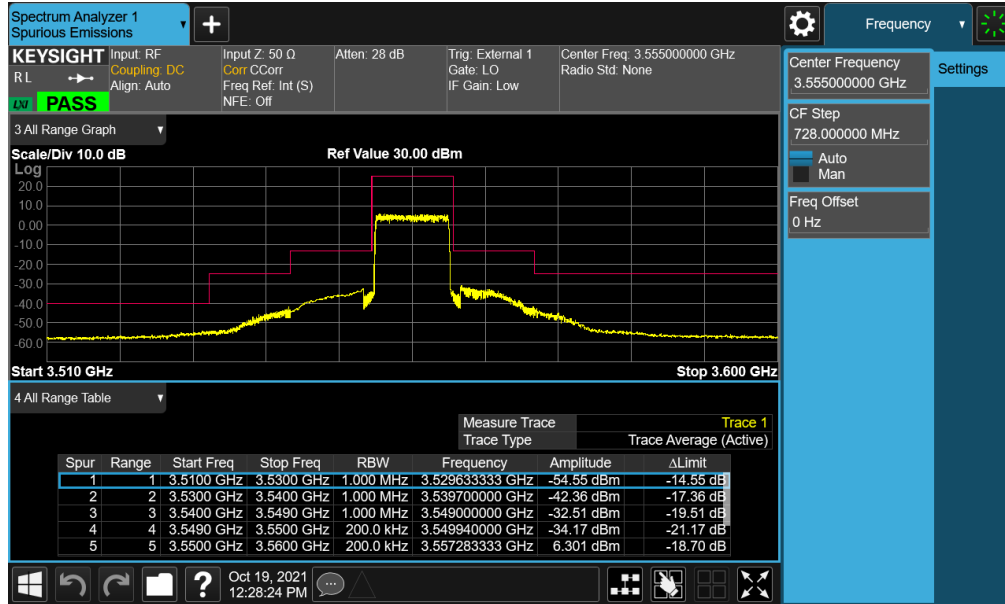
Plot 7-45. Channel Edge Plot (LTE Band 48 - 10MHz QPSK - Low Channel)
