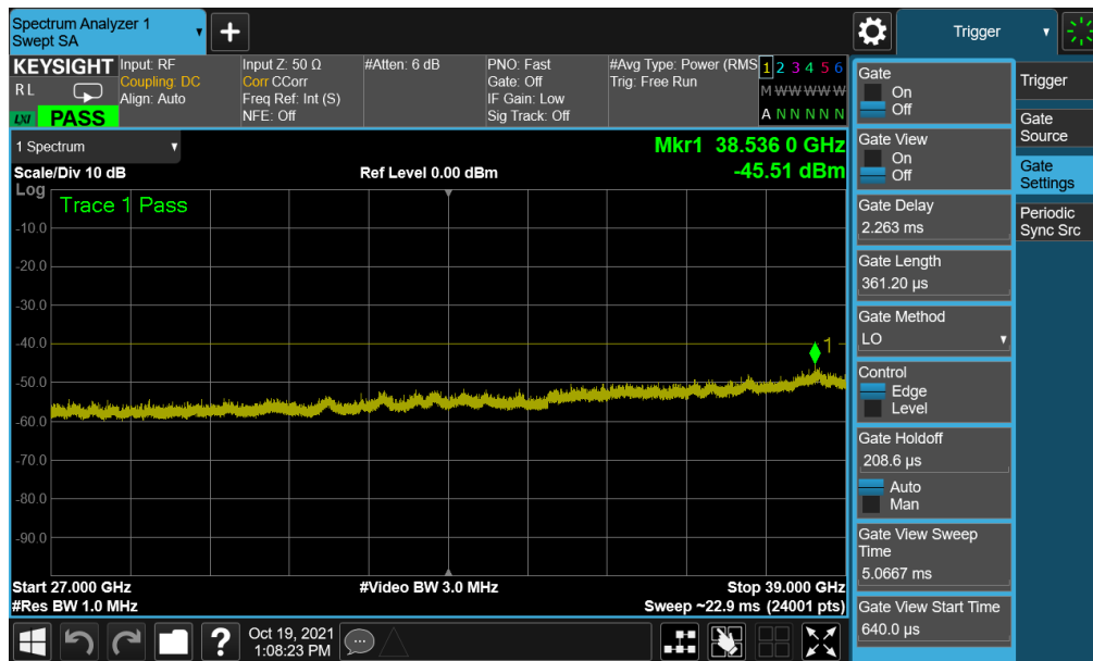
Plot 7-28. Conducted Spurious Plot (LTE Band 48 - 20MHz QPSK - High Channel)
