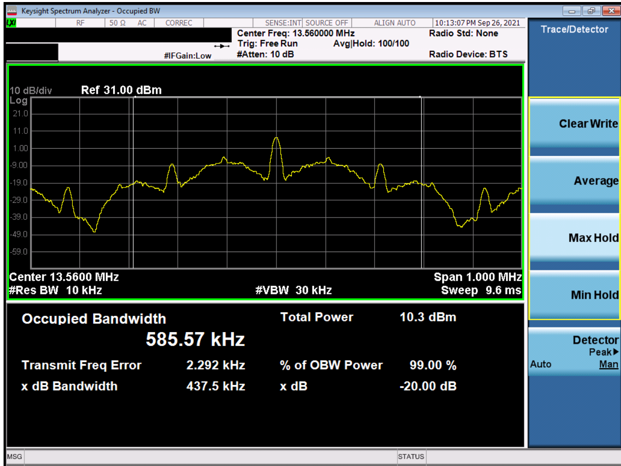
Plot 7-1. 20dB and 99% Bandwidth Plot
