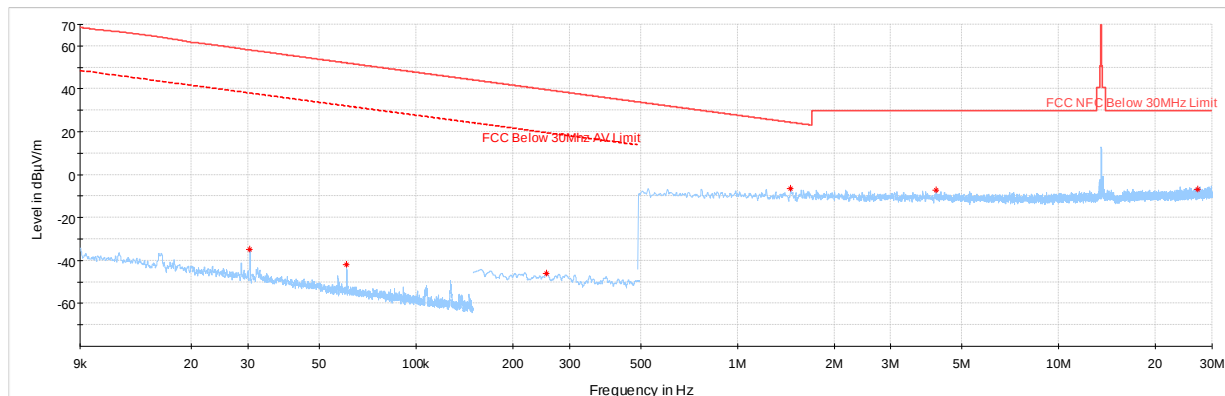
Plot 7-4. Radiated Spurious Emissions 9kHz – 30MHz (Pol. Y)
