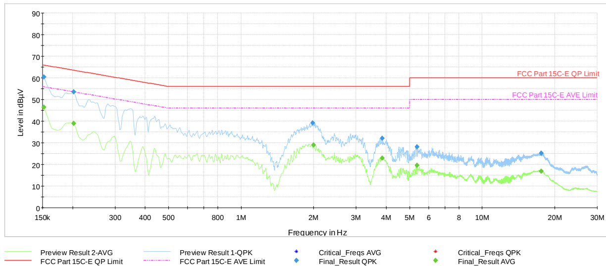
Plot 7-8. AC Line-Conducted Plot (N)
