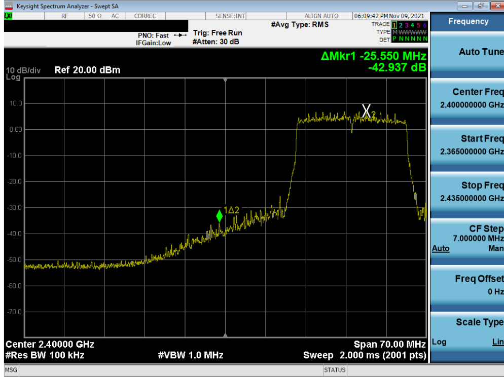
Plot 7-63. Band Edge Plot MIMO ANT1 (802.11ax (2.4GHz) – Ch. 3)
