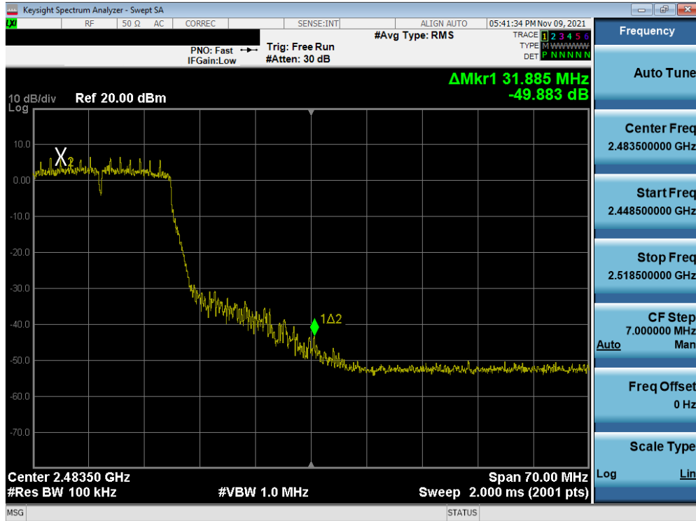
Plot 7-59. Band Edge Plot MIMO ANT1 (802.11n (2.4GHz) – Ch. 10)
