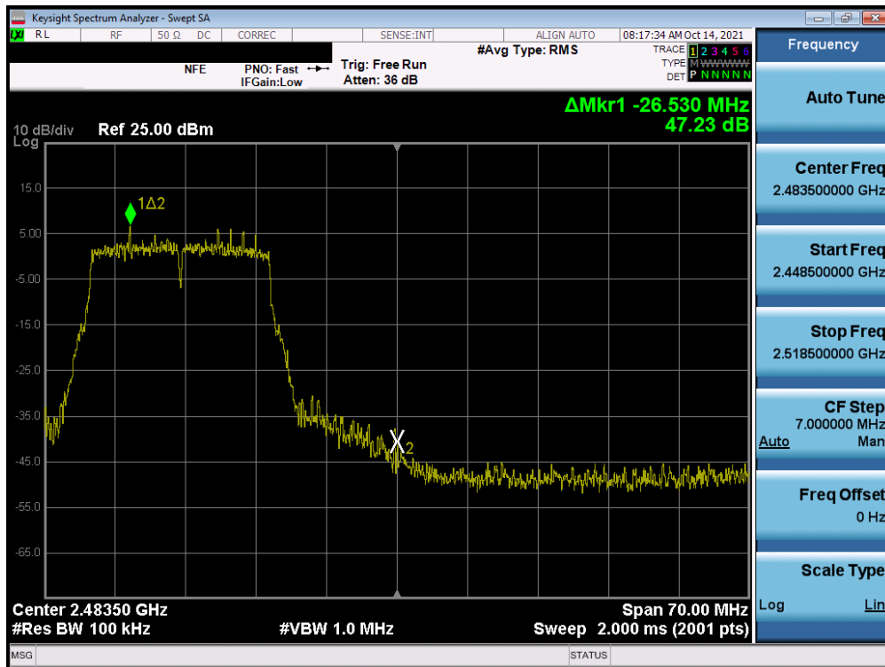
Plot 7-60. Band Edge Plot MIMO ANT1 (802.11n (2.4GHz) – Ch. 11)
