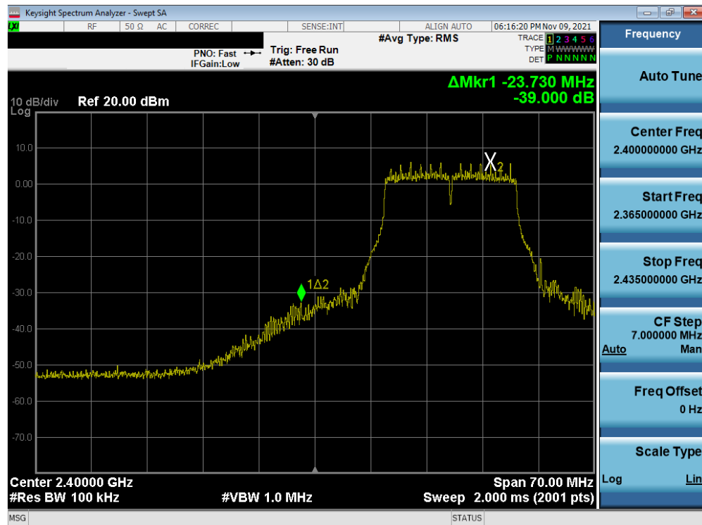
Plot 7-67. Band Edge Plot MIMO ANT2 (802.11g- Ch. 2)
