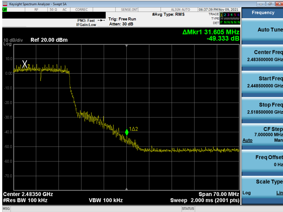
Plot 7-72. Band Edge Plot MIMO ANT2 (802.11n (2.4GHz) – Ch. 10)
