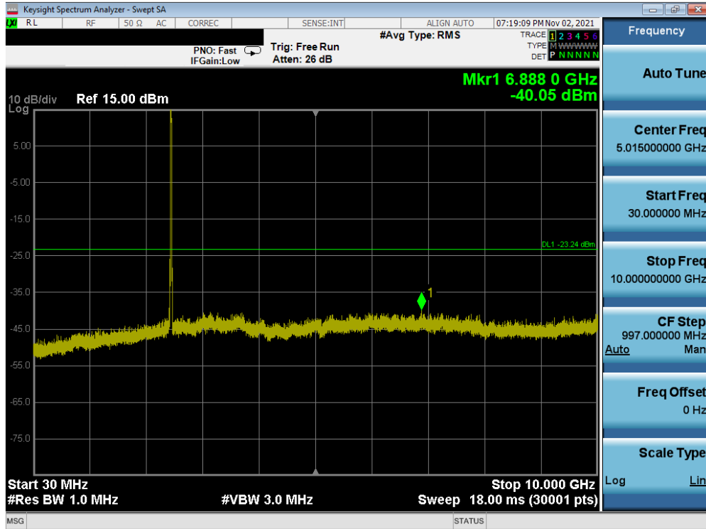
Plot 7-95. Conducted Spurious Plot MIMO ANT1 (802.11g – Ch. 11)
