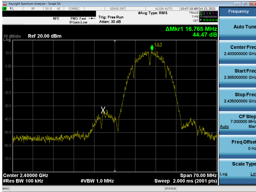
Plot 7-51. Band Edge Plot SISO ANT2 (802.11b – Ch. 1)
