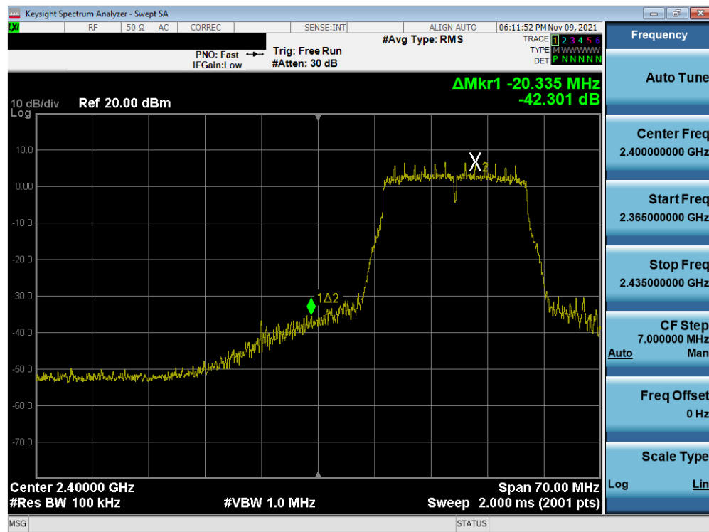
Plot 7-58. Band Edge Plot MIMO ANT1 (802.11n (2.4GHz) – Ch. 2)
