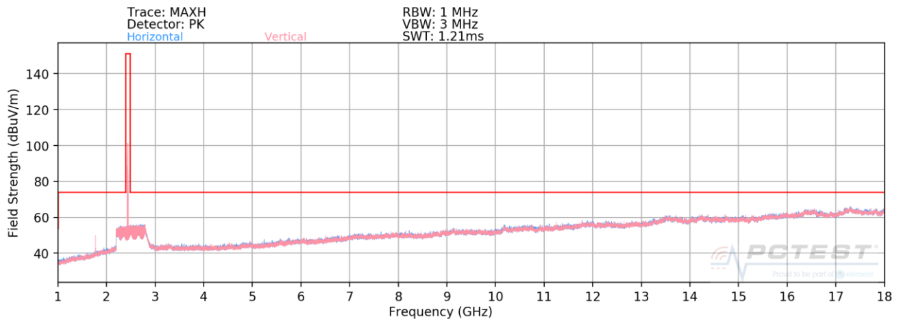
Plot 7-104. Radiated Spurious Plot above 1GHz SISO ANT1 (802.11b – Ch. 6)
