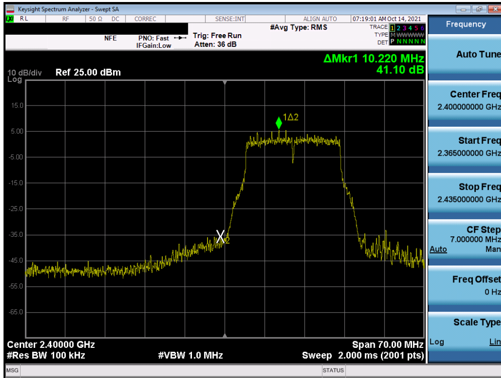
Plot 7-66. Band Edge Plot MIMO ANT2 (802.11g- Ch. 1)
