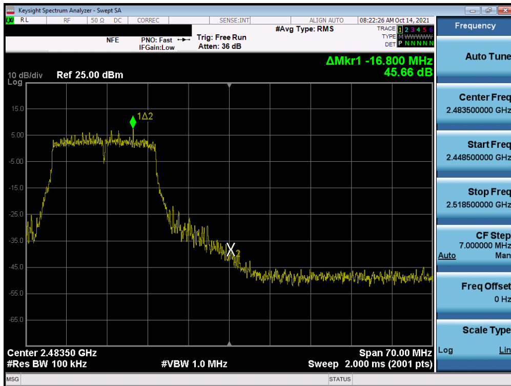
Plot 7-73. Band Edge Plot MIMO ANT2 (802.11n (2.4GHz) – Ch. 11)
