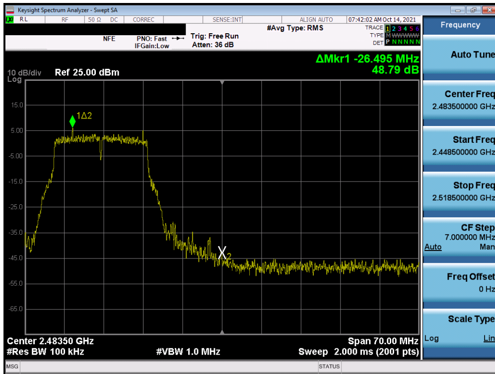
Plot 7-56. Band Edge Plot MIMO ANT1 (802.11g – Ch. 11)
