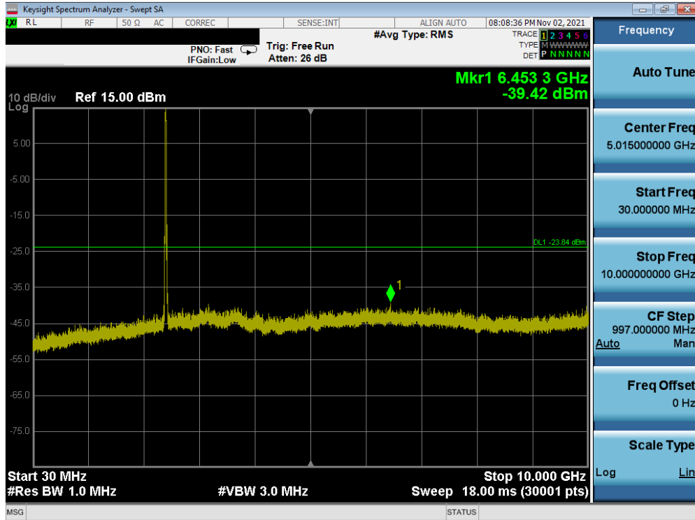
Plot 7-97. Conducted Spurious Plot MIMO ANT2 (802.11g – Ch. 1)
