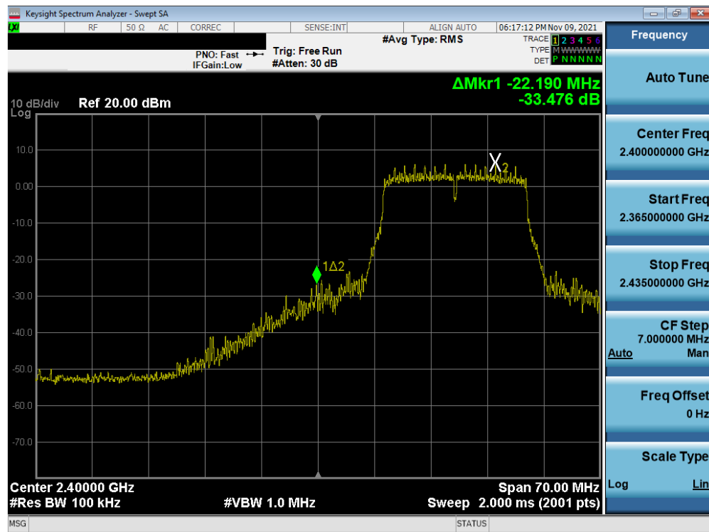
Plot 7-71. Band Edge Plot MIMO ANT2 (802.11n (2.4GHz) – Ch. 2)
