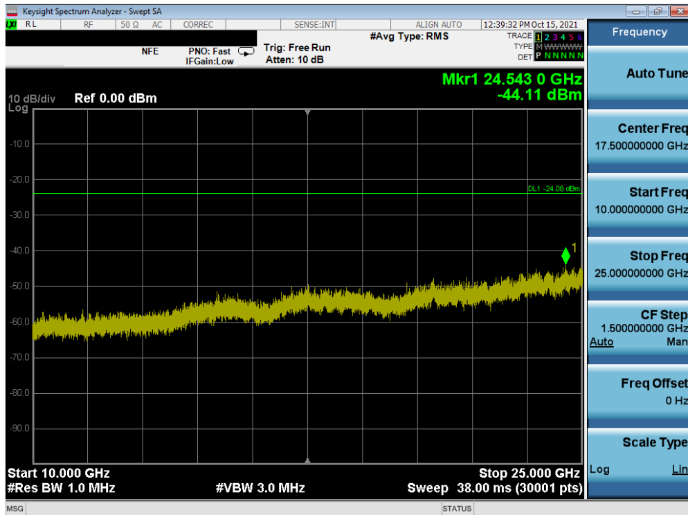
Plot 7-94. Conducted Spurious Plot MIMO ANT1 (802.11g – Ch. 6)
