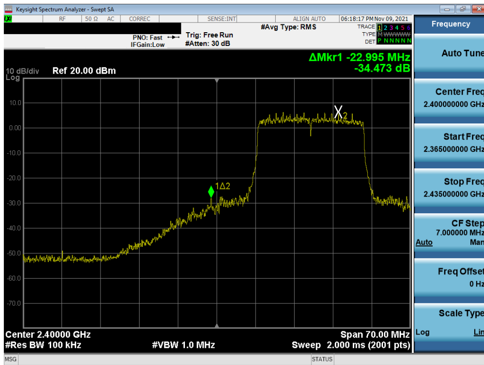
Plot 7-75. Band Edge Plot MIMO ANT2 (802.11ax (2.4GHz) – Ch. 2)
