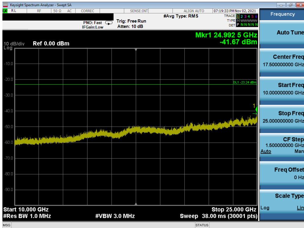
Plot 7-96. Conducted Spurious Plot MIMO ANT1 (802.11g – Ch. 11)
