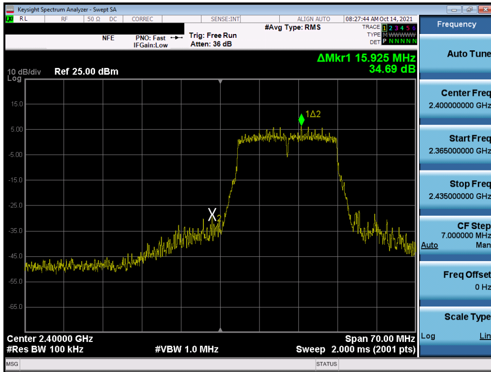
Plot 7-70. Band Edge Plot MIMO ANT2 (802.11n (2.4GHz) – Ch. 1)
