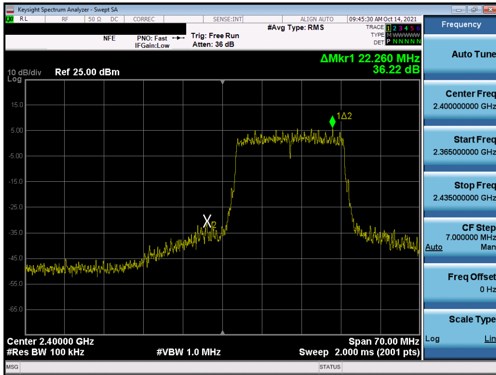
Plot 7-61. Band Edge Plot MIMO ANT1 (802.11ax (2.4GHz) – Ch. 1)
