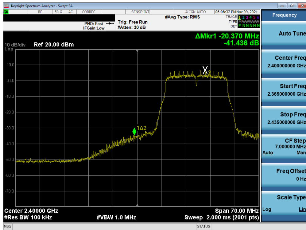
Plot 7-62. Band Edge Plot MIMO ANT1 (802.11ax (2.4GHz) – Ch. 2)
