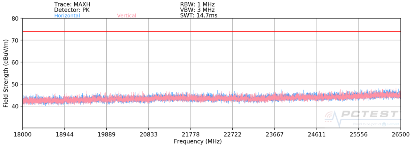
Plot 7-106. Radiated Spurious Plot above 18GHz SISO ANT1
