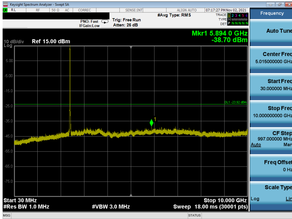
Plot 7-91. Conducted Spurious Plot MIMO ANT1 (802.11g - Ch. 1)
