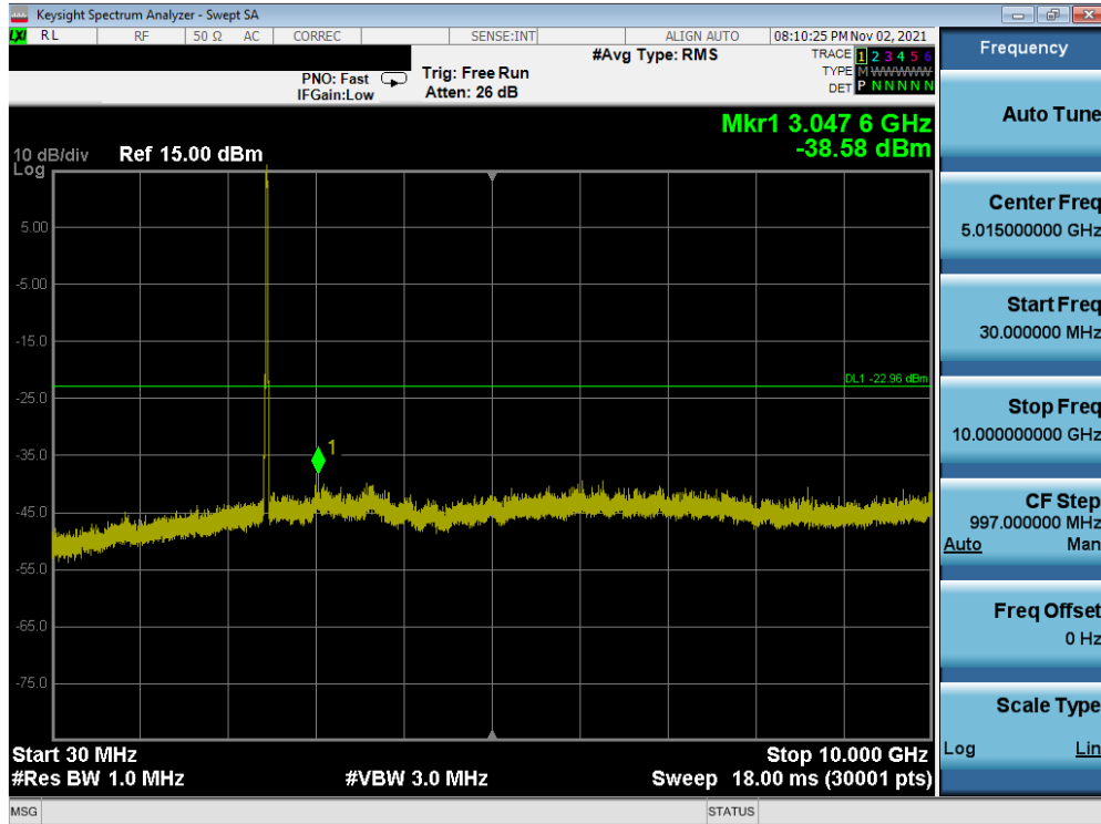
Plot 7-101. Conducted Spurious Plot MIMO ANT2 (802.11g – Ch. 11)
