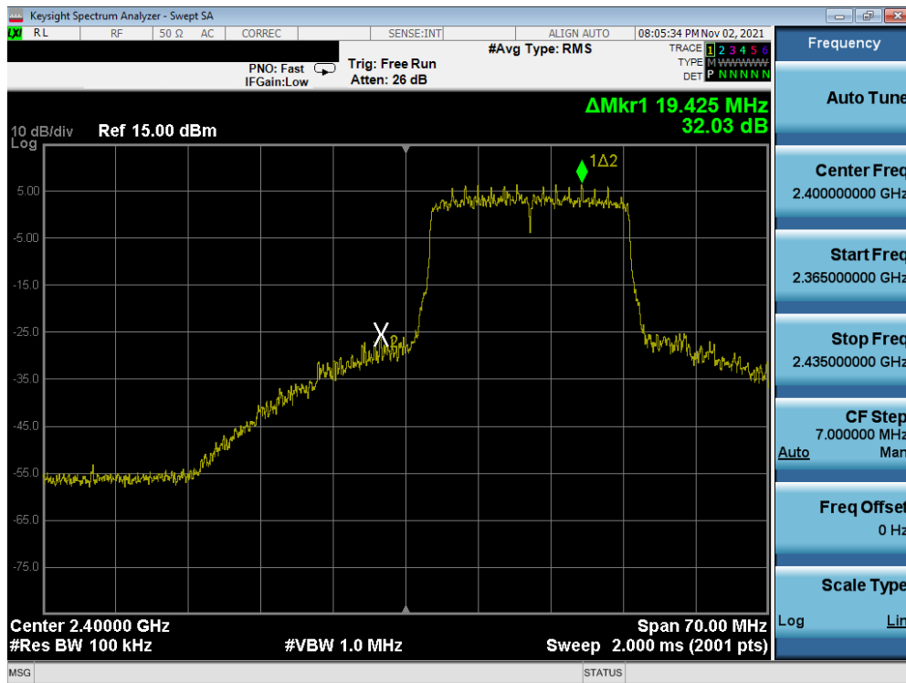
Plot 7-74. Band Edge Plot MIMO ANT2 (802.11ax (2.4GHz) – Ch. 1)
