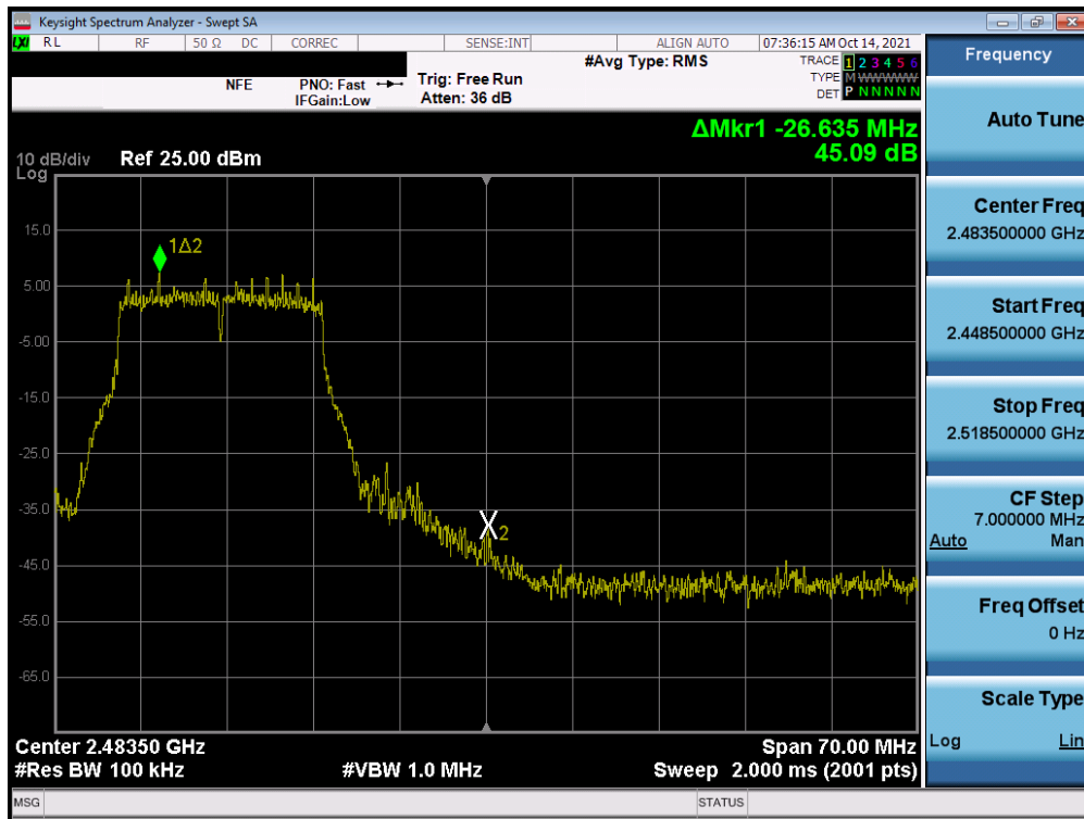
Plot 7-69. Band Edge Plot MIMO ANT2 (802.11g – Ch. 11)
