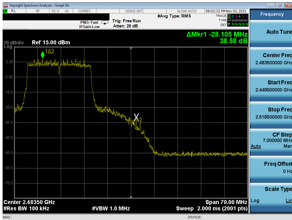
Plot 7-78. Band Edge Plot MIMO ANT2 (802.11ax (2.4GHz) – Ch. 11)
