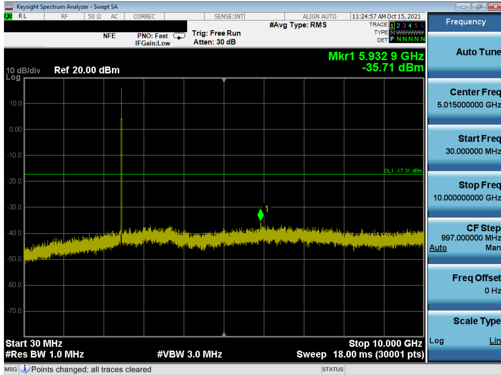
Plot 7-83. Conducted Spurious Plot SISO ANT1 (802.11b – Ch. 11)
