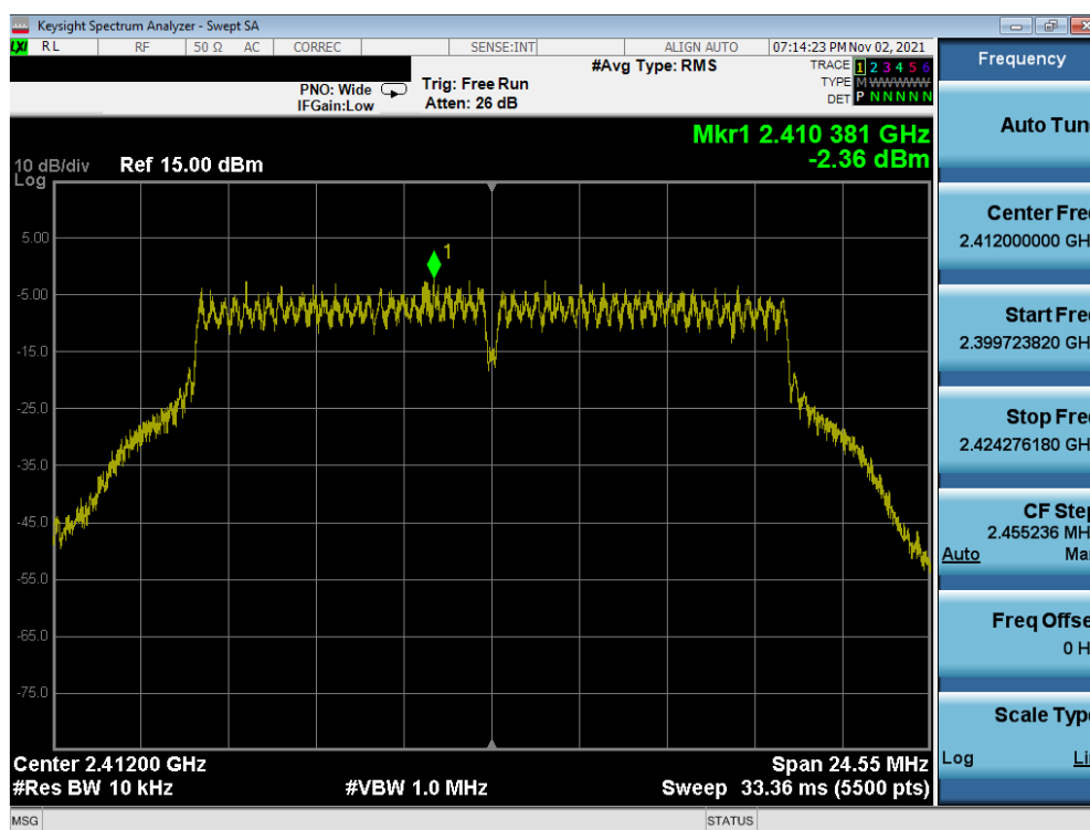
Plot 7-31. Power Spectral Density Plot MIMO ANT1 (802.11g – Ch. 1)
