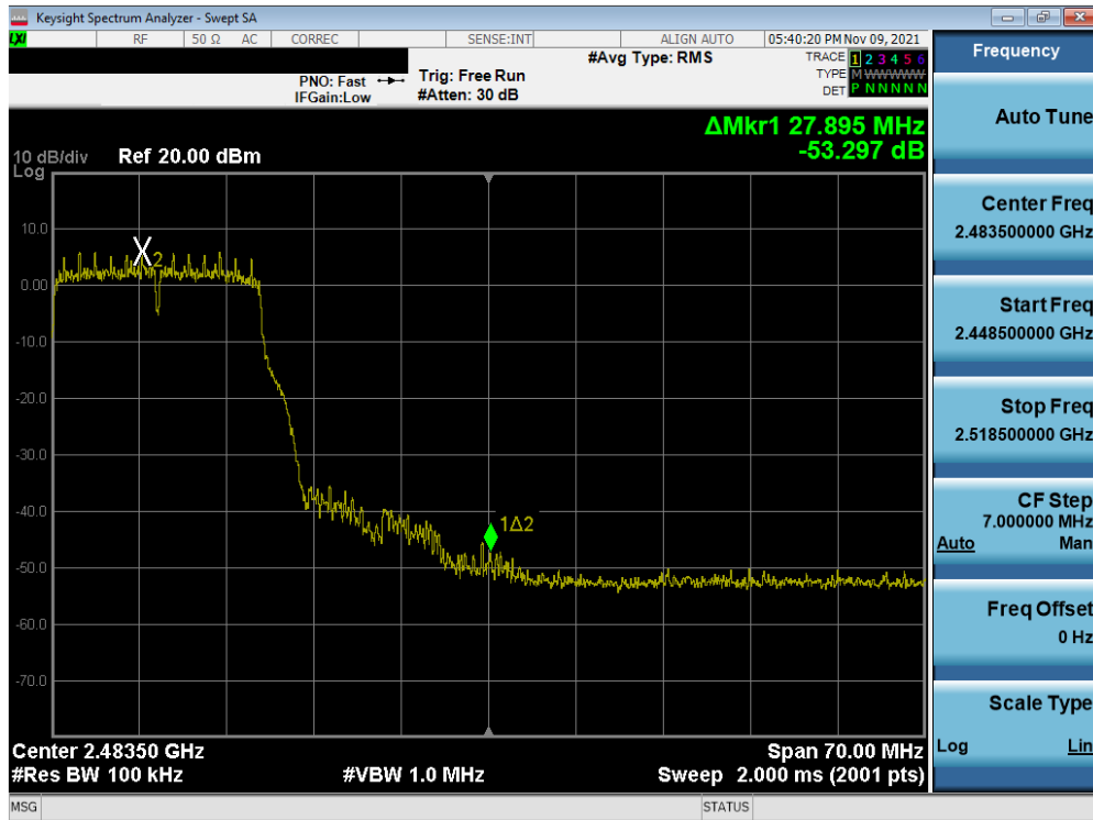
Plot 7-55. Band Edge Plot MIMO ANT1 (802.11g – Ch. 10)
