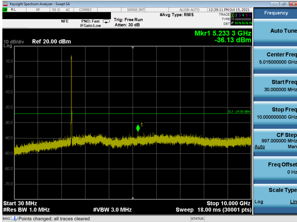
Plot 7-93. Conducted Spurious Plot MIMO ANT1 (802.11g – Ch. 6)
