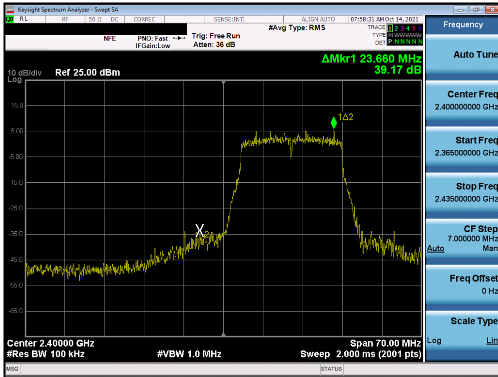
Plot 7-57. Band Edge Plot MIMO ANT1 (802.11n (2.4GHz) – Ch. 1)
