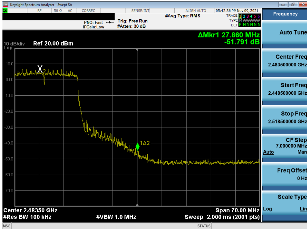
Plot 7-64. Band Edge Plot MIMO ANT1 (802.11ax (2.4GHz) – Ch. 10)
