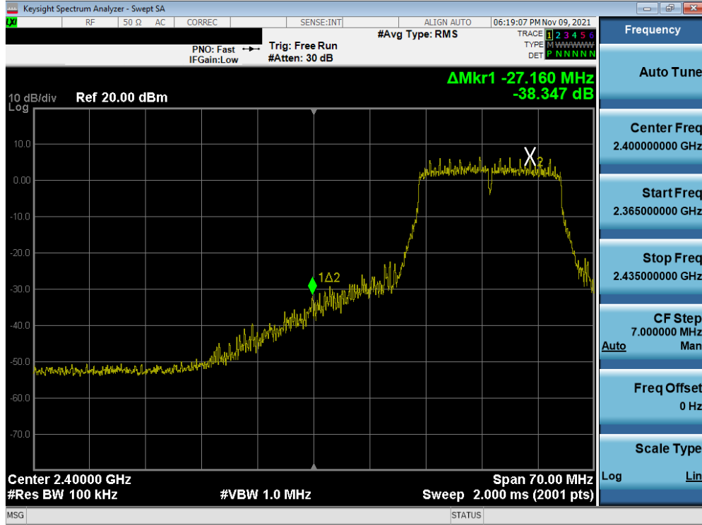
Plot 7-76. Band Edge Plot MIMO ANT2 (802.11ax (2.4GHz) – Ch. 3)
