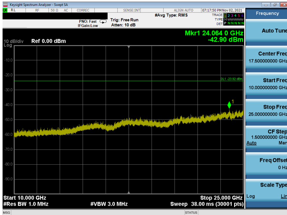
Plot 7-92. Conducted Spurious Plot MIMO ANT1 (802.11g - Ch. 1)
