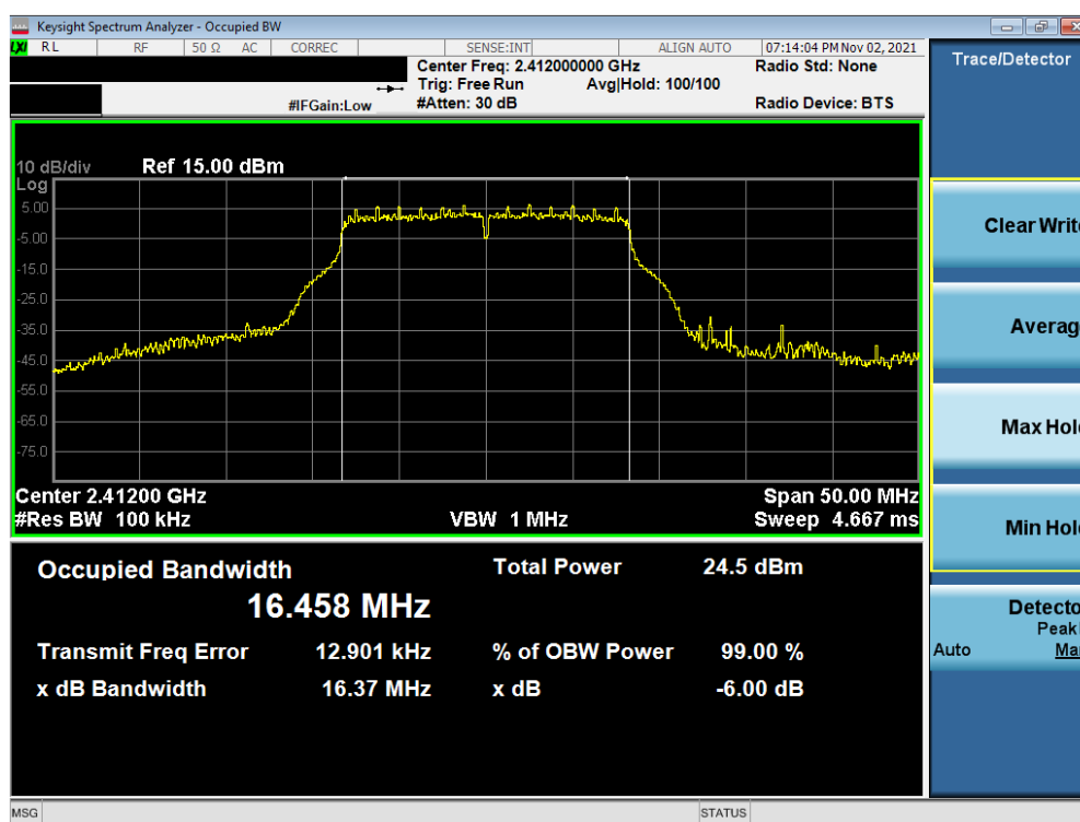
Plot 7-7. 6dB Bandwidth Plot MIMO ANT1 (802.11g – Ch. 1)
