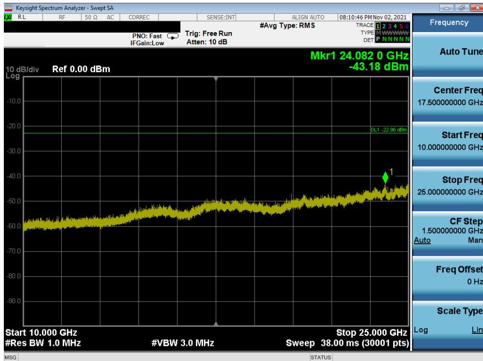
Plot 7-102. Conducted Spurious Plot MIMO ANT2 (802.11g – Ch. 11)
