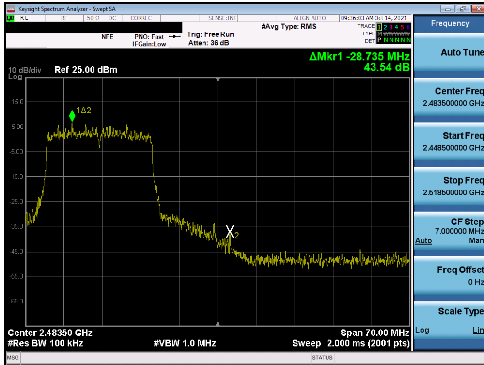
Plot 7-65. Band Edge Plot MIMO ANT1 (802.11ax (2.4GHz) – Ch. 11)
