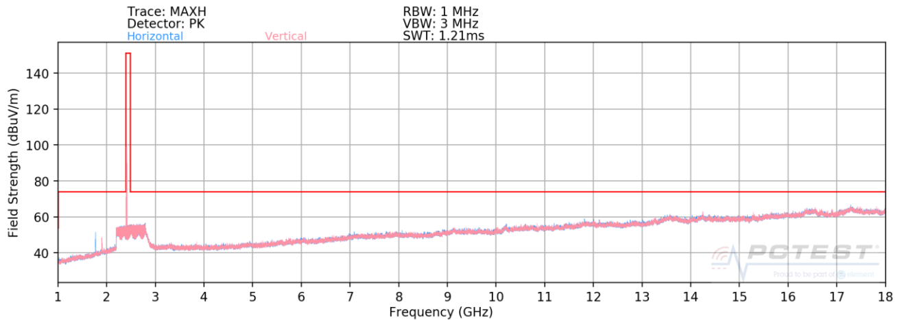
Plot 7-103. Radiated Spurious Plot above 1GHz SISO ANT1 (802.11b – Ch. 1)
