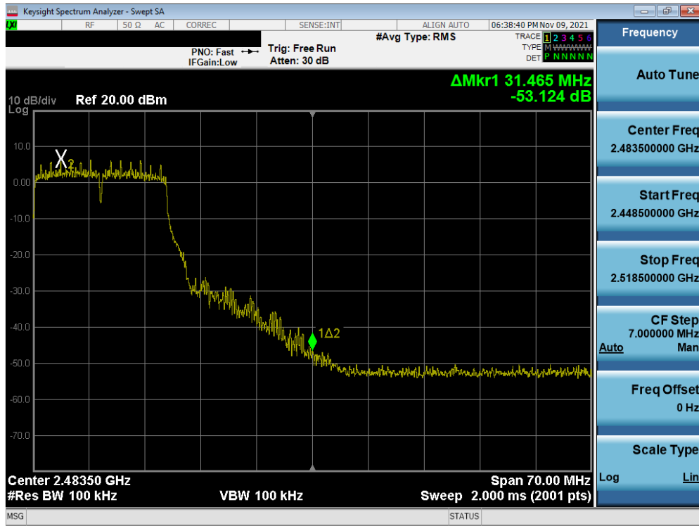
Plot 7-68. Band Edge Plot MIMO ANT2 (802.11g – Ch. 10)
