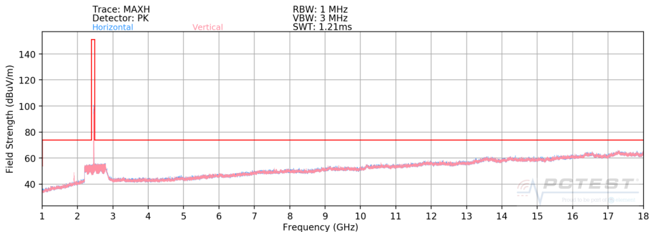
Plot 7-105. Radiated Spurious Plot above 1GHz SISO ANT1 (802.11b – Ch. 11)
