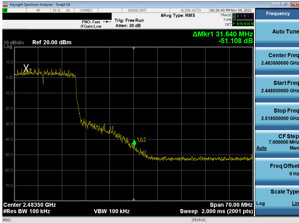
Plot 7-77. Band Edge Plot MIMO ANT2 (802.11ax (2.4GHz) – Ch. 10)
