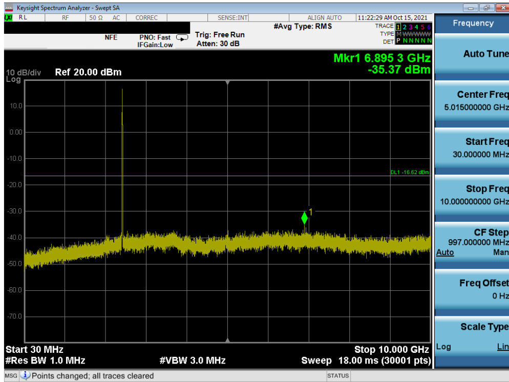
Plot 7-81. Conducted Spurious Plot SISO ANT1 (802.11b – Ch. 6)
