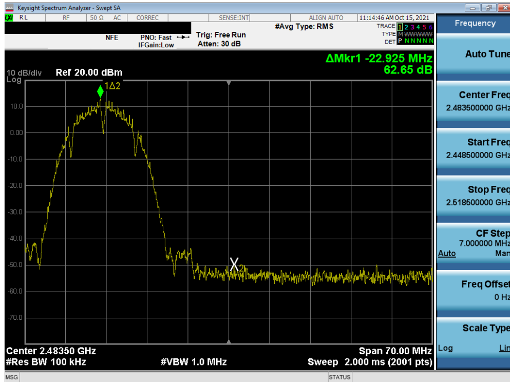
Plot 7-52. Band Edge Plot SISO ANT2 (802.11b – Ch. 11)
