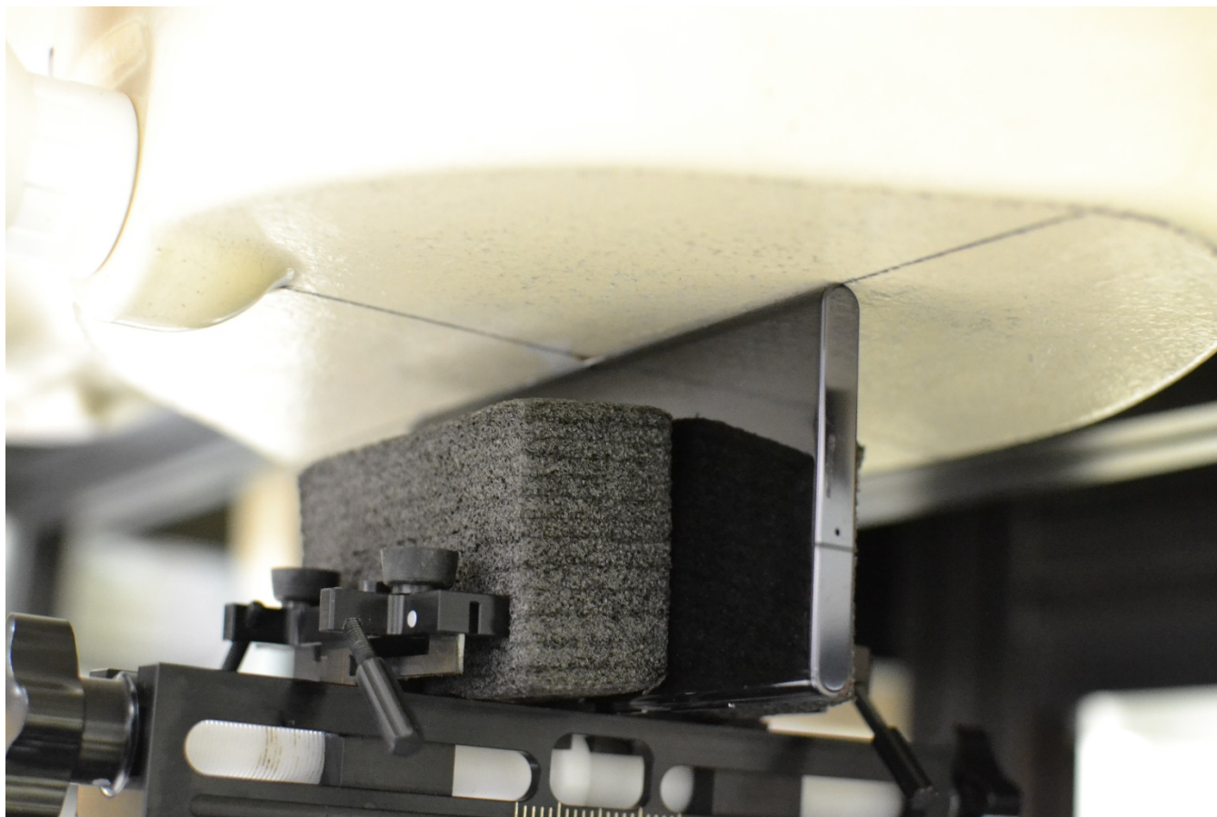
Figure C-10 SAR Test Setup Photo – Phablet, Left Edge at 0 mm
