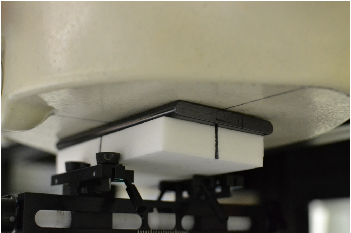
Figure C-8 SAR Test Setup Photo – Phablet, Back Side at 0 mm
