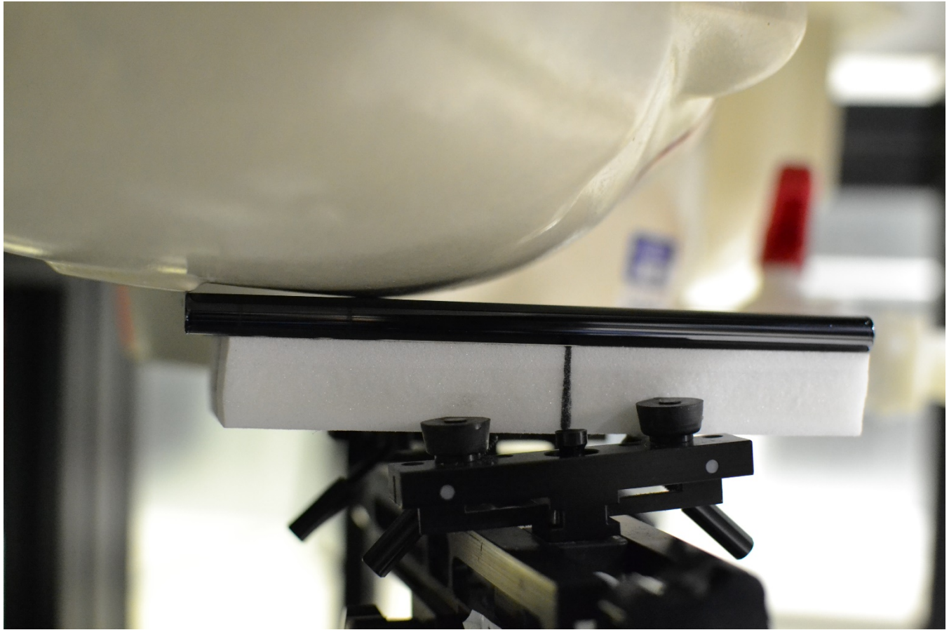
Figure C-3 SAR Test Setup Photo – Head Right, Cheek at 0 mm
