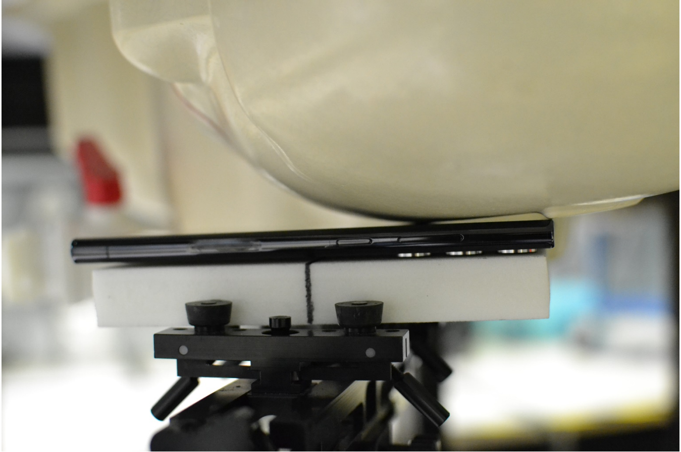
Figure C-5 SAR Test Setup Photo – Head Left, Cheek at 0 mm
