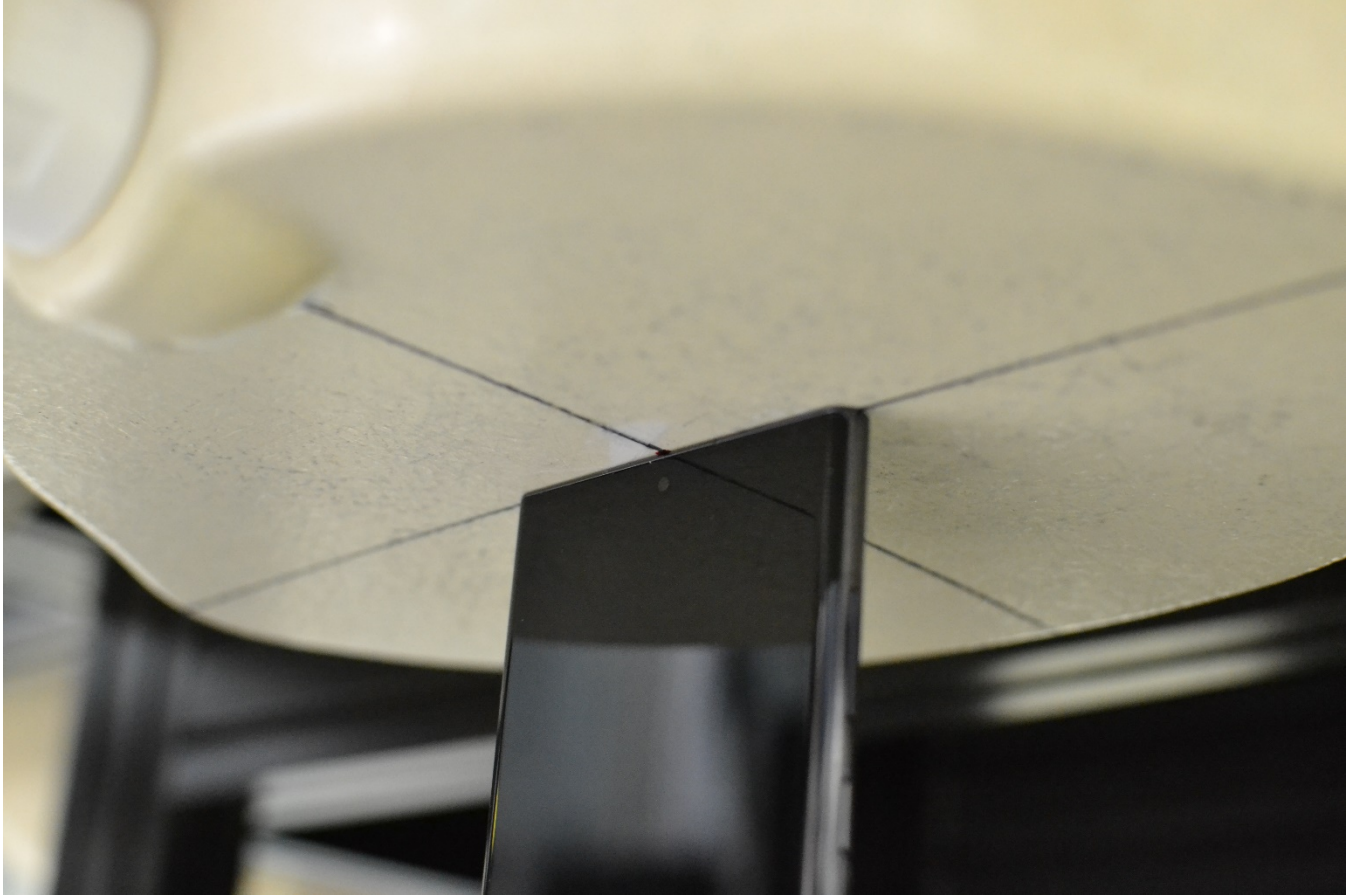
Figure C-11 SAR Test Setup Photo – Phablet, Top Edge at 0 mm
