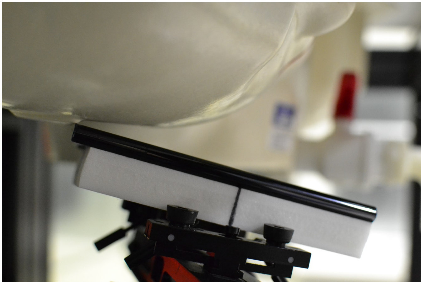
Figure C-4 SAR Test Setup Photo – Head Right, Tilt at 0 mm
