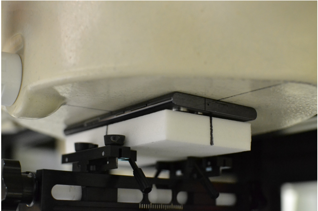
Figure C-9 SAR Test Setup Photo – Phablet, Front Side at 0 mm
