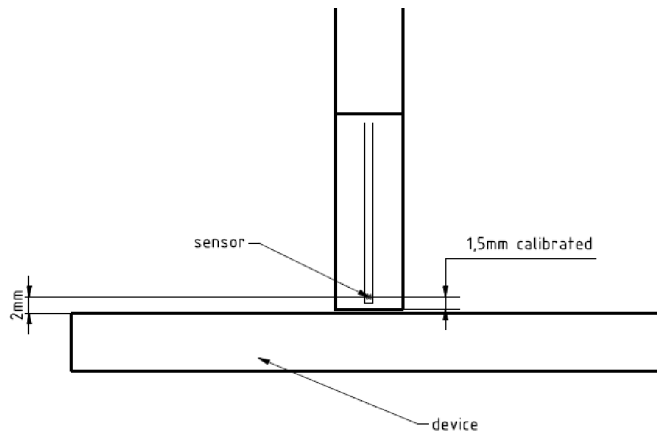
Figure C-2 EUMmWVx Probe
