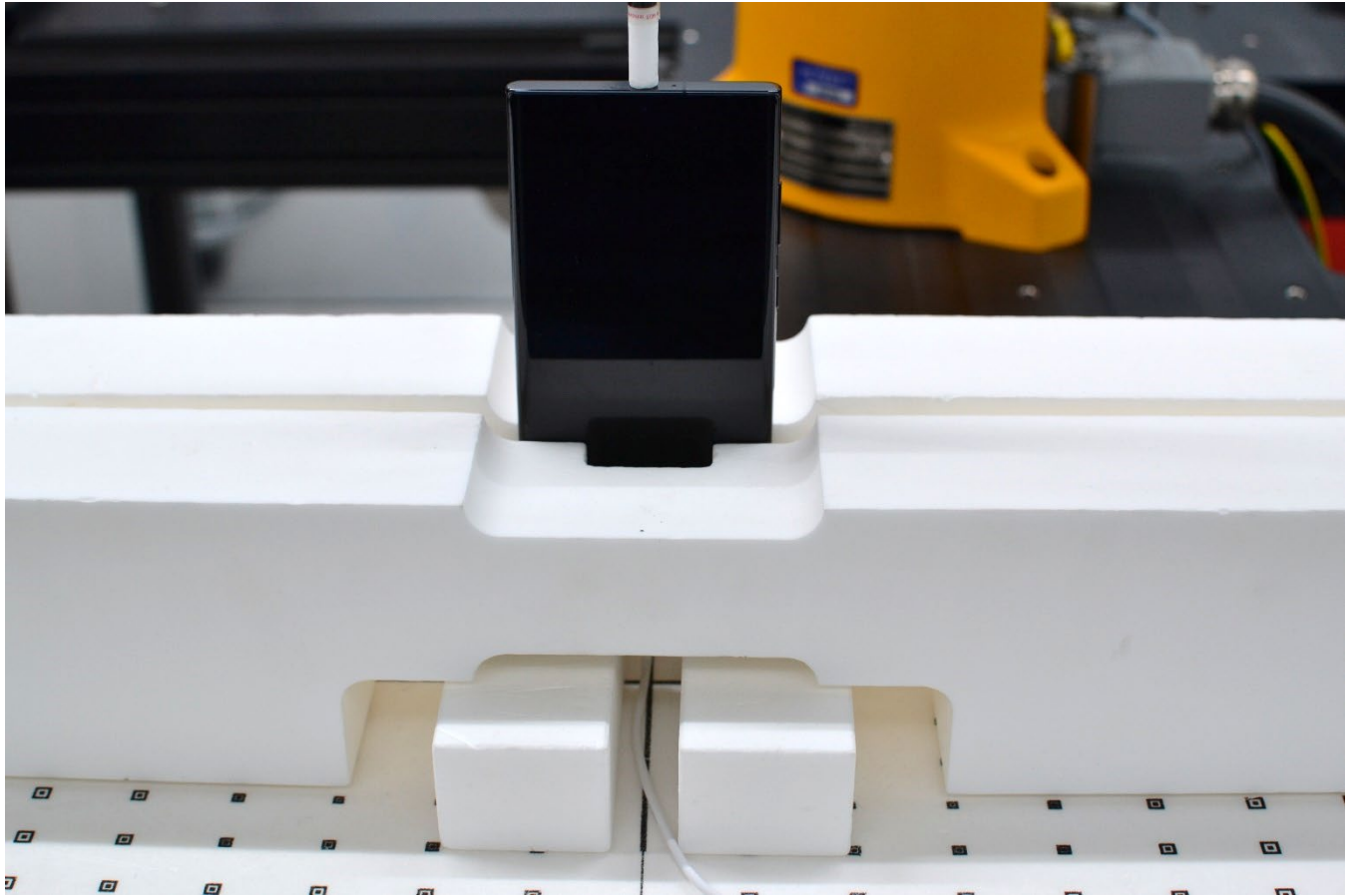
Figure C-15 Near Field Power Density Test Setup Photo – Top Edge at 2 mm
