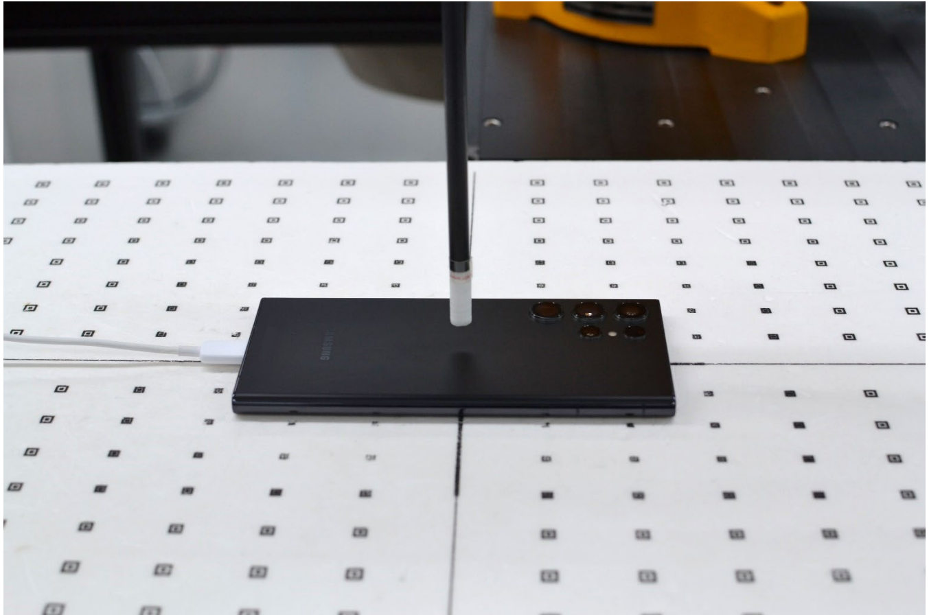
Figure C-16 Near Field Power Density Test Setup Photo – Back Side at 9.51 mm
