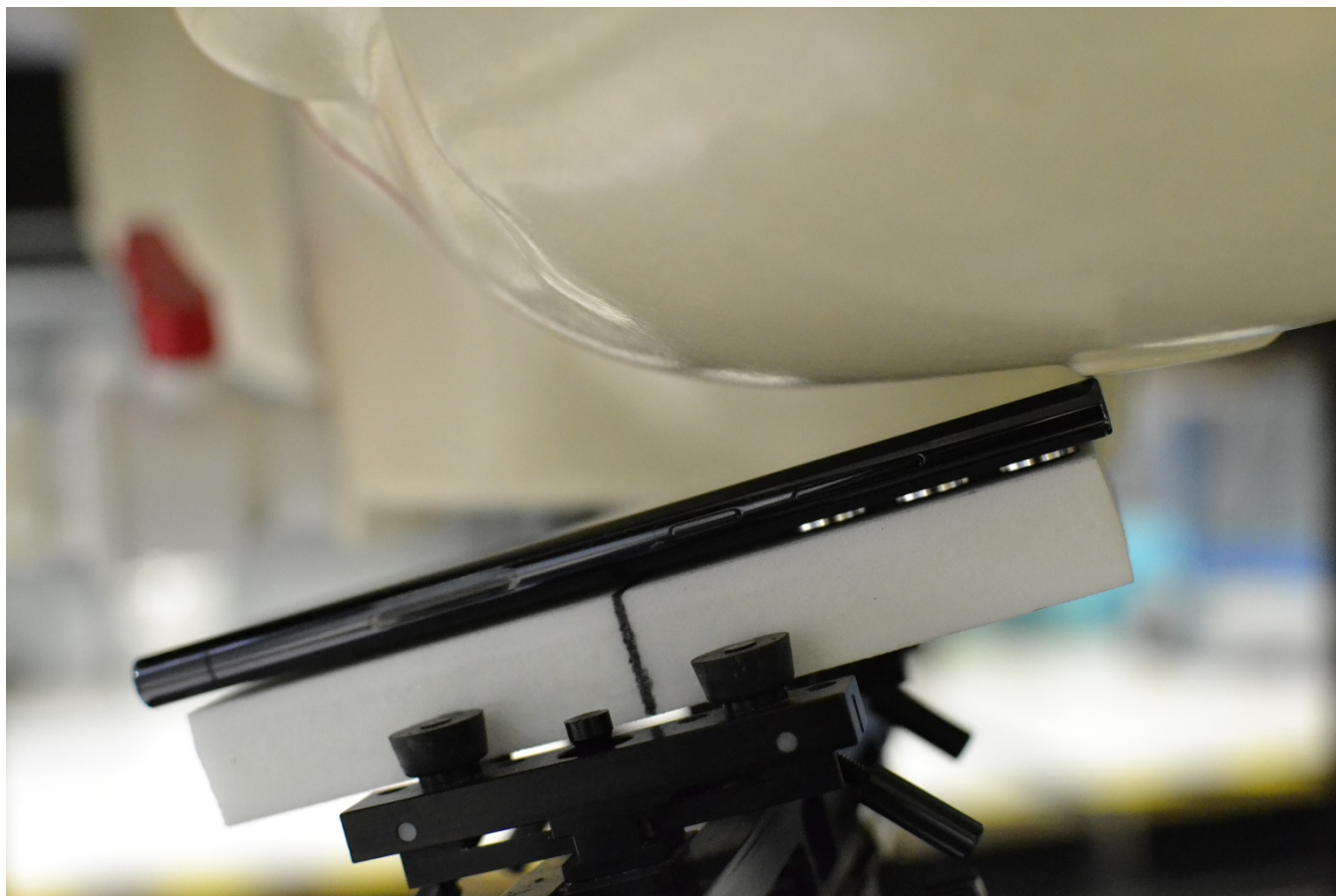
Figure C-6 SAR Test Setup Photo – Head Left, Tilt at 0 mm
