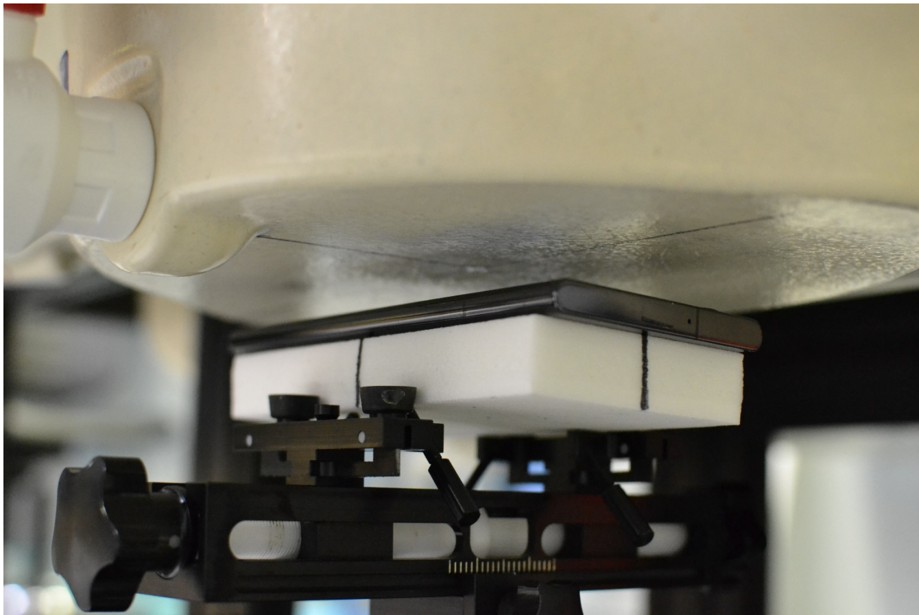
Figure C-7 SAR Test Setup Photo – Bodyworn, Back Side at 15 mm
