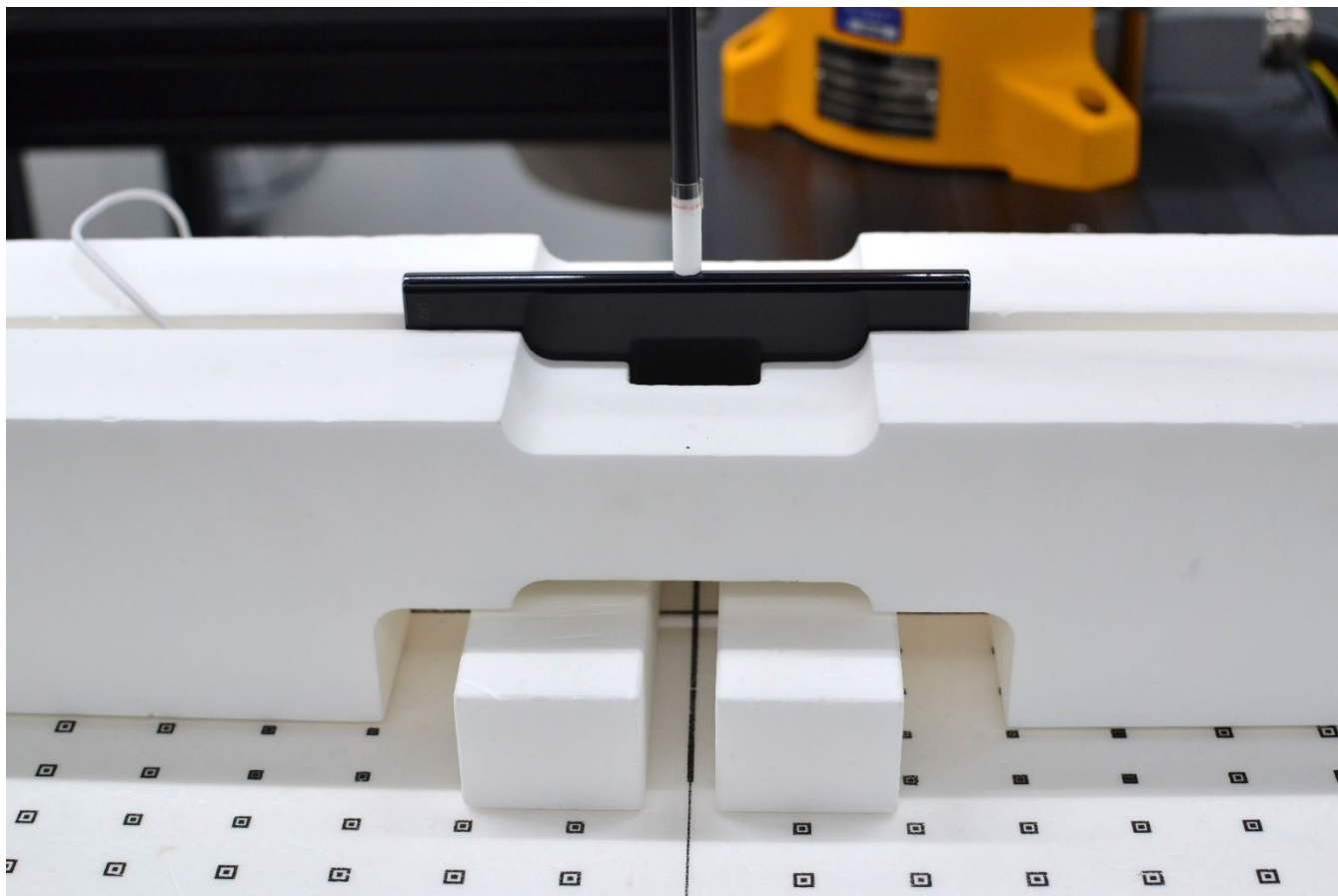
Figure C-14 Near Field Power Density Test Setup Photo – Left Edge at 2 mm
