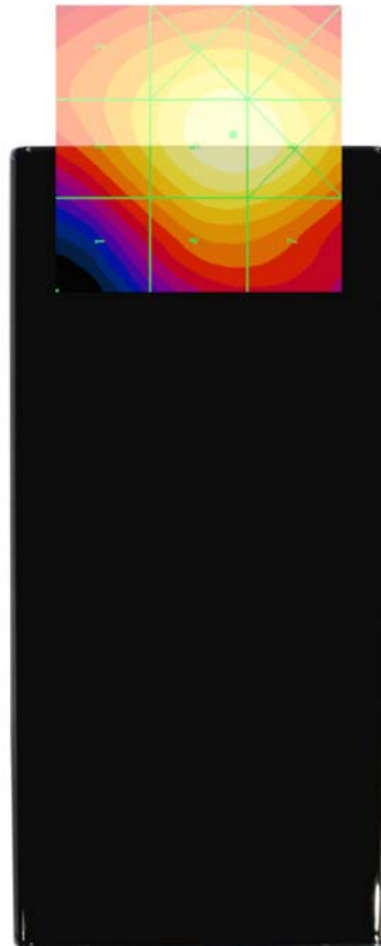
Figure 17-4 E-Field WD Scan overlay
