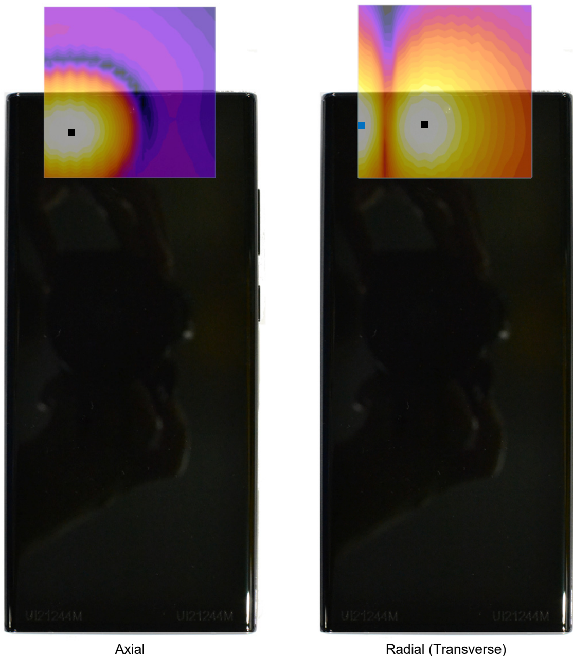
Figure 17-3 T-Coil Scan Overlay Magnetic Field Distributions
