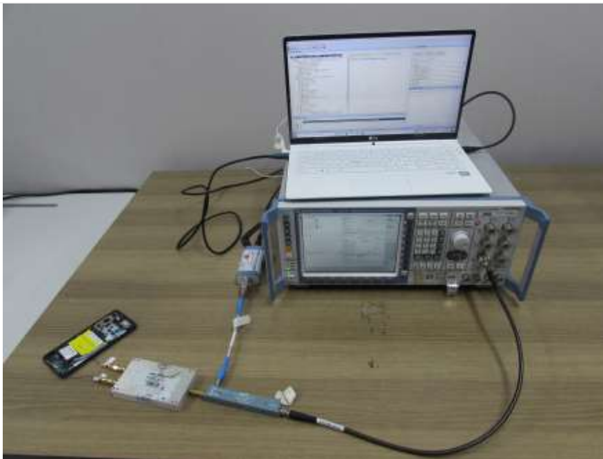
Test setup photo-2 (7-1(b) (Legacy Antenna Switch))
