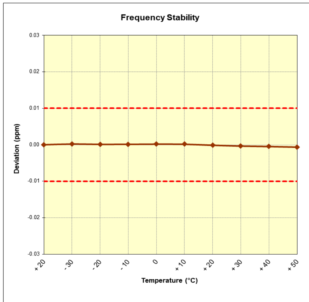
Figure 7-3. Frequency Stability Plot
