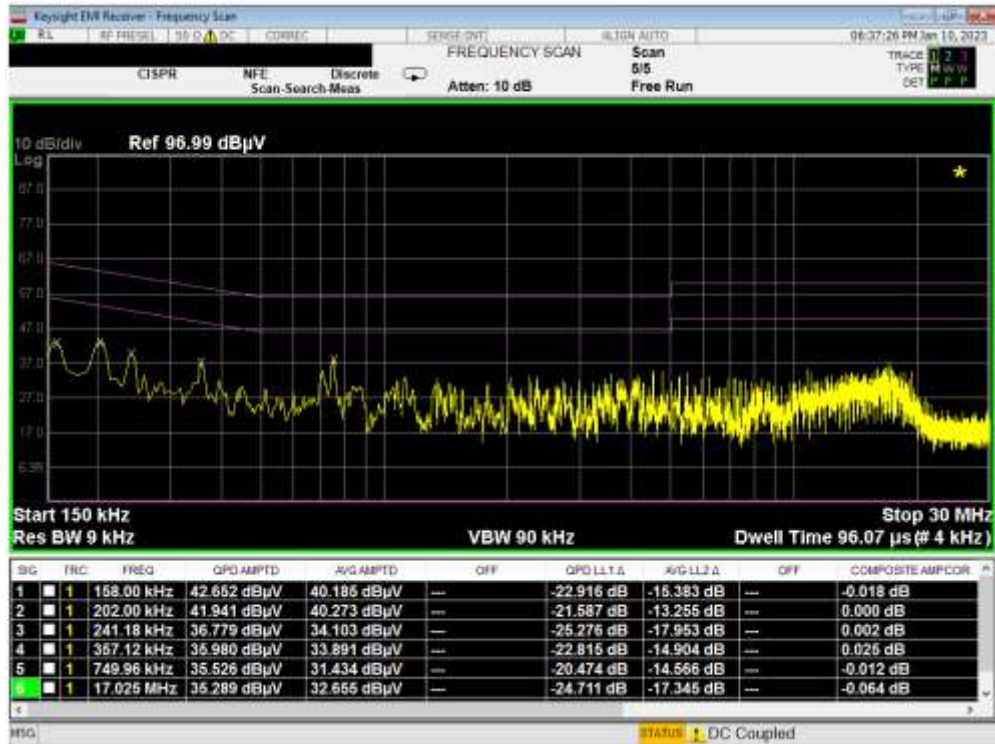
Plot 7-5. Line Conducted Plot (L1) – WCP
