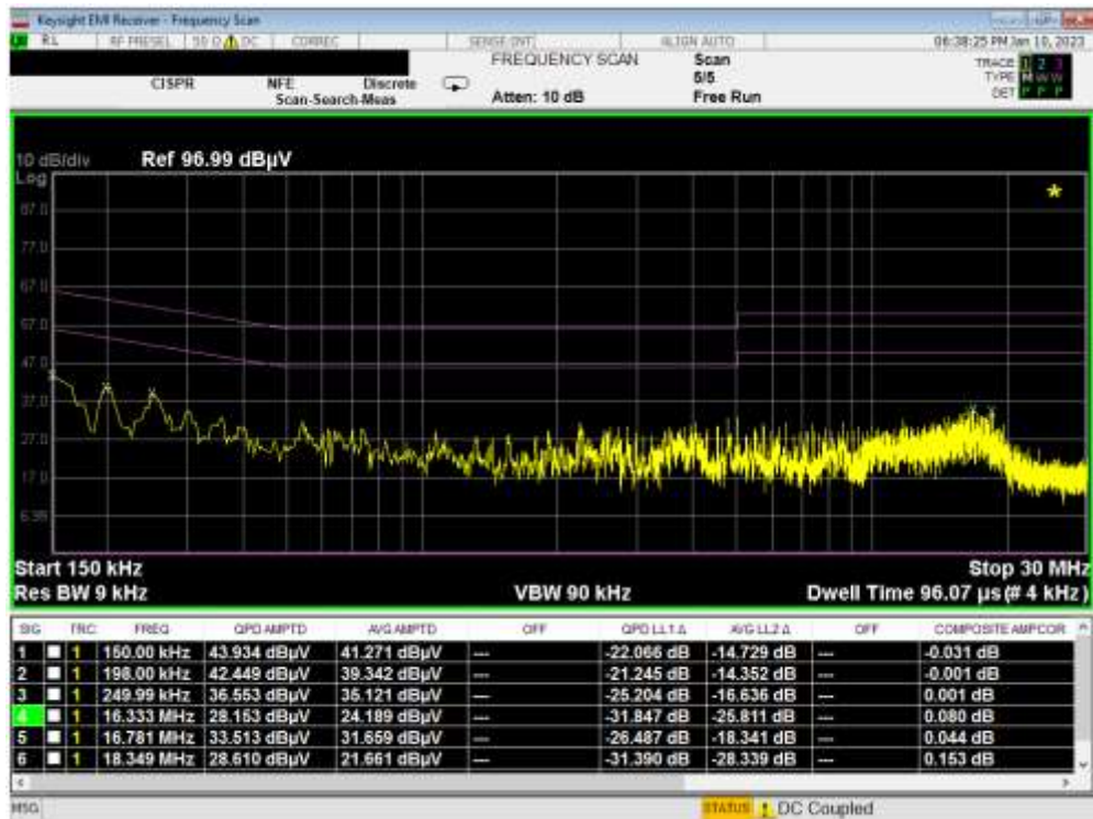
Plot 7-6. Line Conducted Plot (N) – WCP
