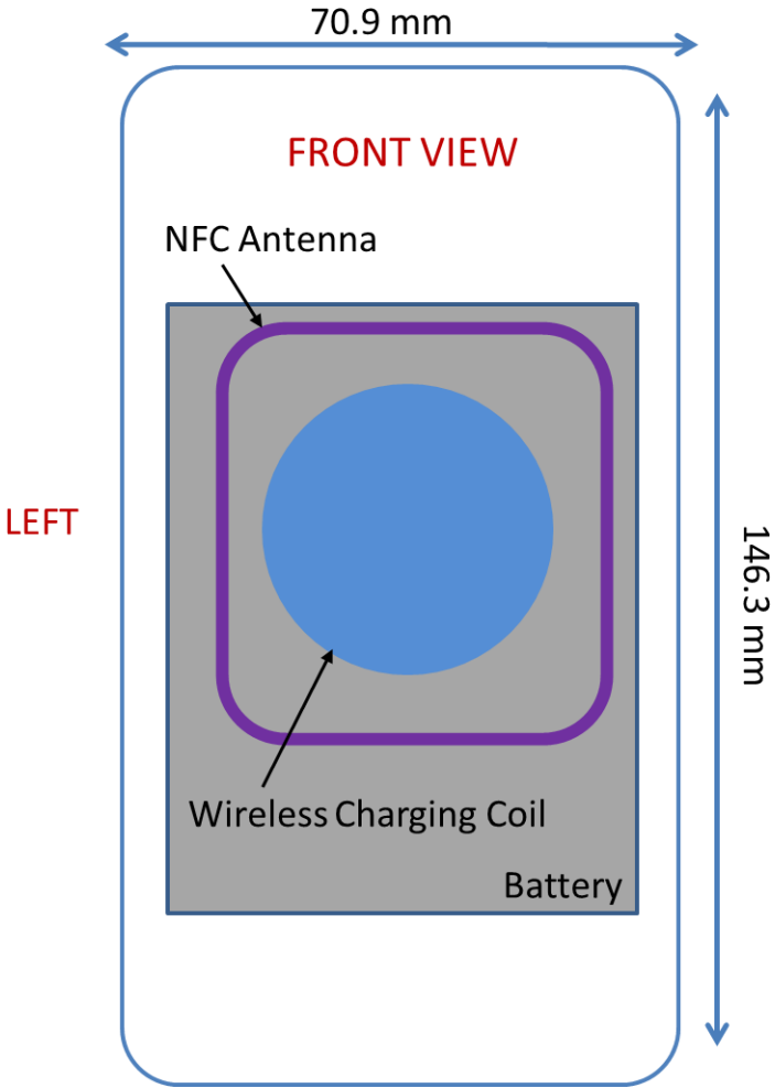
Figure K-2 NFC Antenna Locations
