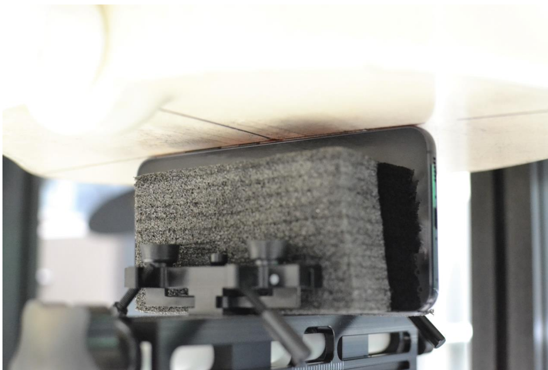
SAR Test Setup Photo 15 – Phablet, Right Edge at 0mm
