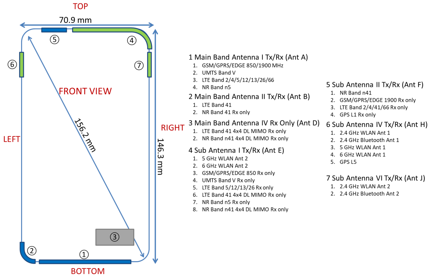
Figure K-1 DUT Antenna Locations
