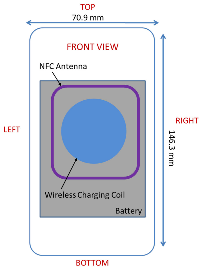
Figure H-2 NFC Antenna Locations
