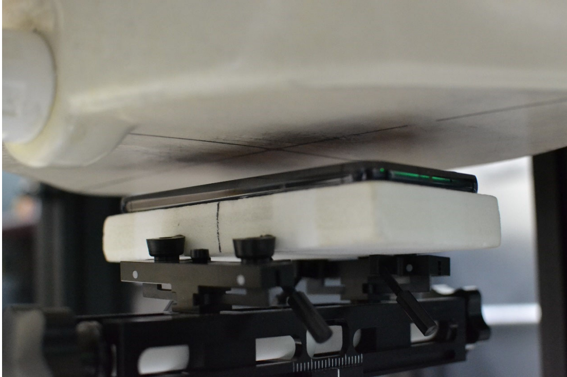
SAR Test Setup Photo 1 – Body-worn, Back Side at 15mm
