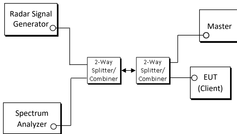
Figure 8-1. Test Setup
