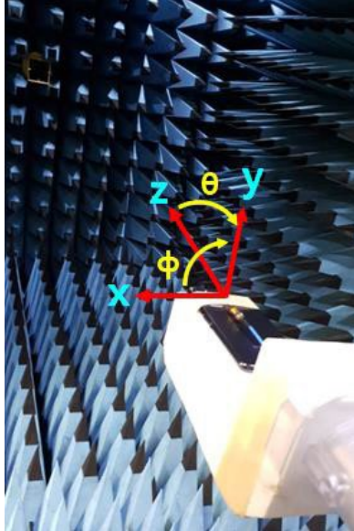
Figure 1: Geometry for SC-52D , SCG20 for Radiation patterns.
