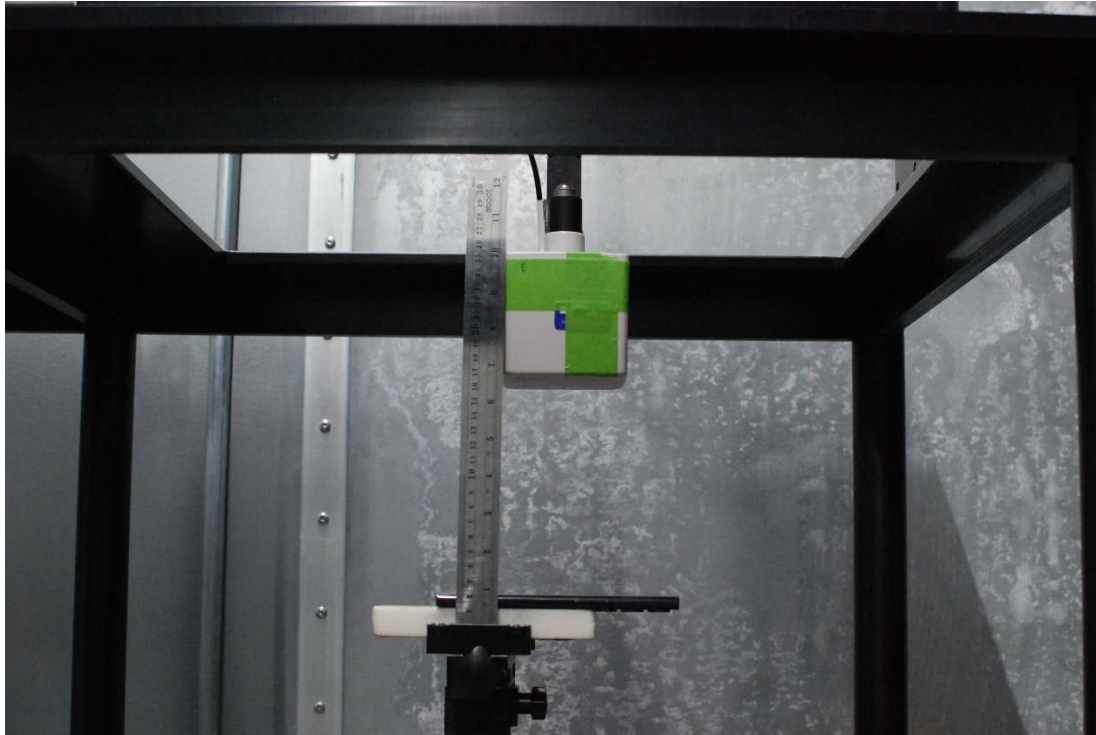
Test Setup Photo 3 H-field, Front side, 15cm
