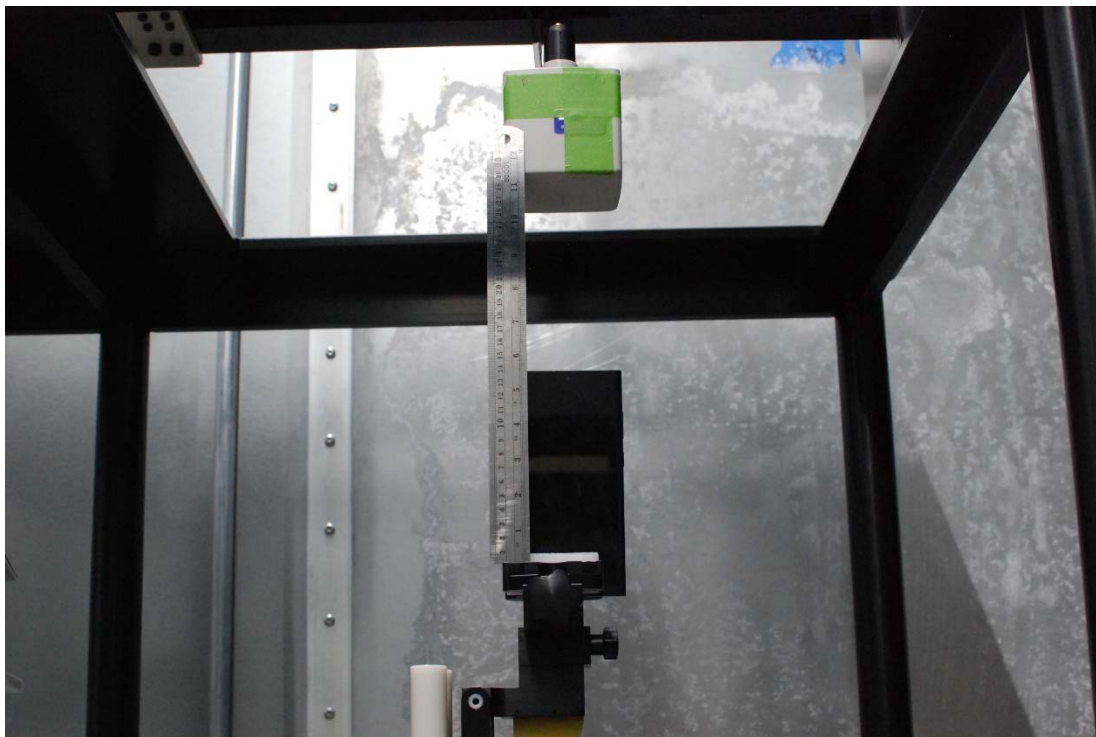
Test Setup Photo 4 H-field, Top edge, 15cm
