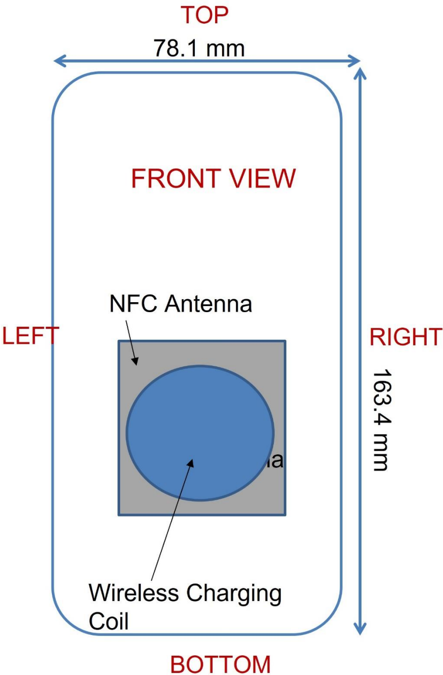
Figure K-2 NFC Antenna Locations
