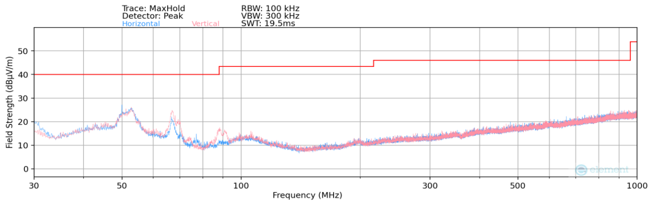
Plot 7-1. Radiated Spurious Plot below 1GHz
