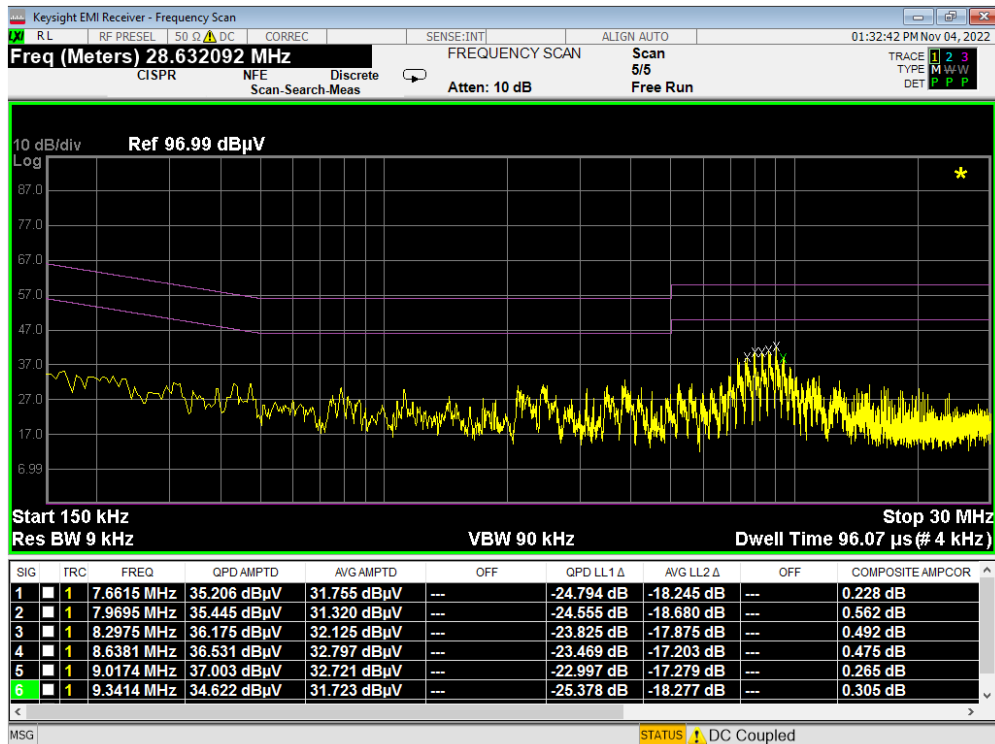
Plot 7-6. Line Conducted Plot (N) with WCP
