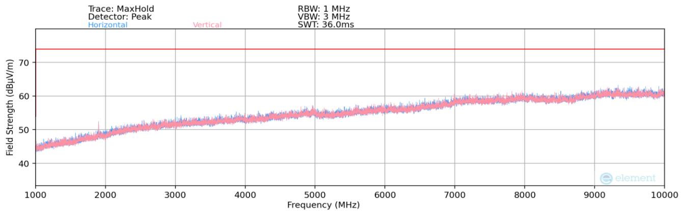
Plot 7-2. Radiated Spurious Plot above 1GHz
