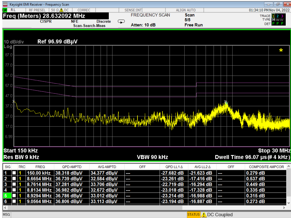
Plot 7-5. Line Conducted Plot (L1) with WCP
